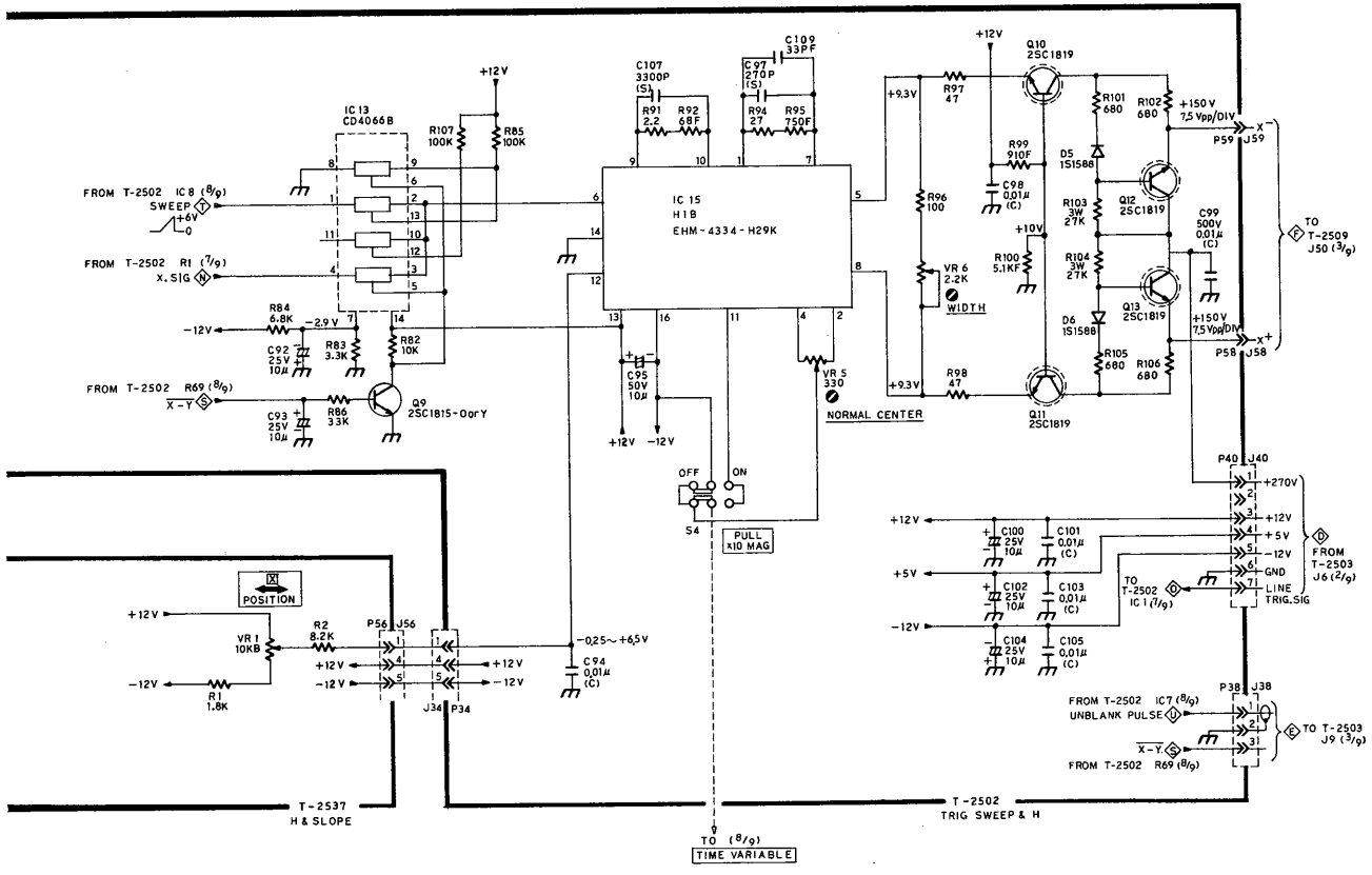
SCHMATIC Model LBO-523 O-1434 (9/9) HORIZONTAL AMP LEADER ELECTRONICS CORP.
