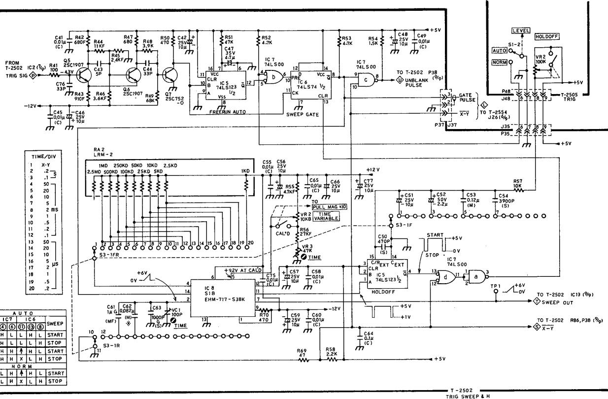
SCHMATIC Model LBO-523 O-1434 (8/9) SWEEP LEADER ELECTRONICS CORP.
