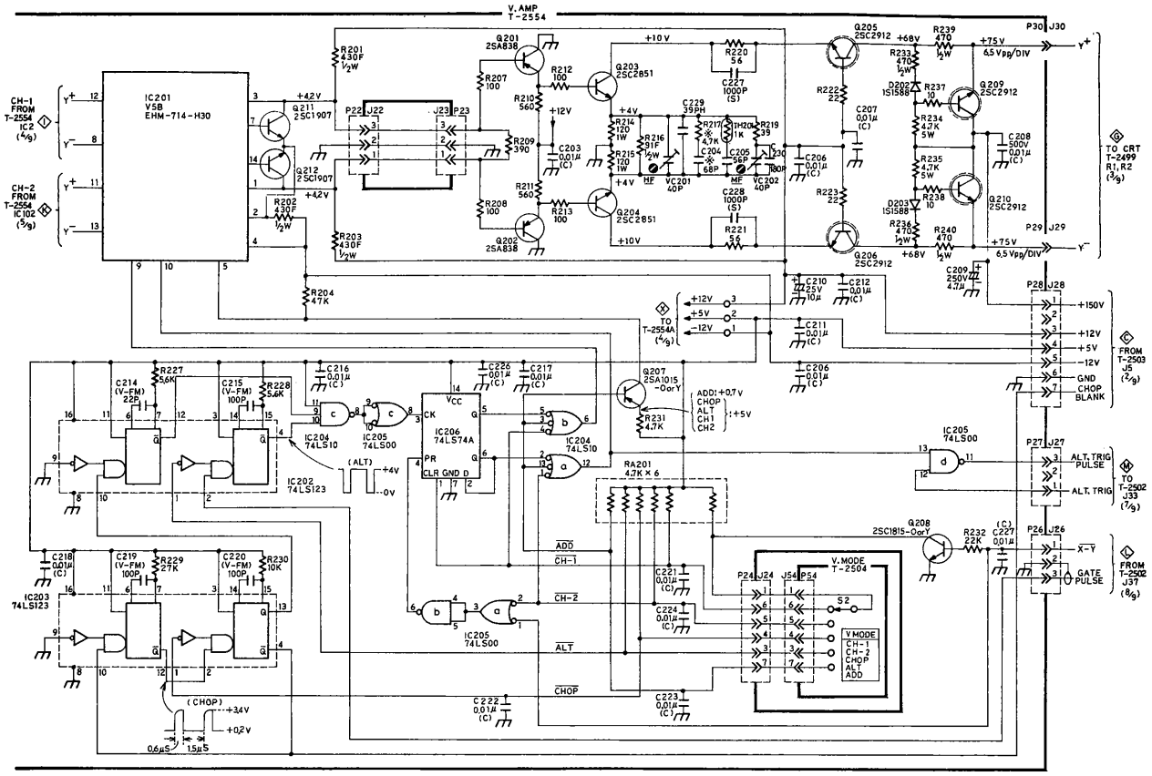
SCHMATIC Model LBO - 522 O - 1433 (7%) VERT. MODE & FINAL AMP LEADER ELECTRONICS CORP.
