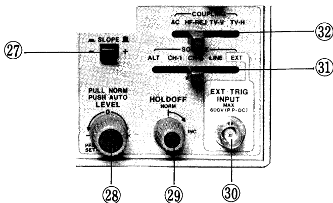
[Synchronizing Block]
