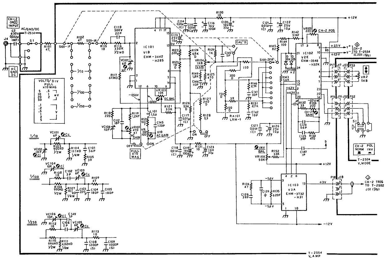
SCHMATIC Model LBO-523 O-1434 (5/9) VERT. PREAMP(CH-2) LEADER ELECTRONICS CORP.
