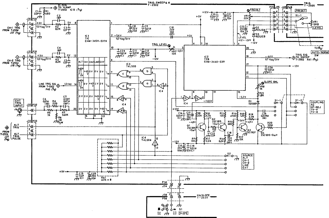
SCHMATIC Model LBO - 522 O - 1433 (7%) TRIG. AMP LEADER ELECTRONICS CORP.
