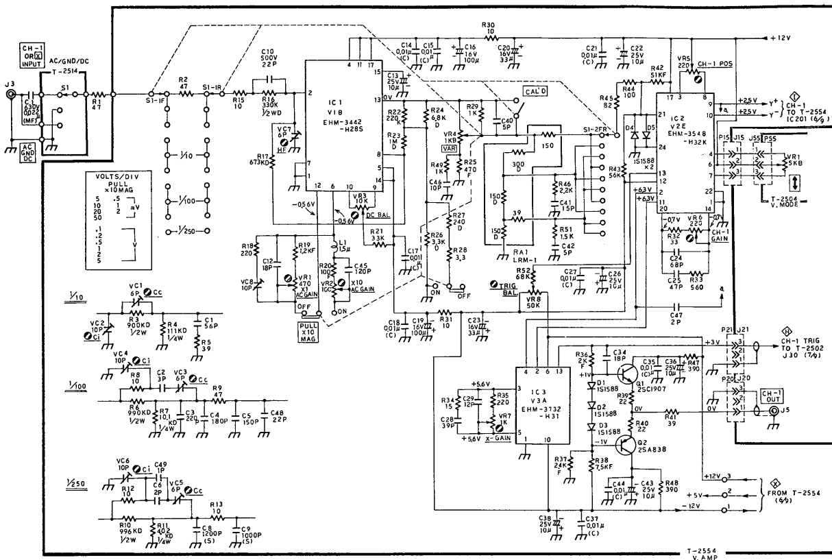
SCHMATIC Model LBO-523 O-1434 (1/9) VERT. PREAMP(CH-1) LEADER ELECTRONICS CORP.
