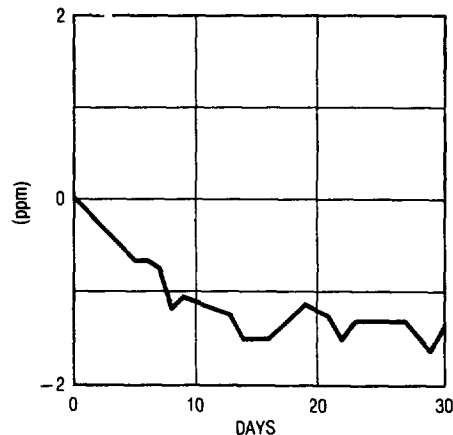
LONG TERM STABILITY OF A TYPICAL DEVICE FROM TIME = 0 WITH NO PRECONDITIONING OR AGING
