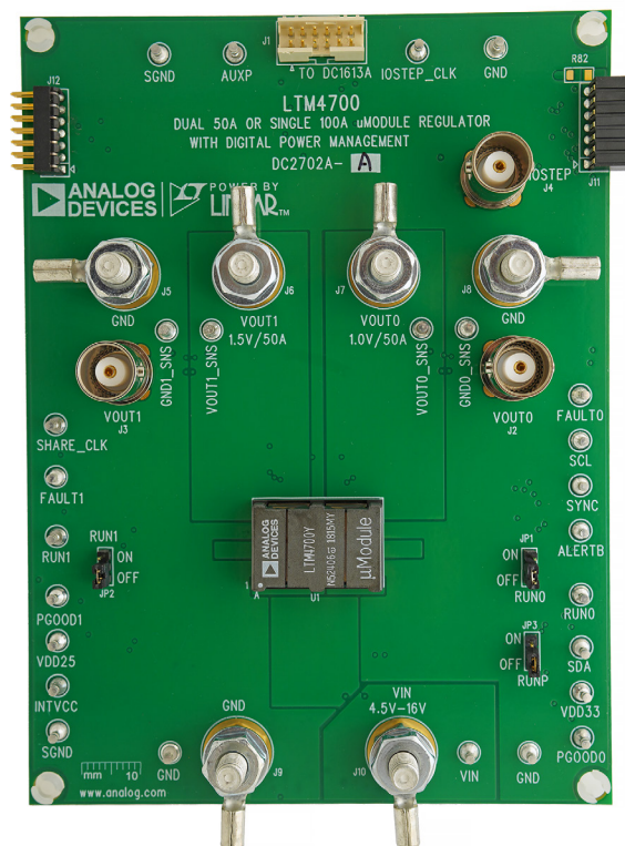
Figure 1. Dual-Output LTM4700/DC2702A-A Demo Circuit
