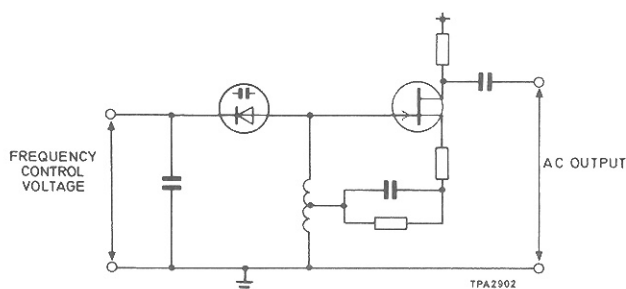
Fig. 3.1 Oscillator circuit
