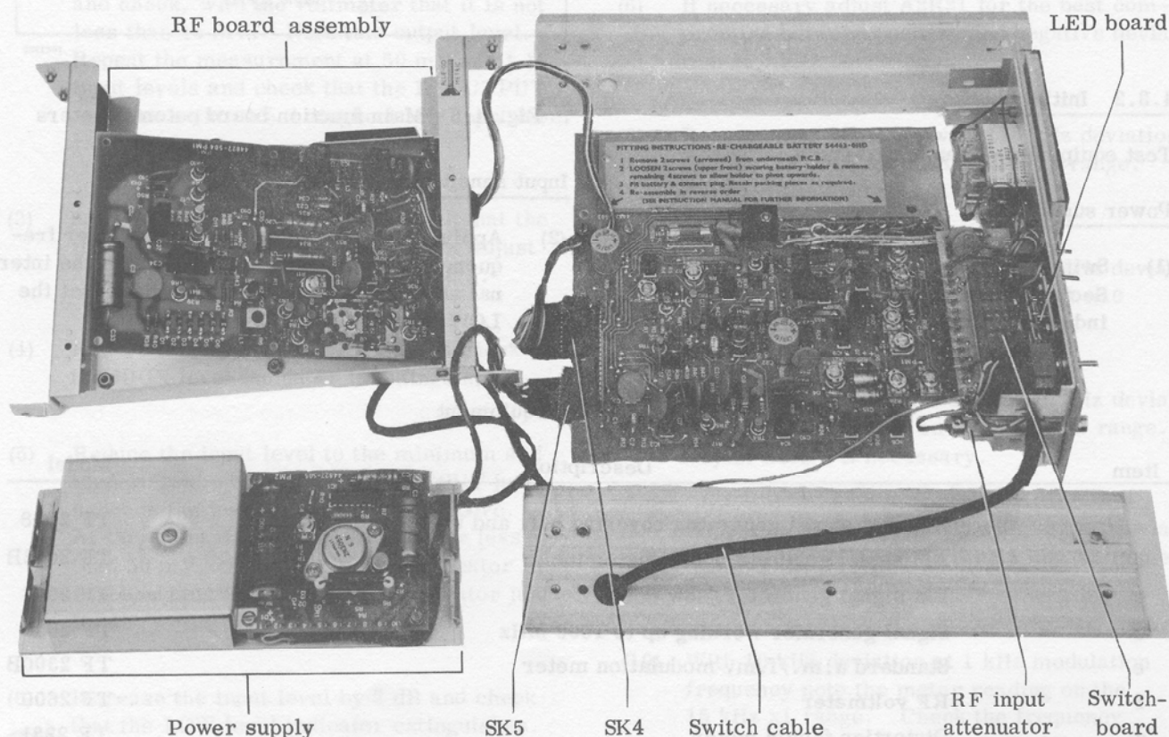
Fig. 4.2 TF 2304 - dismantled
