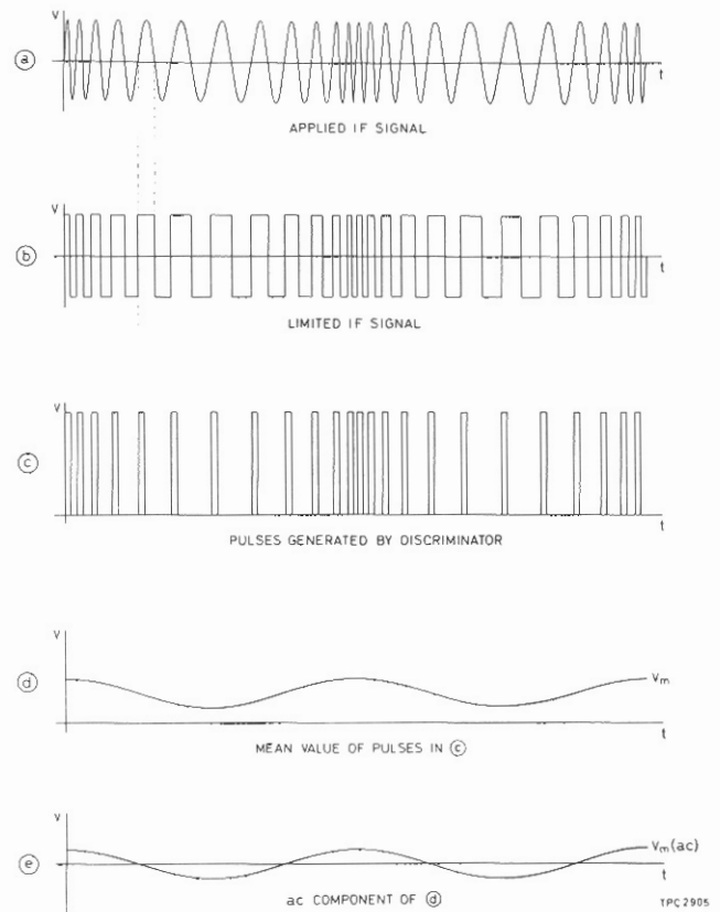
Fig. 3.2 FM demodulation
