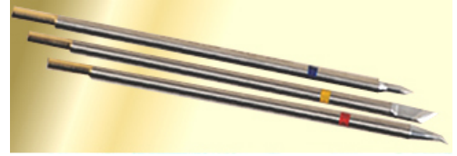
Here's the New Line of Heater Tip Cartridges Featuring Color-Coded Temperature Bands From EasyBraid Announcing that "Works With MX Soldering Stations" Blue: 600° Series, Yellow: 700° Series, Red: 800° Series
