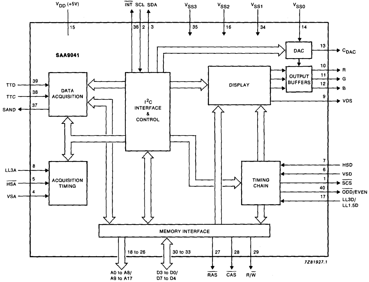
Fig. 1 Block diagram.
