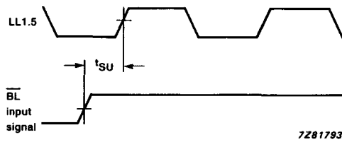
Fig. 7 \overline{BL} timing waveform; 50/60 Hz picture frequency; f = 27 MHz.
