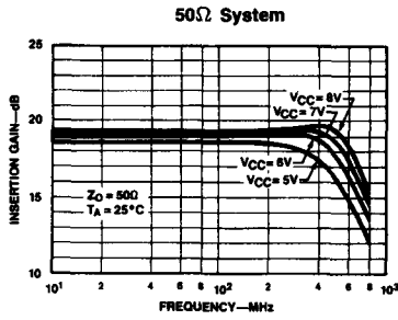
a. Insertion Gain vs Frequency ( S_{21} )
