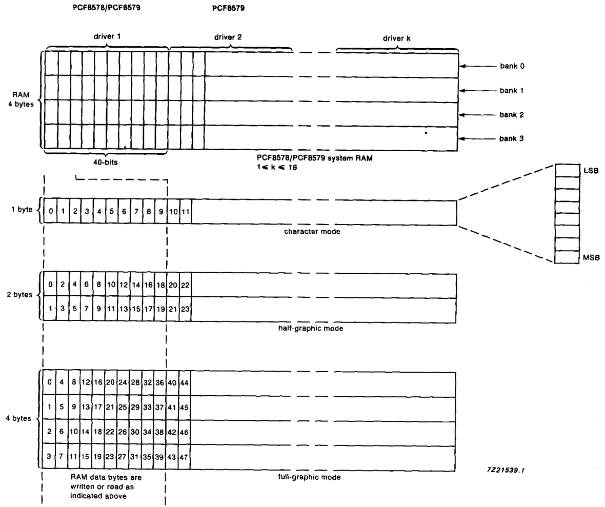
Fig.9 RAM access mode.
