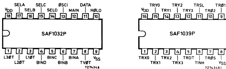
Fig. 1 Pin designations.
