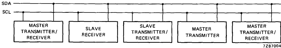
Fig.16 System configuration.
