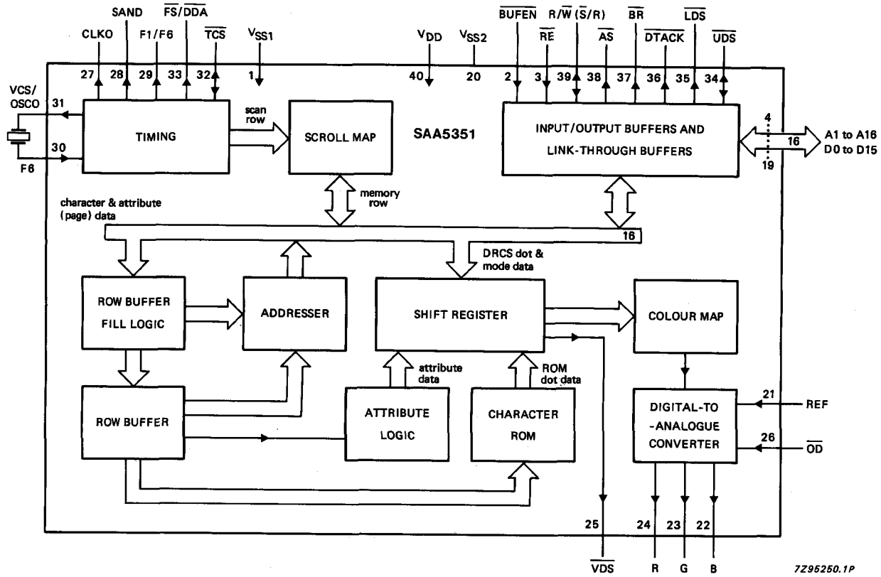
Fig. 1 Block diagram.
