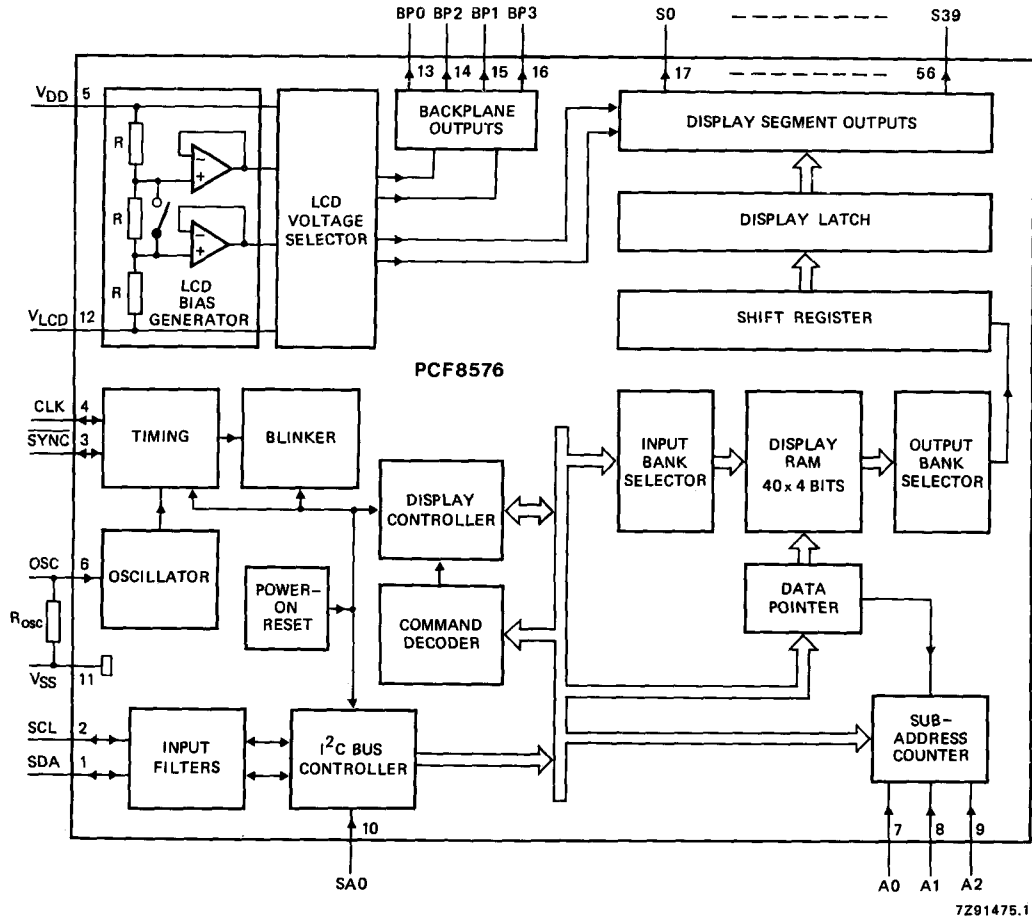
Fig. 1 Block diagram.
