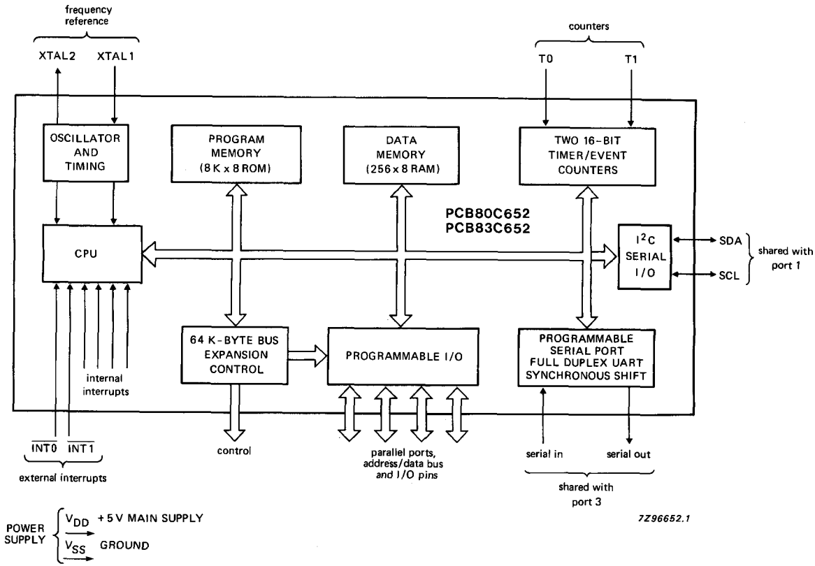
Fig. 1 Block diagram.
