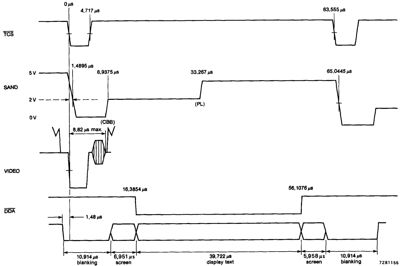
Fig. 12 Timing of synchronization and blanking outputs; all timings are nominal and assume f_{FG} = 6,041957 \text{ MHz} .
