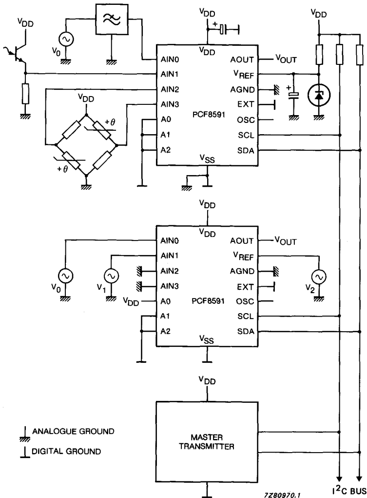
Fig. 18 Application diagram.
