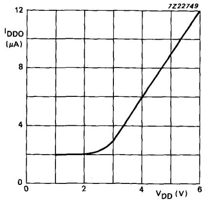
Fig.18 Typical supply current as a function of supply voltage (clock); T_{\text{amb}} = -40 to +85 °C.
