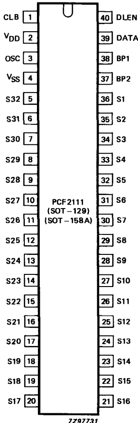
Fig. 7 Pinning diagram; PCF2111
