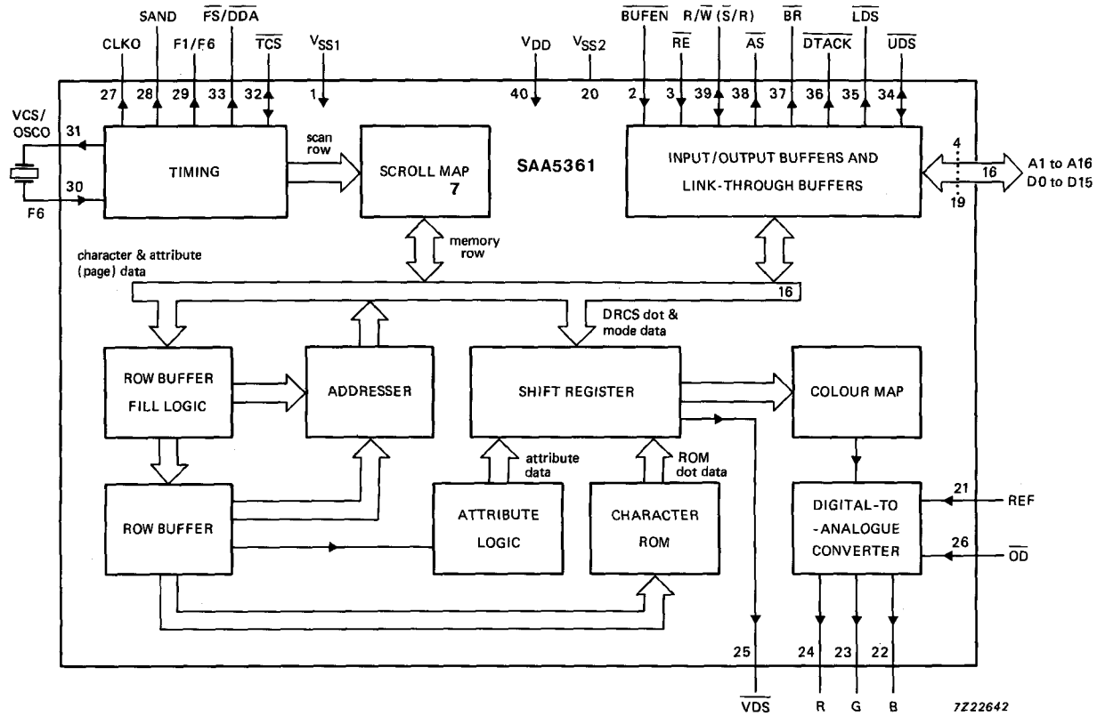
Fig. 1 Block diagram.
