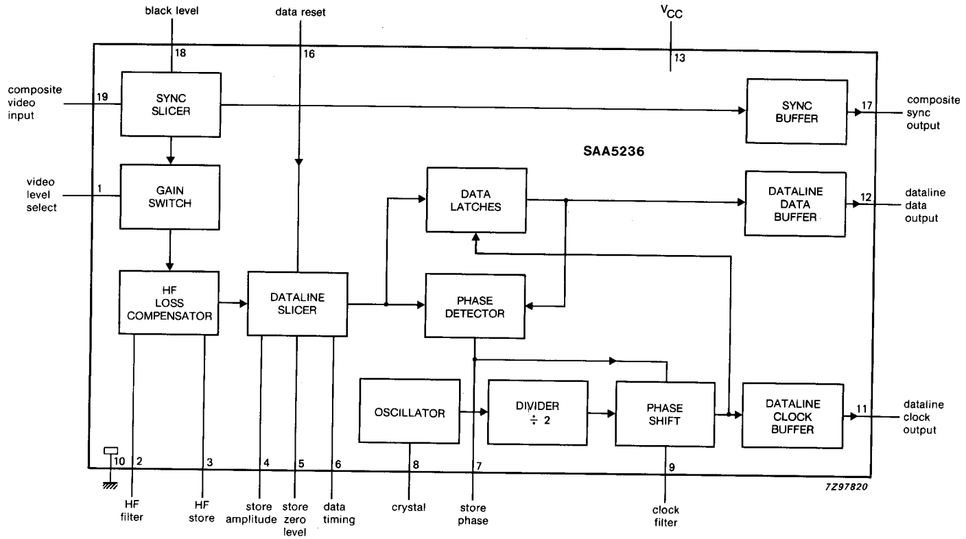
Fig. 1 Block diagram.
