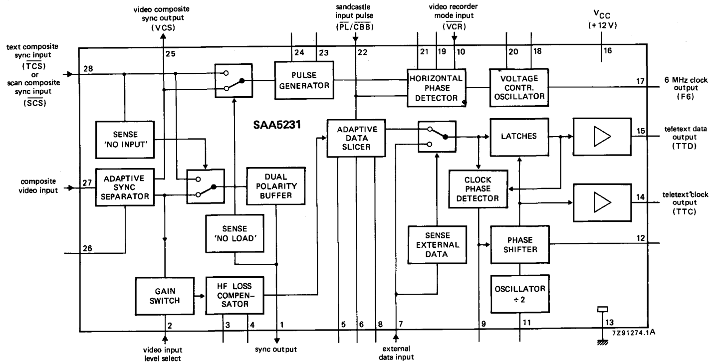
Fig. 1 Block diagram.
