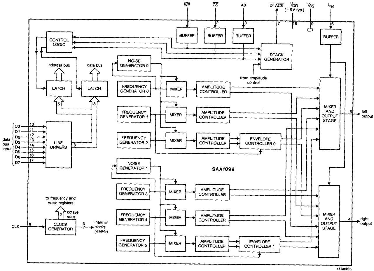
Fig. 1 Block diagram.
