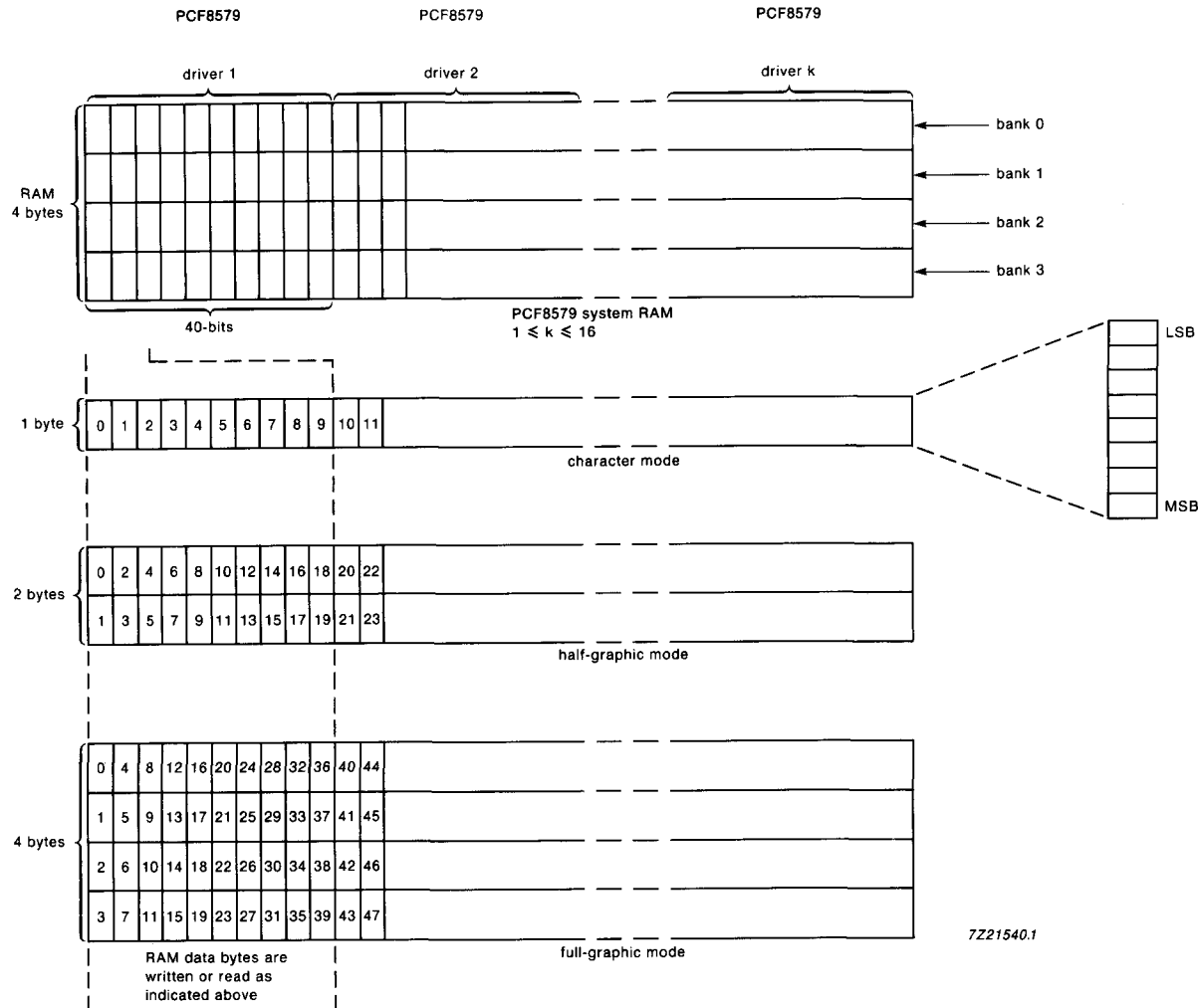
Fig.7 RAM ACCESS mode.
