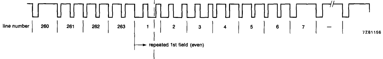
Fig. 13 Vertical synchronization and blanking waveforms; separation of broad pulses = 4,717 \mu\text{s} ; equalizing pulse widths = 2,23 \mu\text{s} .
