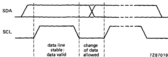
Fig.8 Bit transfer.
