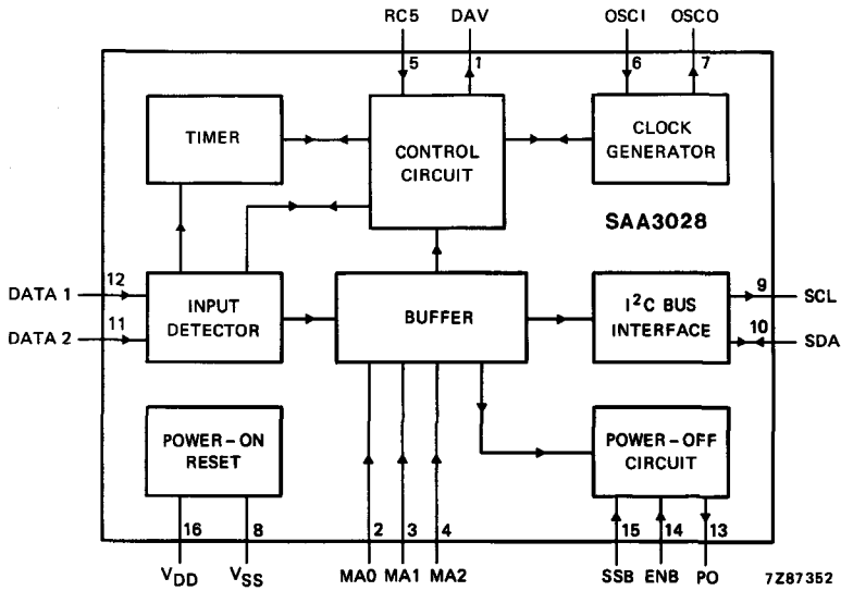
Fig. 1 Block diagram.
