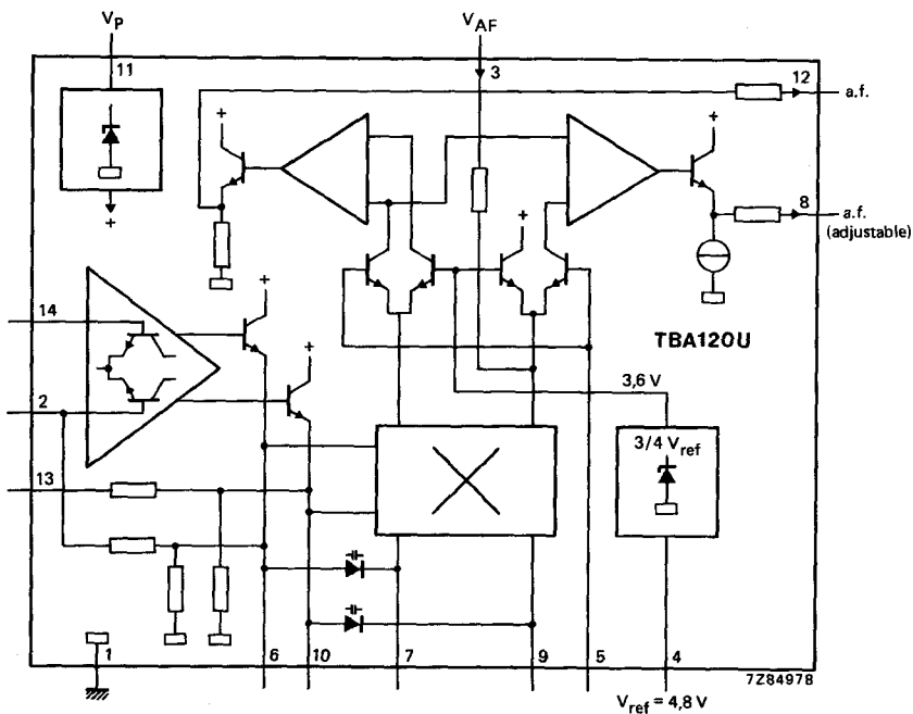
Fig. 1 Block diagram.
