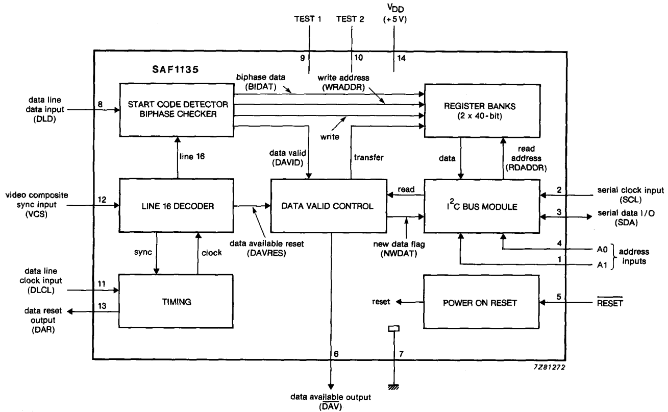
Fig. 1 Block diagram.
