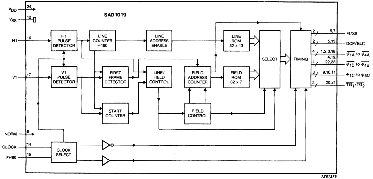
Fig.1 Block diagram.
