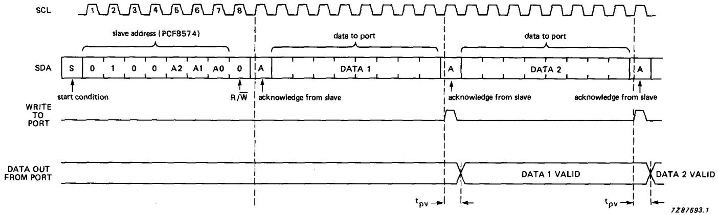
Fig.10 WRITE mode (output port).
