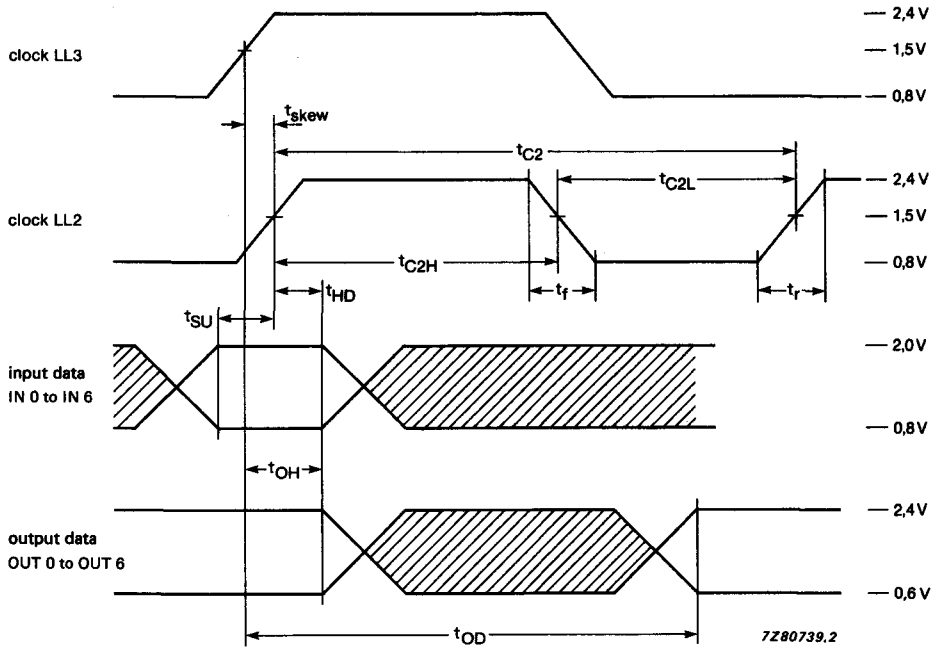
Fig. 5 Timing diagram.
