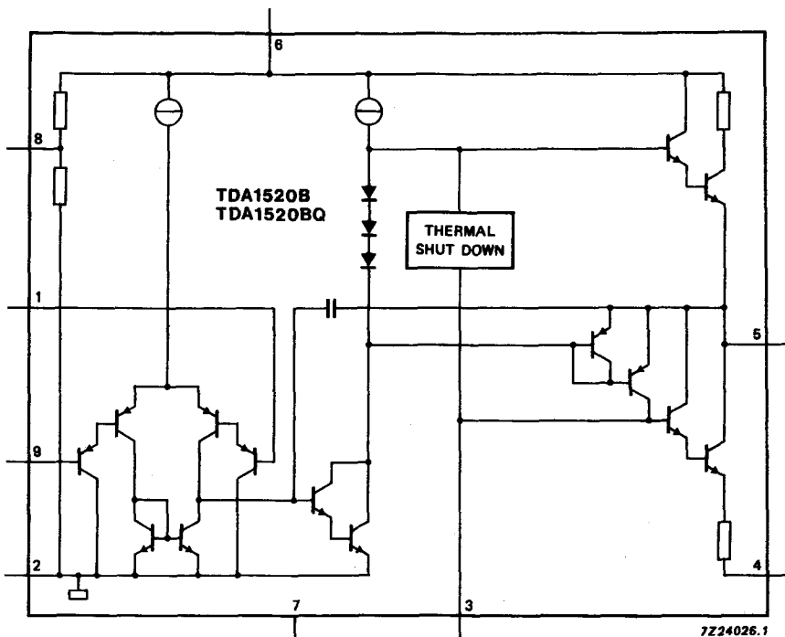
Fig. 1 Block diagram.
