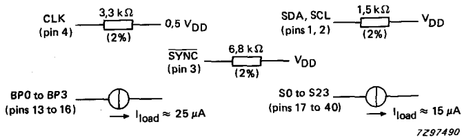
Fig. 19 Test loads.
