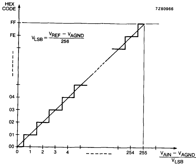
Fig. 9a A/D conversion characteristics of single-ended inputs.
