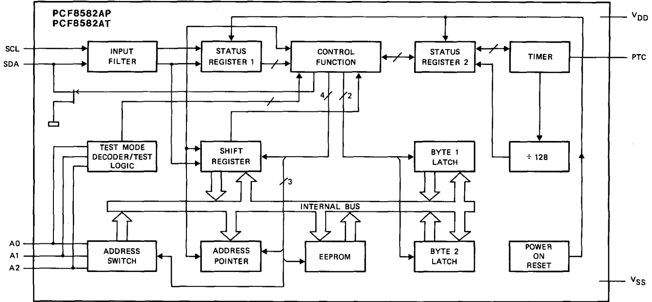
Fig. 1 Block diagram.
