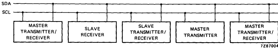
Fig.14 System configuration.
