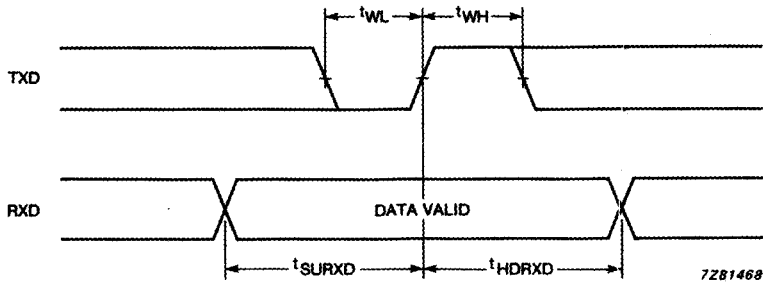
7281468 Fig. 5 RXD input waveform.
