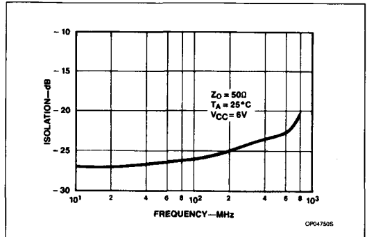
Figure 12. Isolation vs Frequency ( S_{12} )
