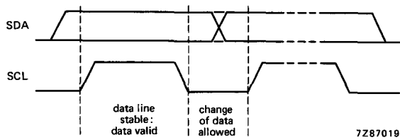
Fig.12 Bit transfer.
