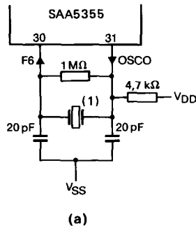
Fig. 4(a) Oscillator circuit for SAA5355 stand-alone sync mode and (b) equivalent circuit of crystal at resonance (see characteristics for values).
