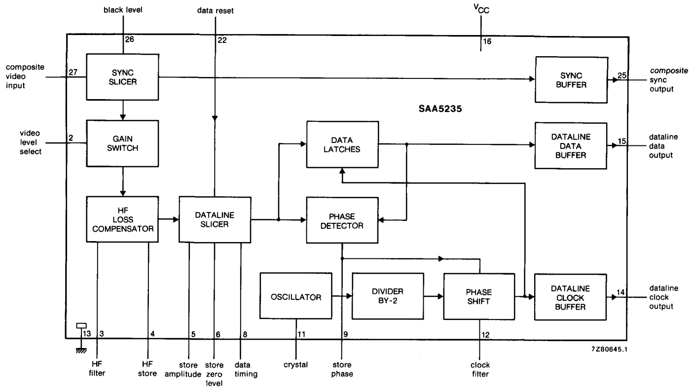
Fig. 1 Block diagram.
