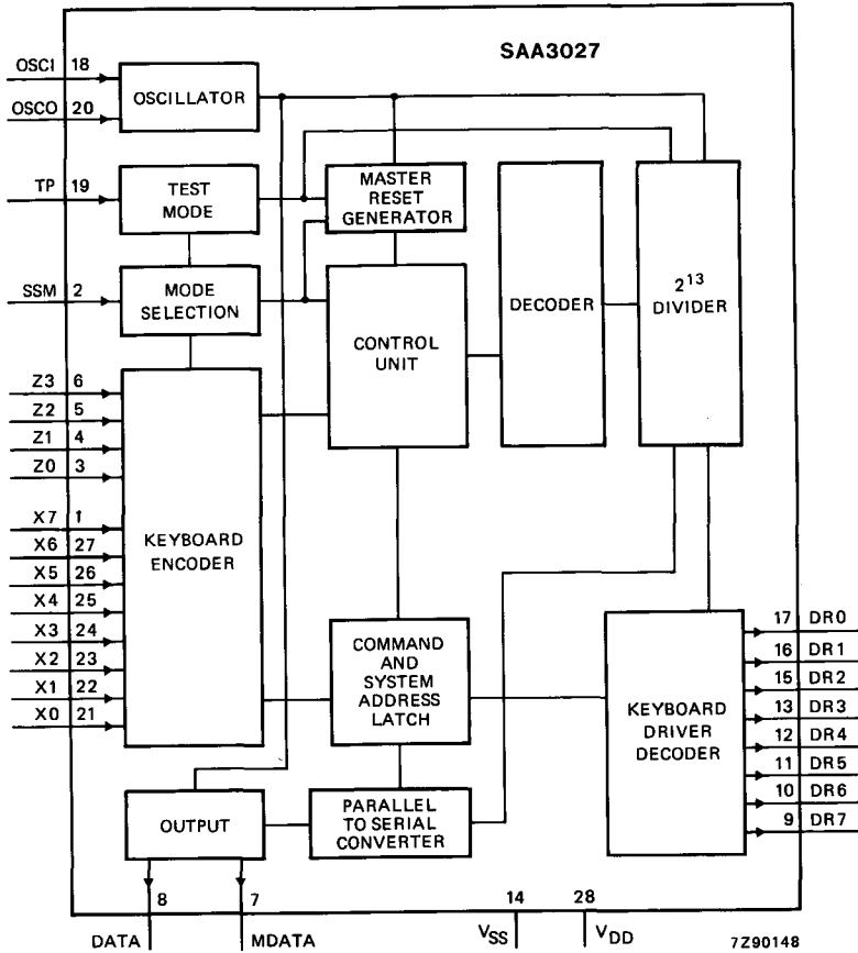
Fig. 1 Block diagram.
