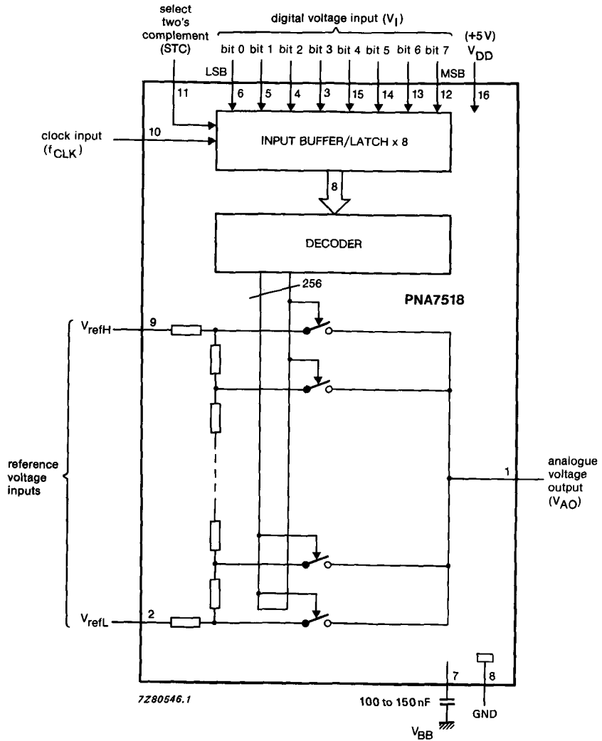
Fig. 1 Block diagram.
