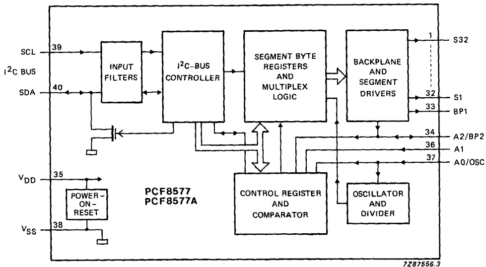
Fig.1 Block diagram.
