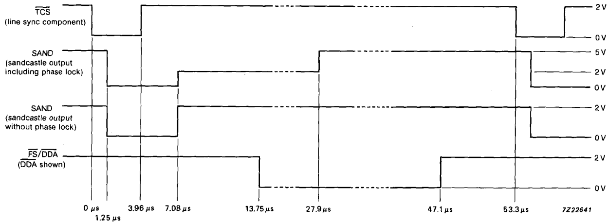
Fig. 12 Timing of synchronization and blanking outputs; all timings are nominal and assume f_{F6} = 7.2 \text{ MHz} .
