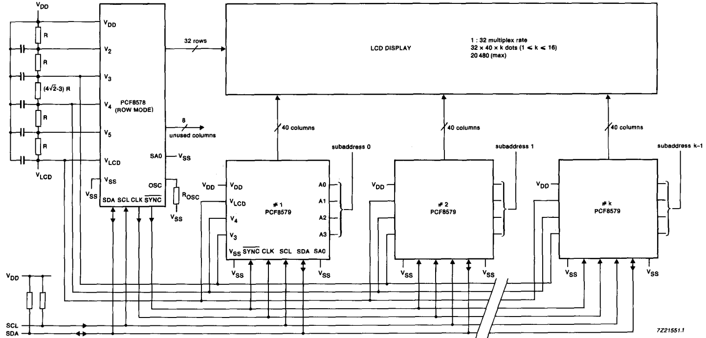
Fig.19 Typical LCD driver system with 1:32 multiplex rate.
