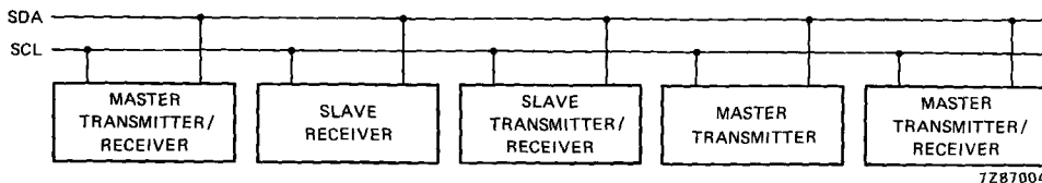
Fig.10 System configuration.
