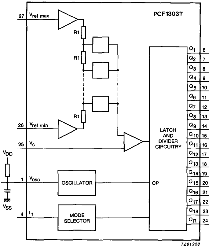
Fig. 1 Block diagram.
