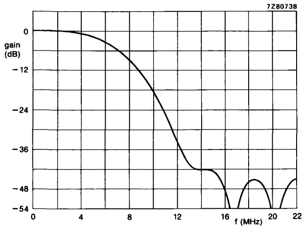
Fig. 4 Frequency response.
