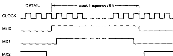
Fig. 4 Timing diagram.
