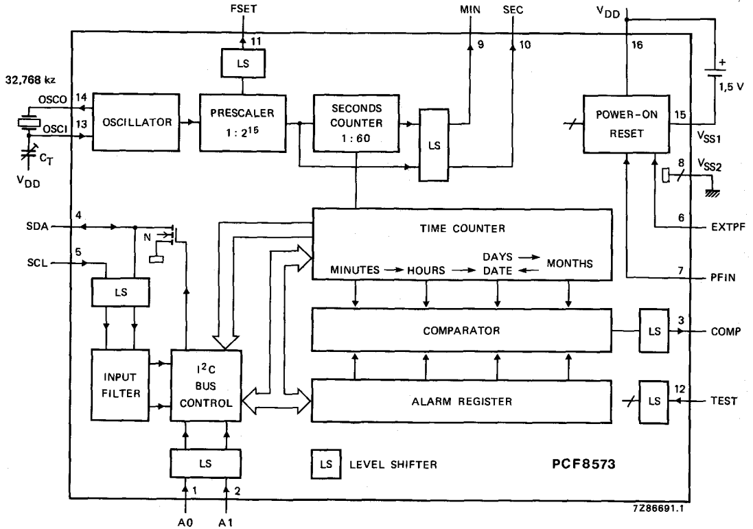
Fig.1 Block diagram.
