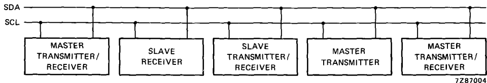
Fig. 13 System configuration.
