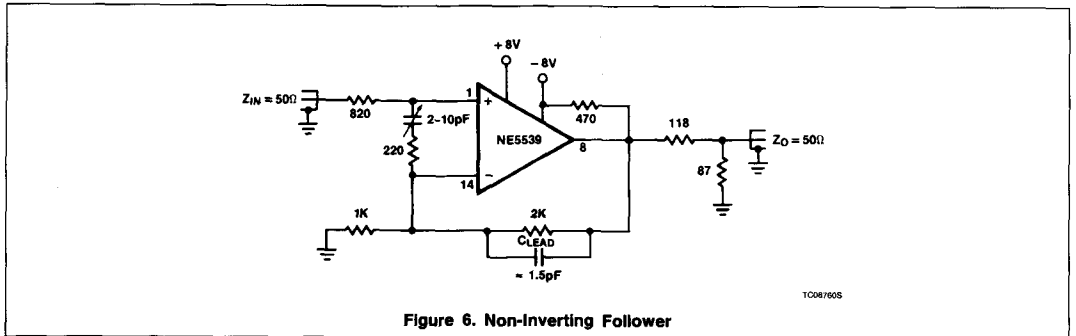
Figure 6. Non-Inverting Follower
