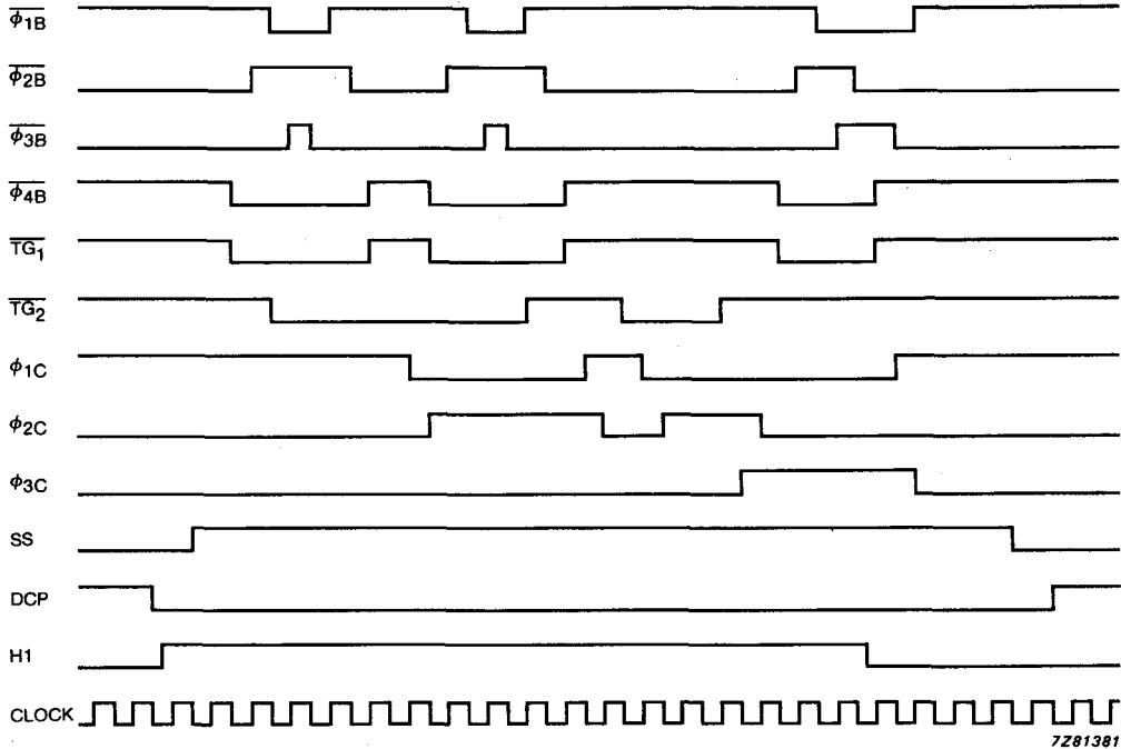
Fig.3 Line transport (625 lines).
