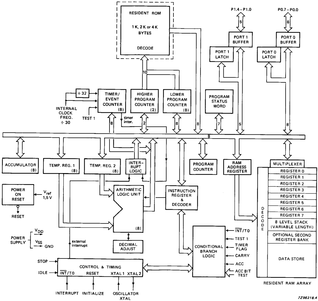
Fig. 1 Block diagram.
