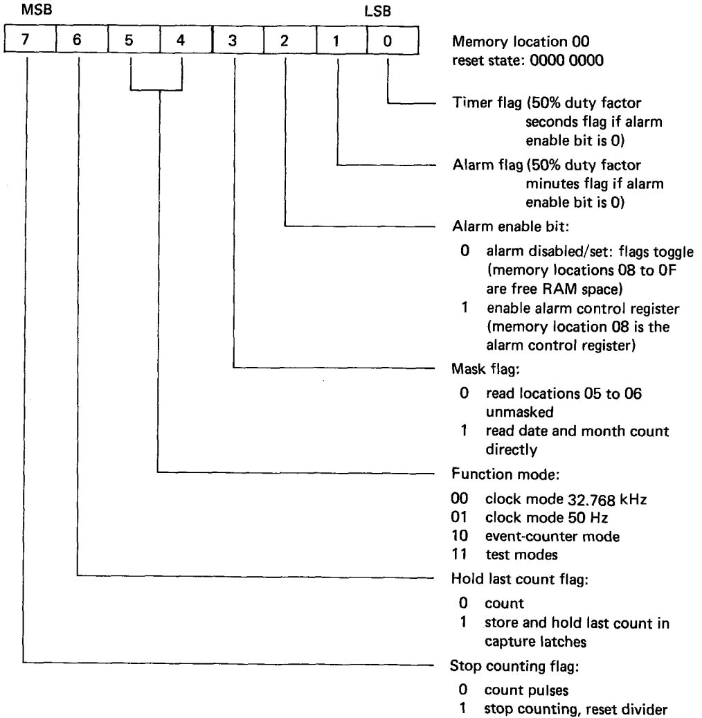
Fig.3 Control/status register.
