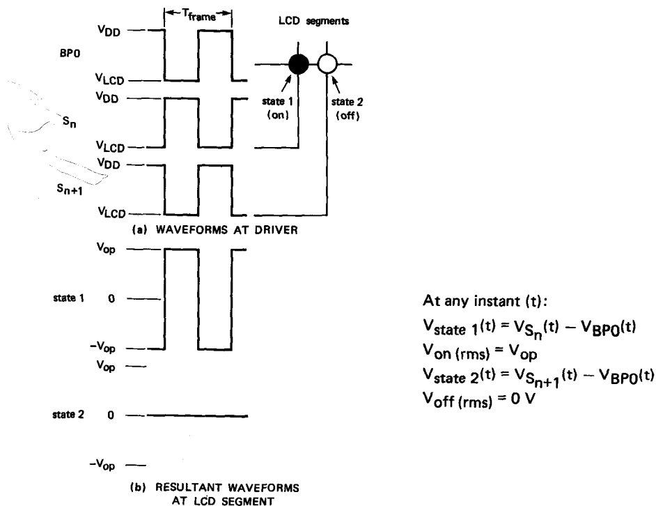
Fig.4 Static drive mode waveforms: V_{op} = V_{DD} - V_{LCD} .
