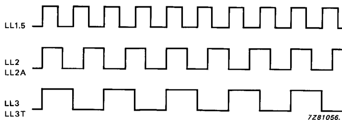
Fig. 3 Relationship between clock outputs.
