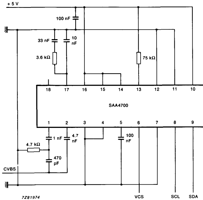
Fig. 9 Application circuit.
