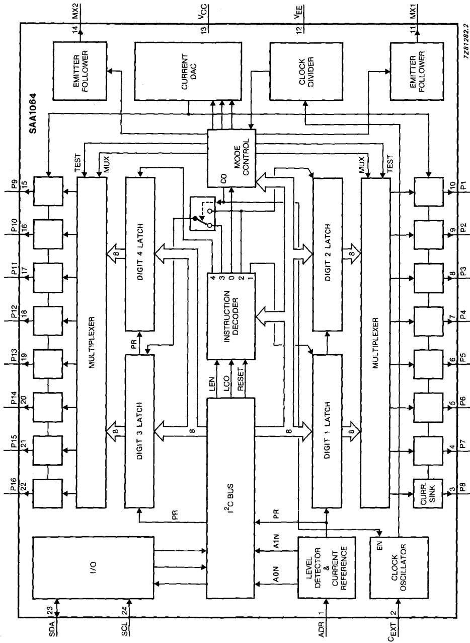
Fig. 1 Block diagram.
