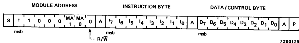
Fig. 3 I 2 C bus write format.
