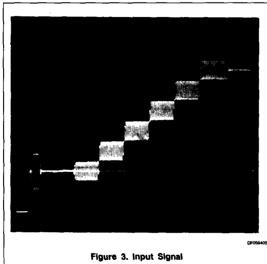
Figure 3. Input Signal
