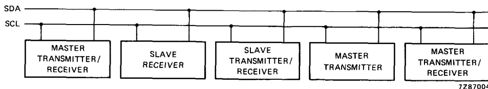
Fig. 13 System configuration.
