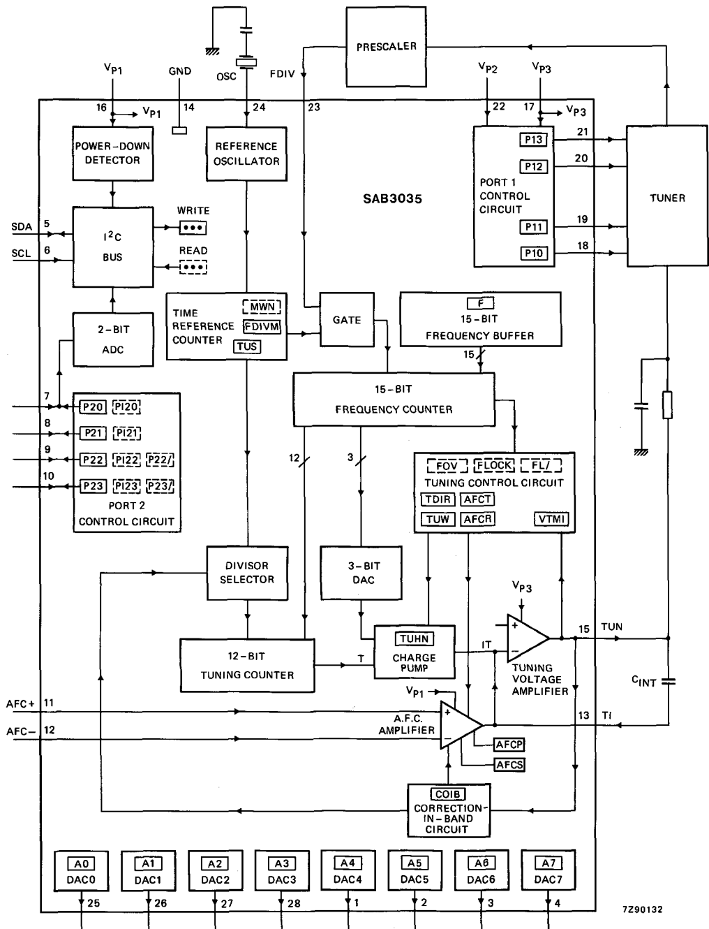
Fig. 1 Block diagram.
