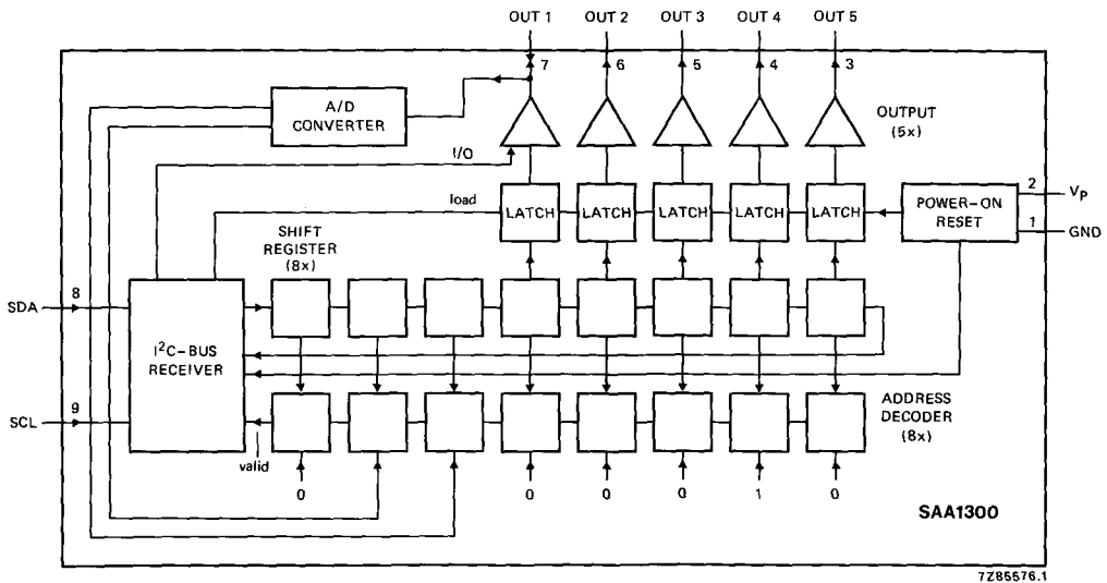
Fig. 1 Block diagram.
