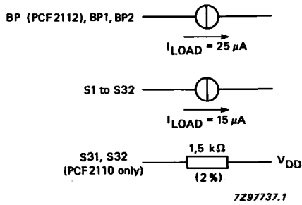
Fig. 16 Test loads.
