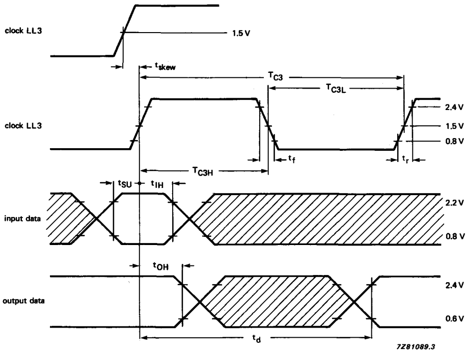
Fig.11 Timing diagram.
