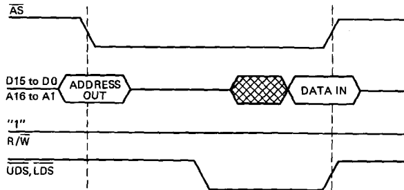
Fig. 18 Bus timing for display memory access.
