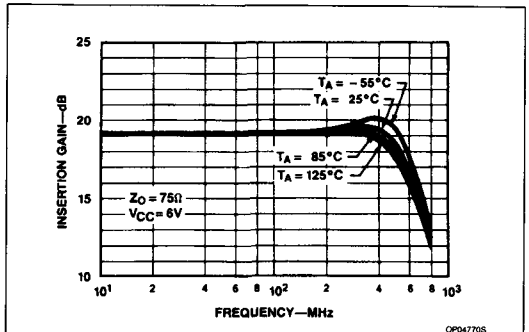
Figure 14. Insertion Gain vs Frequency ( S_{21} )
