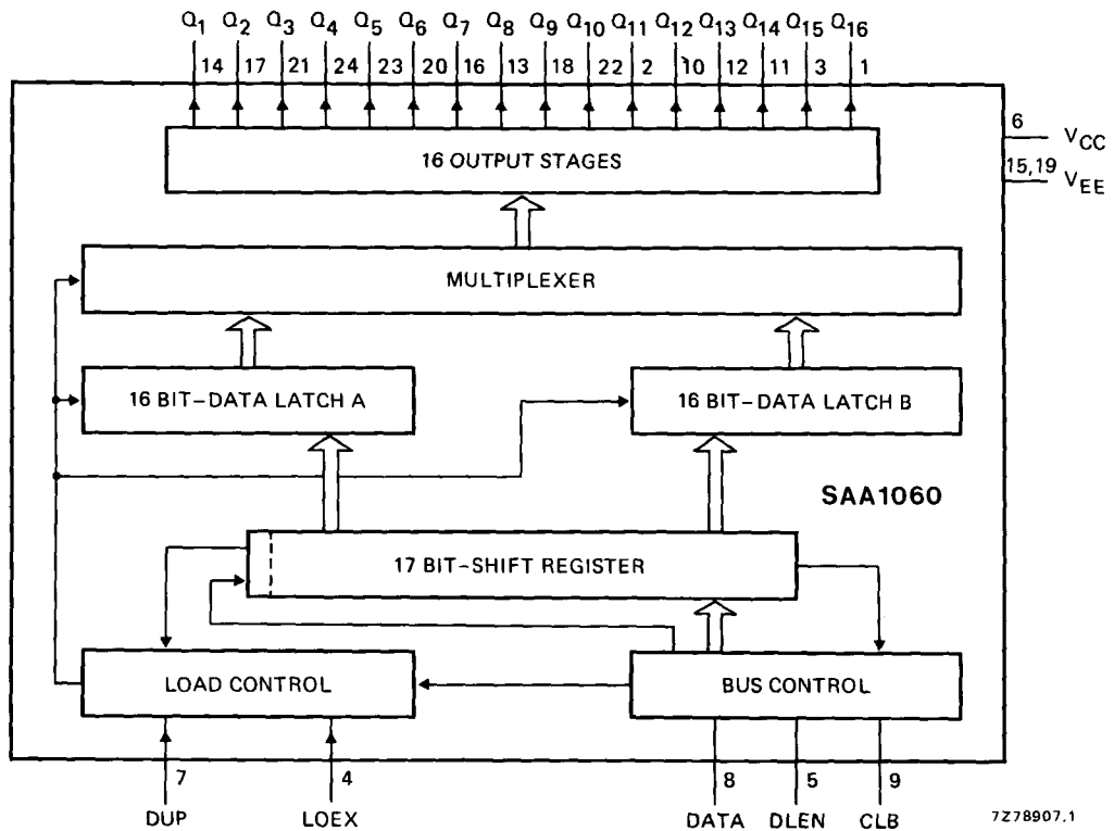
Fig. 1 Block diagram.
