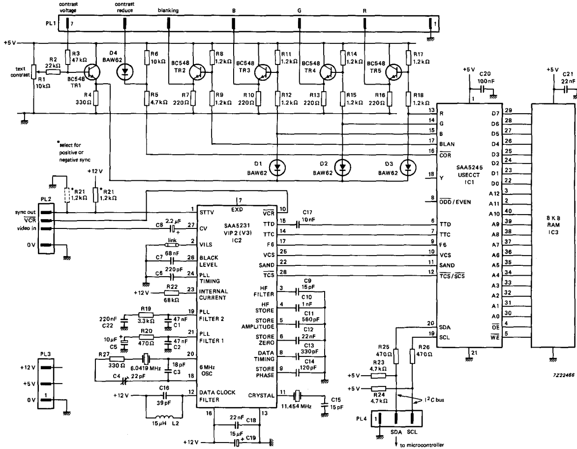
Fig. 11 USECCT based multi-page decoder circuit diagram.
