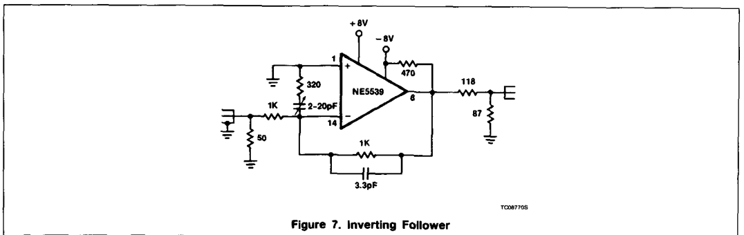
Figure 7. Inverting Follower
