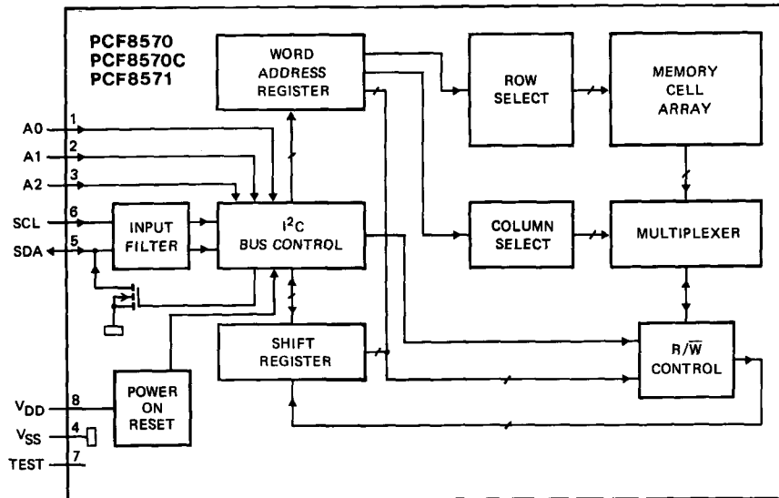
Fig.1 Block diagram.
