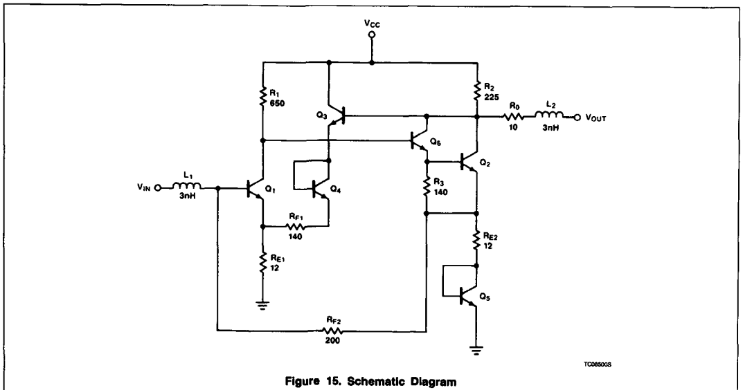
Figure 15. Schematic Diagram
