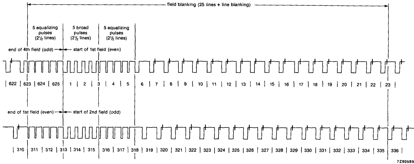
Fig. 13 Vertical synchronization and blanking waveforms; separation of broad pulses = 3.96 \mu s; equalizing pulse widths = 7.88 \mu s.
