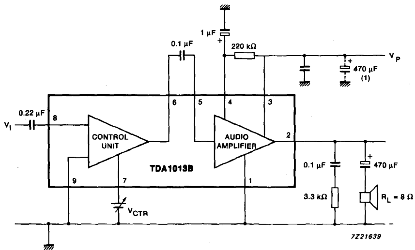
Fig.10 Application diagram.
