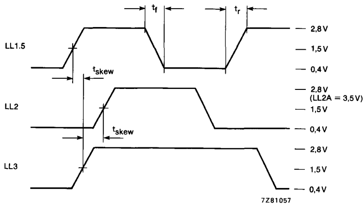
Fig. 4 Timing diagram.
