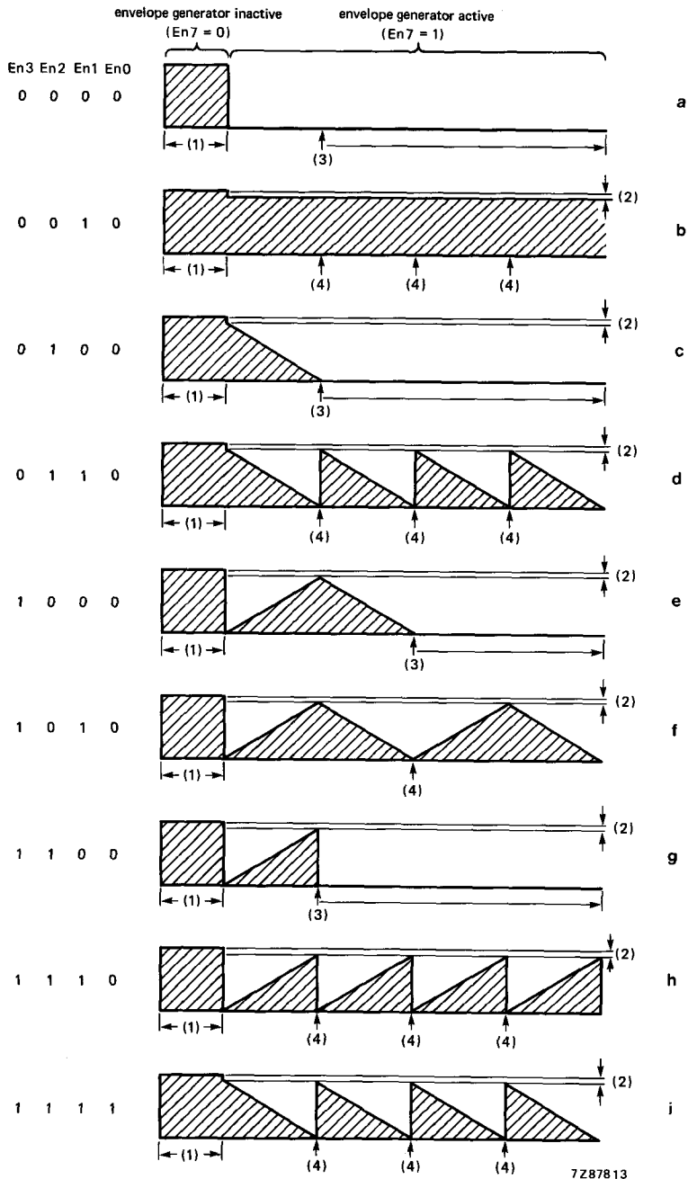
Fig. 5 Envelope waveforms.
