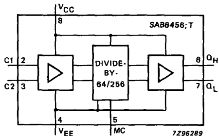
Fig. 1 Block diagram.
