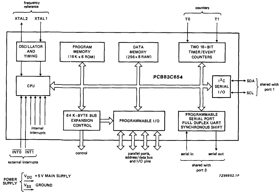
Fig. 1 Block diagram.
