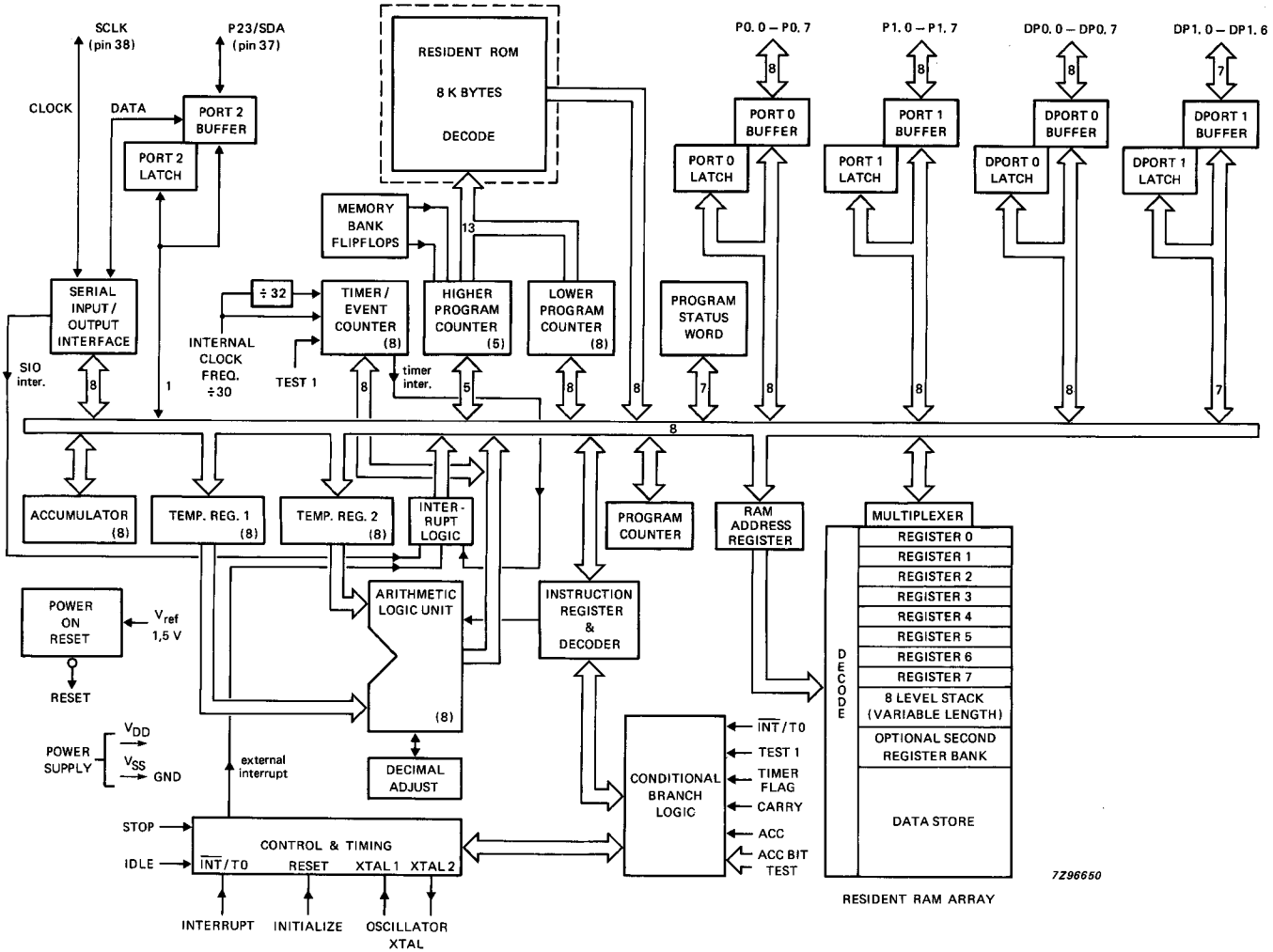
Fig. 1 Block diagram.
