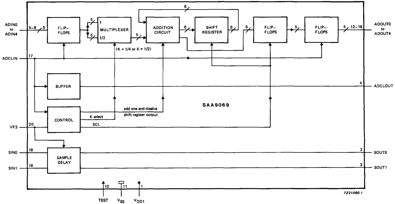
Fig. 1. Block diagram.
