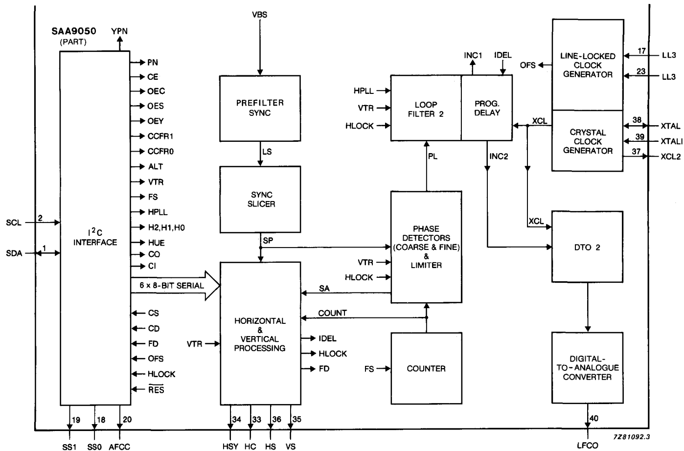
Fig.1b Block diagram; continued from Fig.1a.
