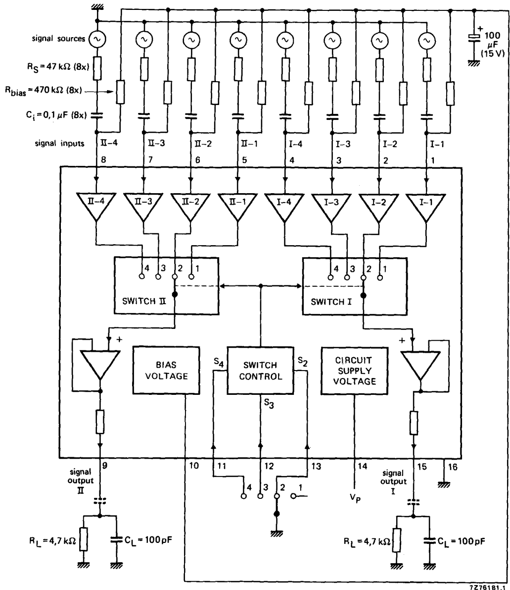
Fig. 1 Block diagram.
