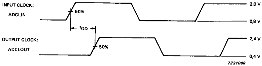
Fig. 3 Input and output clock signal phase relationship.
