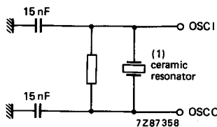
Fig. 8 Oscillator circuit.
