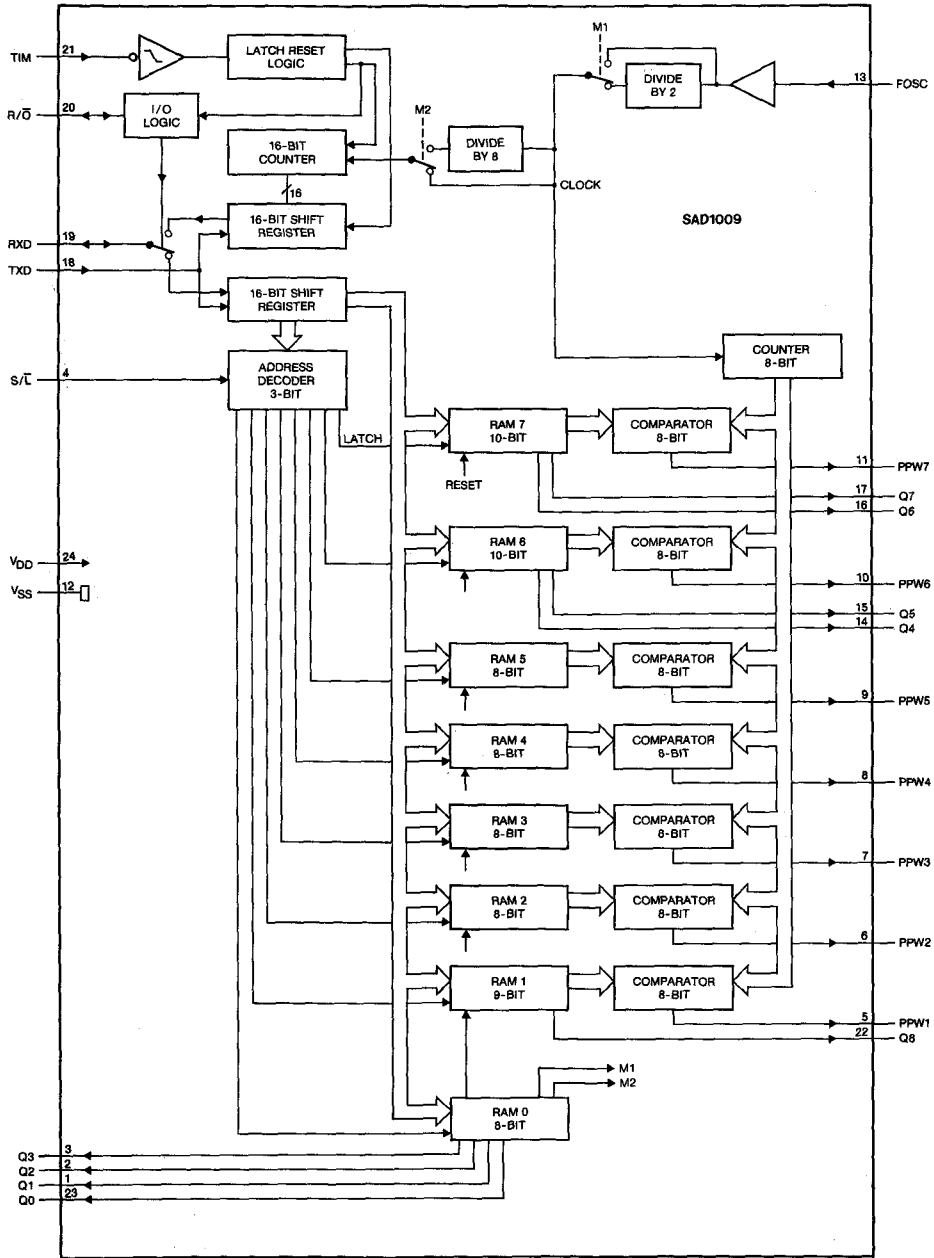
Fig. 1 Block diagram.
