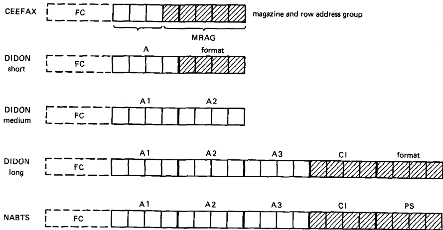
Fig. 3 Five prefixes.
