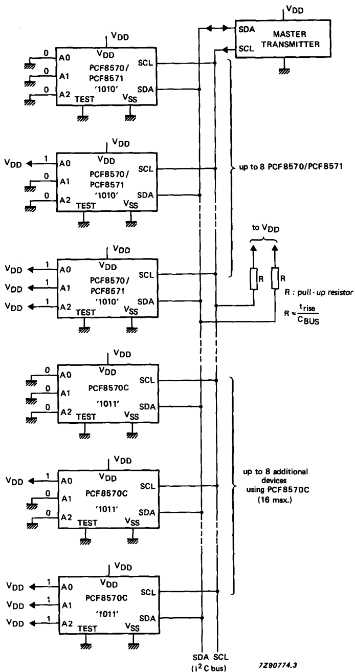
Fig.11 Application diagram.
