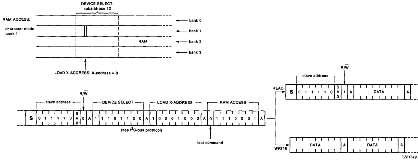
Fig.10 Example of commands specifying initial data byte RAM locations.
