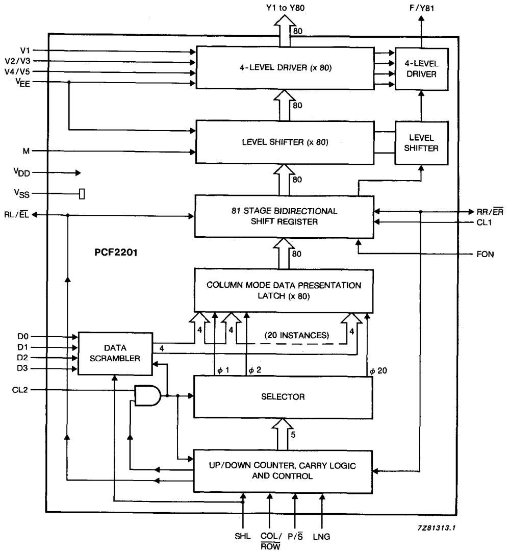
Fig. 1 Block diagram.
