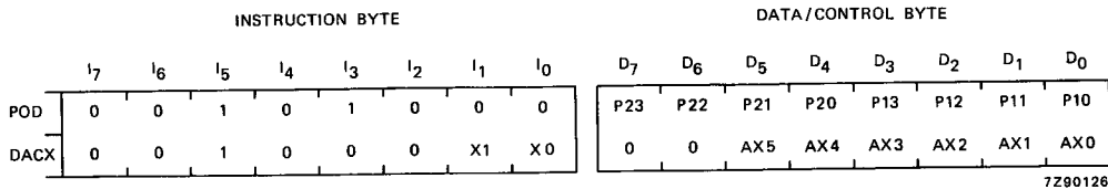
Fig. 5 Control programming.
