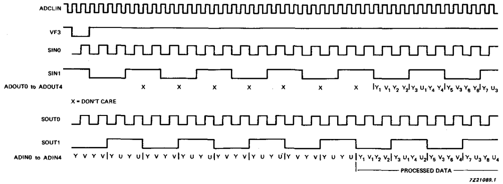
Fig. 5 Timing diagram.
