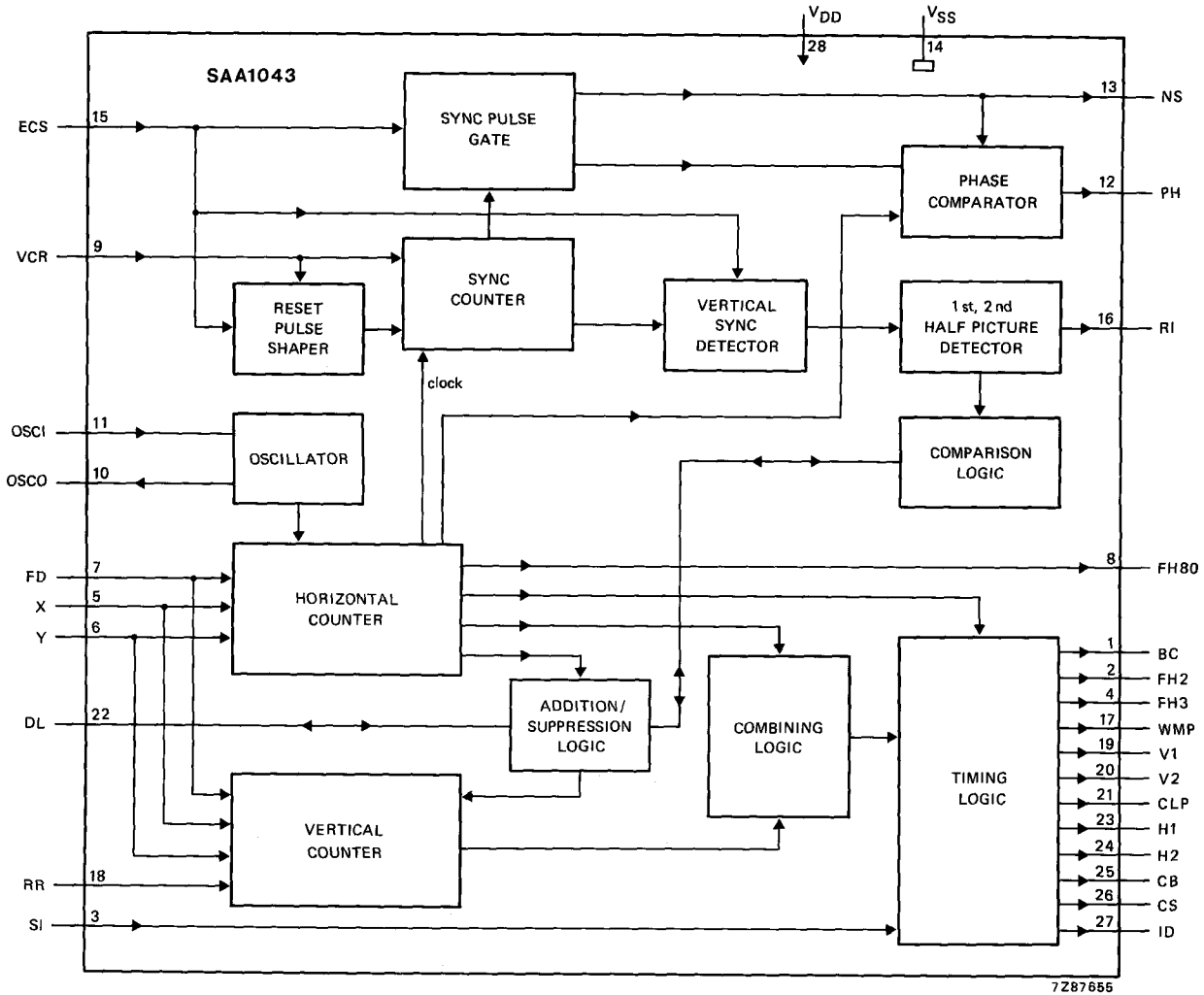
Fig. 1 Block diagram.
