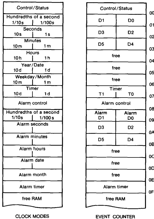
Fig.4 Register arrangement.
