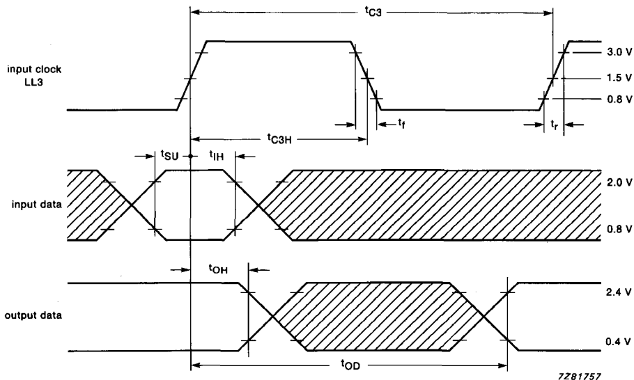
Fig. 9 Timing diagram.
