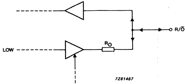
7281467 Fig. 4 Equivalent R/O output port.
