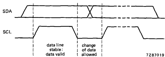
Fig.14 Bit transfer.
