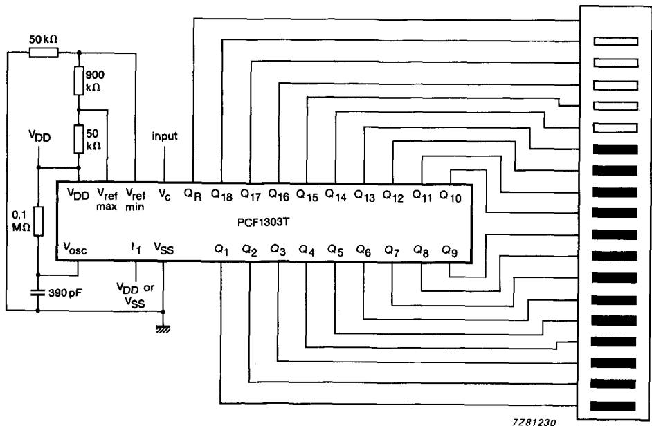
Fig. 3 Typical application.
