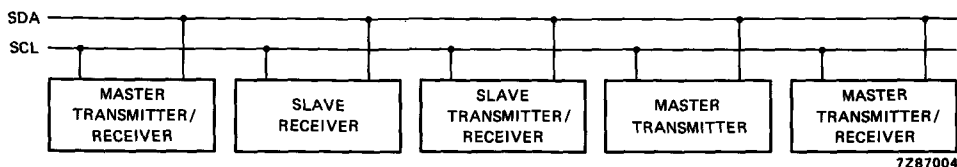
Fig.12 System configuration.
