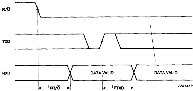
7281469 Fig. 6 RXD output waveform.
