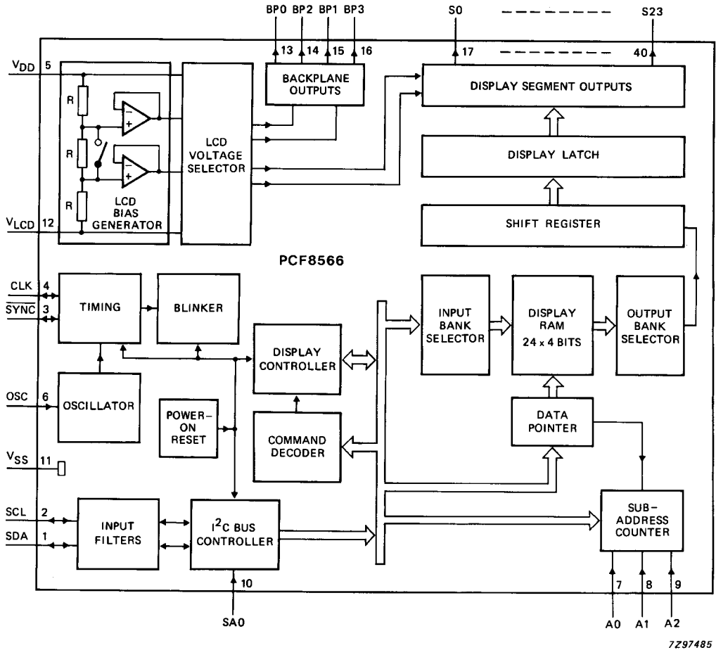
Fig. 1 Block diagram.
