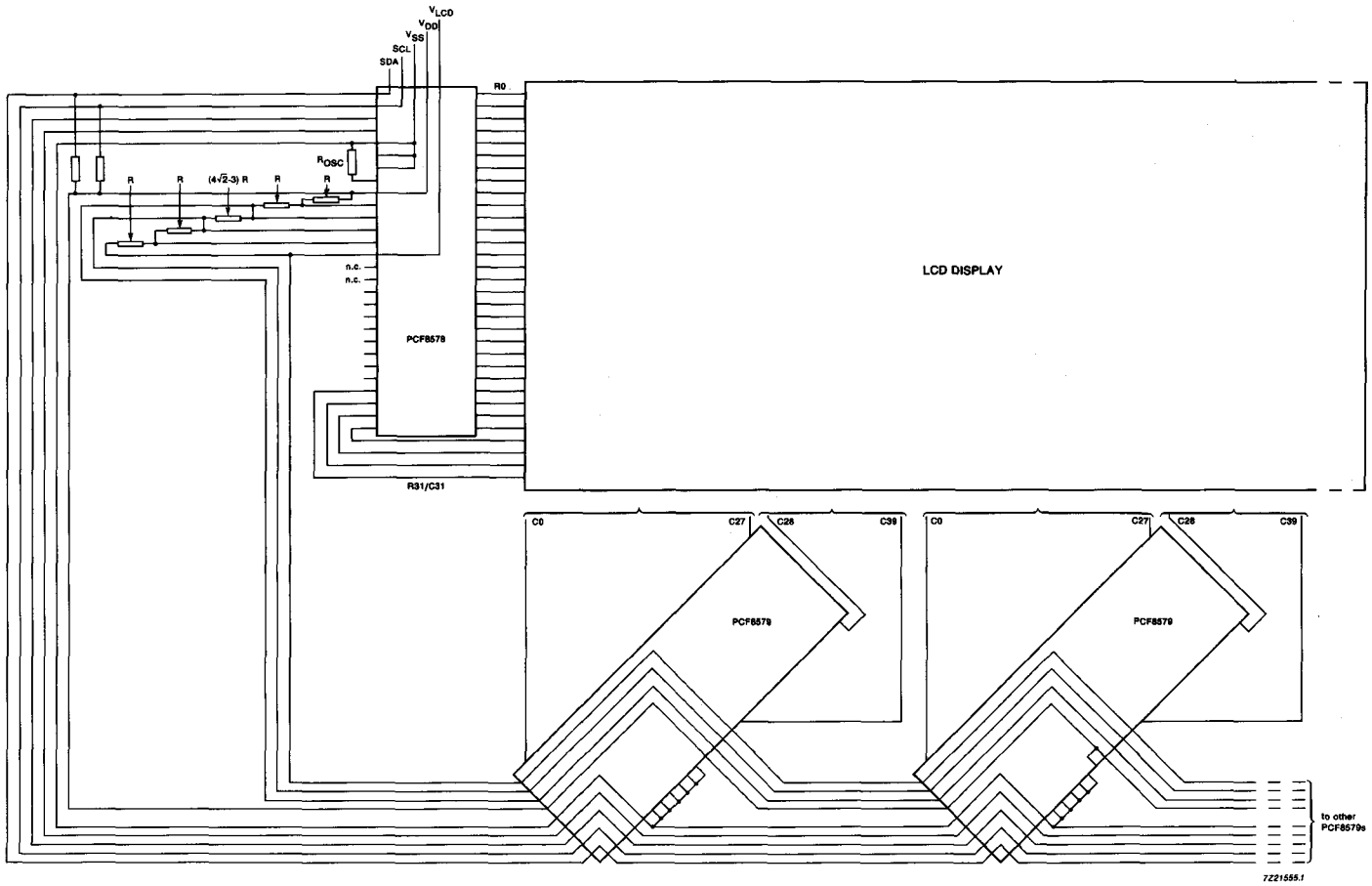
Fig.22 Example of single plane wiring, single screen with 1:32 multiplex rate (PCF8578 in row driver mode).
