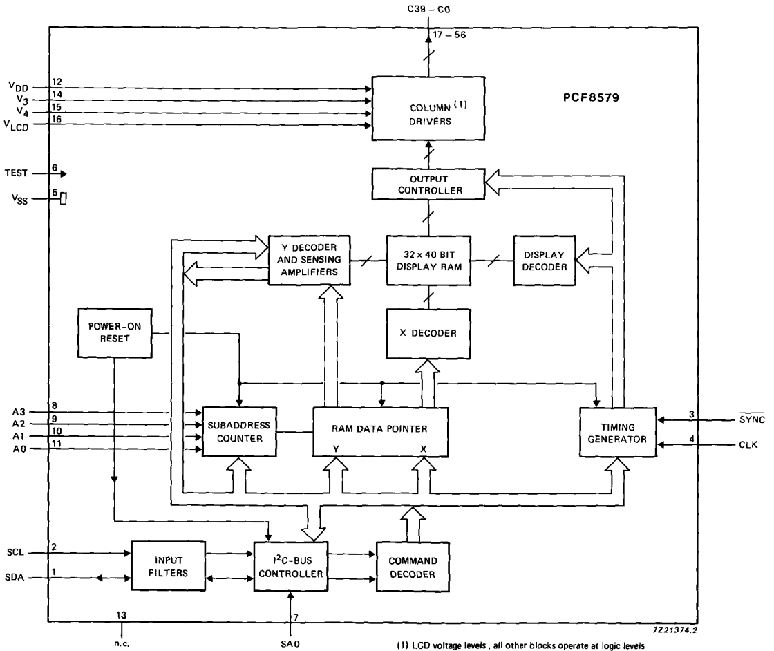
Fig.1 Block diagram.
