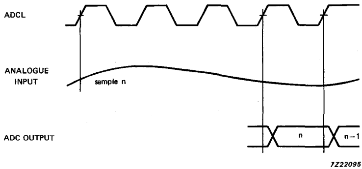
Fig. 6 ADC required.
