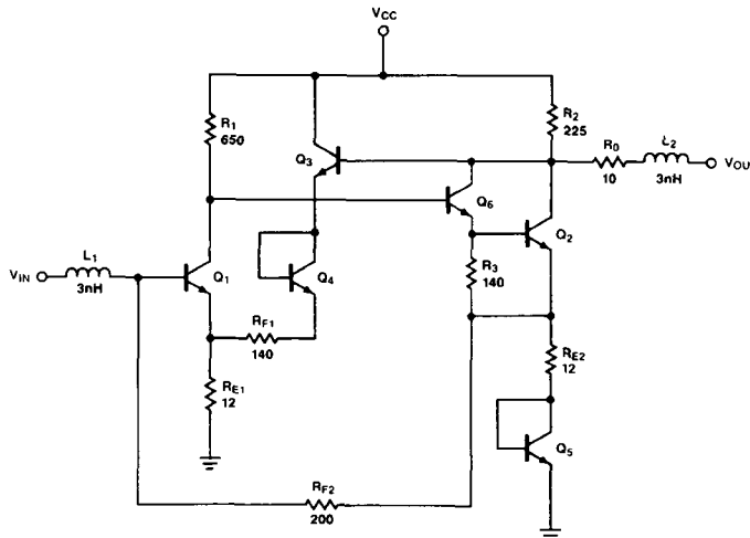
Figure 15. Schematic Diagram
