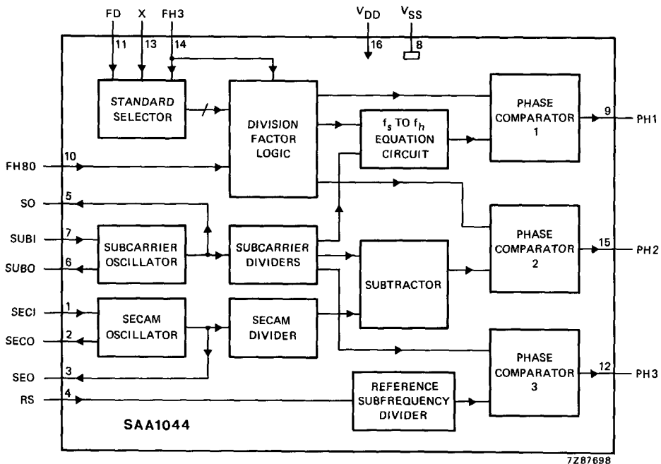
Fig.1 Block diagram.
