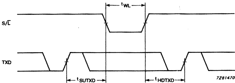
7281470 Fig. 7 S/L input waveform.
