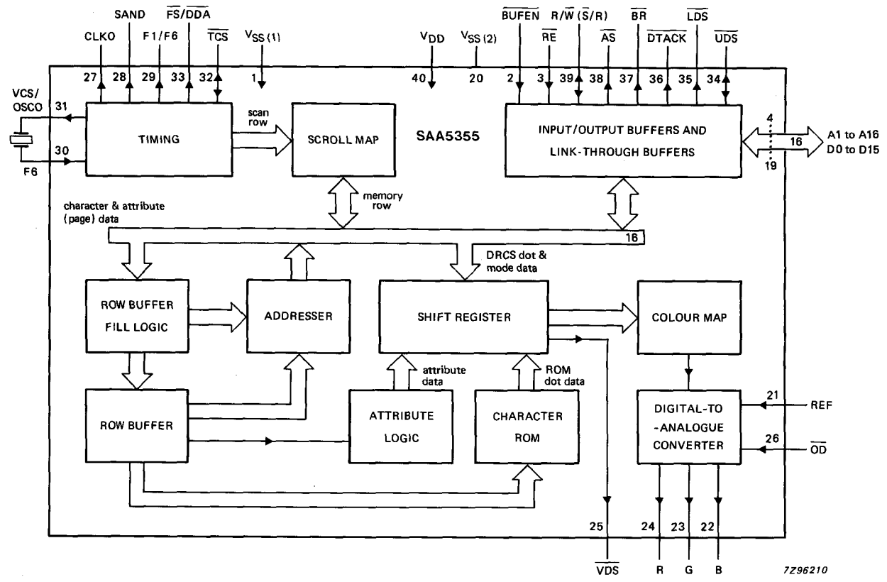
Fig. 1 Block diagram.
