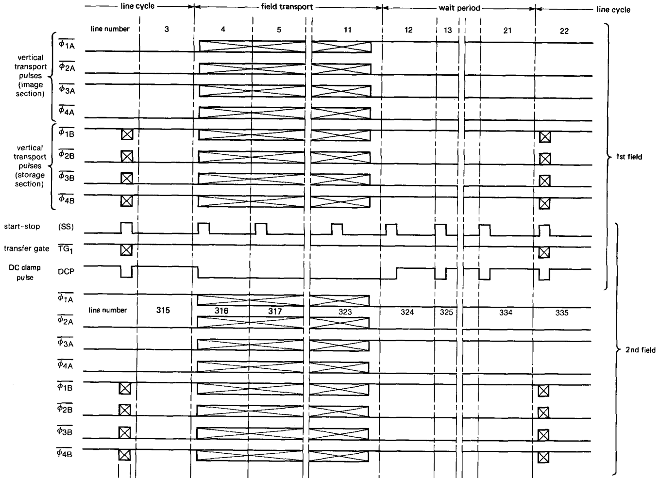
Fig.7 MNPPG cycles during field blanking (625 lines).
