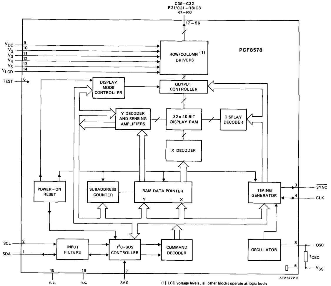
Fig.1 Block diagram.
