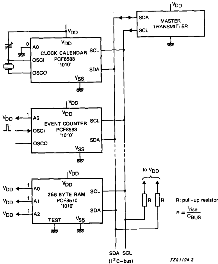
Fig.16 PCF8583 address.
