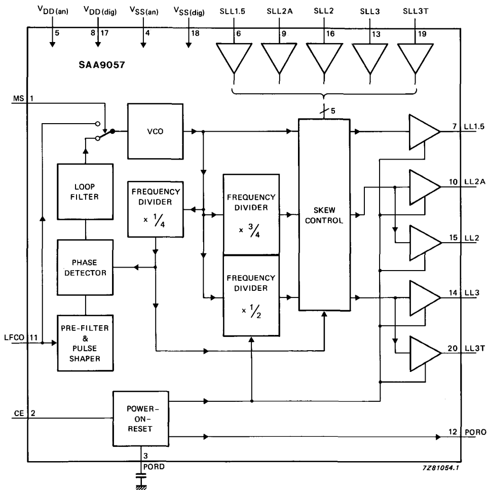
Fig. 1 Block diagram.
