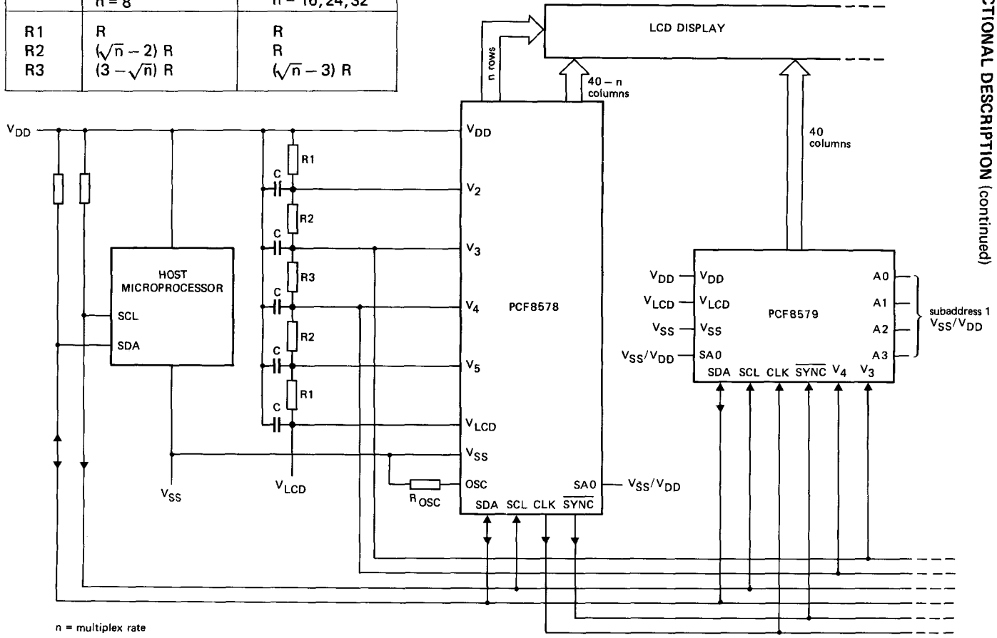
Fig.3 Typical mixed mode configuration.
