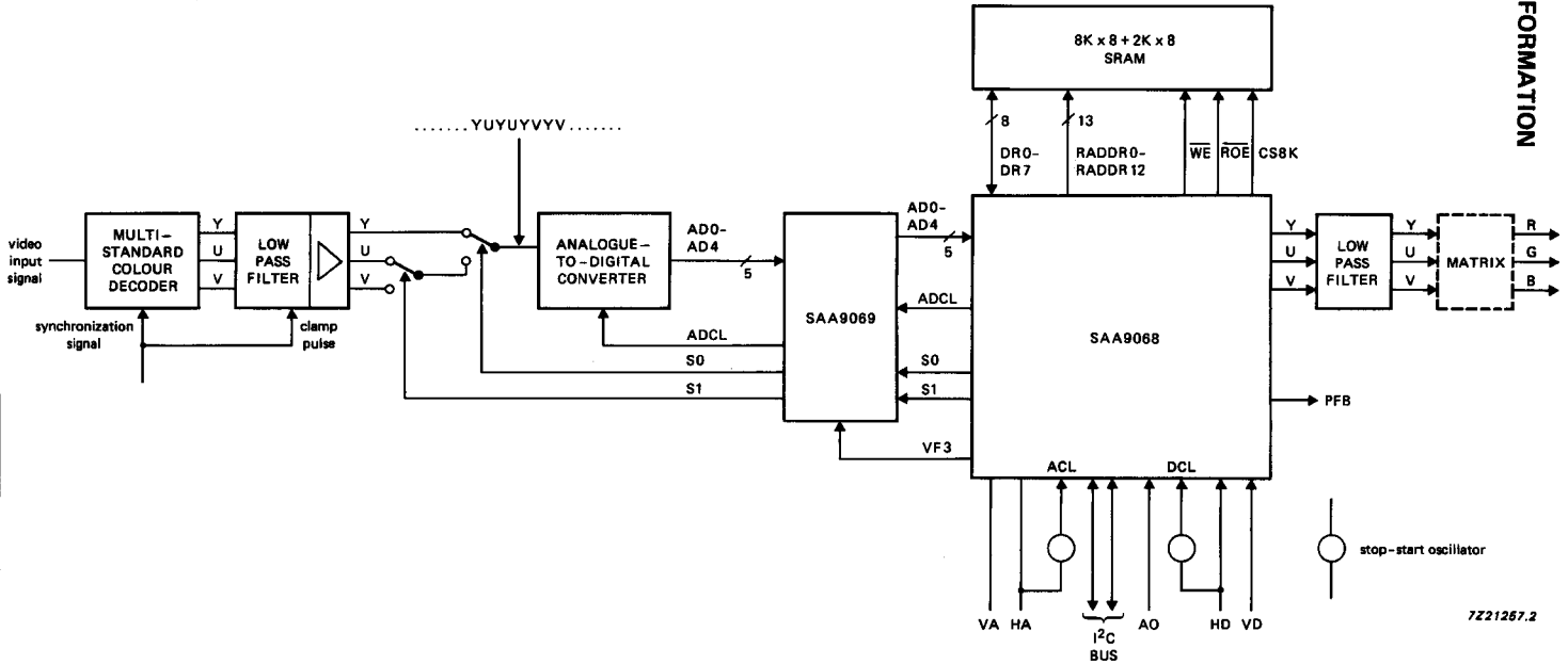
Fig. 9 Application diagram, using SAA9069.
