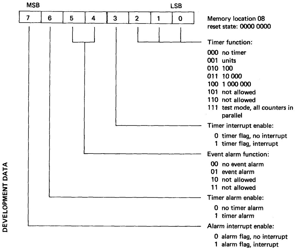
Fig.8b Alarm control register, event-counter mode.
