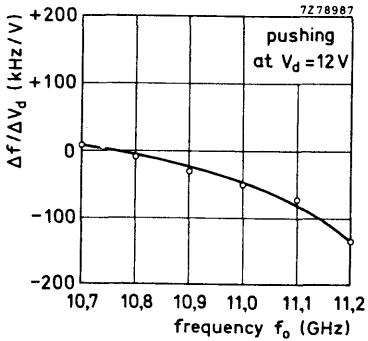
Fig. 8 Pushing of the Gunn oscillator, measured as a function of frequency and diode voltage.
