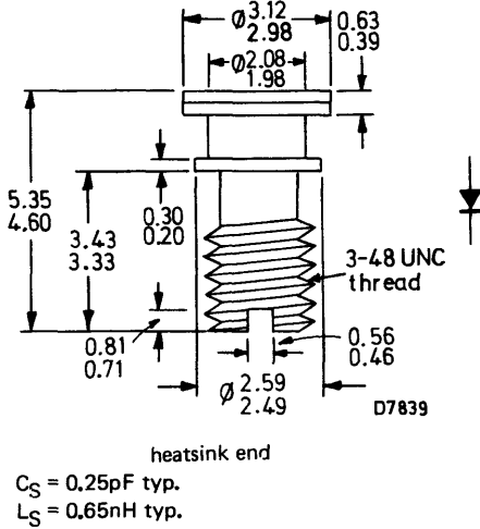
case style SOD-44
