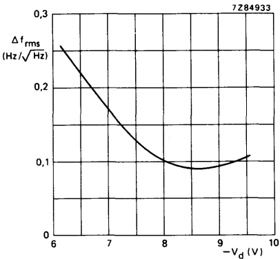
Fig. 8 Single-sideband f.m. noise at f_0 \approx 10,5 GHz, as a function of the diode voltage V_d , measured in a bandwidth of 1 Hz at 100 kHz distance from the carrier.
