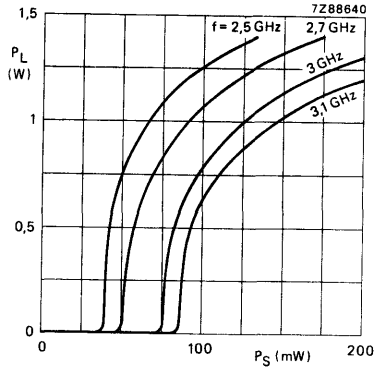
Fig. 7 Load power at V_{CE} = 28\text{ V} as a function of source power with frequency as parameter.
