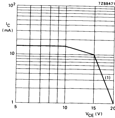
Fig. 2 D.C. SOAR at T_{case} \leq 150^\circ C ; R_{BE} \leq 150 \Omega .
