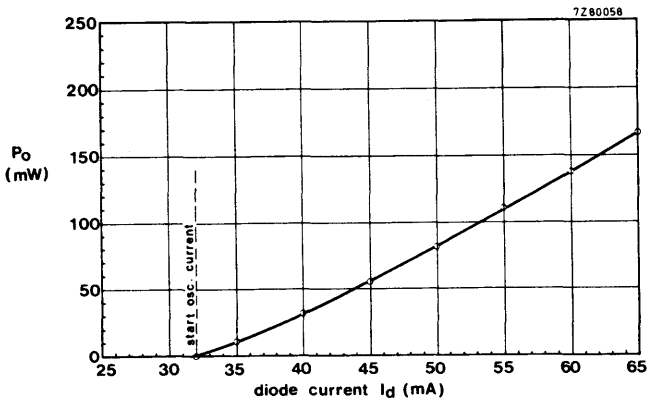
Fig. 6 Output power of the IMPATT oscillator, measured as a function of the diode current I_d at f_o = 11 GHz.
