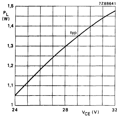
Fig. 8 Load power at f = 3\text{ GHz} and P_S = 0,2\text{ W} as a function of collector-emitter voltage.
