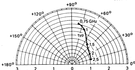
Fig. 8 Forward transmission coefficient s_{fe} .
