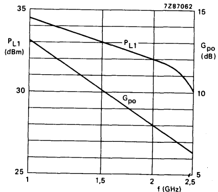
Fig. 7 Load power and power gain, associated with 1 dB compressed power gain, as a function of frequency.
