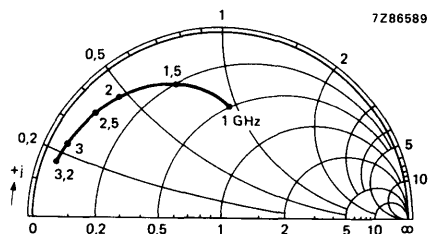
Fig. 9 Optimum load impedance as a function of frequency for P_{L1} .
