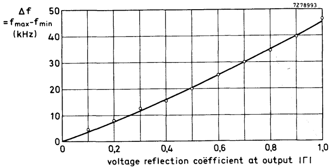
Fig. 9 Frequency pulling of the Gunn oscillator as a function of the modulus of the voltage reflection coefficient. (Output via isolator and OSM connector.) V_d = 12 V; f_o = 11 GHz; P_o = 88 mW; I_d = 495 mA.
