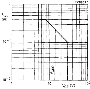
Fig. 2 D.C. SOAR at T_{mb} \leq 75 \text{ }^\circ\text{C} . I Region of permissible d.c. operation. II Permissible extension provided R_{BE} \leq 500 \text{ } \Omega .
