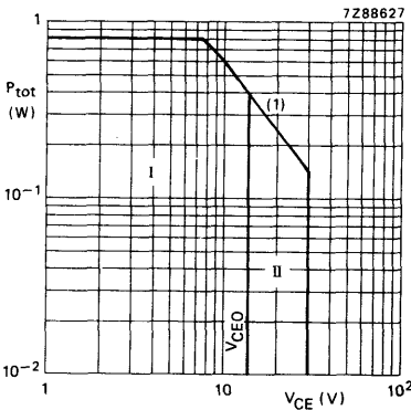
(1) Second breakdown limit (independent of temperature). Fig. 4 D.C. SOAR at T_{mb} \leq 75 \text{ }^\circ\text{C} . I Region of permissible d.c. operation. II Permissible extension provided R_{BE} \leq 250 \text{ } \Omega .
