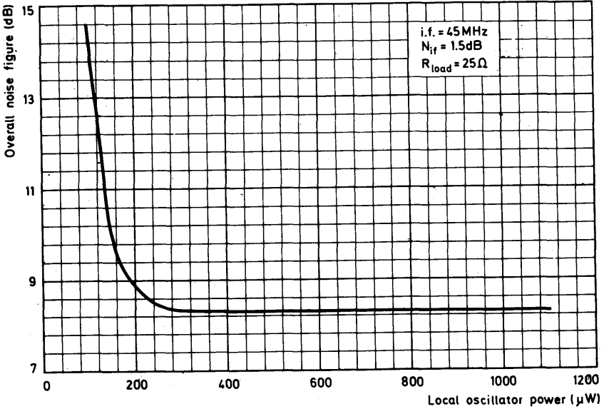
Fig.3 Typical overall noise figure as a function of local oscillator power at 34.86 GHz
