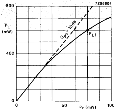
Fig. 4 Load power as a function of source power. Typical values; V_{CE} = 15\text{ V} I_C = 140\text{ mA} } regulated; f = 2,1\text{ GHz} ; T_{mb} = 25\text{ }^\circ\text{C} .
