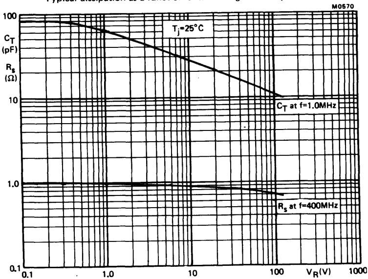
Typical diode capacitance and series resistance as a function of reverse voltage
