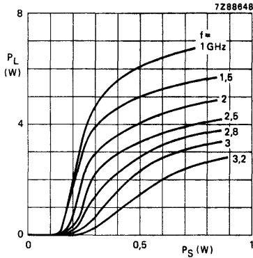
Fig. 11 Load power as a function of source power with frequency as parameter.
