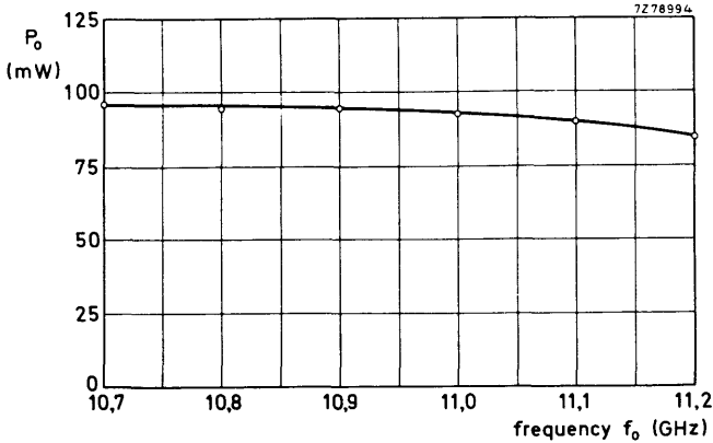
Fig. 5 Output power as a function of frequency for the Gunn oscillator with diode voltage V_D = 12 V.
