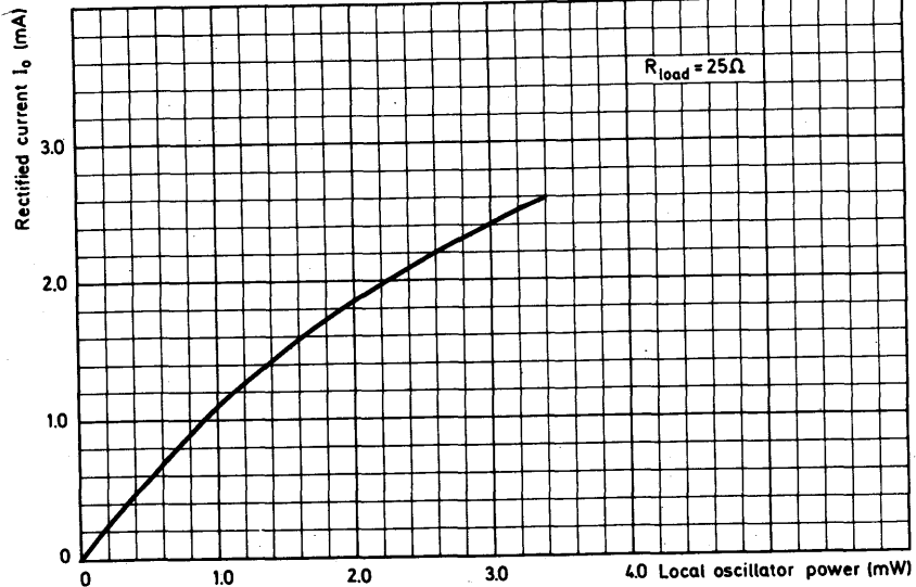
Fig.2 Typical rectified current as a function of local oscillator power at 34.86 GHz
