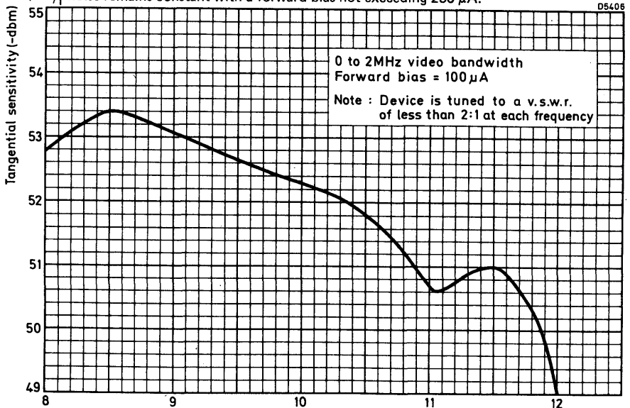
Tangential sensitivity as a function of frequency
