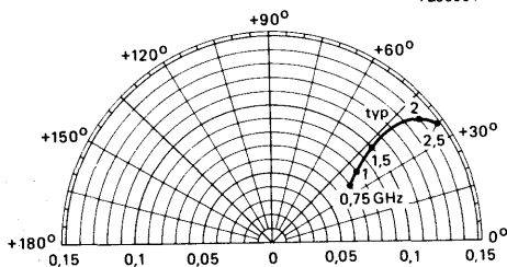
Fig. 7 Reverse transmission coefficient s_{re} .
