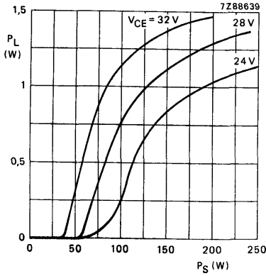
Fig. 6 Load power at f = 3\text{ GHz} as a function of source power with collector-emitter voltage as parameter.
