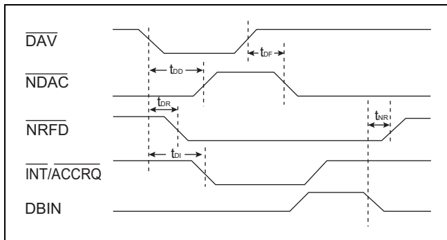
Figure 10. Acceptor Handshake Timing
