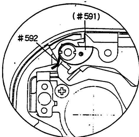
fig. 14-3 Spring #592
