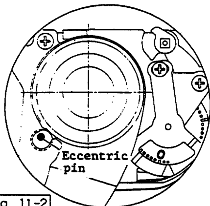
fig. 11-2 Eccentric pin #394
