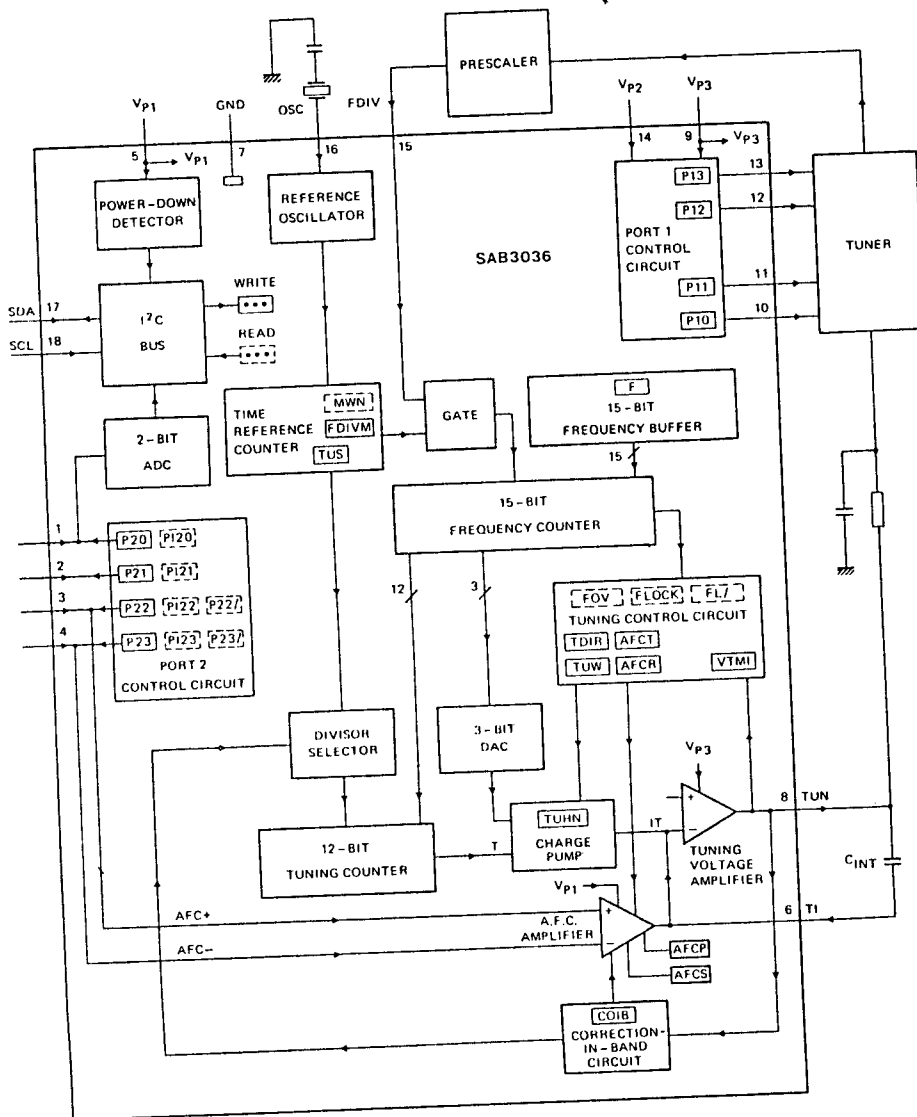
Fig. 1 Block diagram.
