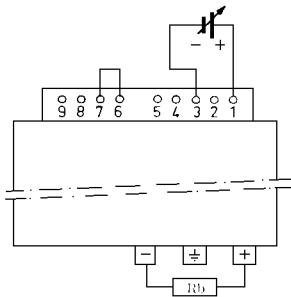
Fig. 7d. Voltage programming with external voltage
