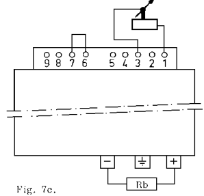
Fig. 7c. Voltage programming with external rheostat
