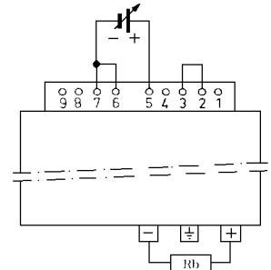
Fig. 7f. Current programming with external voltage
