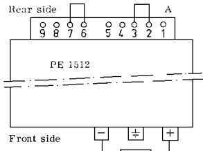
Fig. 7a. Normal use Rb = load Belastung belasting charge
