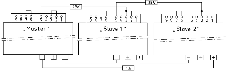
Fig. 7g. Series connection according to "Master and slave" system
