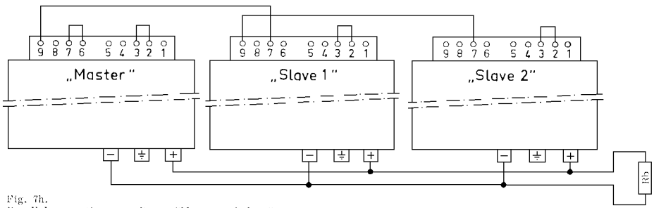
Fig. 7h. Parallel connection according to "Master and slave" system
