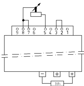
Fig. 7e. Current programming with external rheostat
