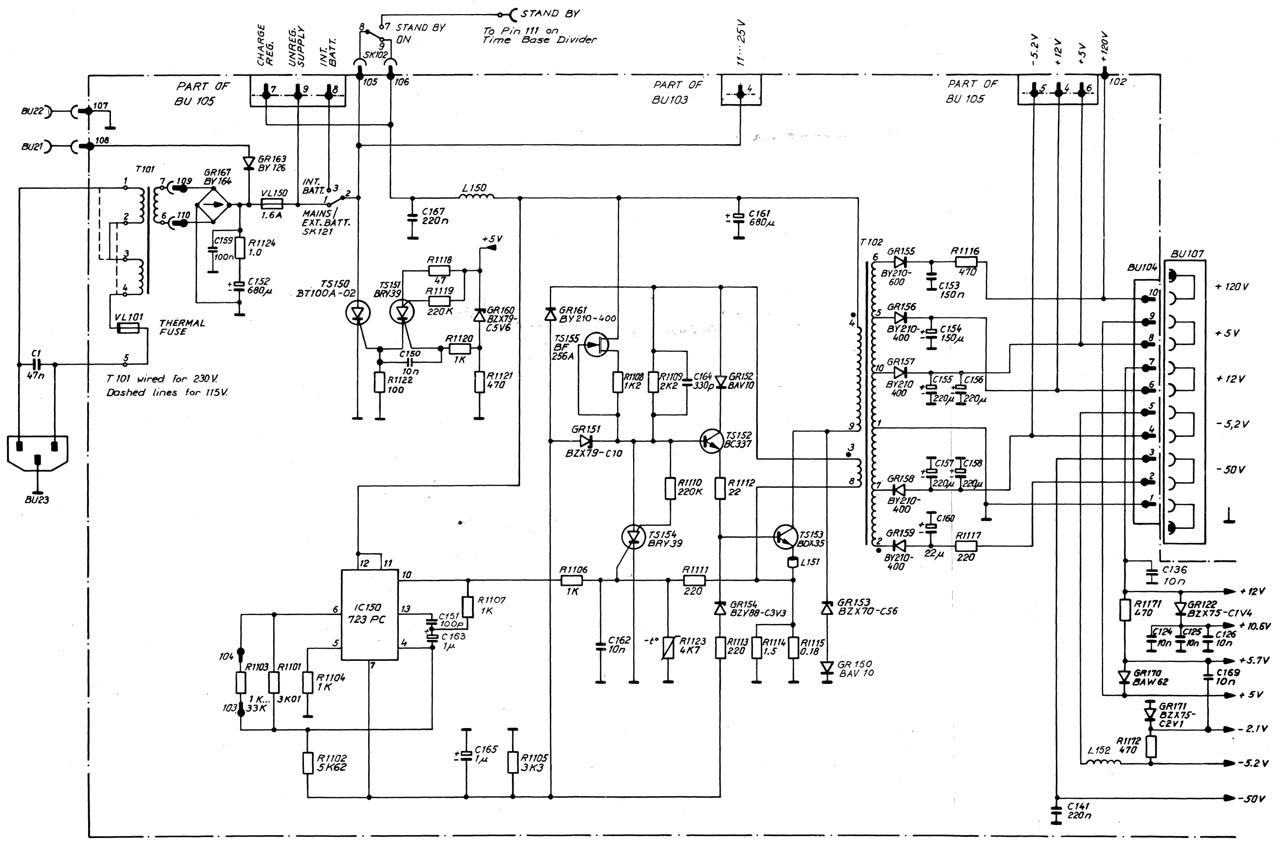
Figure X-5. Power supply
