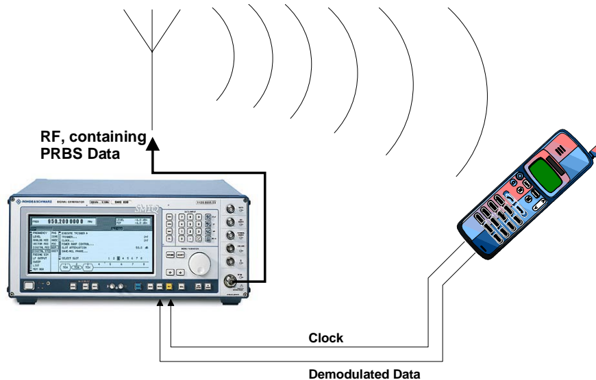
Fig. 2-234 BER Measurement
