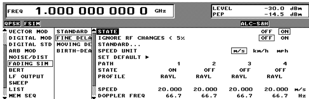
Fig. 2-41 Menu FINE DELAY
