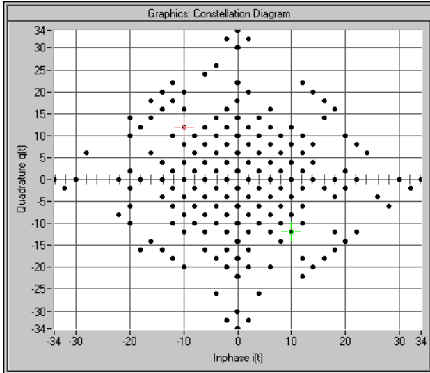
Fig. 2-153 Constellation with 16 uncorrelated channels (1 time slot)
