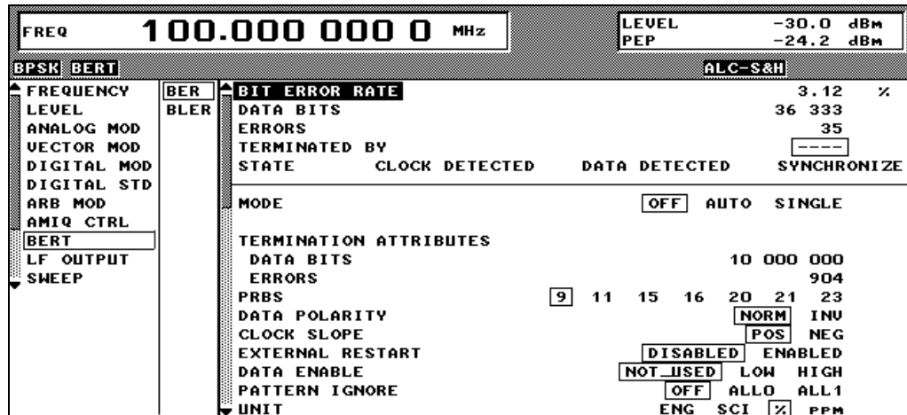
Fig. 2-235 Operating menu for BER measurement
