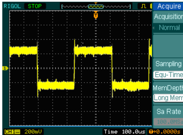
Figure 3- 2 Waveform display
