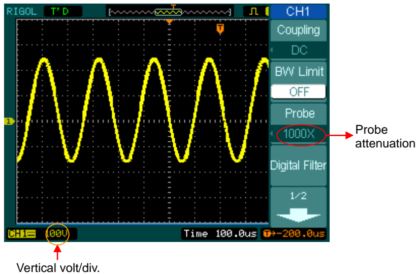
Figure 2- 8 Use the 1000:1 attenuation
