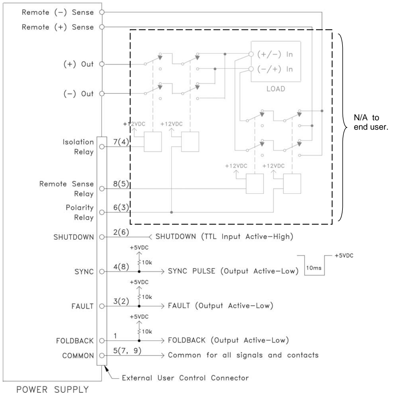
Figure 2.1-8 Example of Open Collector, TTL Input, and Relay Output Circuits
