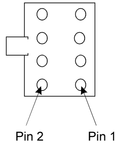
Figure 2.1-7 External User Connector Designation (8-pin Molex)
