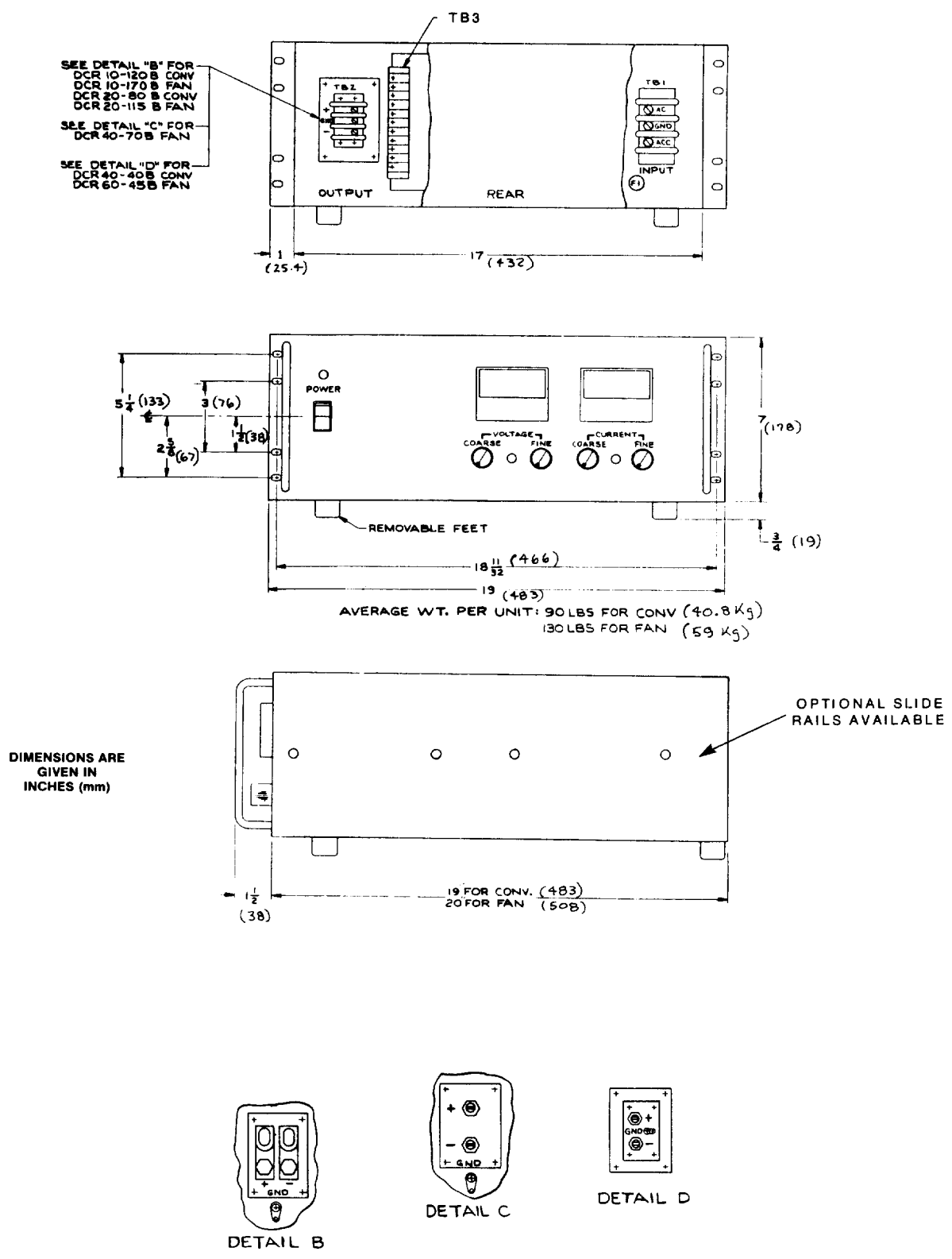
Figure 6-13 DCR-B Outline Drawing
