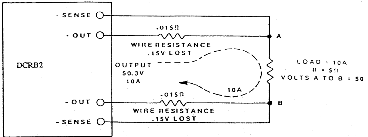
Figure 3-4 Illustration of Load Lead Resistance (Remote Sensing)
