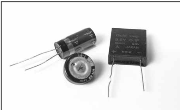
Fig. 23: Various types of double layer electrolytic capacitors.
