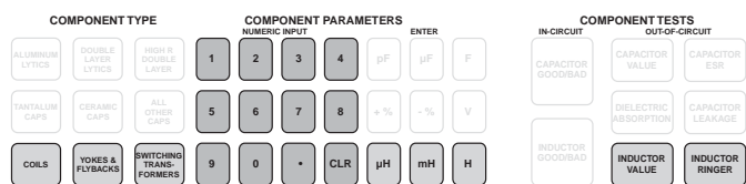
Fig. 15: Controls used for out-of-circuit inductor testing.
