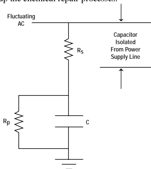
Fig. 45: The Equivalent Series Resistance has the result of isolating the capacitor from the power supply line, reducing its filtering capabilities.
