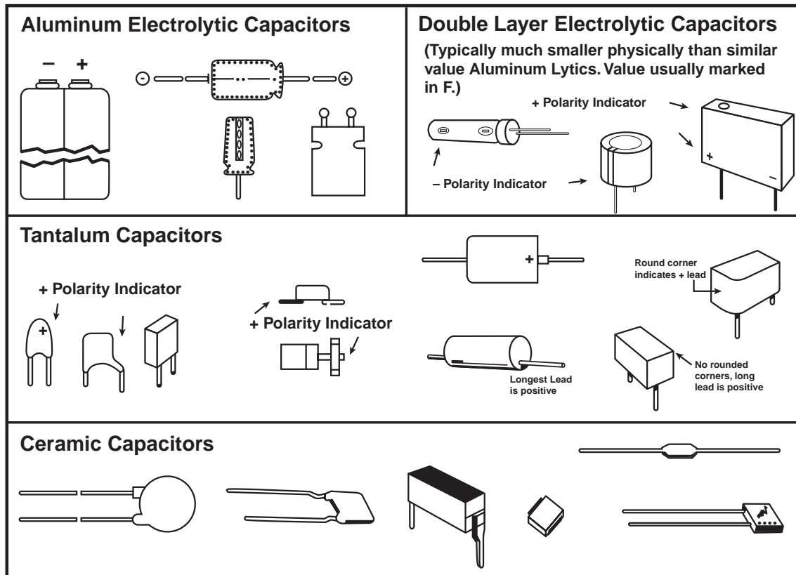
Fig. 20: Each capacitor type may be identified by its unique physical characteristics.
