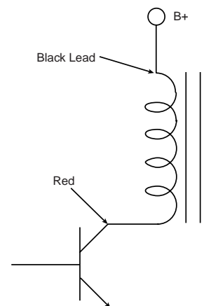
Fig. 31: Connect to the primary side of a flyback to do the ringing test.
