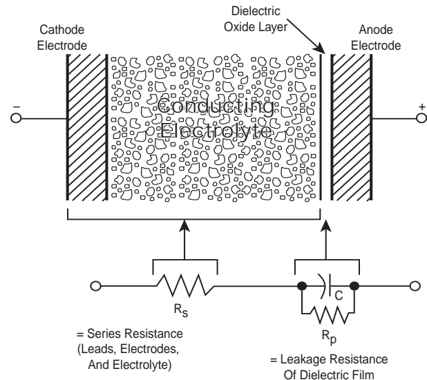
Fig. 38: Construction of an electrolytic capacitor and its equivalent circuit.
