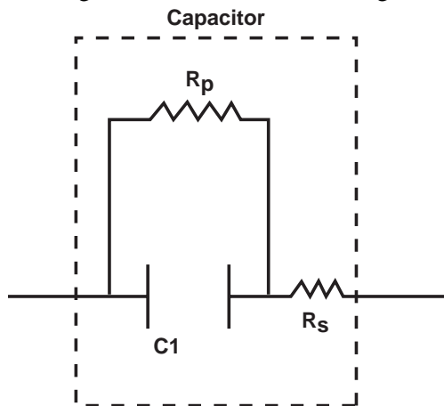
Fig. 42: Equivalent circuit of a practical capacitor.
