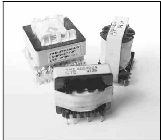
Fig. 26: Common types of switching transformers.
