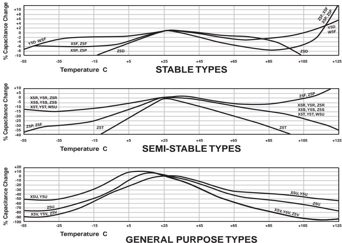
Fig. 41: Temperature change versus capacity change of non-temperature compensated ceramic disc capacitors.
