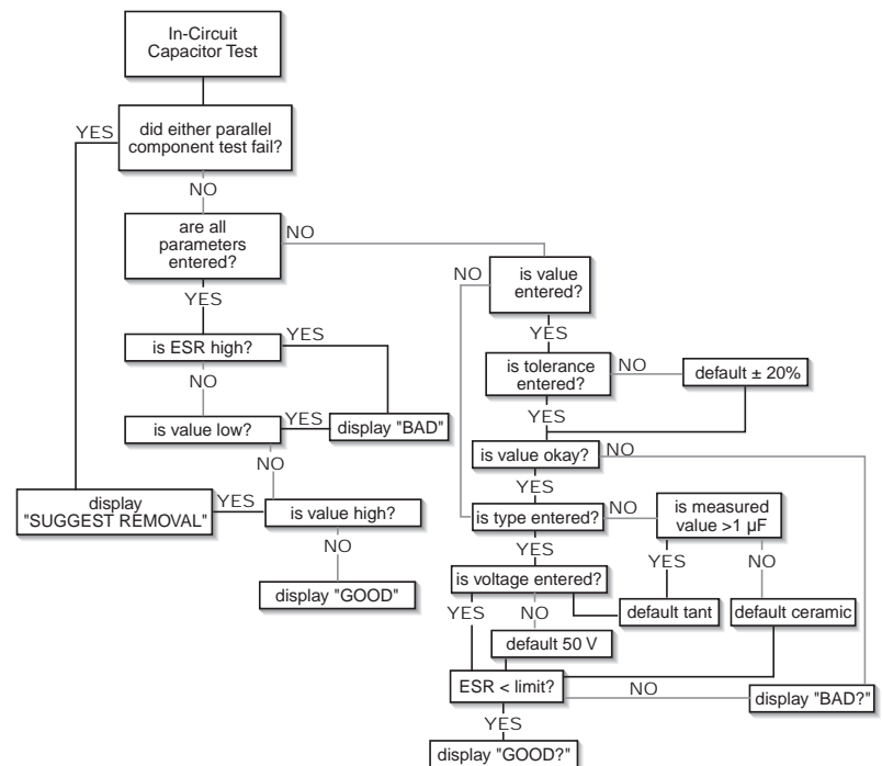
Fig. 29: In-Circuit Capacitor Test flow chart.
