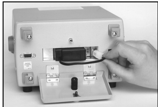
Fig. 6: The optional BY289 is installed in the LC103 for portable operation.
