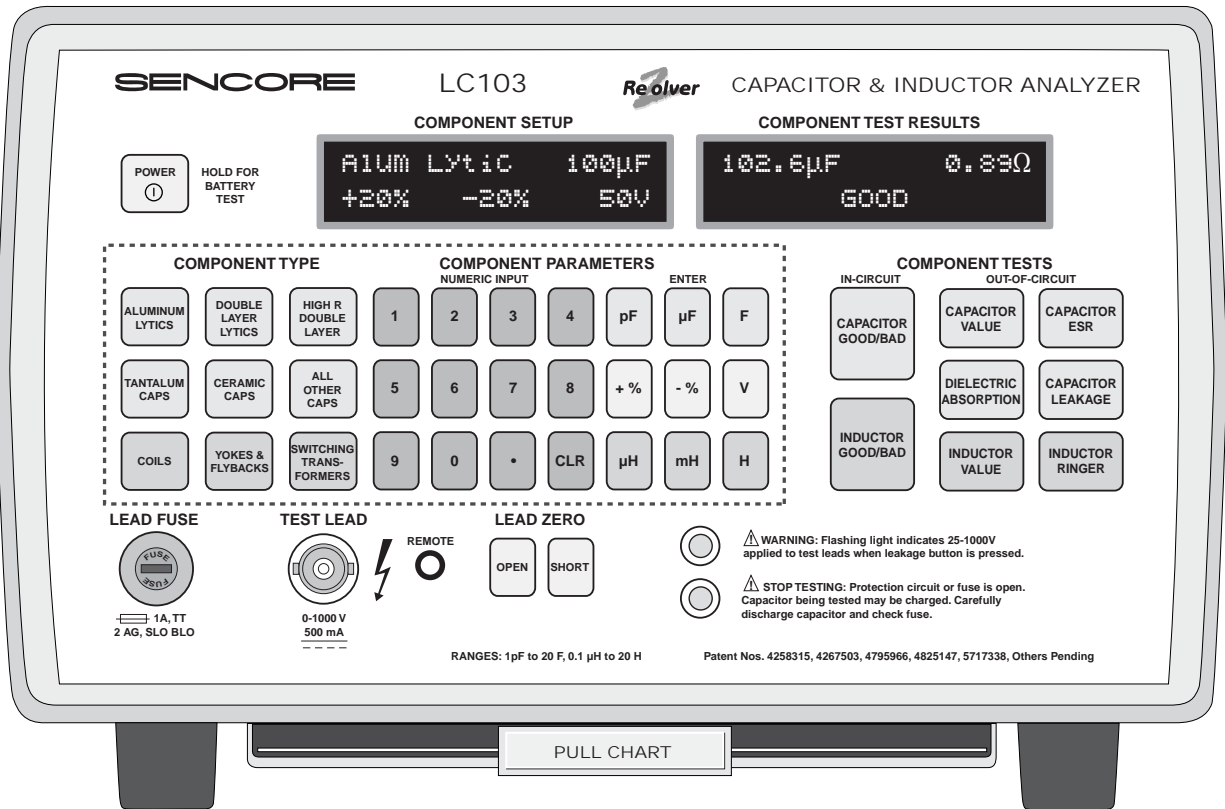
Fig. 10: Controls used for entering component data.
