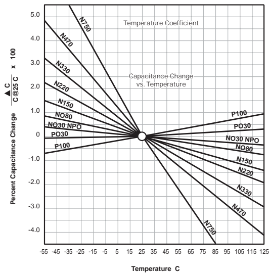
Fig. 39: Temperature change versus capacity change of P100 to N750 temperature compensated ceramic disc capacitors.
