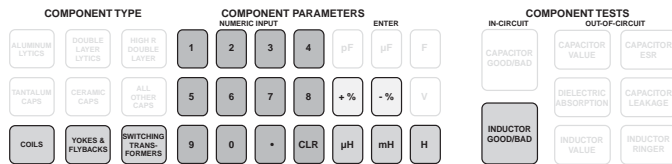
Fig. 14: Controls used for in-circuit inductor testing.
