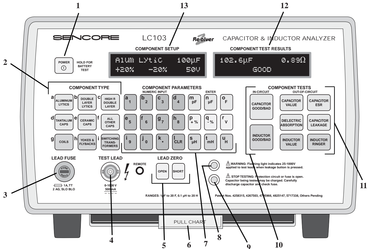
Fig. 1: Location of front panel controls.
