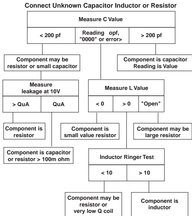
Fig. 28: Use this flow chart to help identify small axial lead inductors, capacitors, and resistors from one another.
