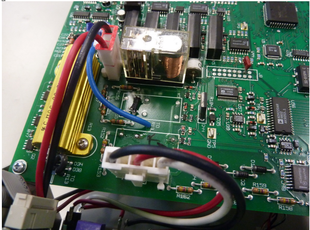
Sencore_LC103_4.JPG (443.77 kB, 1200x900 - viewed 123 times.)
