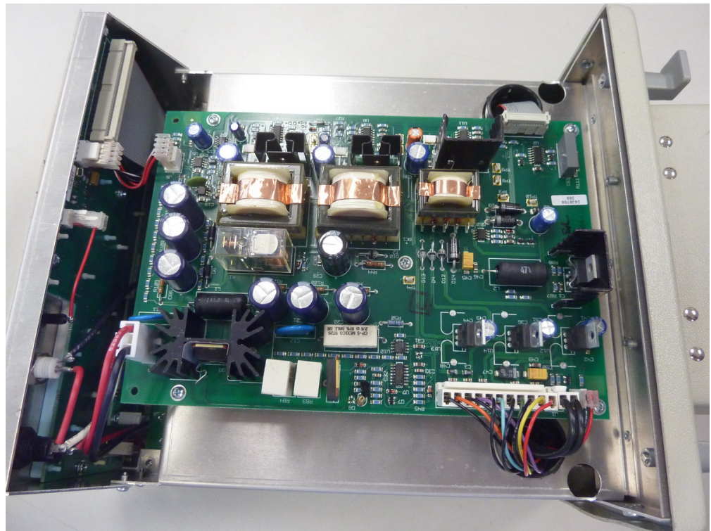
Sencore_LC103_6.JPG (404.55 kB, 1200x900 - viewed 140 times.)
