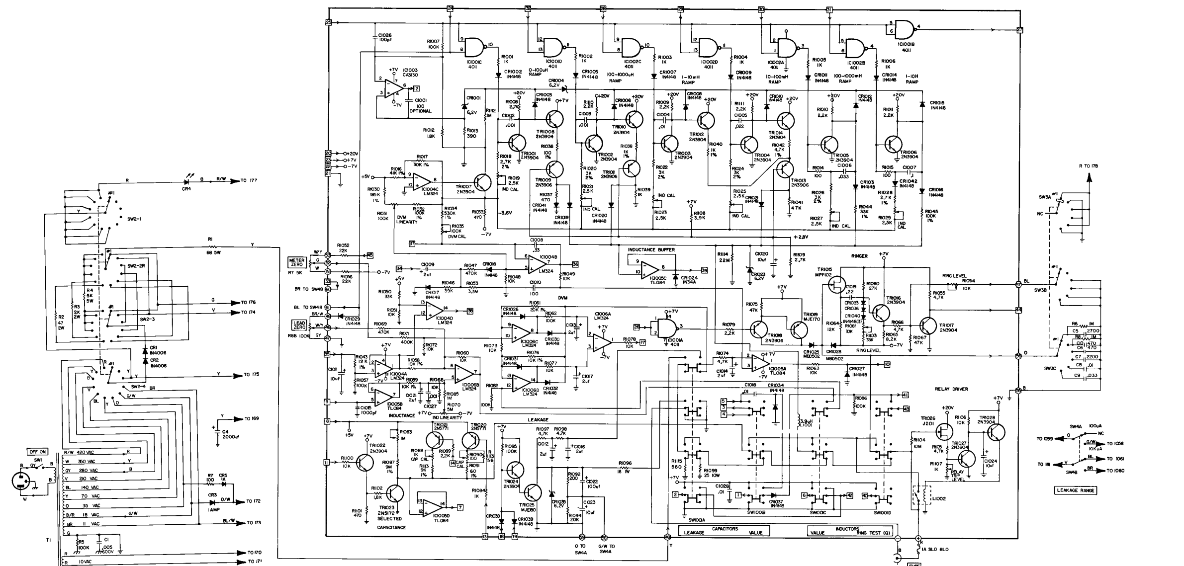
1000 BOARD - ANALOG
