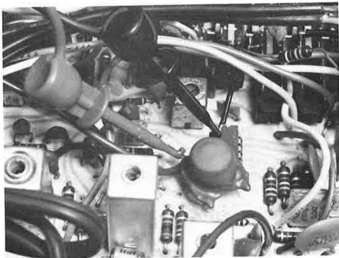
Fig. 24— Inductance values can be checked in-circuit with the LC75 inductance test.
