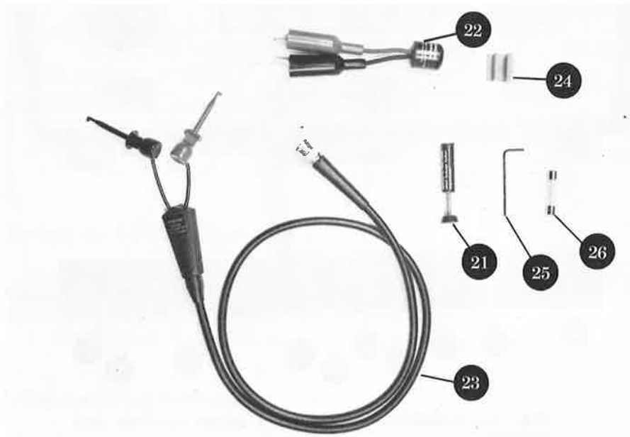
Fig. 3— Supplied accessories
