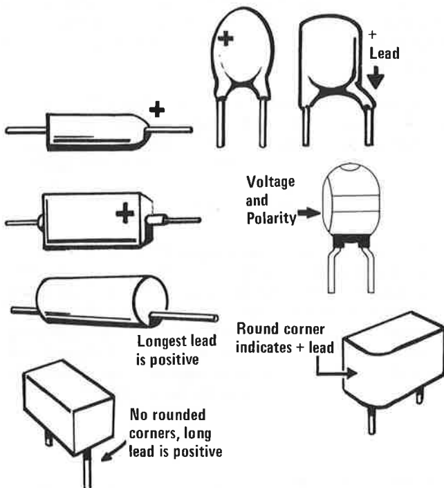
Fig. 13— Solid tantalum electrolytics come in all sizes and shapes. The most common shapes are shown here.
