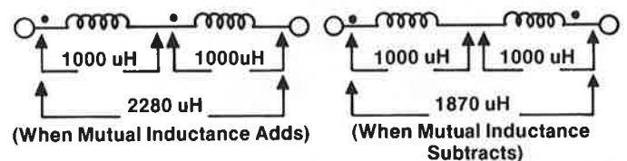
Fig. 26— The "Z METER 2" will show the actual inductance of two coils with mutual inductance. Mutual inductance can either add or subtract from the individual reading of the windings.
