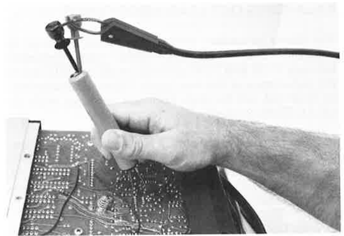
Fig. 25— The optional Touch Test Probe can be used with the "Z METER 2" to check the inductance and ringing of coils that are mounted flat on the PC board.
