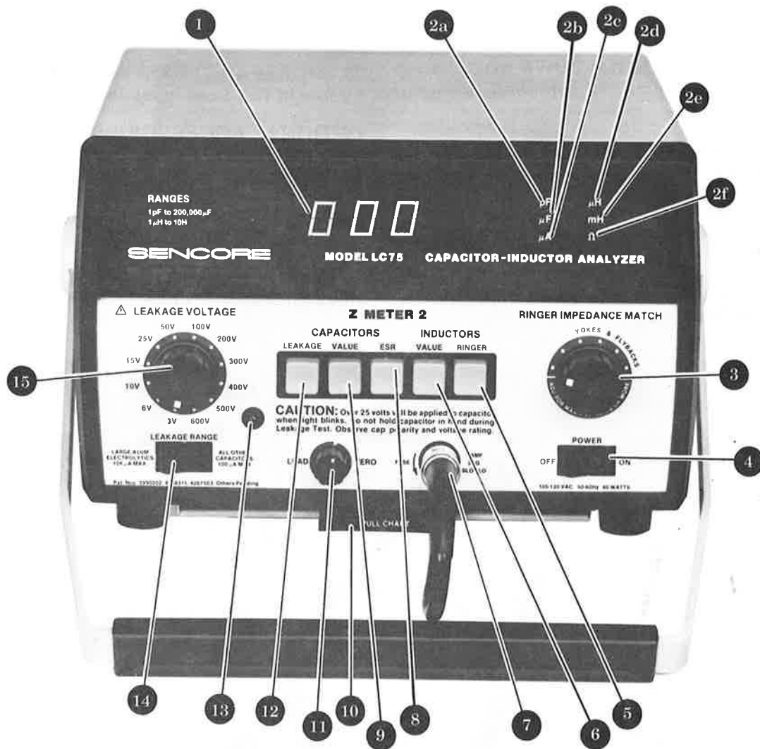
Fig. 1— Location of LC75 front panel controls and features.
