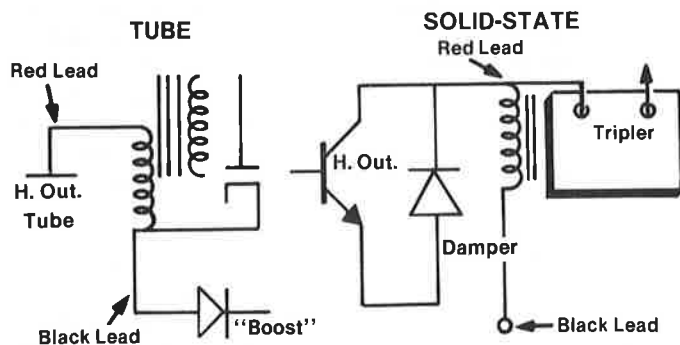
Fig. 29—The "Z METER 2" provides a quick in-circuit ringing test on tube or solid state chassis.
