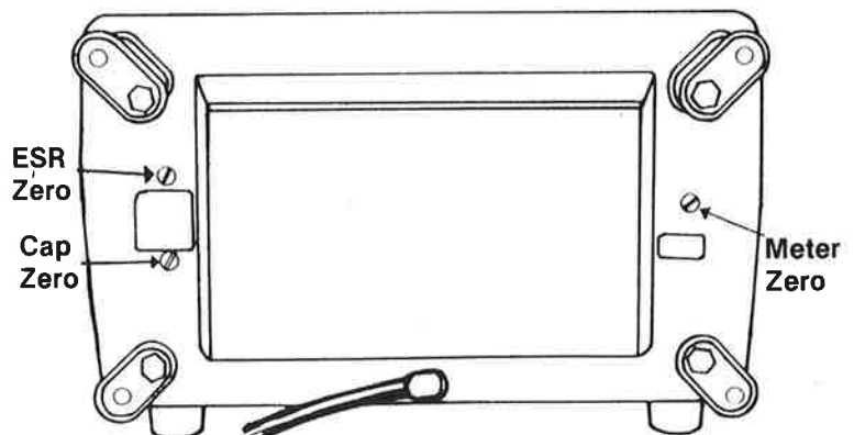
Fig. 30— LC75 Zeroing Adjustments
