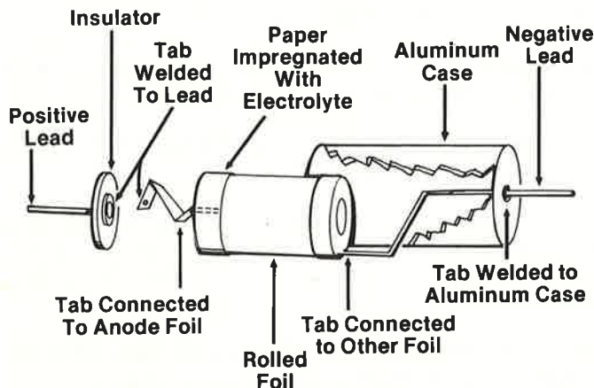
Fig. 19— An electrolytic can become intermittent due to a poor or corroded weld.
