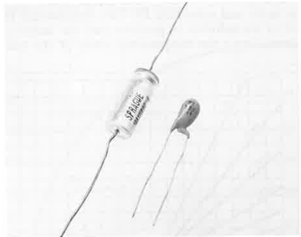
Fig. 37— The tantalum lytic on the right is much smaller in physical size than an aluminum lytic of similar capacity and working voltage.
