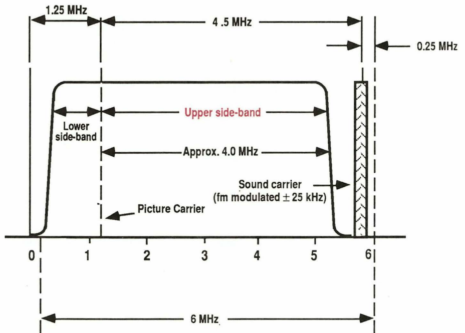
Fig. 1: The broadcast industry uses vestigial sideband RF signal, and you must set the tuner to the upper sideband.
