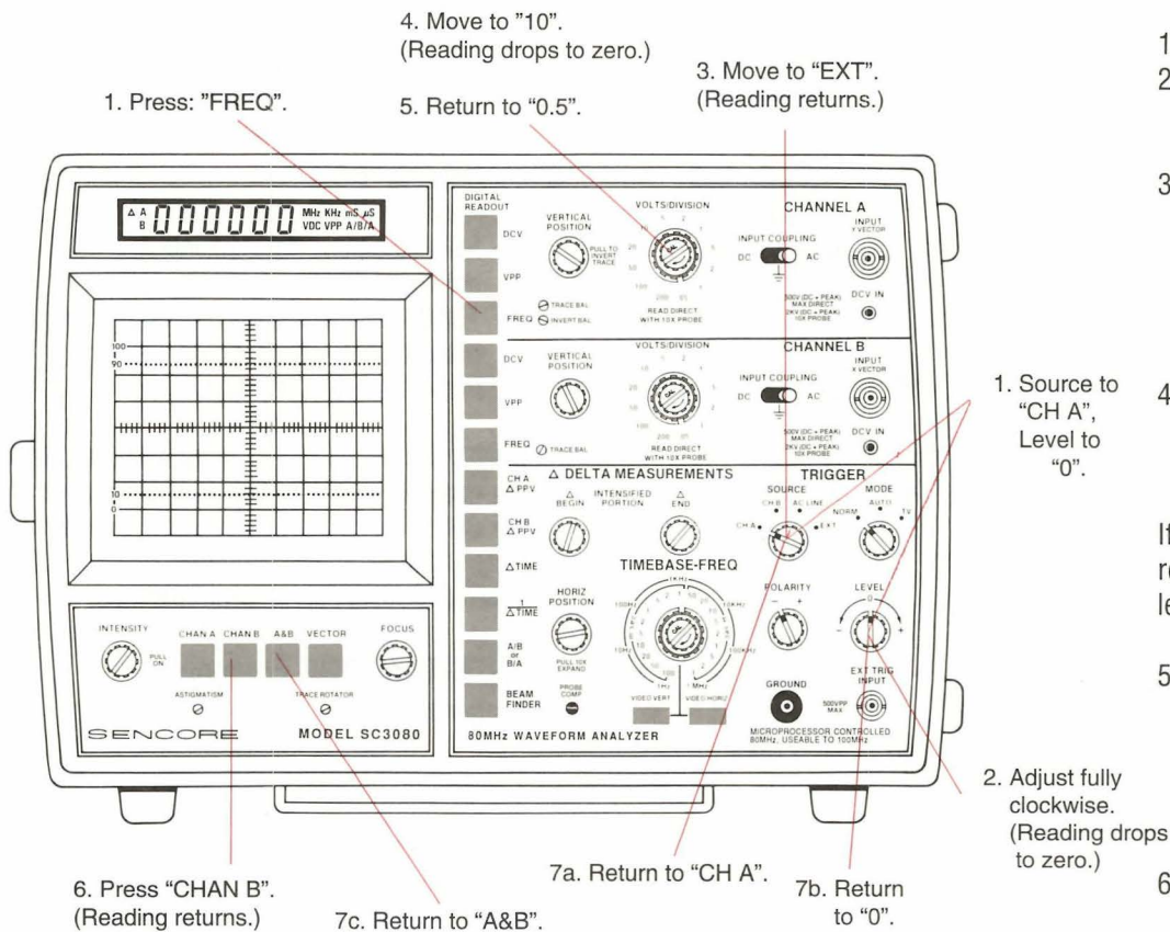
Fig. 10: The frequency function needs the triggering circuits to be properly adjusted, and then automatically displays frequency.
