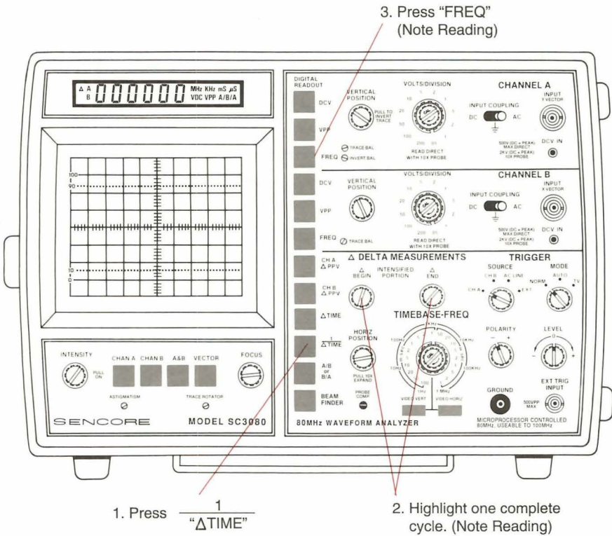
Fig. 13: The 1/Δ TIME function lets you measure frequency more accurately than a conventional scope. But always use the AUTO-TRACKING FREQ function if high accuracy is needed.
