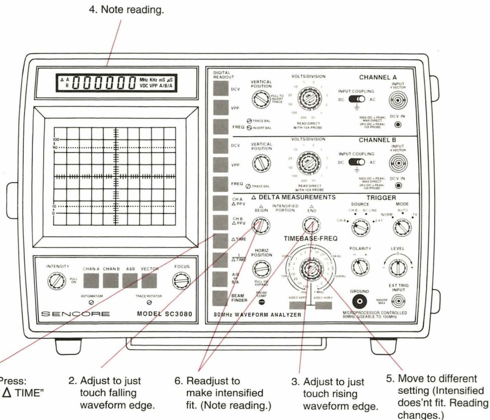
Fig. 12: The \Delta TIME readings are accurate whether the horizontal circuits are in or out of the "cal" mode.
