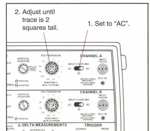
Fig. 4: Step #2: GET A FAT LINE. After the trace is on the screen, these steps ensure the signal is large enough to measure.
