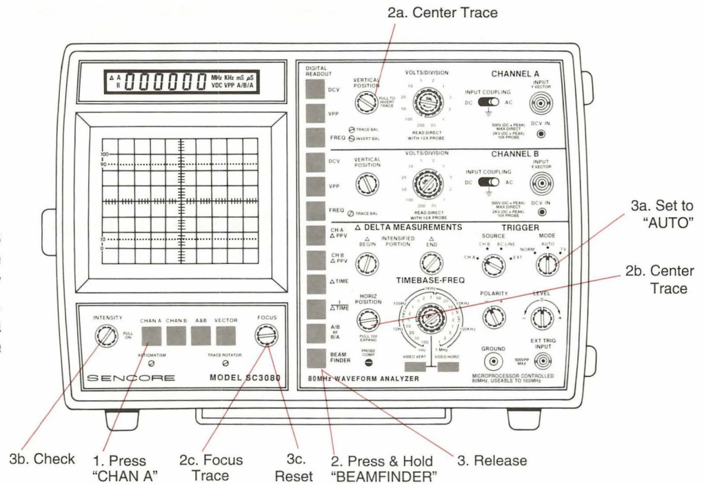
Fig. 3: Step #1: GET A LINE. Following these steps always returns a trace to the CRT, no matter how badly the front panel controls are misadjusted.
