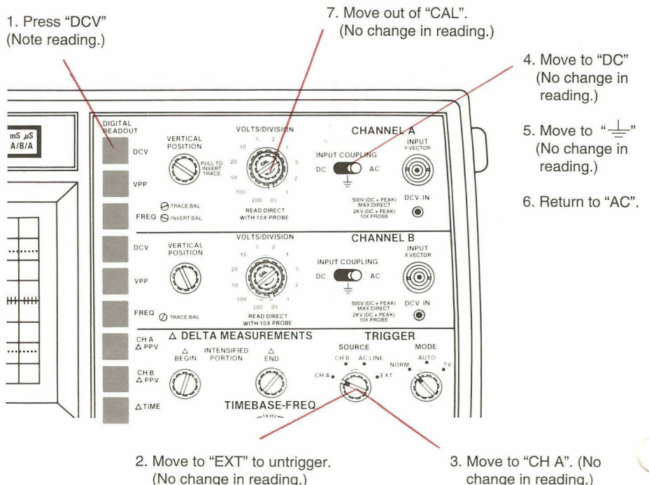
Fig. 8: Follow these steps as you learn to make DC voltage readings.
