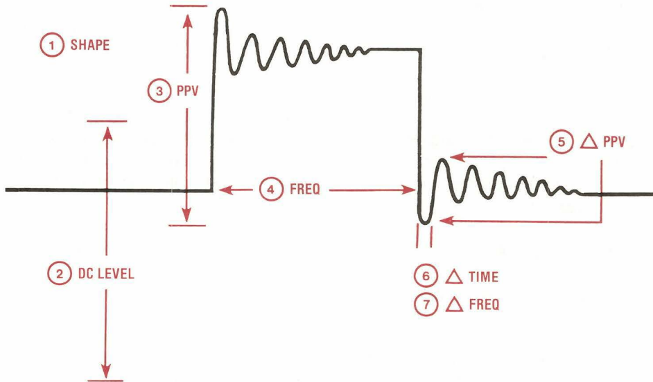
Fig. 6: These seven steps let you fully analyze any waveform. With the SC3080, you only use the CRT for step #1. The digital readout provides steps #2 through #7.
