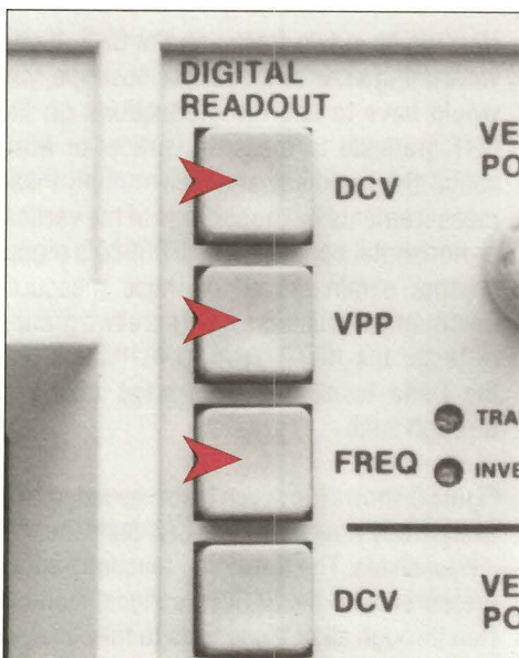
Fig. 7: The AUTO-TRACKING™ functions are DC volts, peak-to-peak volts and frequency. Each automatically tracks along with the CRT to measure the parameter from the entire waveform.
