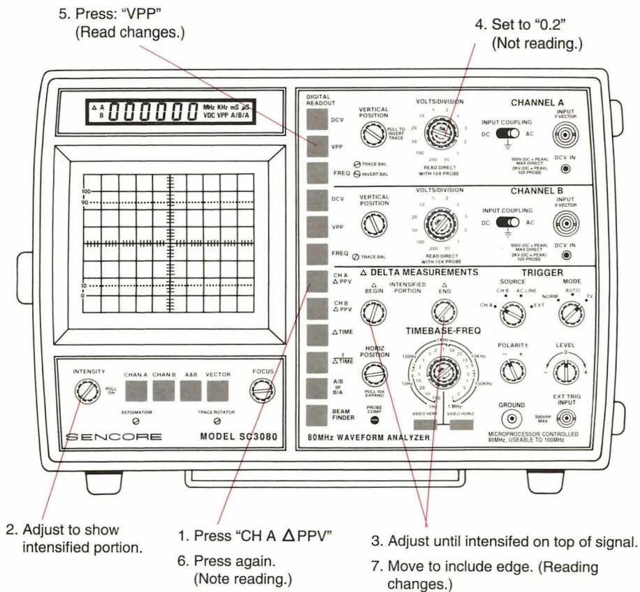
Fig. 11: The \Delta PPV function lets you measure the amplitude of any small part of a waveform.
