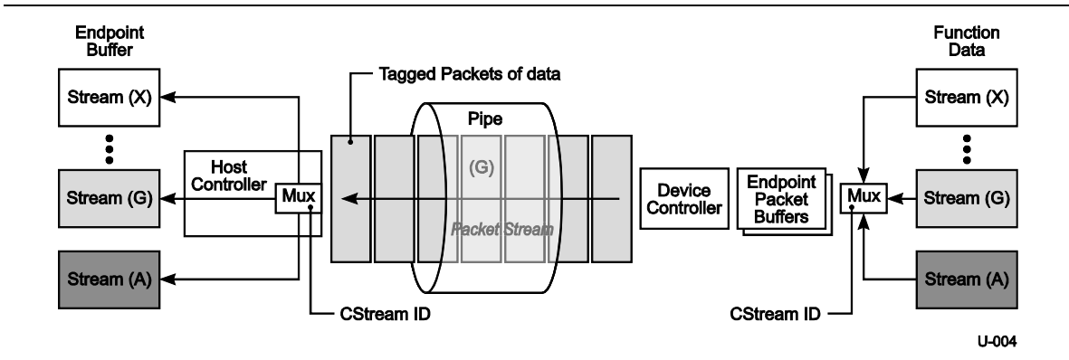
Figure 4-3. Enhanced SuperSpeed IN Stream Example
