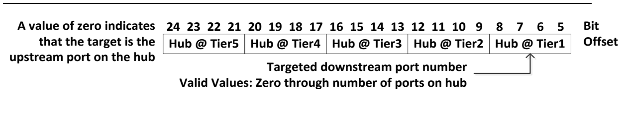
Figure 8-32. Route String Detail
