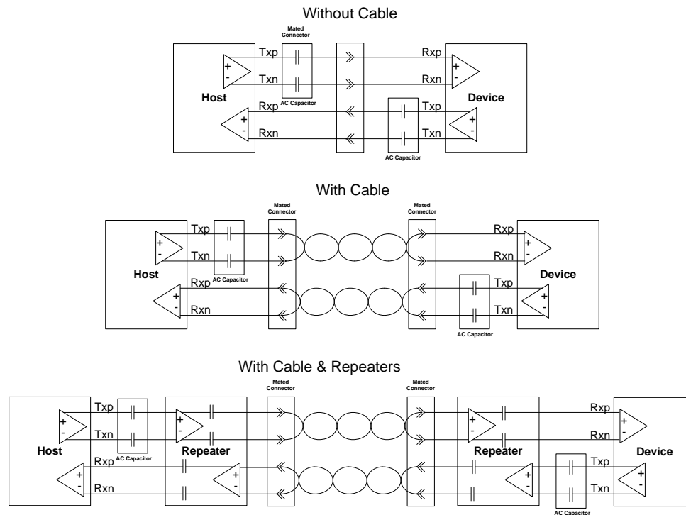
Figure 6-5. Channel Models
