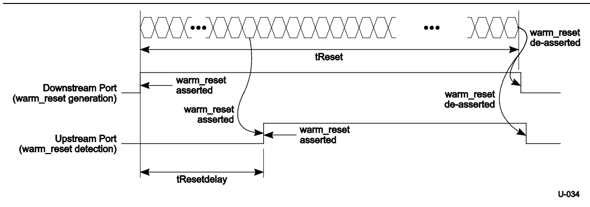
Figure 6-31. Example of Warm Reset Out of U3
