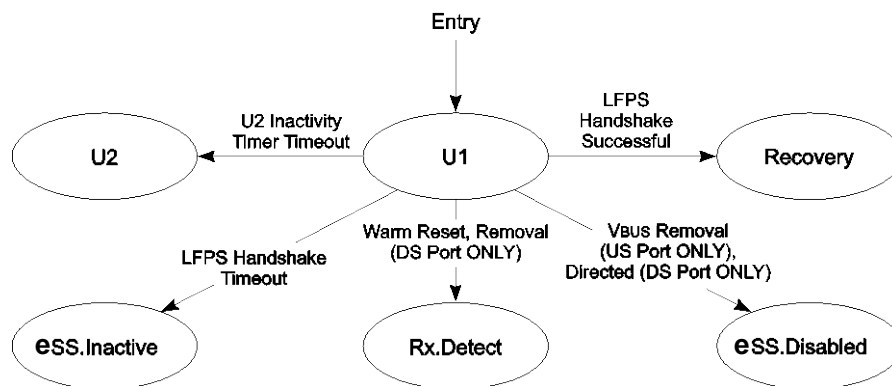
Figure 7-19. U1
