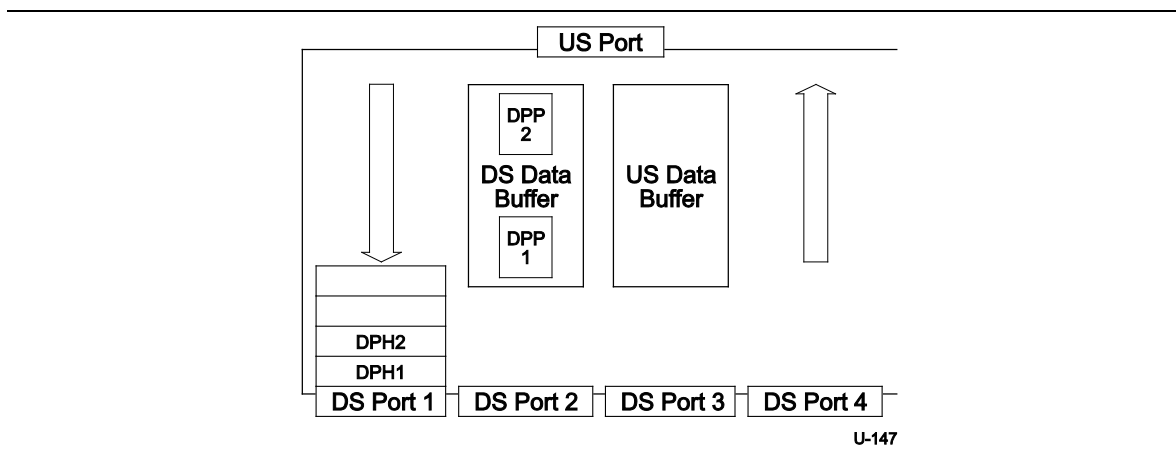
Figure 10-9. SuperSpeed Hub Data Buffer Traffic (Header Packet Buffer Only Shown for DS Port 1)
