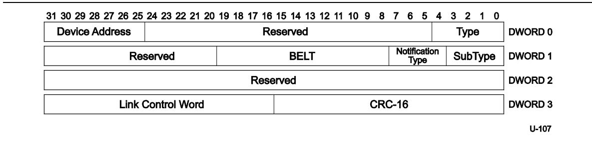
Figure 8-25. Latency Tolerance Message Device Notification
