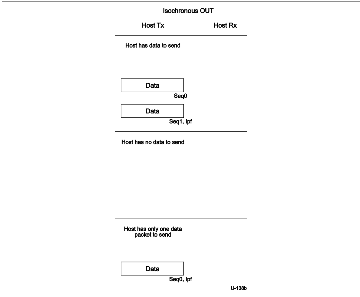
Figure 8-63. Sample Enhanced SuperSpeed Isochronous OUT Transaction
