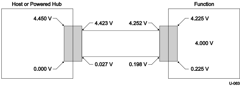
Figure 11-5. Worst-case Voltage Drop Topology (Steady
