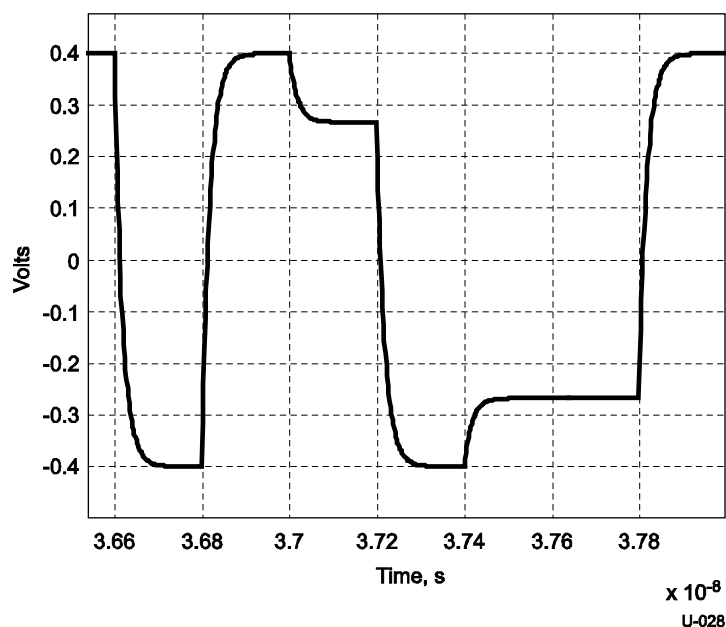
Figure 6-20. De-Emphasis Waveform
