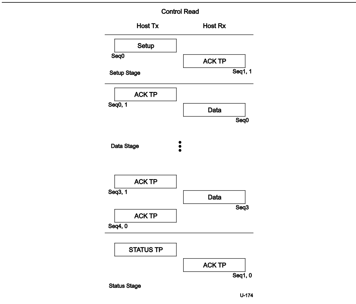
Figure 8-47. Control Read Sequence
