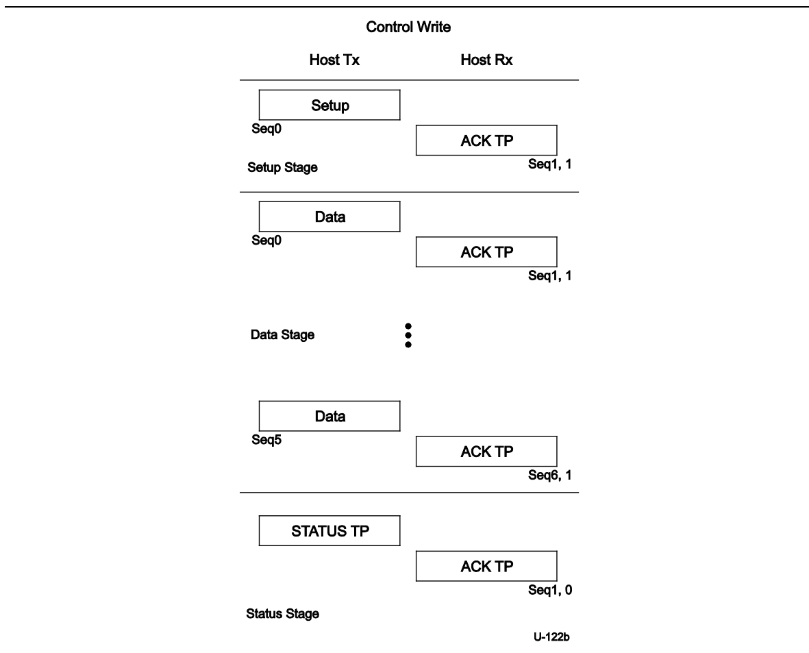
Figure 8-48. Control Write Sequence
