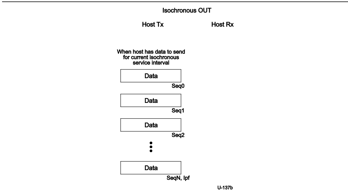
Figure 8-61. Enhanced SuperSpeed Isochronous OUT Transaction Format
