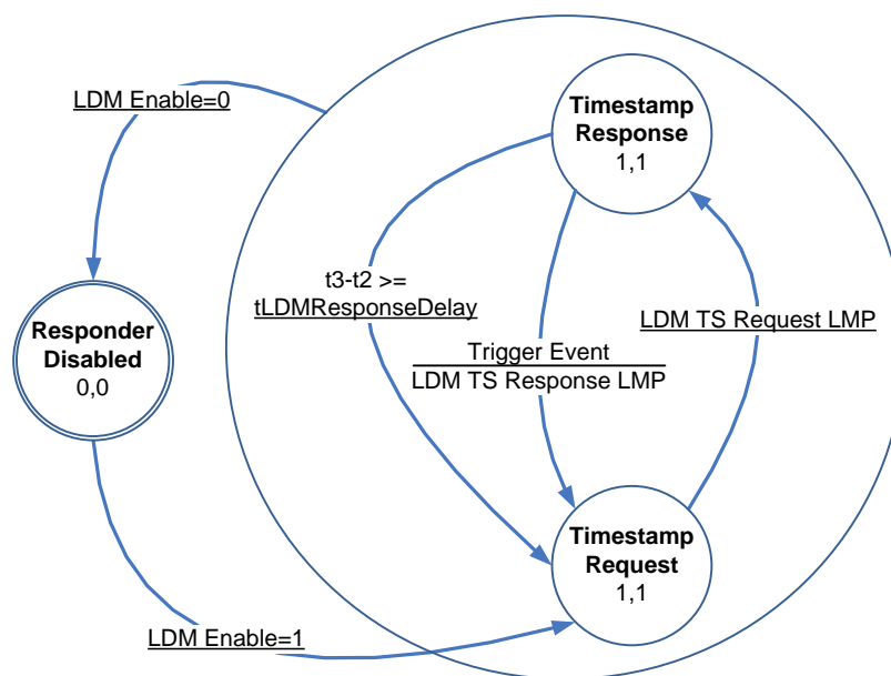
Figure 8-15. LDM Responder State Machine
