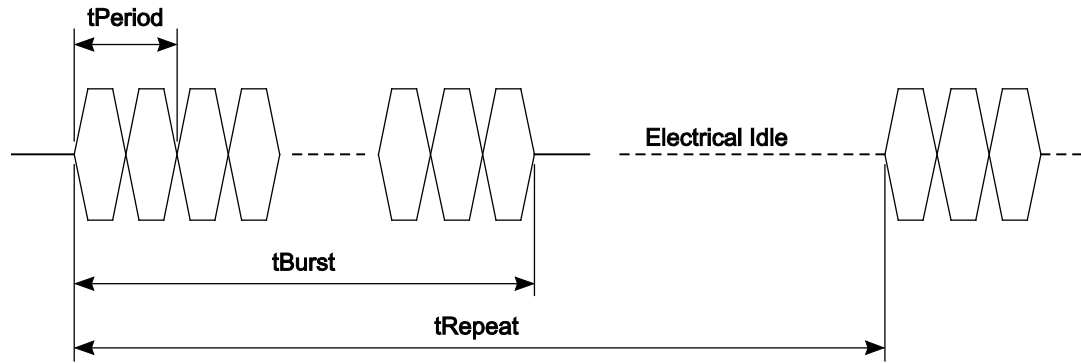
Figure 6-29. LFPS Signaling
