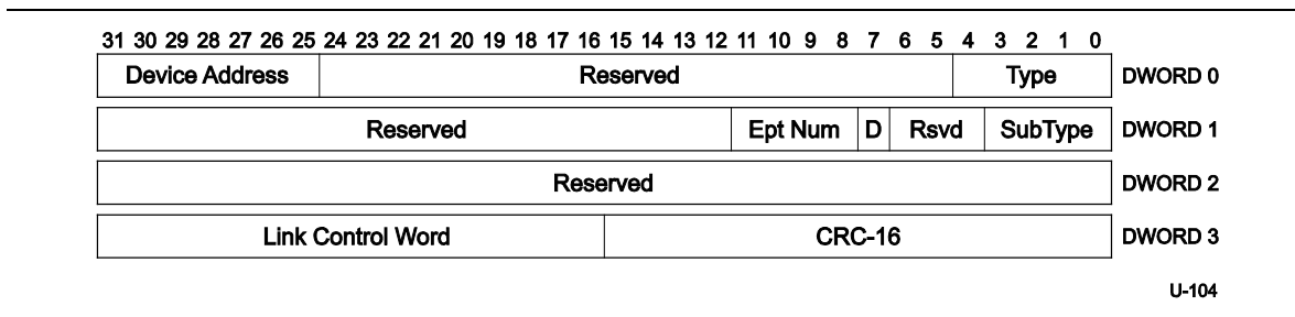
Figure 8-22. STALL Transaction Packet
