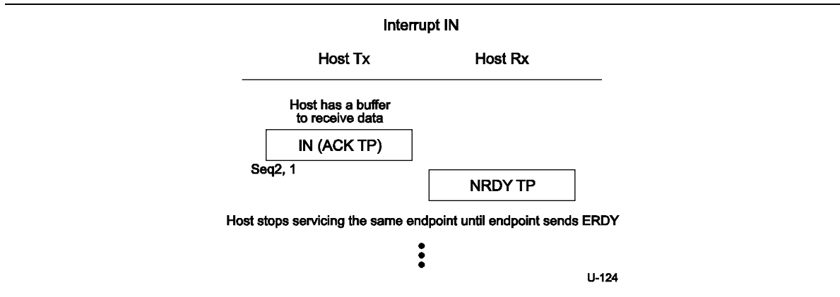
Figure 8-50. Host Stops Servicing Interrupt IN Transaction Once NRDY is Received
