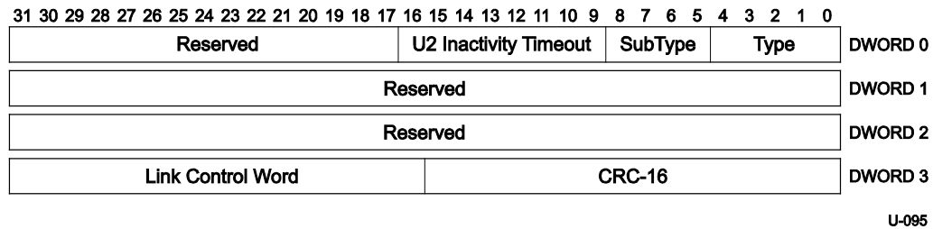
Figure 8-6. U2 Inactivity Timeout LMP
