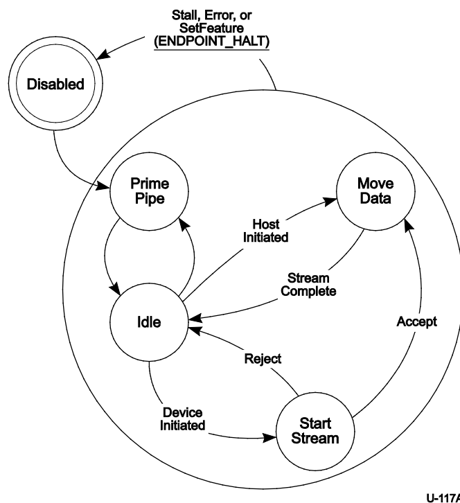
Figure 8-38. General Stream Protocol State Machine (SPSM)
