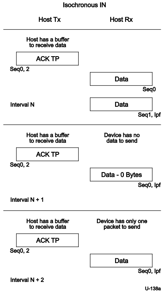
Figure 8-62. Sample Enhanced SuperSpeed Isochronous IN Transaction
