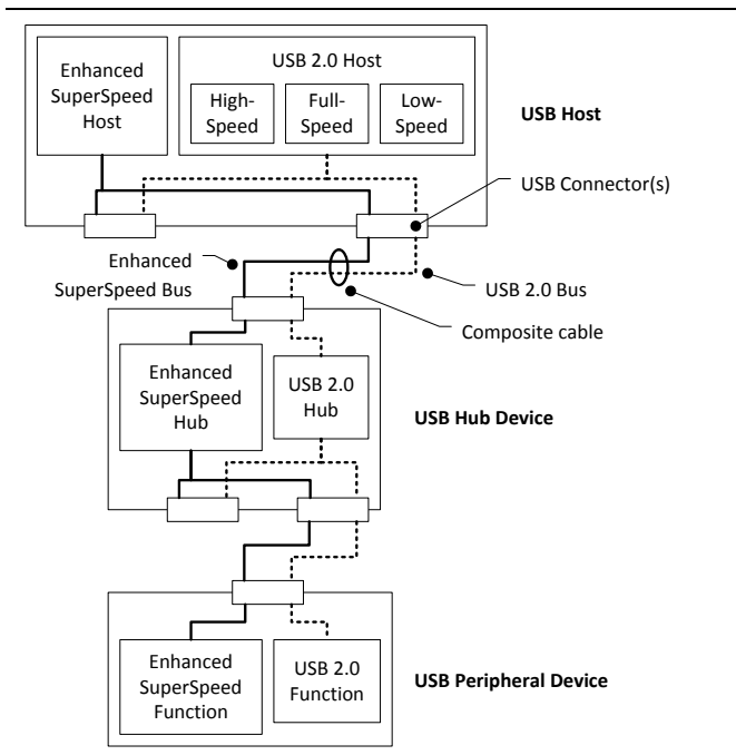
Figure 3-1. USB 3.1 Dual Bus System Architecture
