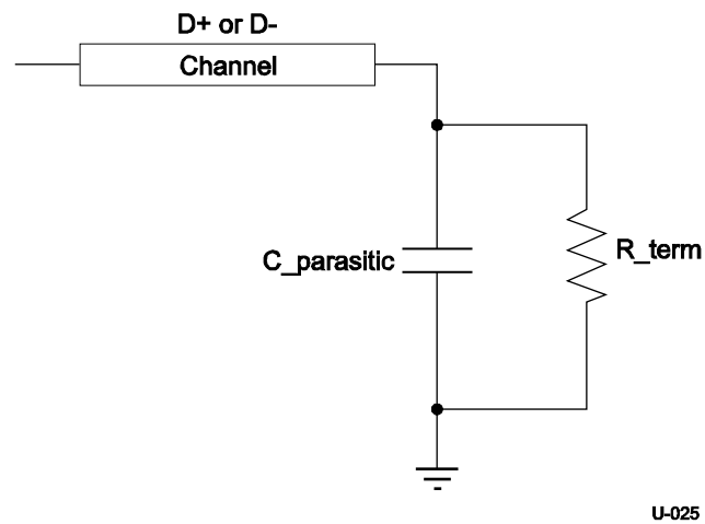
Figure 6-18. Device Termination Schematic
