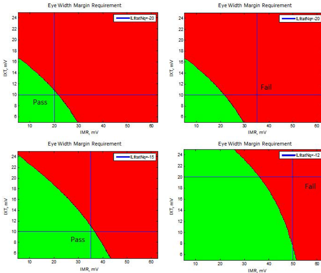
Figure 5-26. Pass/Fail Examples
