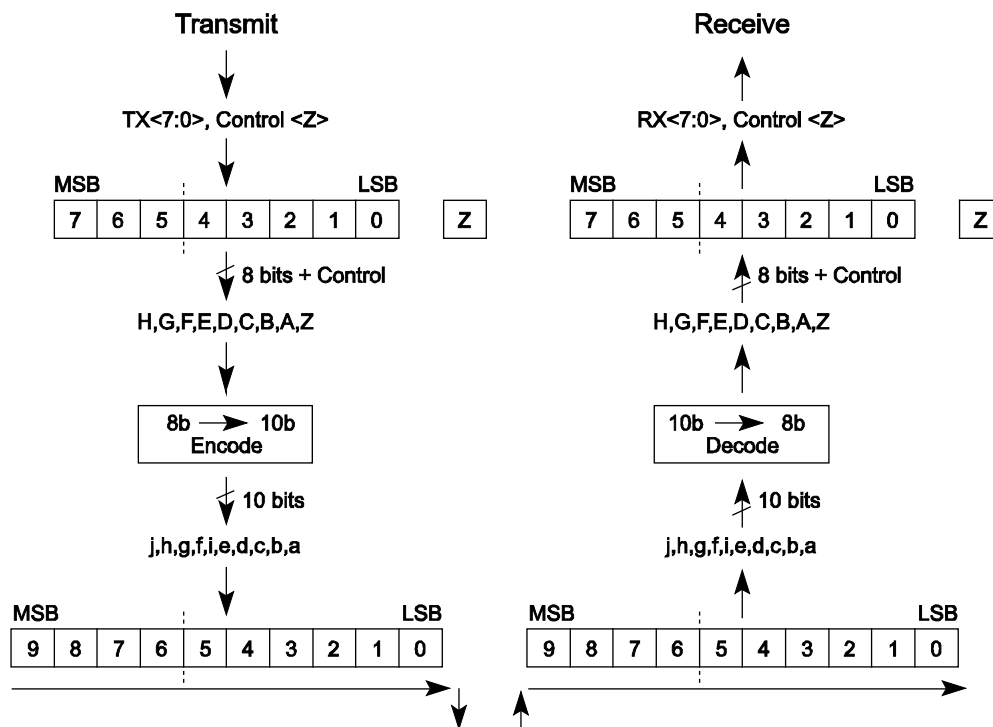
Figure 6-6. Character to Symbol Mapping
