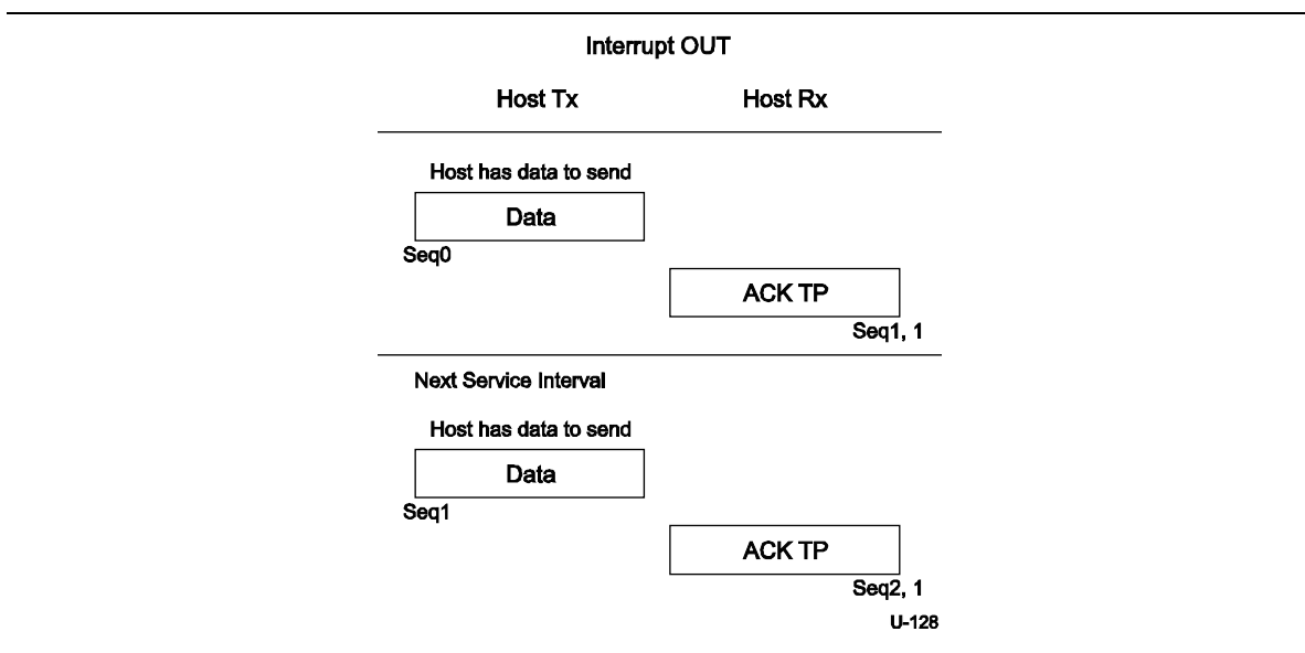
Figure 8-54. Host Sends Interrupt OUT Transaction in Each Service Interval
