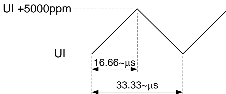
Figure 6-15. Example of Period Modulation from Triangular SSC
