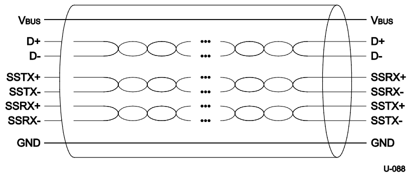
Figure 3-2. USB 3.1 Cable
