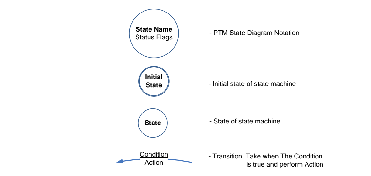
Figure 8-13. LDM State Machine Notation
