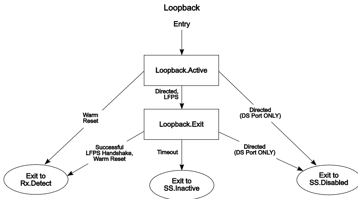
Figure 7-23. Loopback Substate Machine
