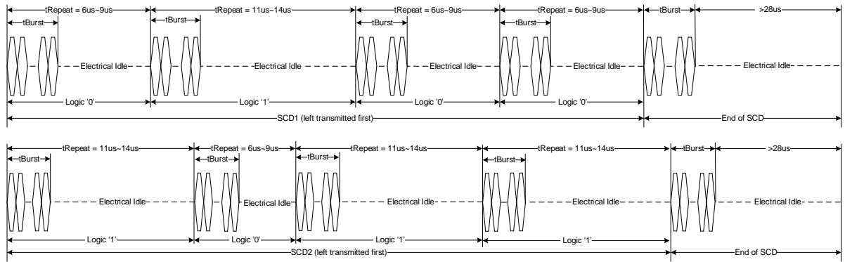
Figure 6-33. SCD1/SCD2 transmission
