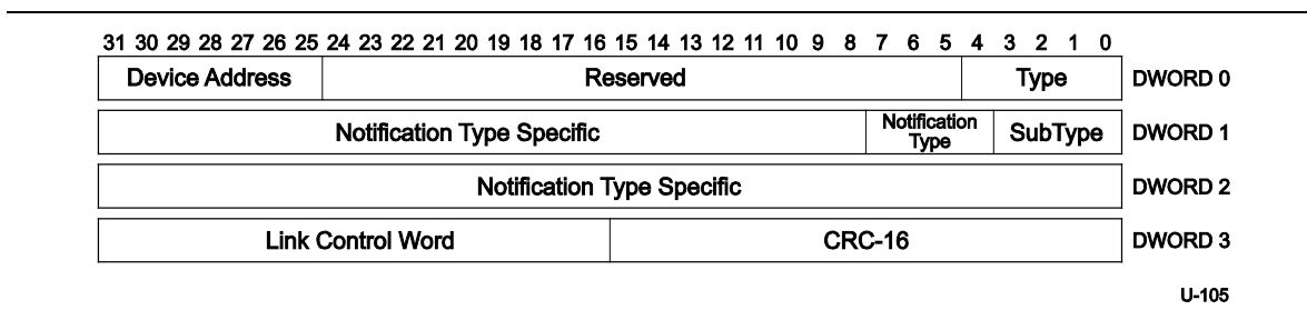
Figure 8-23. Device Notification Transaction Packet
