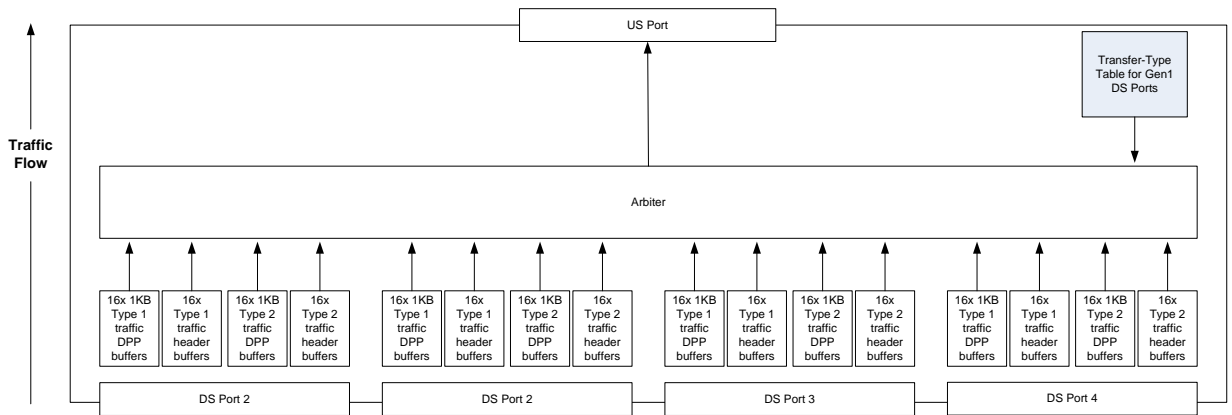
Figure 10-17. Logical Representation of Upstream Flowing Buffers
