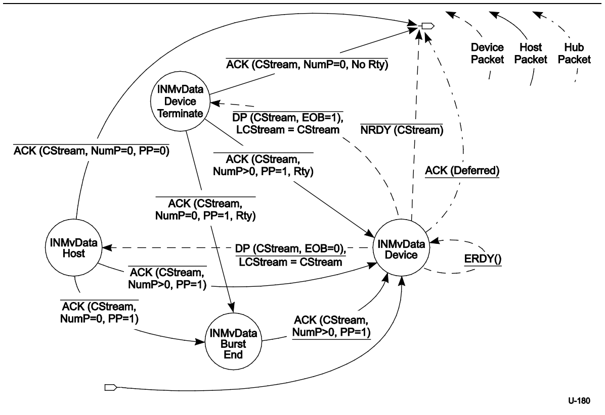
Figure 8-44. Host IN Move Data State Machine (HIMDSM)
