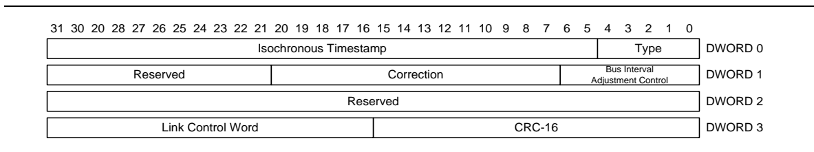
Figure 8-31. Isochronous Timestamp Packet
