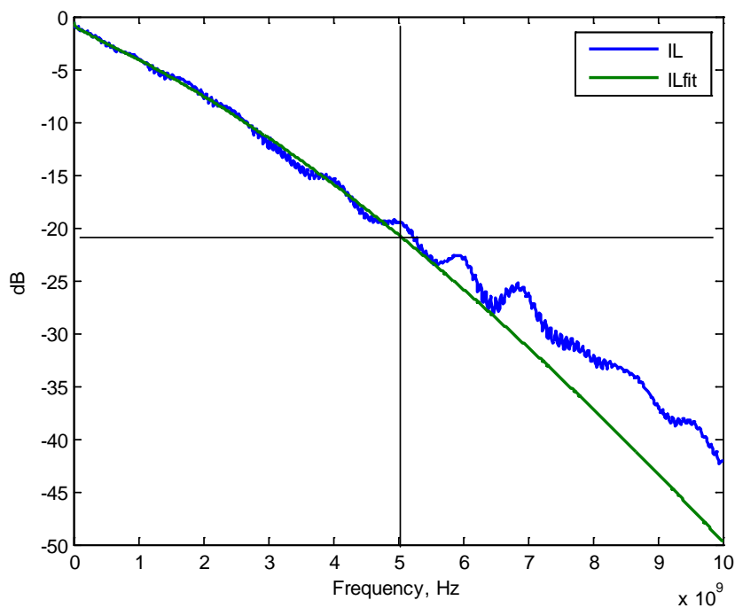
Figure 5-24. Illustration of Insertion Loss Fit at Nyquist Frequency
