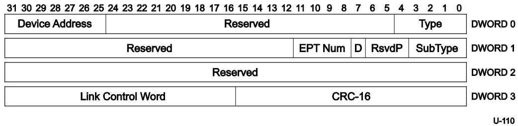
Figure 8-29. PING_RESPONSE Transaction Packet
