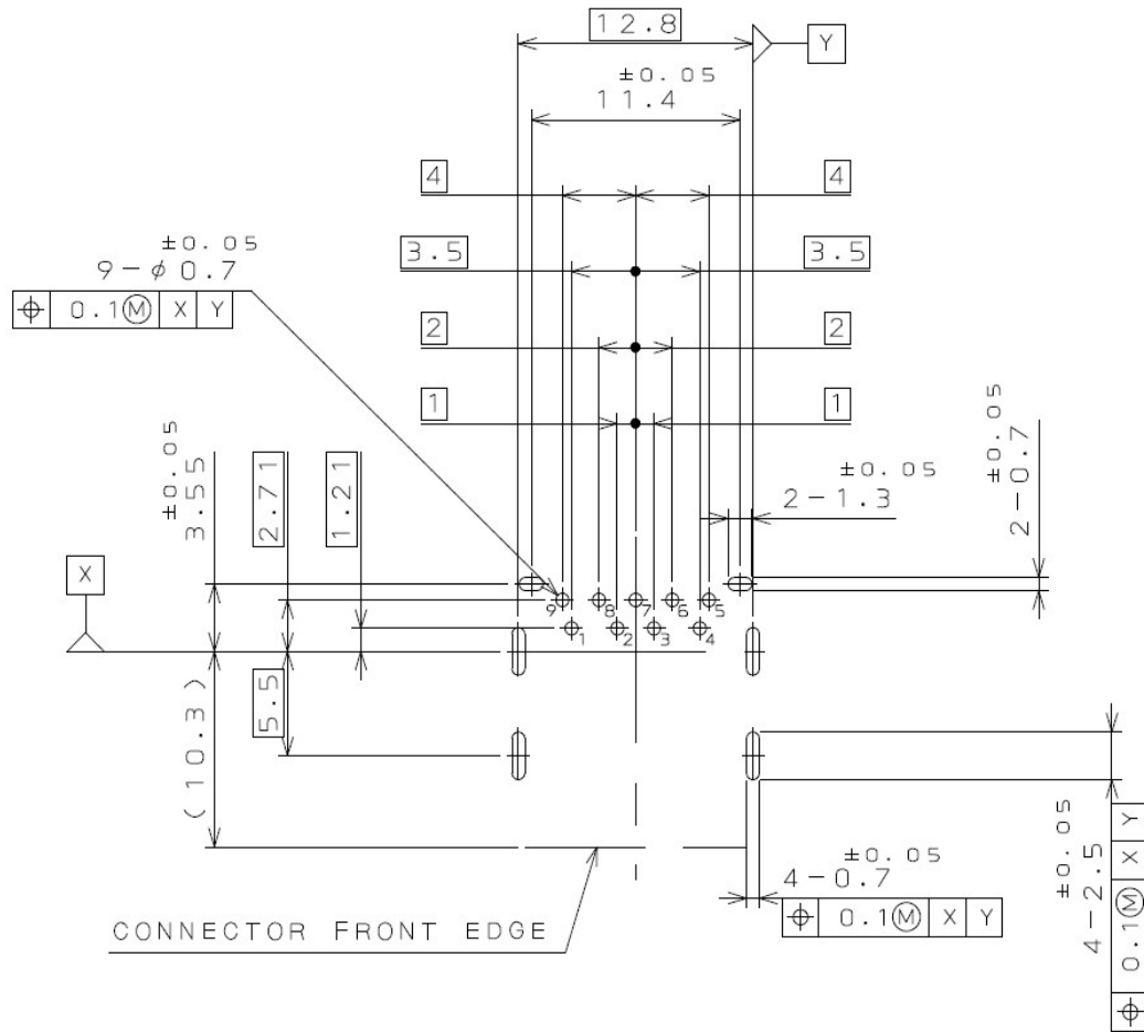
PCB LAYOUT (REF.) (STANDARD MOUNT TYPE)
