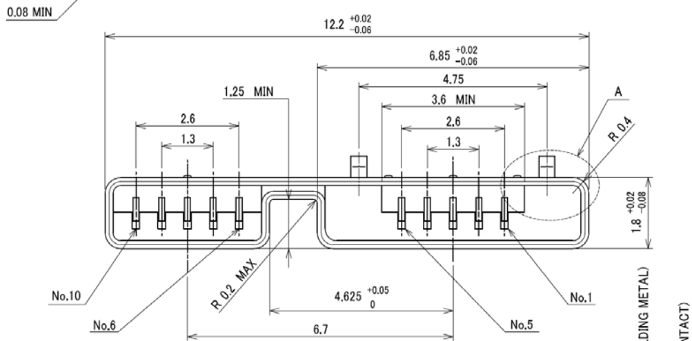
USB3.0 Micro-A Plug
