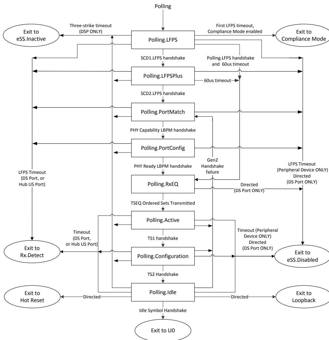
Figure 7-18. Polling Substate Machine
