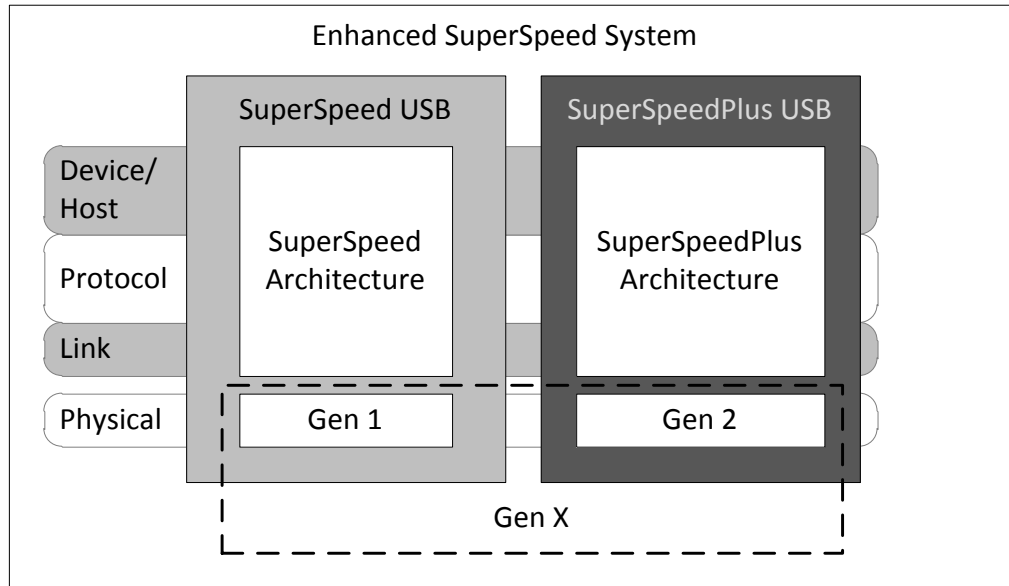
Figure 3-3. USB 3.1 Terminology Reference Model
