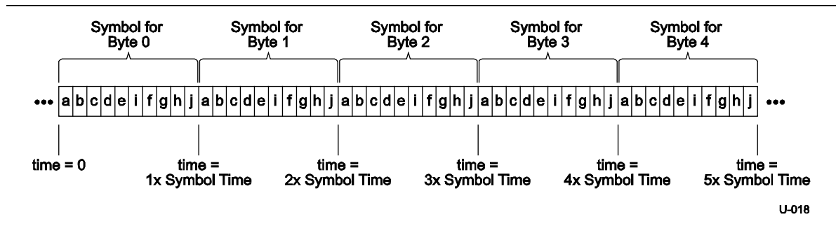
Figure 6-7. Bit Transmission Order
