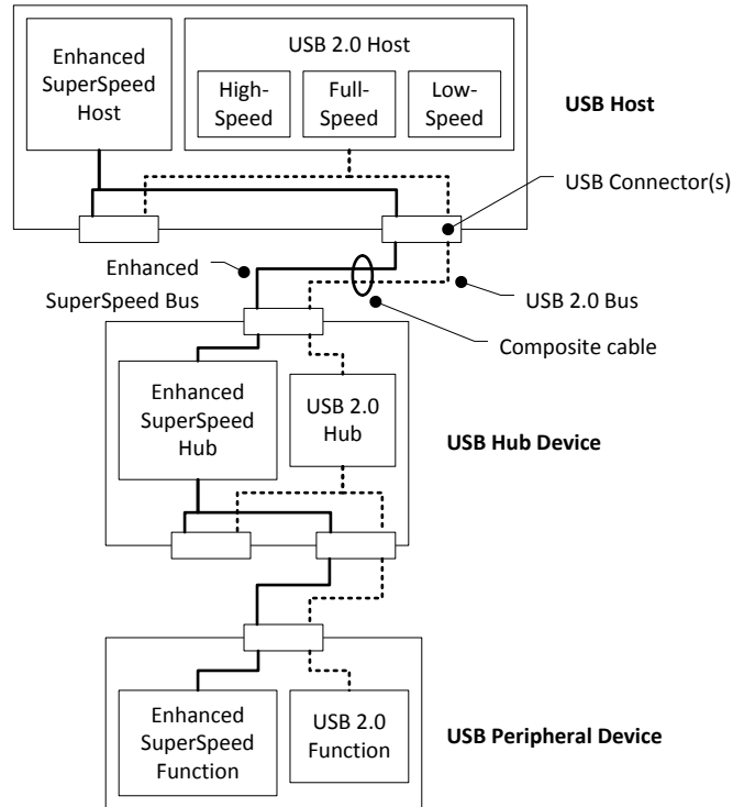
Figure 10-4. Simple USB Topology
