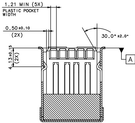
SECTION S-S
