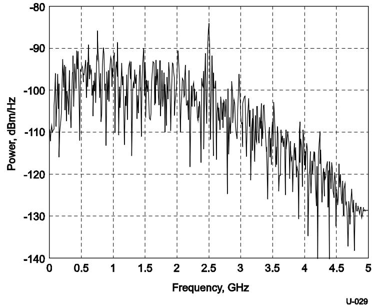
Figure 6-23. Frequency Spectrum of TSEQ
