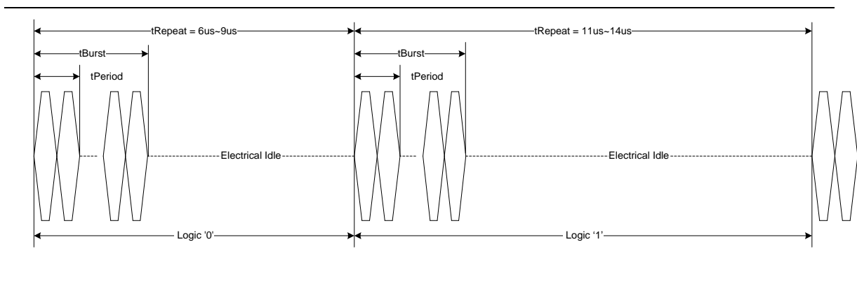
Figure 6-32. Example of Binary Representation based on Polling.LFPS
