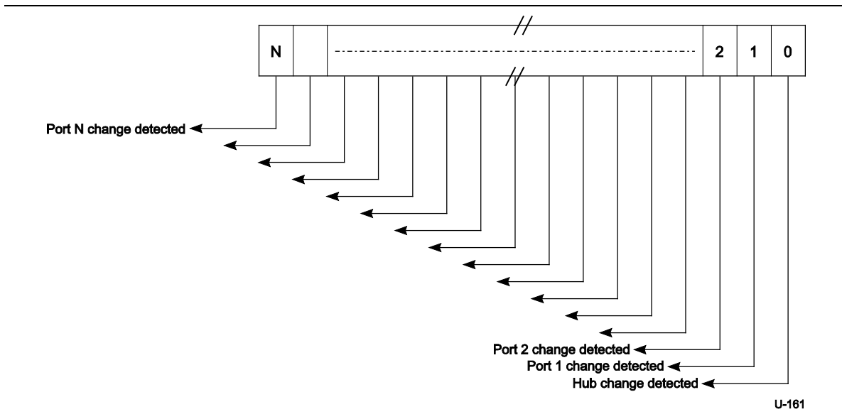
Figure 10-24. Hub and Port Status Change Bitmap
