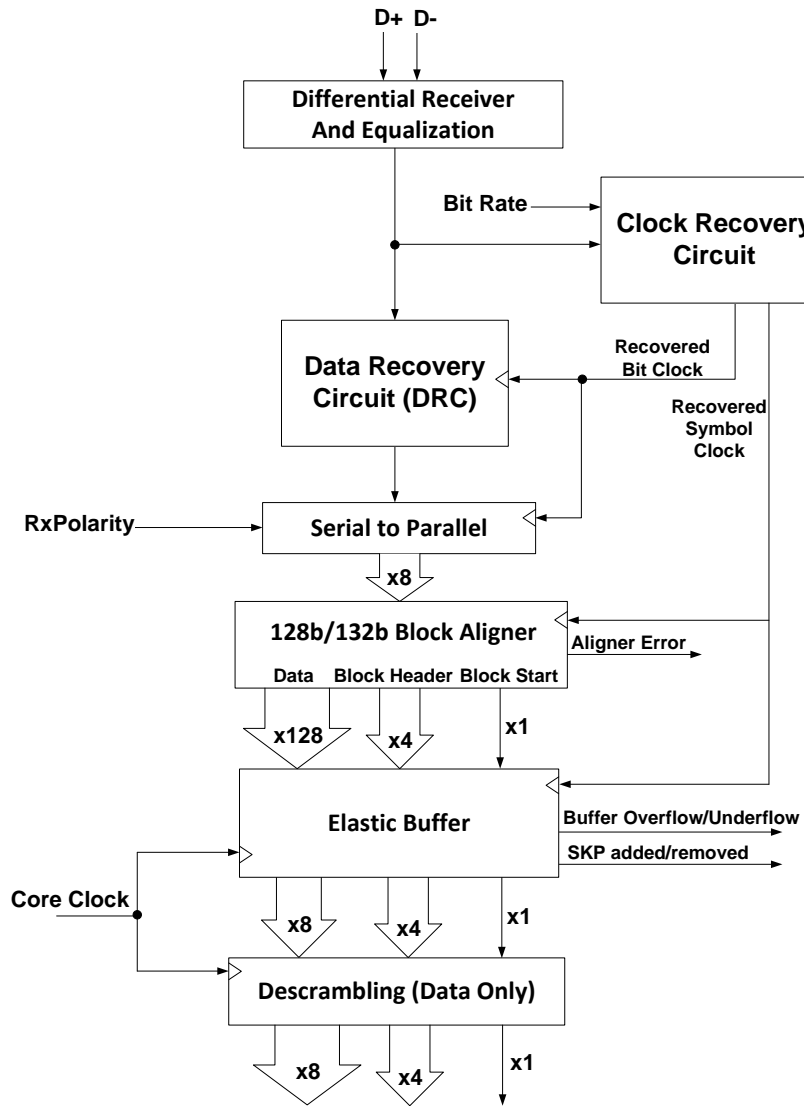
Figure 6-4. Gen 2 Receiver Block Diagram
