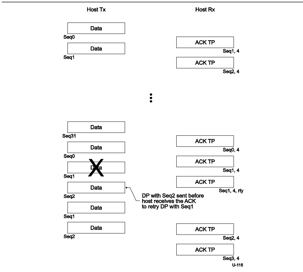
Figure 8-37. Sample BULK OUT Sequence
