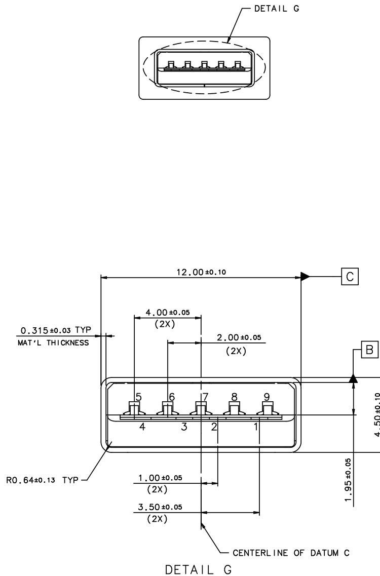
Figure 5-4. USB 3.1 Standard-A Plug Interface Dimensions
