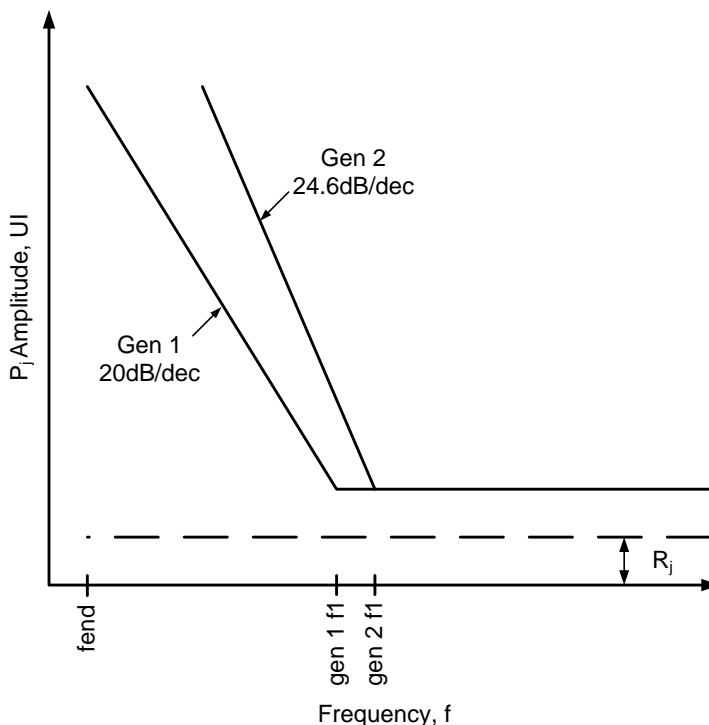
Figure 6-28. Jitter Tolerance Curve
