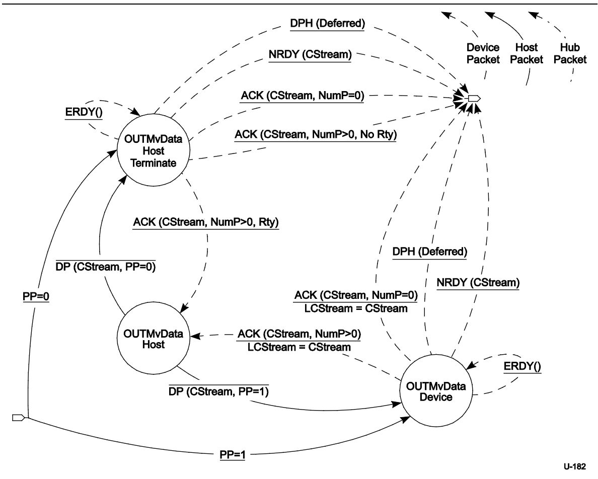
Figure 8-46. Host OUT Move Data State Machine (HOMDSM)
