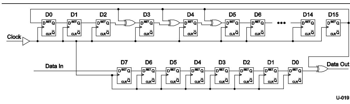
Figure 6-8. LFSR with Scrambling Polynomial
