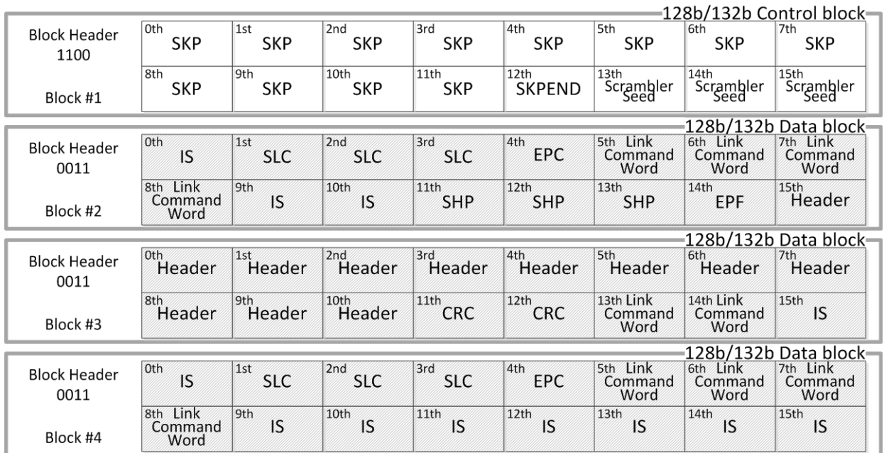
Figure D-3. Example placement of Gen 2 SKP Block, Idle Symbols, Link Command and Header Packet
