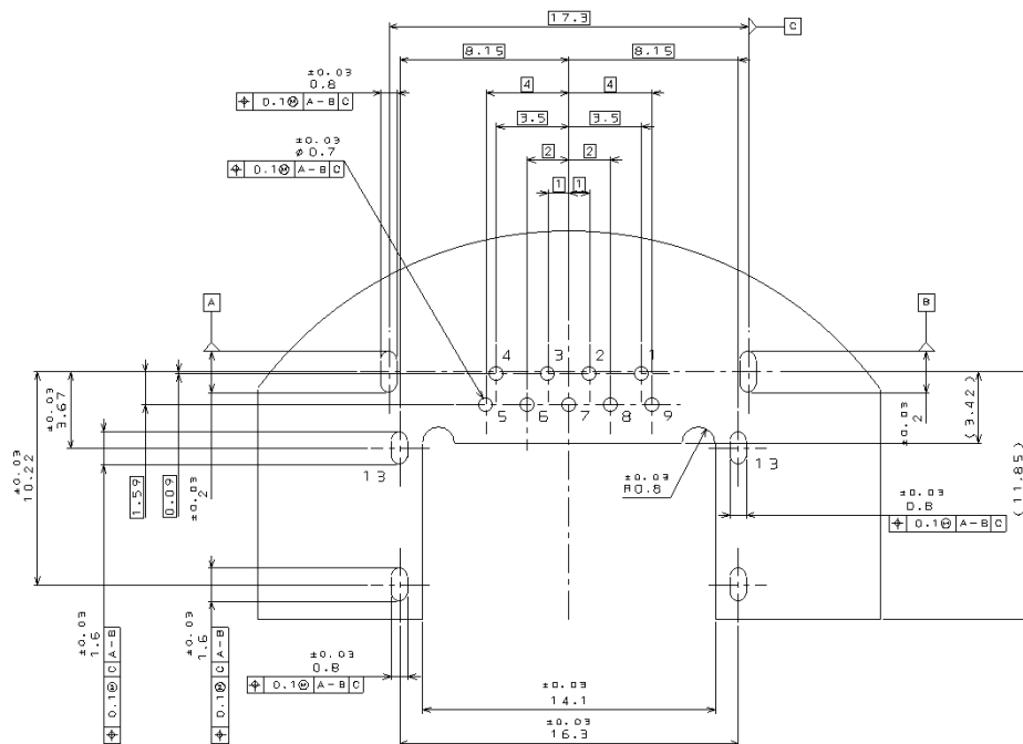
Figure 5-7. Example Footprint for the USB 3.1 Standard-A Receptacle - Mid-Mount Reverse Mount Through-Hole with Insertion Detect
