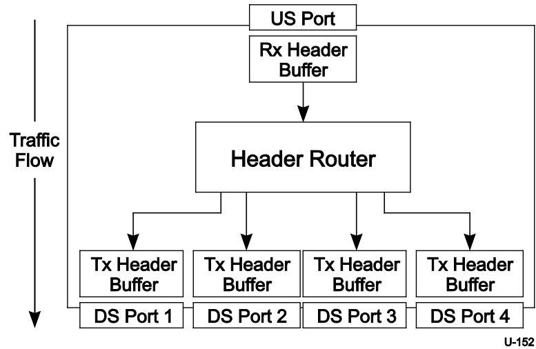
Figure 10-15. Example SS Hub Header Packet Buffer Architecture - Downstream Traffic
