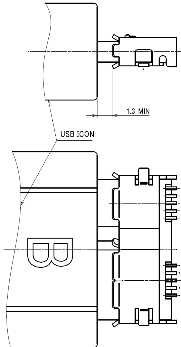
Figure 5-33. Mated USB 3.1 Micro-B Connector
