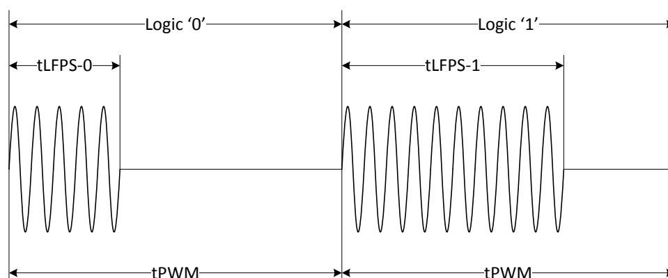
Figure 6-34. Logic Representation of LBPS
