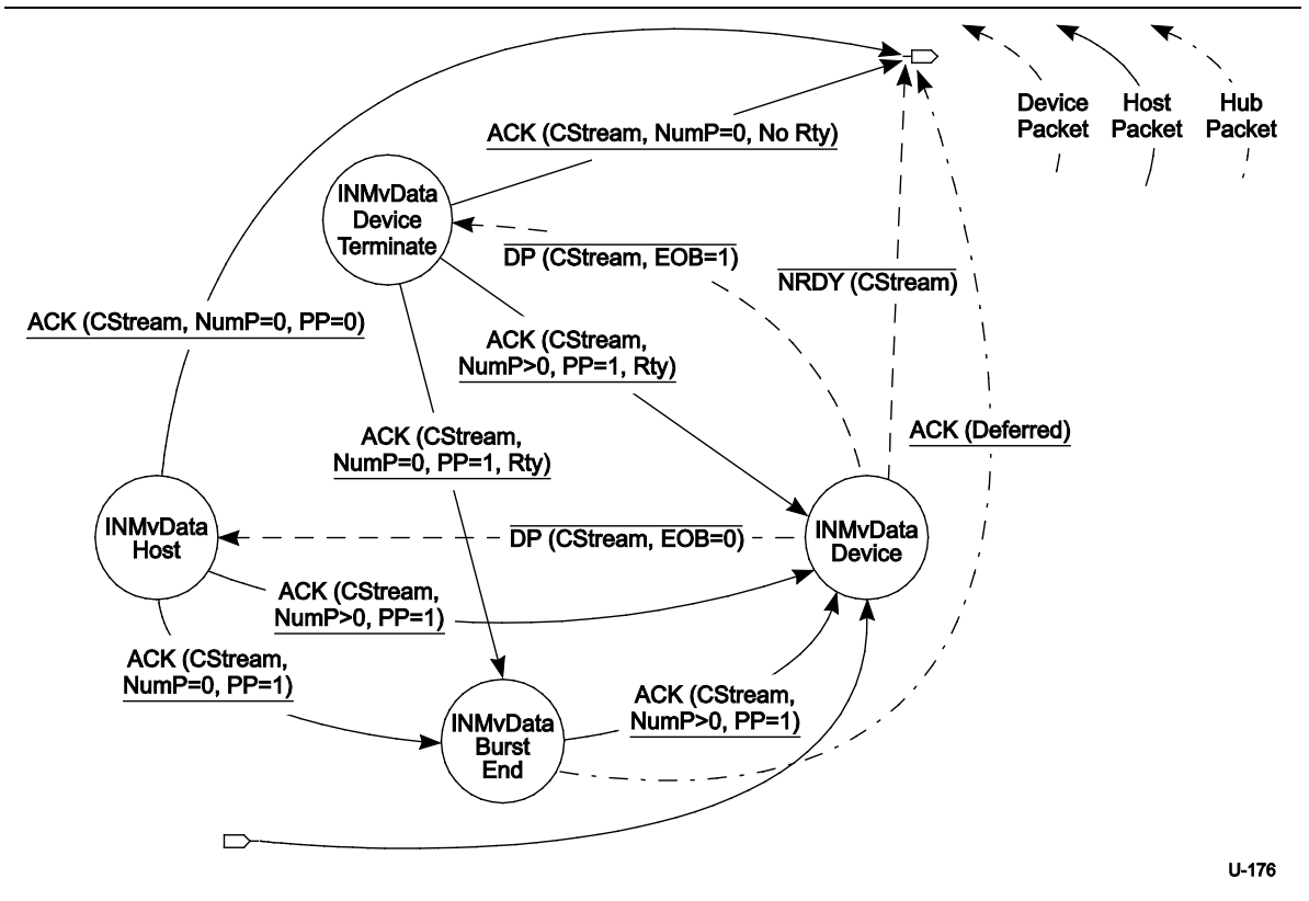
Figure 8-40. Device IN Move Data State Machine (DIMDSM)
