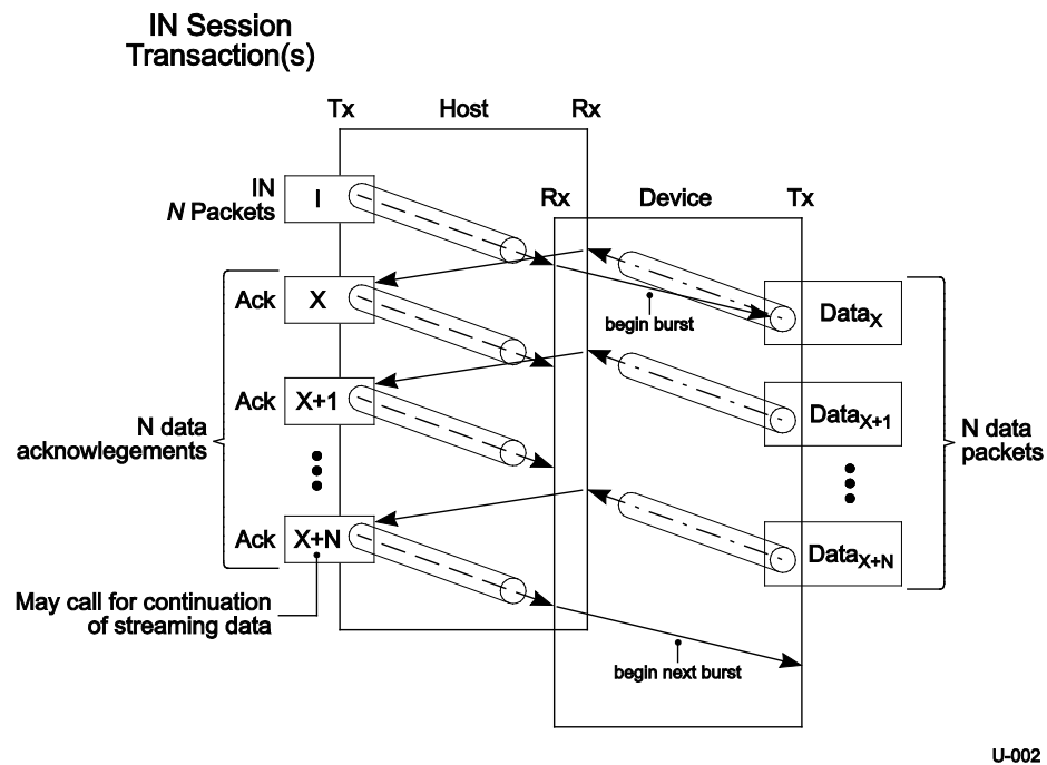
Figure 4-1. Enhanced SuperSpeed IN Transaction Protocol
