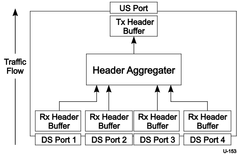
Figure 10-16. Example SS Hub Header Packet Buffer Architecture - Upstream Traffic
