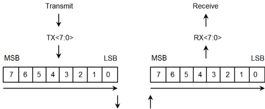
Figure 6-9. Gen 2 Serialization and Deserialization Order
