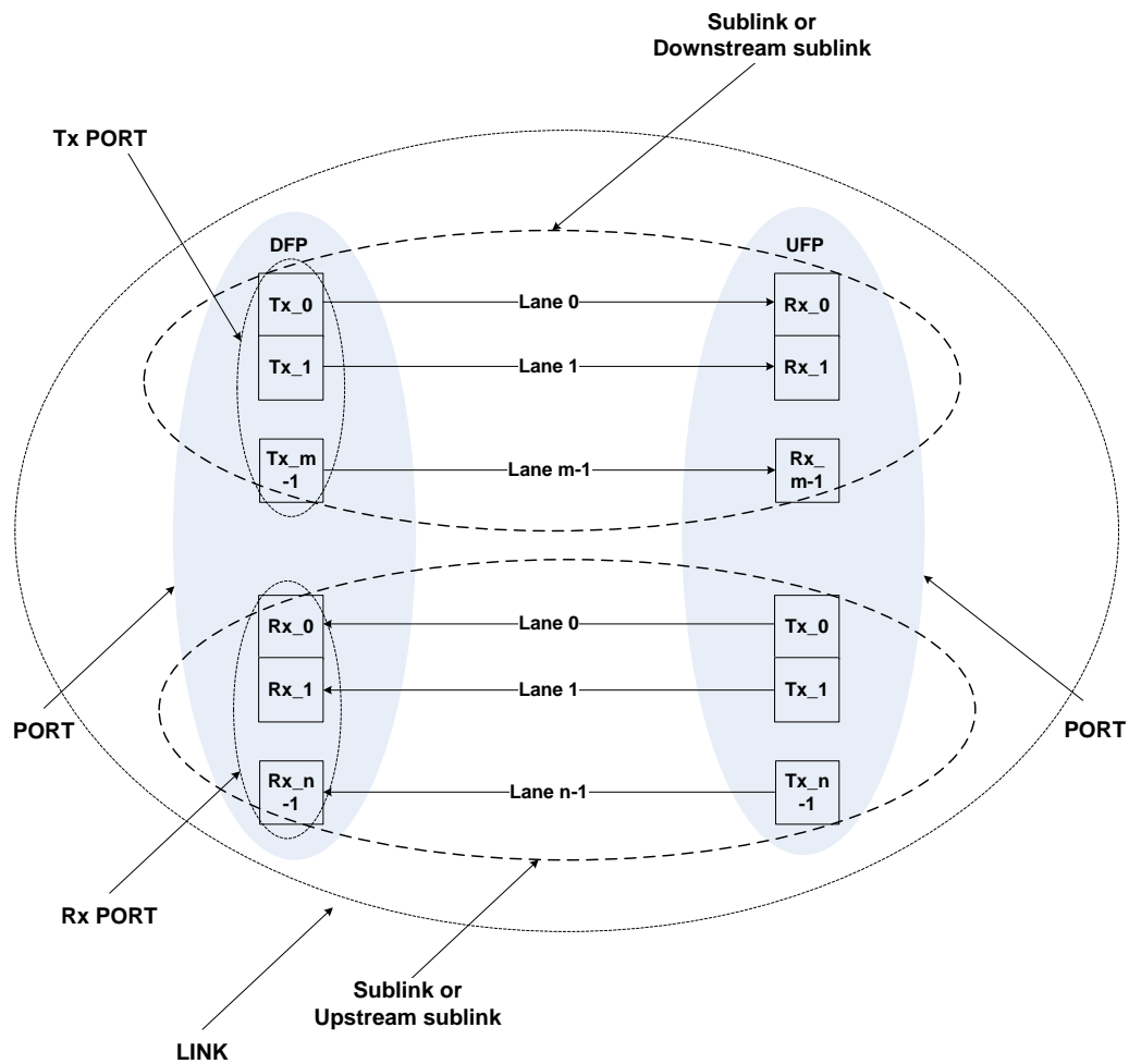
Figure 2-1. Port and Link Pictorial
