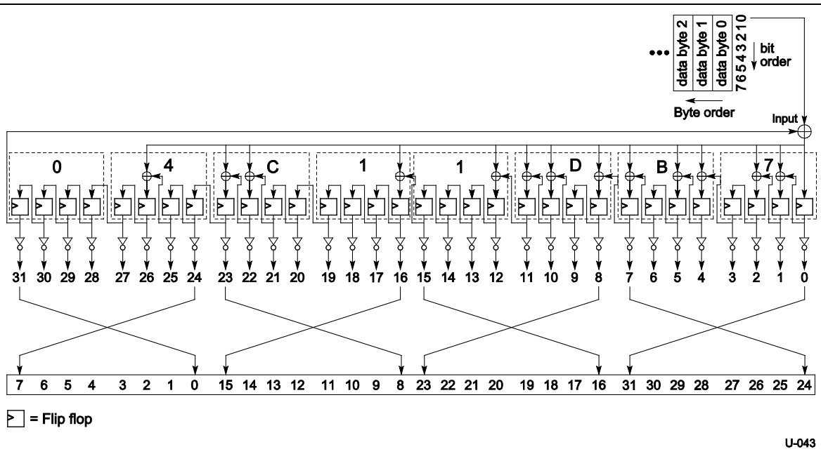
Figure 7-10. CRC-32 Remainder Generation
