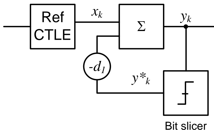
Figure 6-26. Gen 2 reference DFE Function
