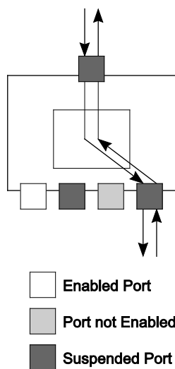
Figure 10-7. Resume Connectivity
