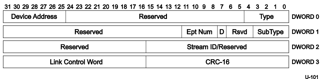
Figure 8-19. NRDY Transaction Packet
