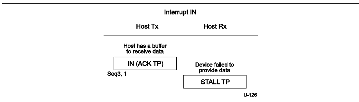
Figure 8-52. Endpoint Sends STALL TP
