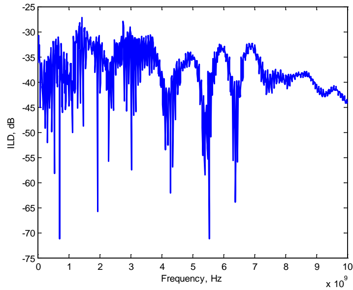
Figure 5-25. Example of Insertion Loss Deviation
