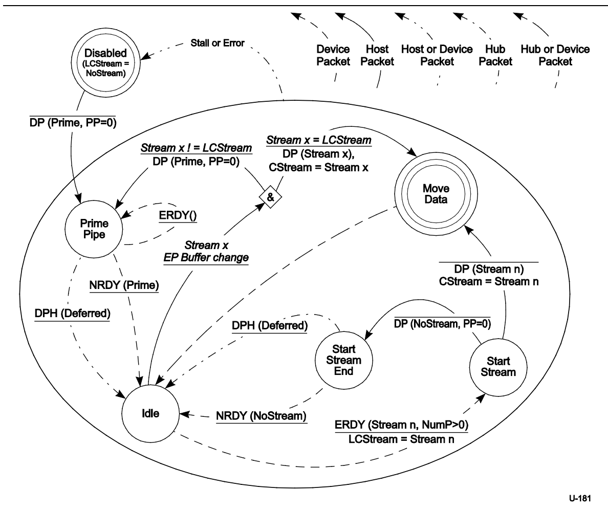
Figure 8-45. Host OUT Stream Protocol State Machine (HOSPSM)
