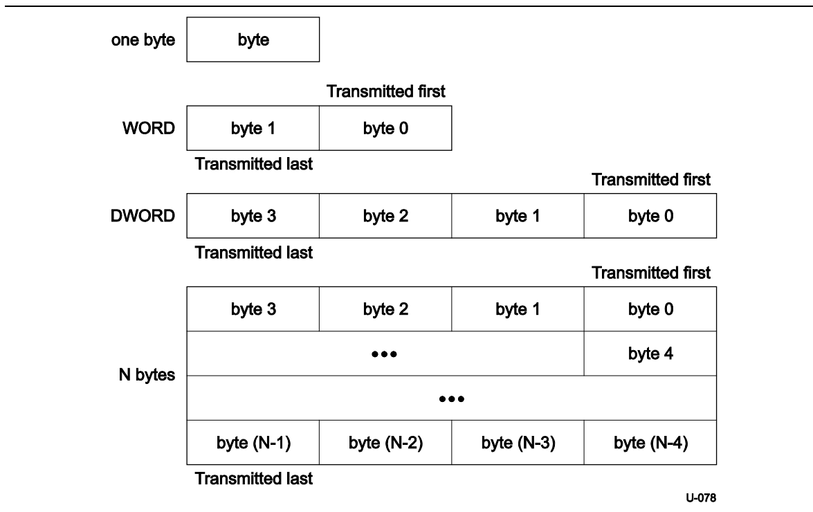
Figure 7-2. Byte Ordering
