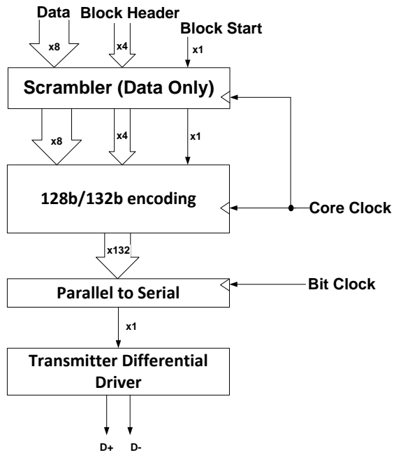
Gen 2 transmitter
