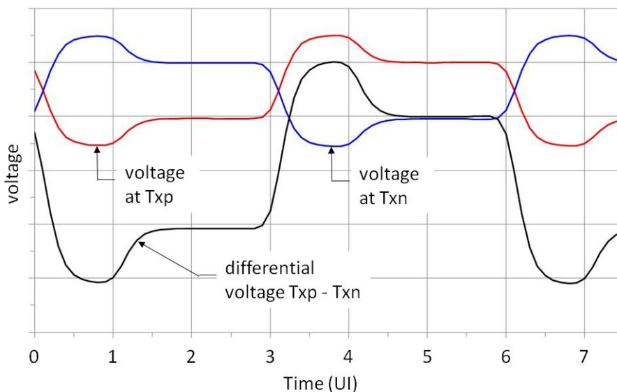
Figure 6-17. Single-ended and Differential Voltage Levels
