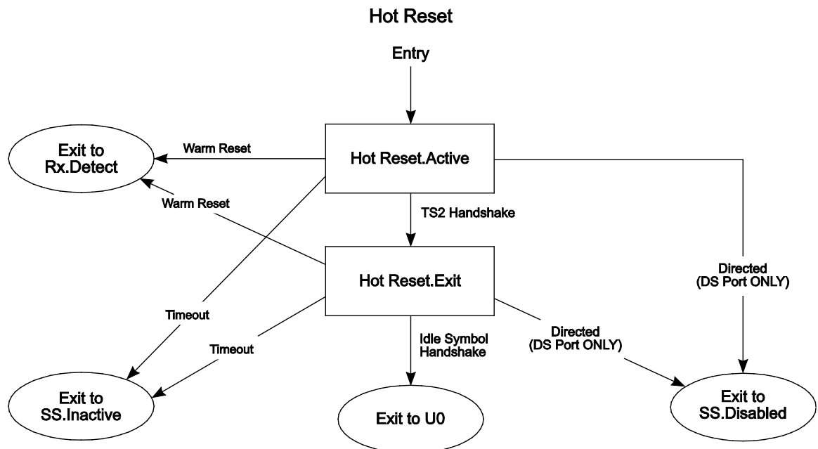
Figure 7-24. Hot Reset Substate Machine
