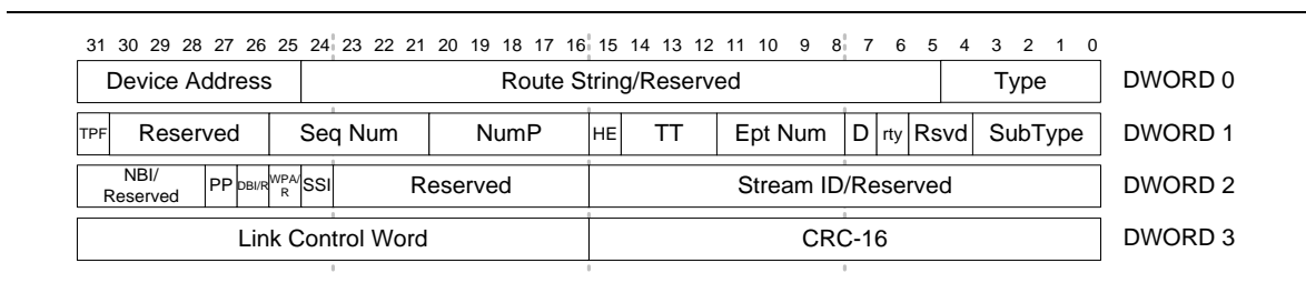
Figure 8-2. Example Transaction Packet
