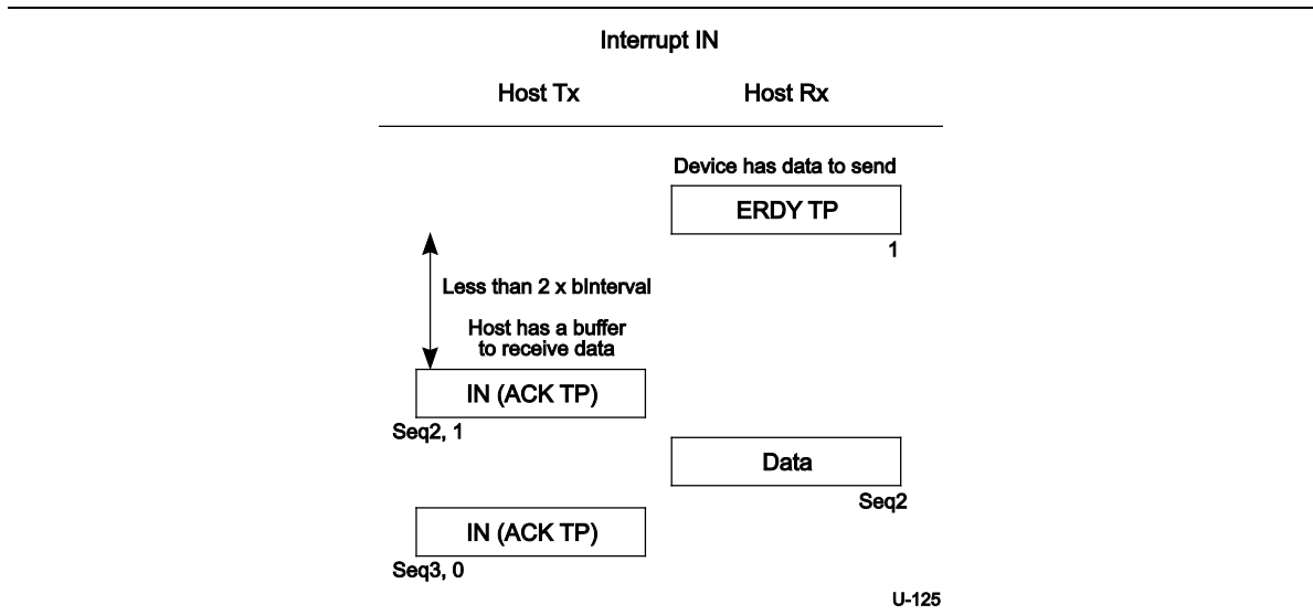
Figure 8-51. Host Resumes IN Transaction after Device Sent ERDY
