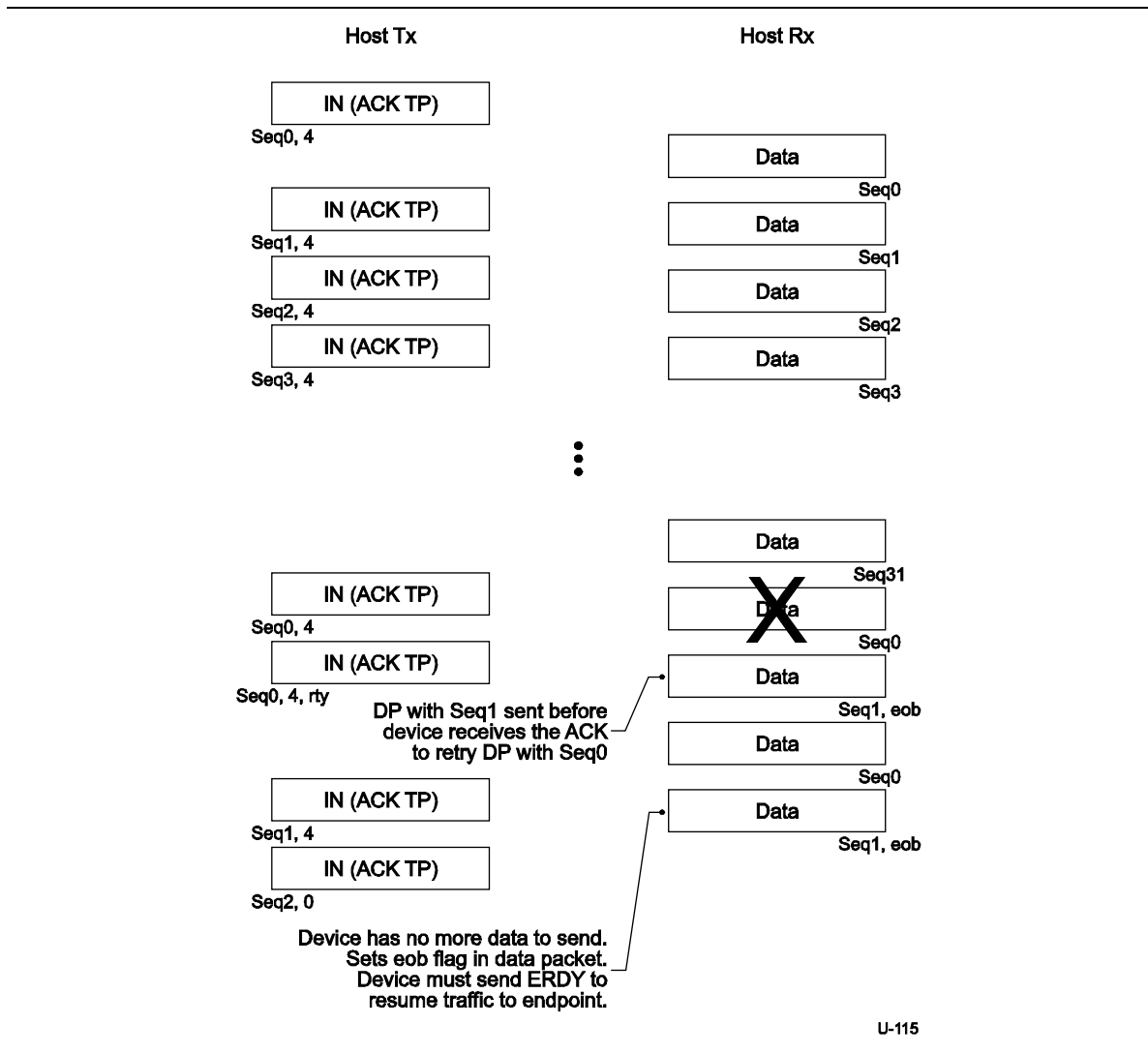
Figure 8-36. Sample BULK IN Sequence
