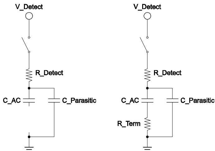
Figure 6-36. Rx Detect Schematic
