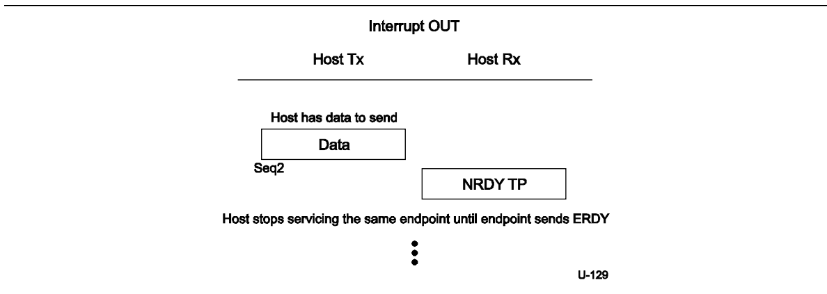
Figure 8-55. Host Stops Servicing Interrupt OUT Transaction Once NRDY is Received
