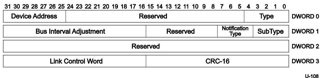
Figure 8-26. Bus Interval Adjustment Message Device Notification
