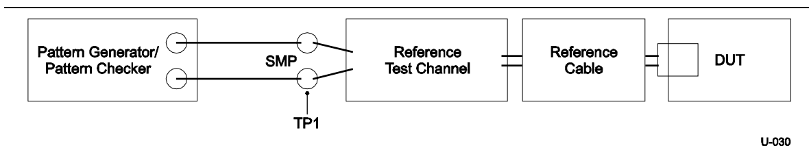
Figure 6-27. Rx Tolerance Setup
