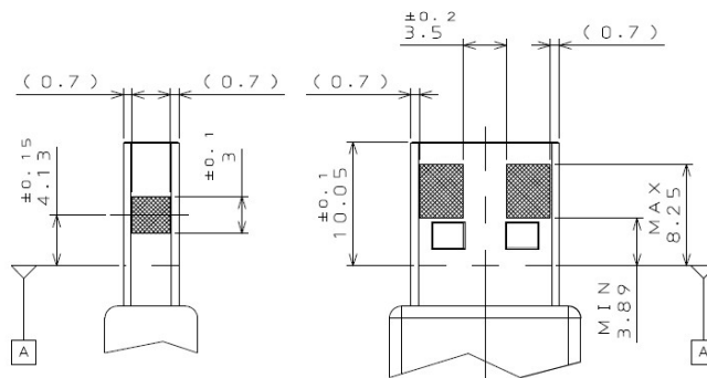
Figure 5-2. Example USB 3.1 Standard-A Receptacle with Grounding Springs and Required contact zones on the Standard-A Plug.
