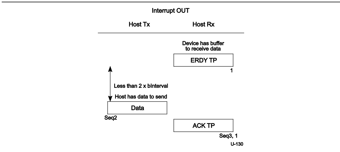
Figure 8-56. Host Resumes Sending Interrupt OUT Transaction After Device Sent ERDY
