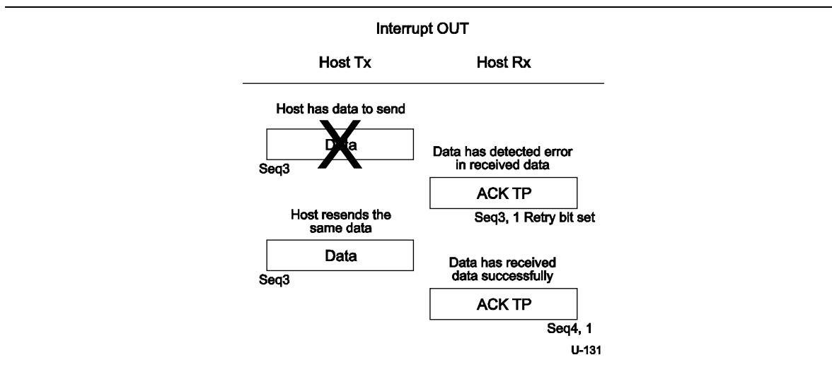
Figure 8-57. Device Detects Error in Data and Host Resends Data
