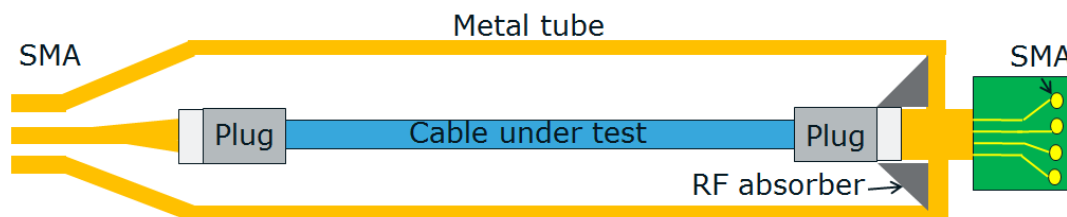
Figure 5-29. Set Up For Cable SE Measurement (subject to change)
