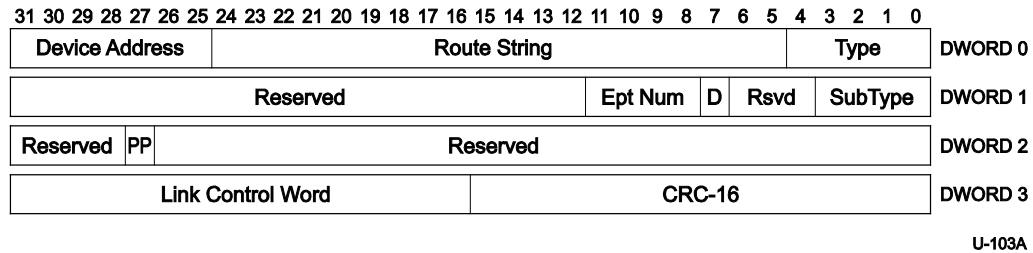
Figure 8-21. STATUS Transaction Packet
