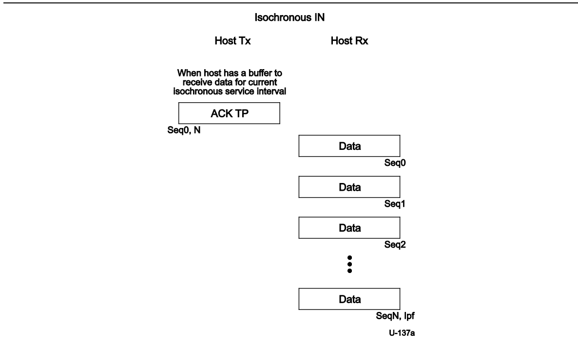
Figure 8-60. Enhanced SuperSpeed Isochronous IN Transaction Format
