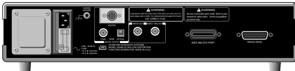
Figure 2-7 Rear Panel
