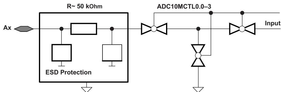
Figure 27-2. Analog Multiplexer
