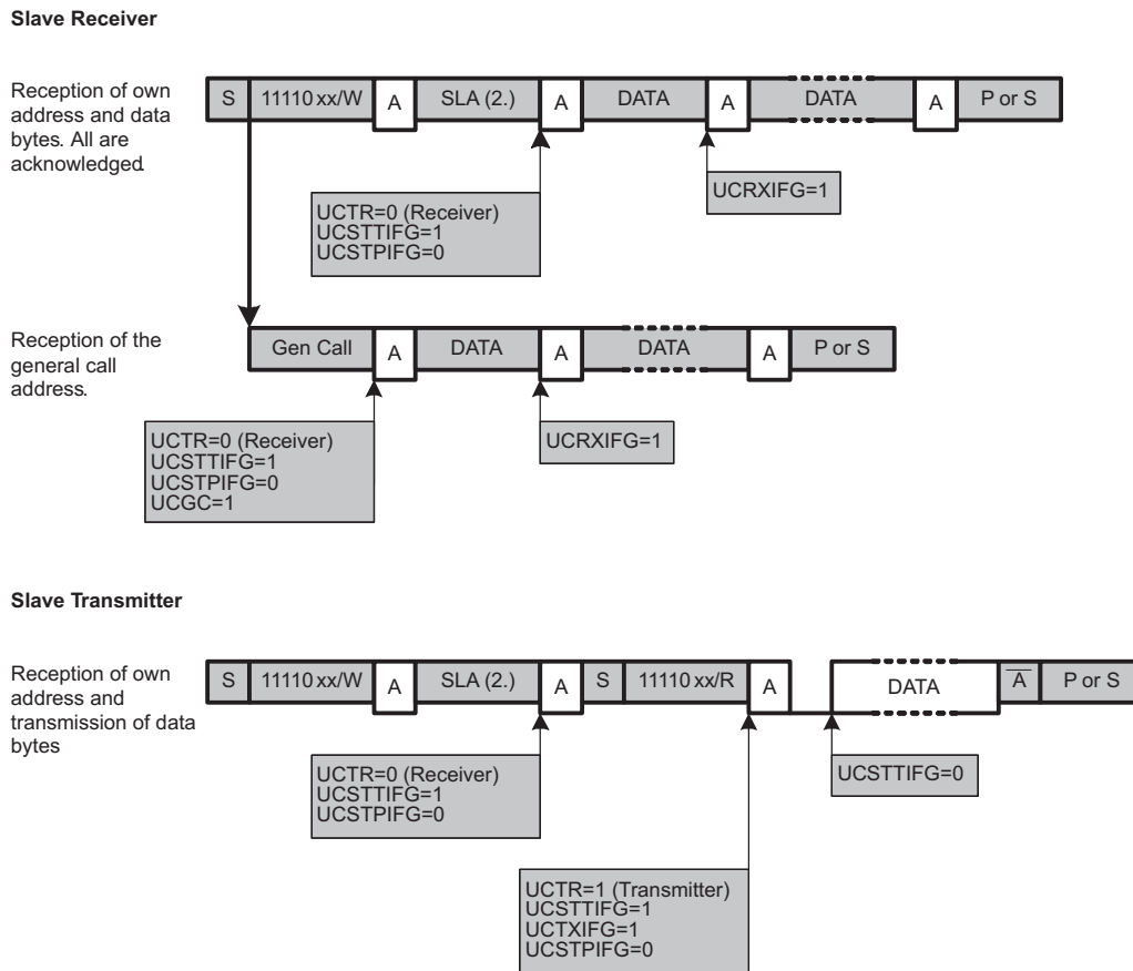
Figure 36-11. I 2 C Slave 10-Bit Addressing Mode
