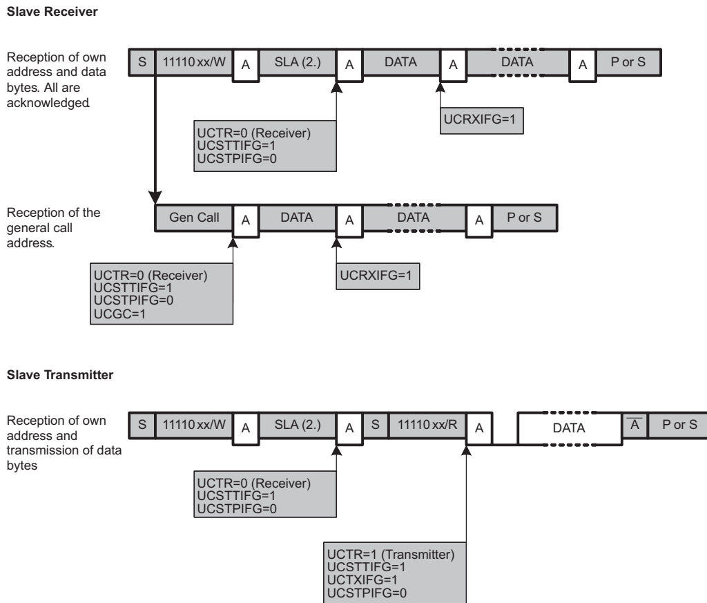
Figure 39-11. I 2 C Slave 10-Bit Addressing Mode
