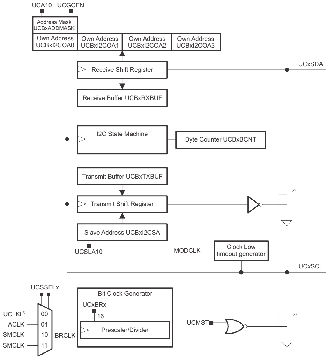
Figure 39-1. eUSCI_B Block Diagram – I 2 C Mode
