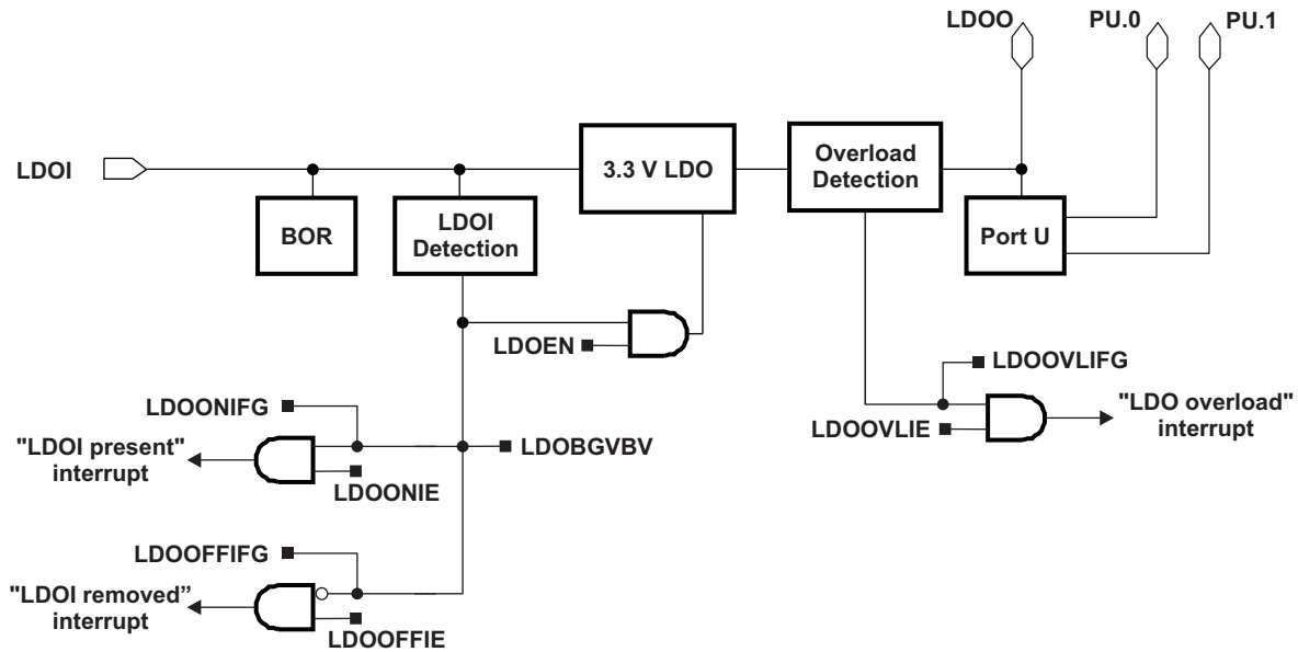
Figure 41-1. LDO Block Diagram
