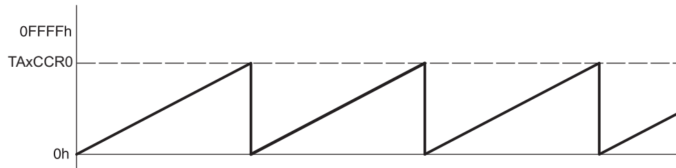
Figure 17-2. Up Mode
