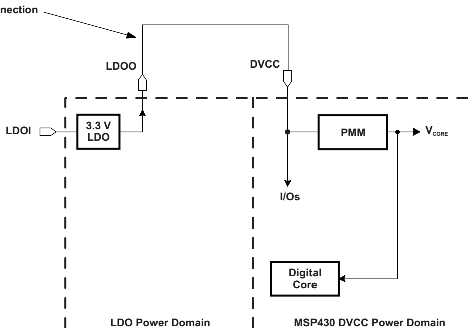
Figure 41-3. Powering Entire MSP430 From LDOI
