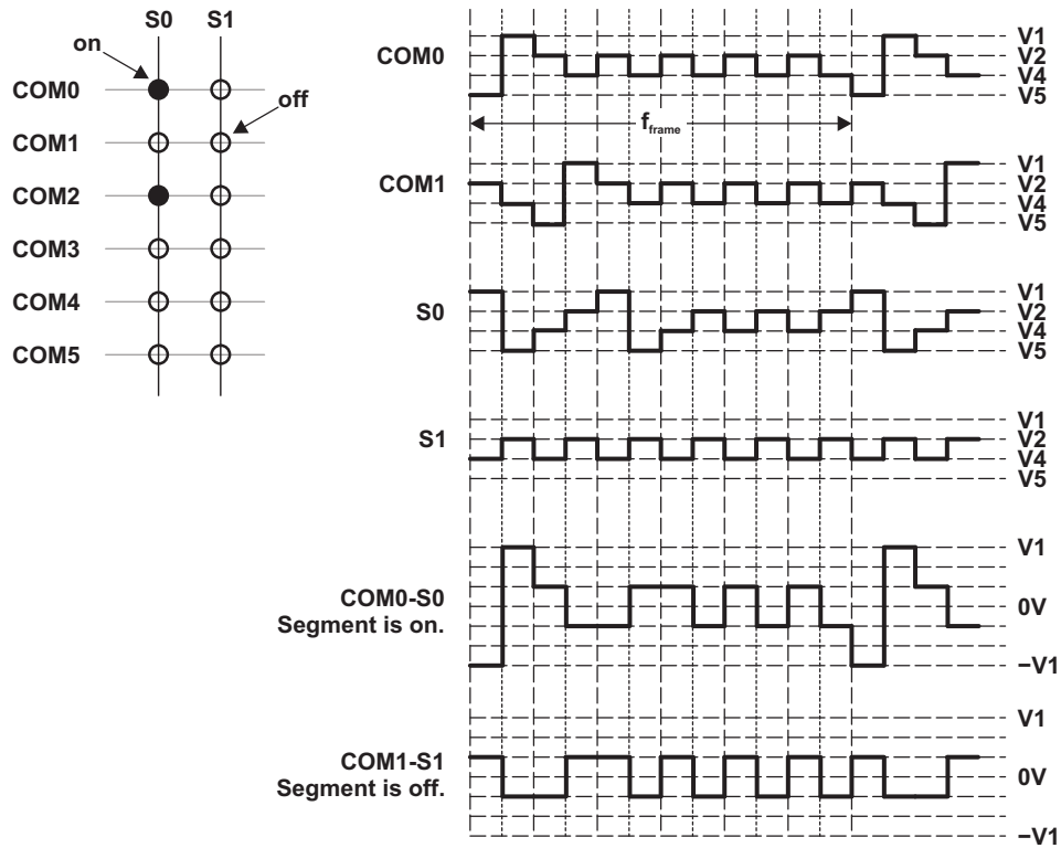
Figure 33-9. Example 6-Mux Waveforms
