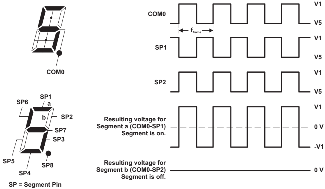
Figure 32-4. Example Static Waveforms
