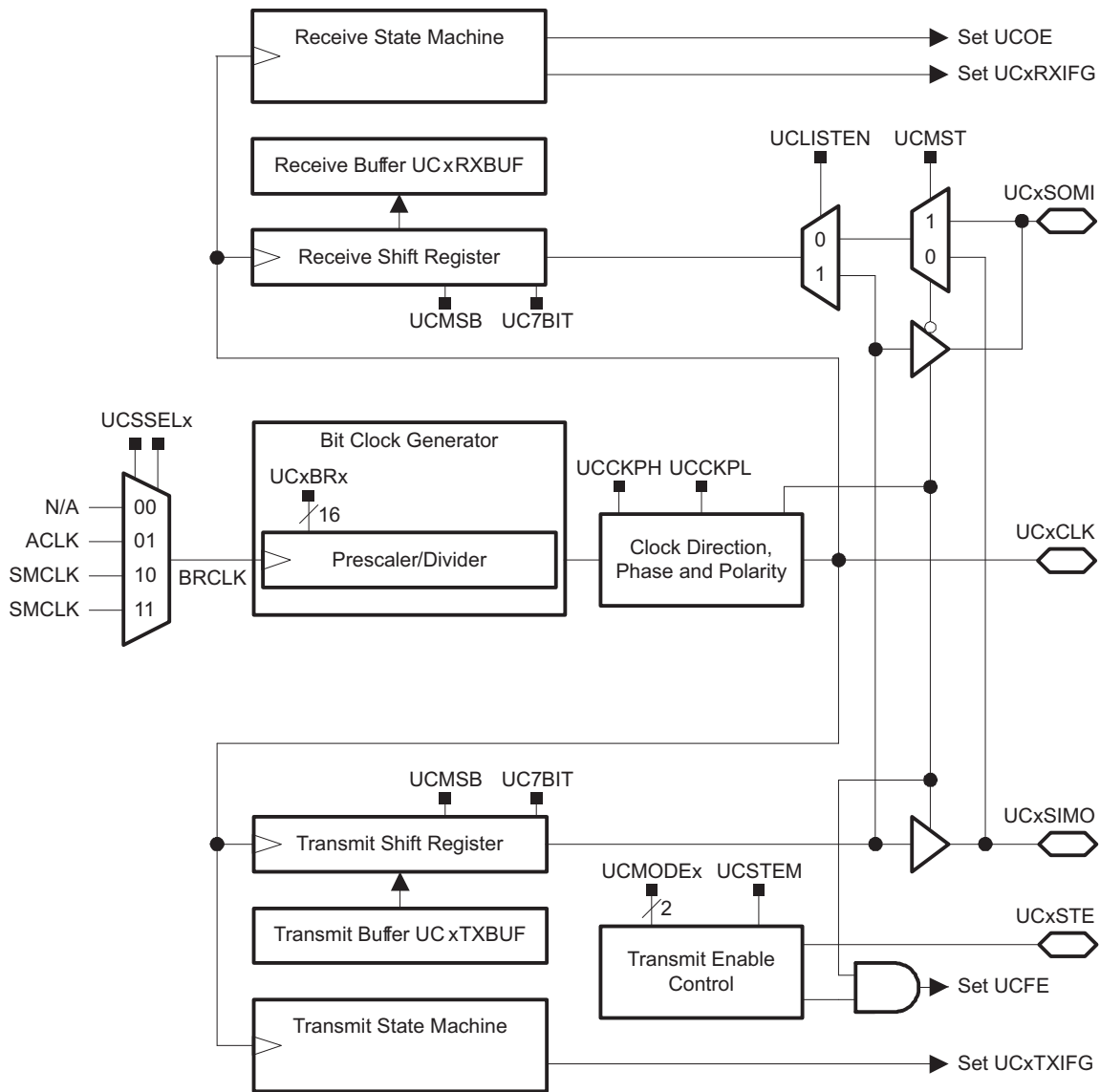
Figure 38-1. eUSCI Block Diagram – SPI Mode
