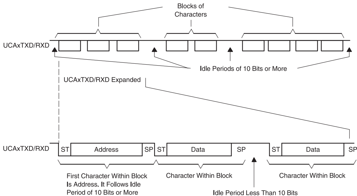
Figure 34-3. Idle-Line Format
