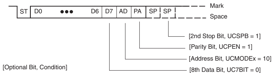
Figure 37-2. Character Format
