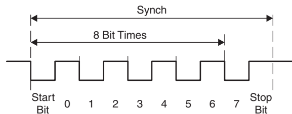
Figure 37-6. Auto Baud-Rate Detection – Synch Field
