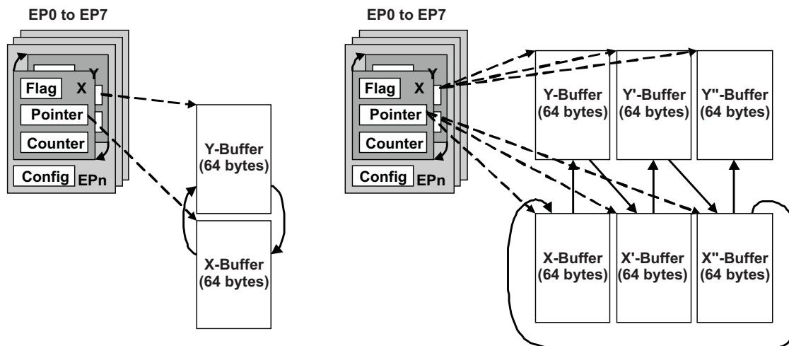
Figure 40-6. Data Buffers and Descriptors
