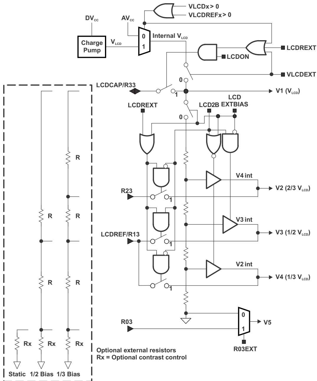
Figure 32-3. Bias Generation
