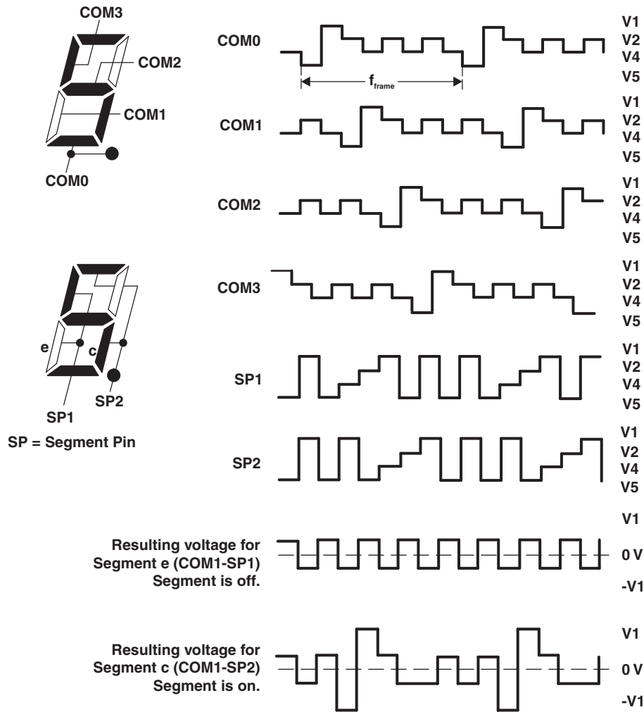
Figure 32-10. Example 4-Mux Waveforms
