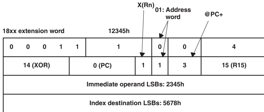
Figure 6-28. Example for Extended Immediate or Indexed Instruction
