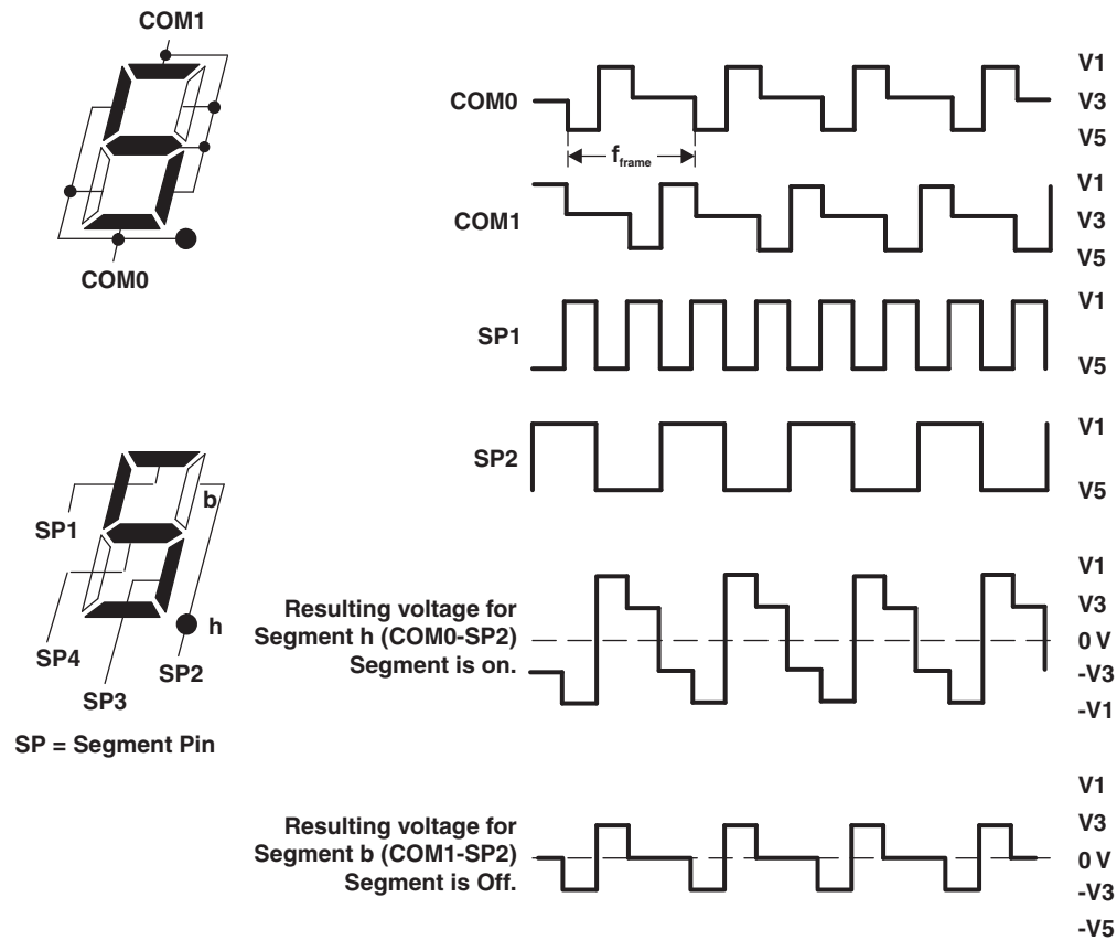
Figure 32-6. Example 2-Mux Waveforms
