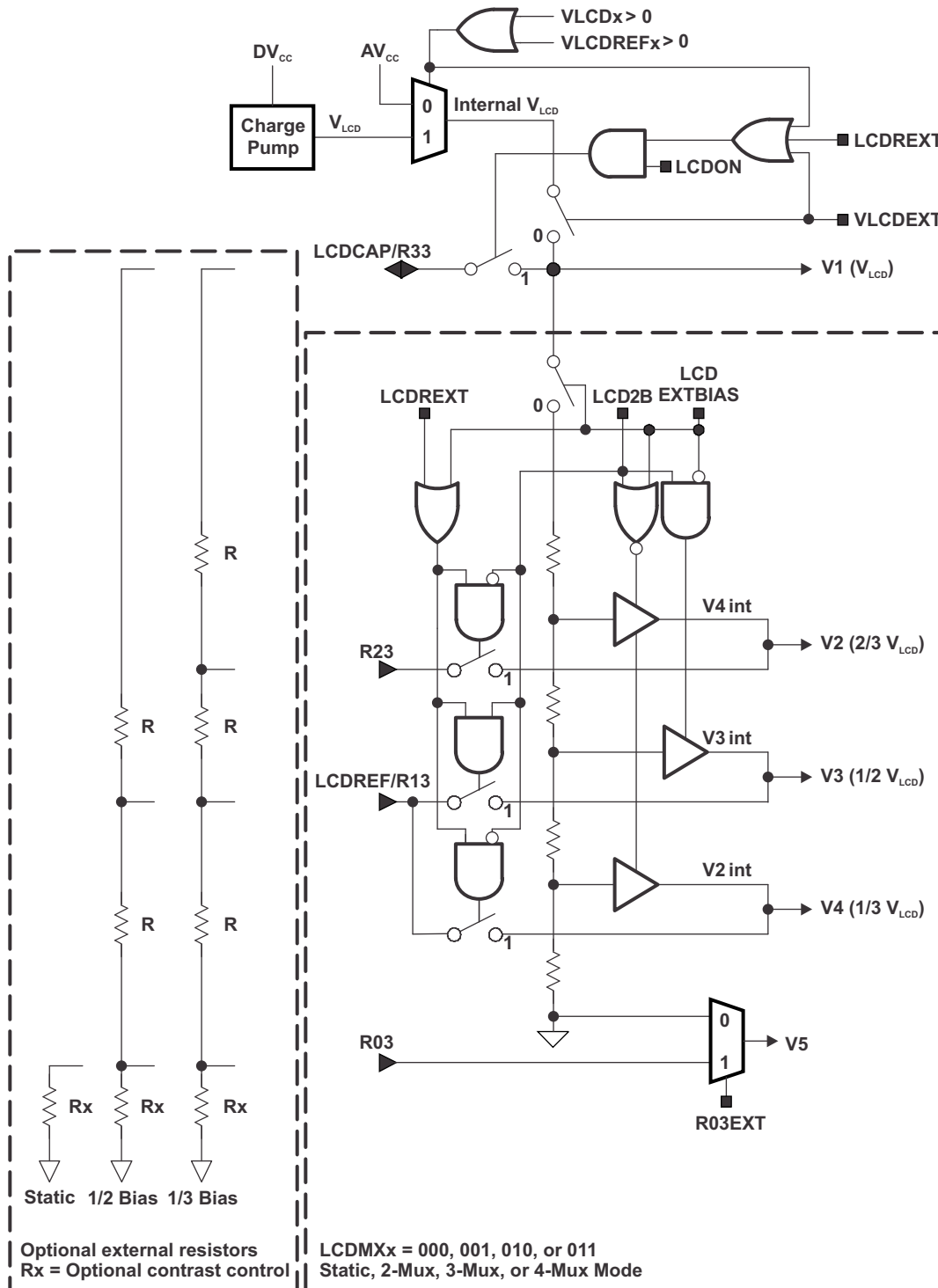
Figure 33-4. Bias Generation
