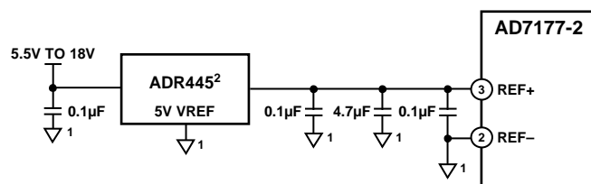
1 ALL DECOUPLING IS TO AVSS. 2 ANY OF THE ADR440/ADR441/ADR443/ADR444/ADR445 FAMILY OF REFERENCES CAN BE USED. THE ADR444 AND ADR441 BOTH ENABLE REUSE OF THE 5V ANALOG SUPPLY NEEDED FOR AVDD1 TO POWER THE REFERENCE VIN.
