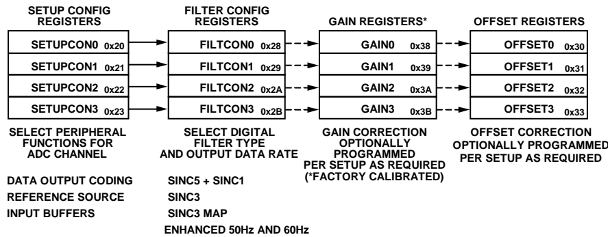
Figure 45. ADC Setup Register Grouping
