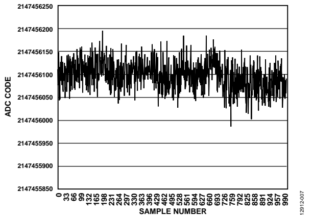
Figure 7. Noise (Analog Input Buffers Enabled, V REF = 5 V, Output Data Rate = 5 SPS)
