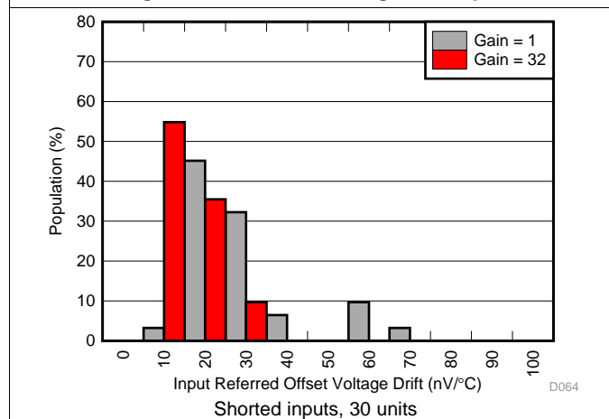
Figure 6. ADC1 Offset Voltage vs Temperature Distribution
