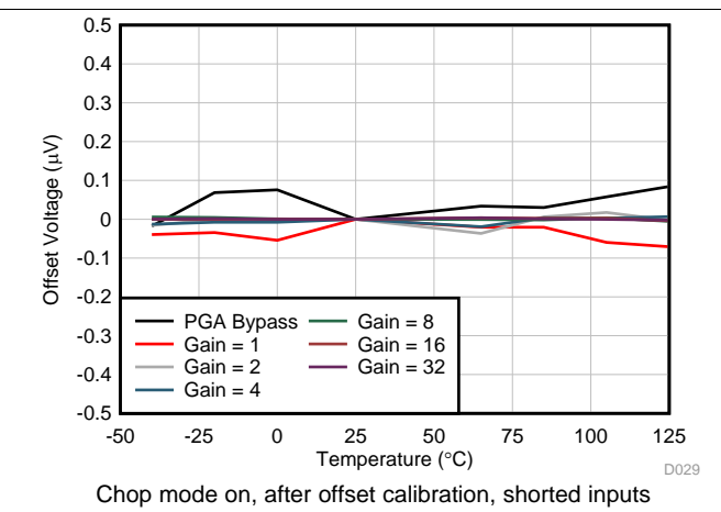
Figure 5. ADC1 Offset Voltage vs Temperature
