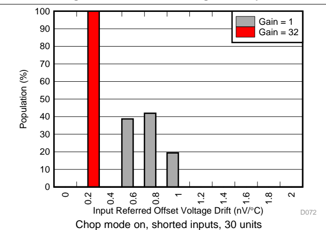
Figure 7. ADC1 Offset Voltage vs Temperature Distribution
