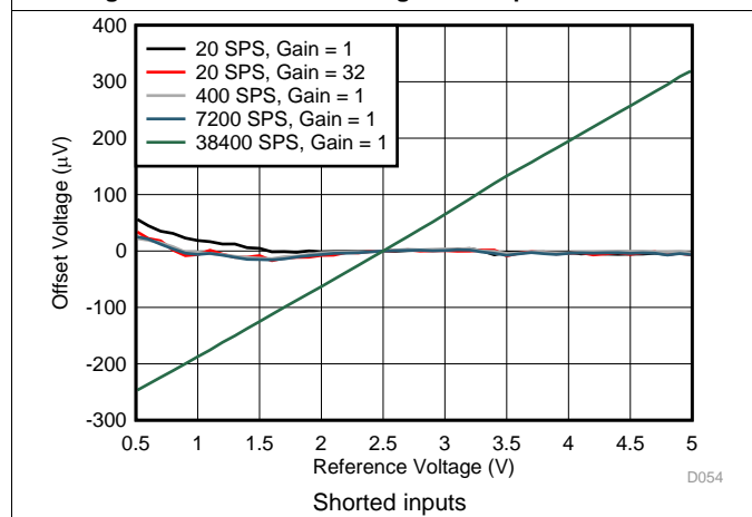
Figure 8. ADC1 Offset Voltage vs Reference Voltage
