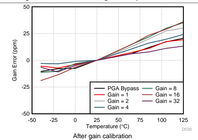
Figure 9. ADC1 Gain Error vs Temperature
