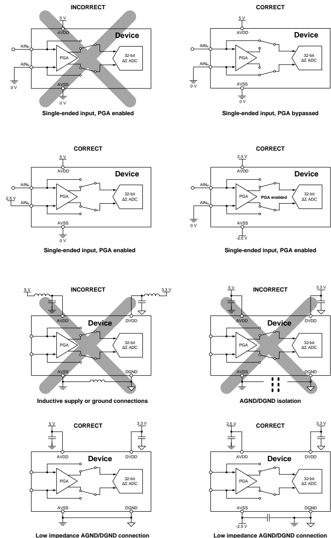
Figure 158. Dos and Don'ts Circuit Connections
