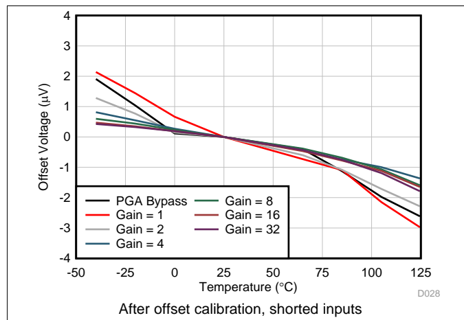
Figure 4. ADC1 Offset Voltage vs Temperature
