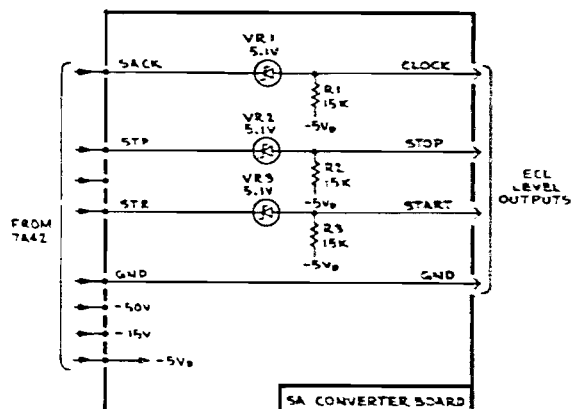
7A42 SIGNATURE ANALYSIS TTL TO ECL LEVEL CONVERTER
