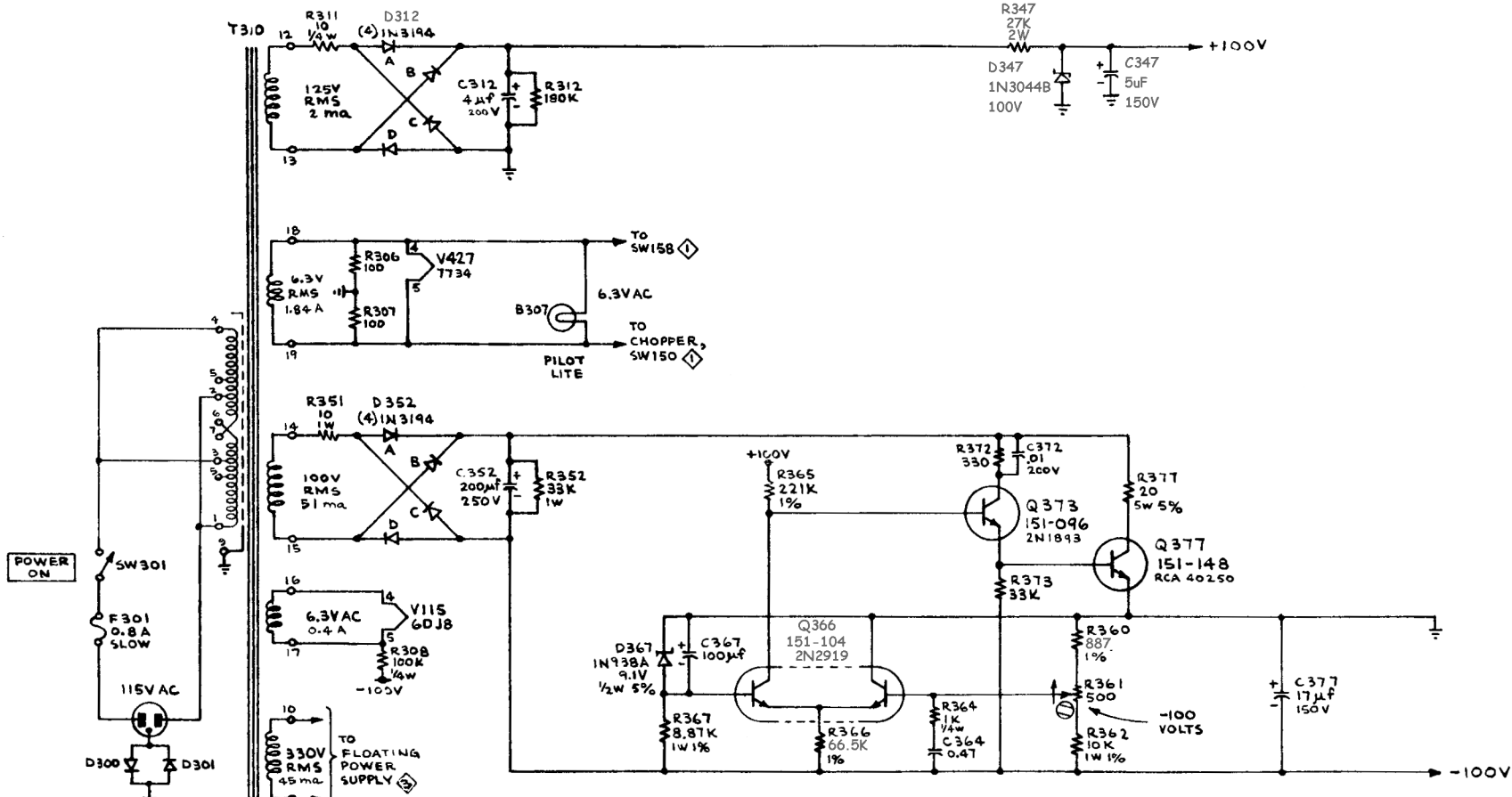
POWER SUPPLY 2
