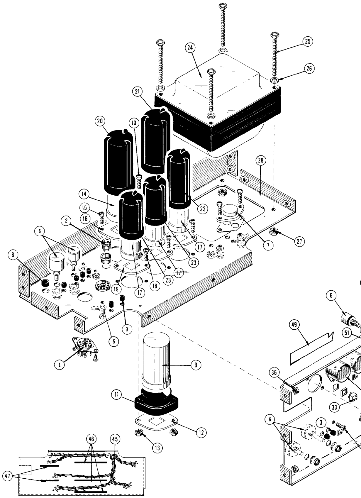
FIG. 2 CHASSIS
