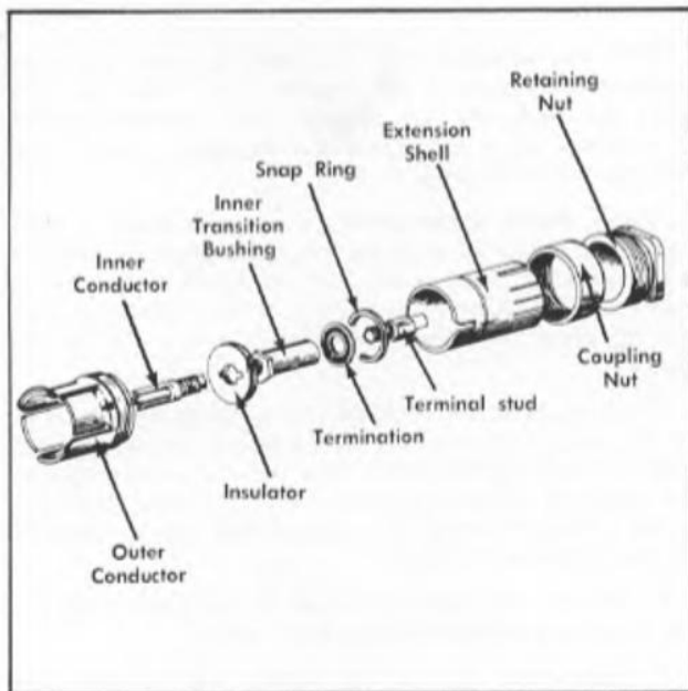
Fig. 4-4. Exploded view of + and - Output connectors.
