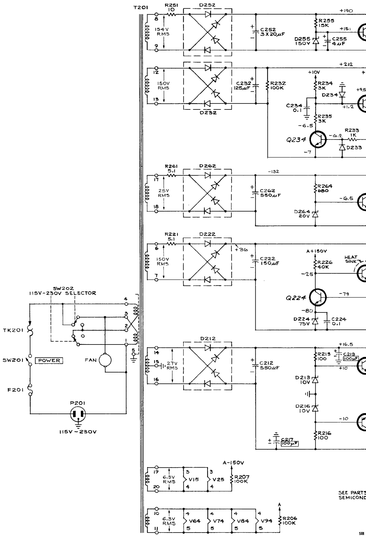
TYPE 106 SQUARE WAVE GENERATOR
