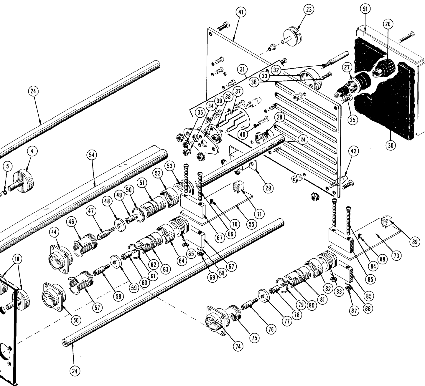
FIG. 1 FRONT
