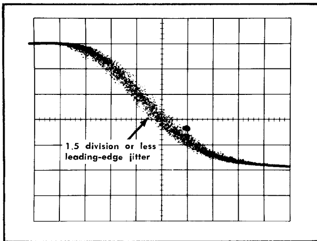
Fig. 5-6. Typical sampling system display of trigger jitter.
