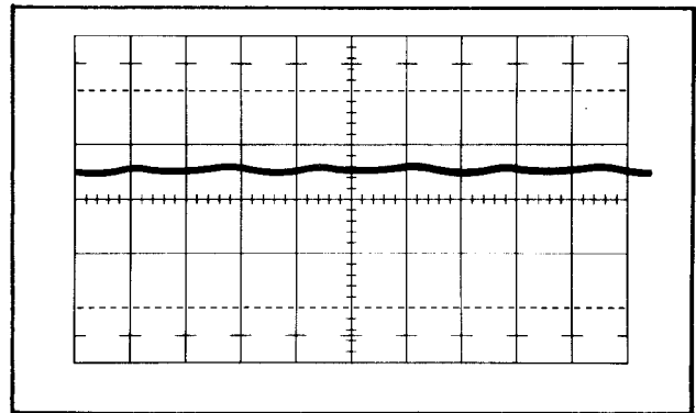
Fig. 6-7. Typical test oscilloscope display of power-supply ripple (60-cycle line). Sweep rate, 5 milliseconds/division; vertical deflection, 0.2 volt/division (0.02 volt/division and 10X probe).
