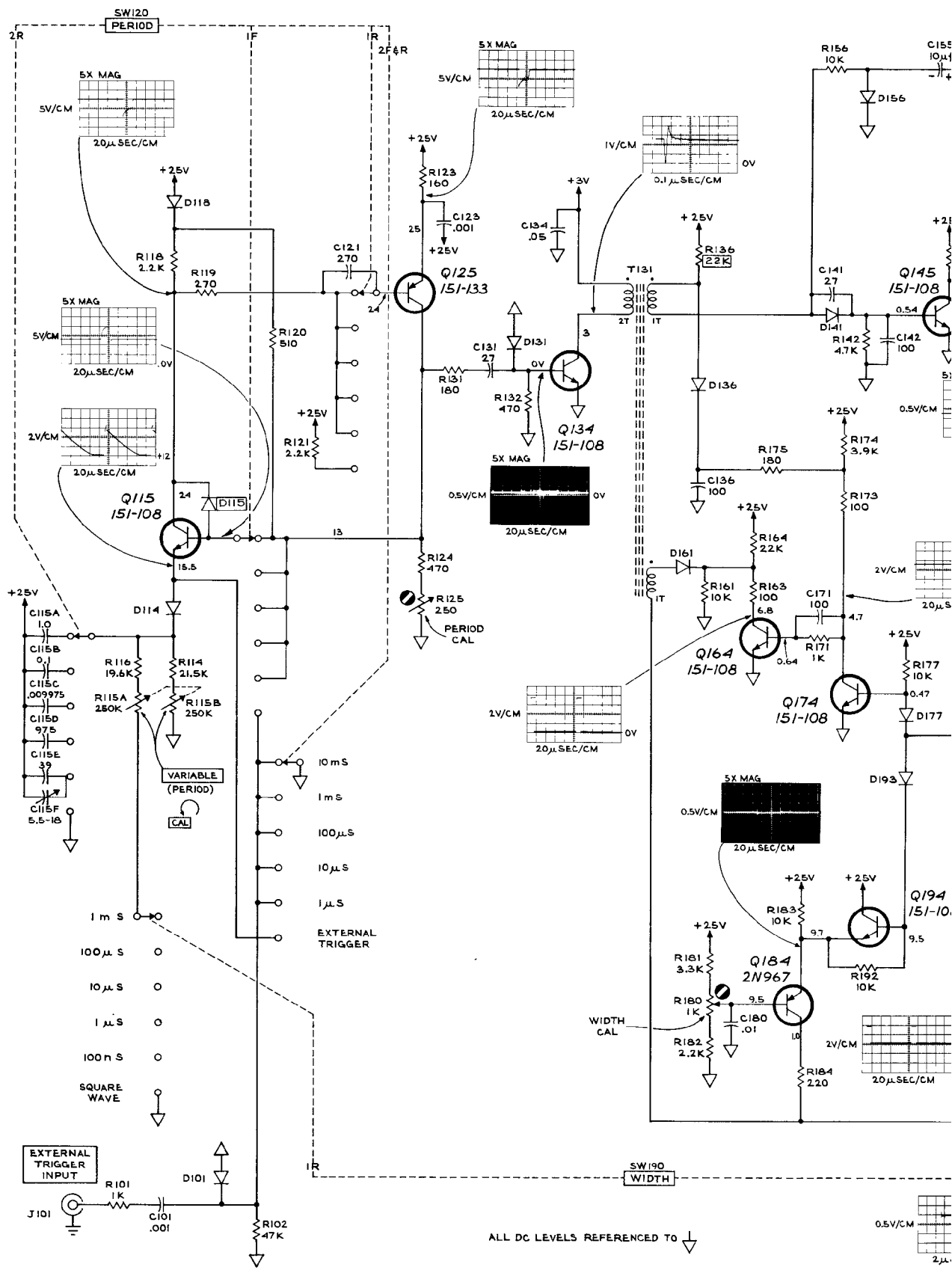
TYPE 114 PULSE GENERATOR
