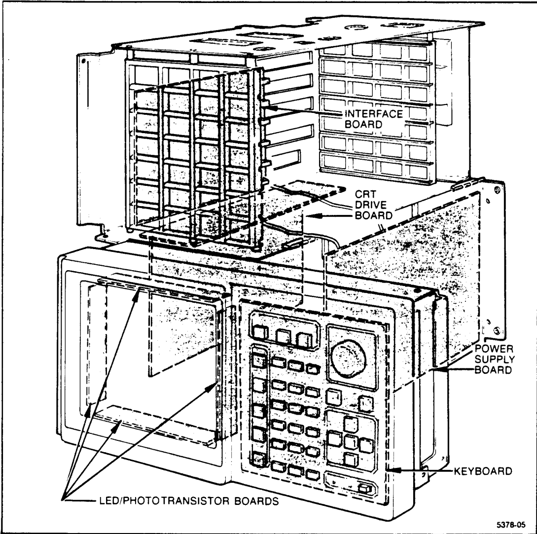
Figure 4-2. 1241 mainframe board locations.
