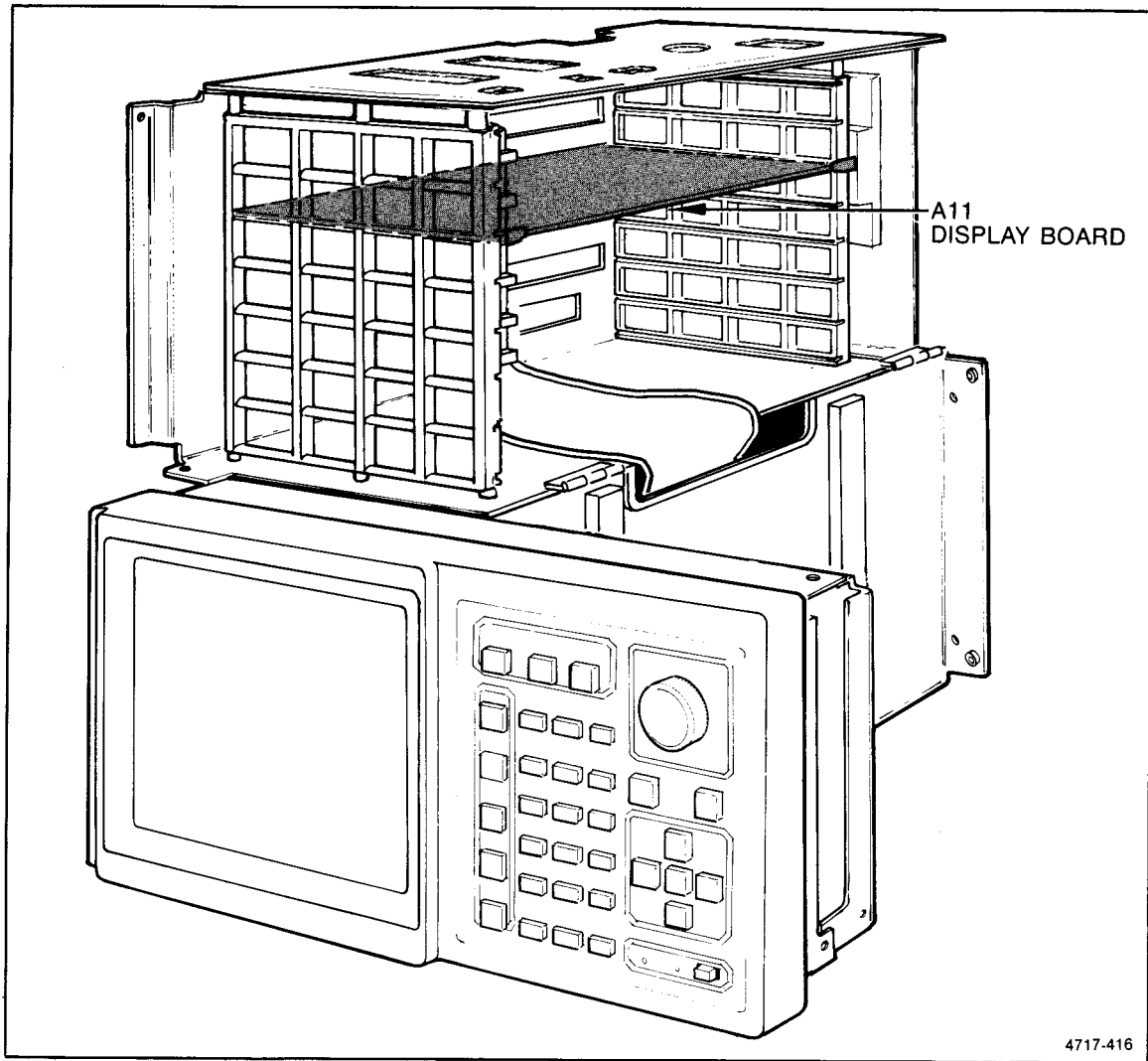
Figure 10-6. A12 1241 Display Board Mainframe Location.
