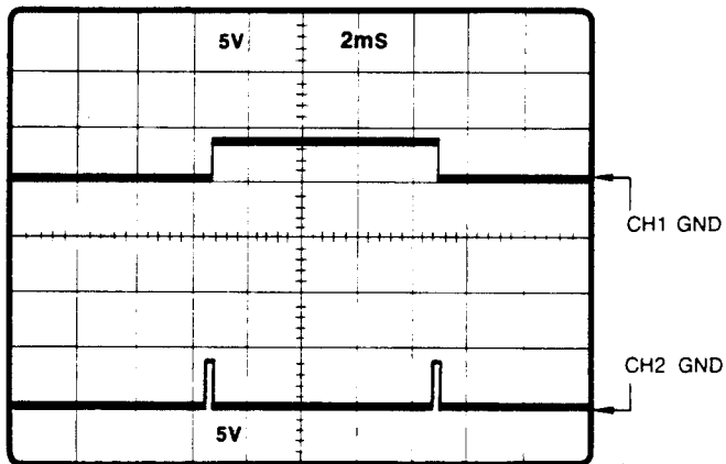
Figure 8-13. A13U138-11 VDRIVE-GREEN(H); A13U138-12 VDRIVE(H).
