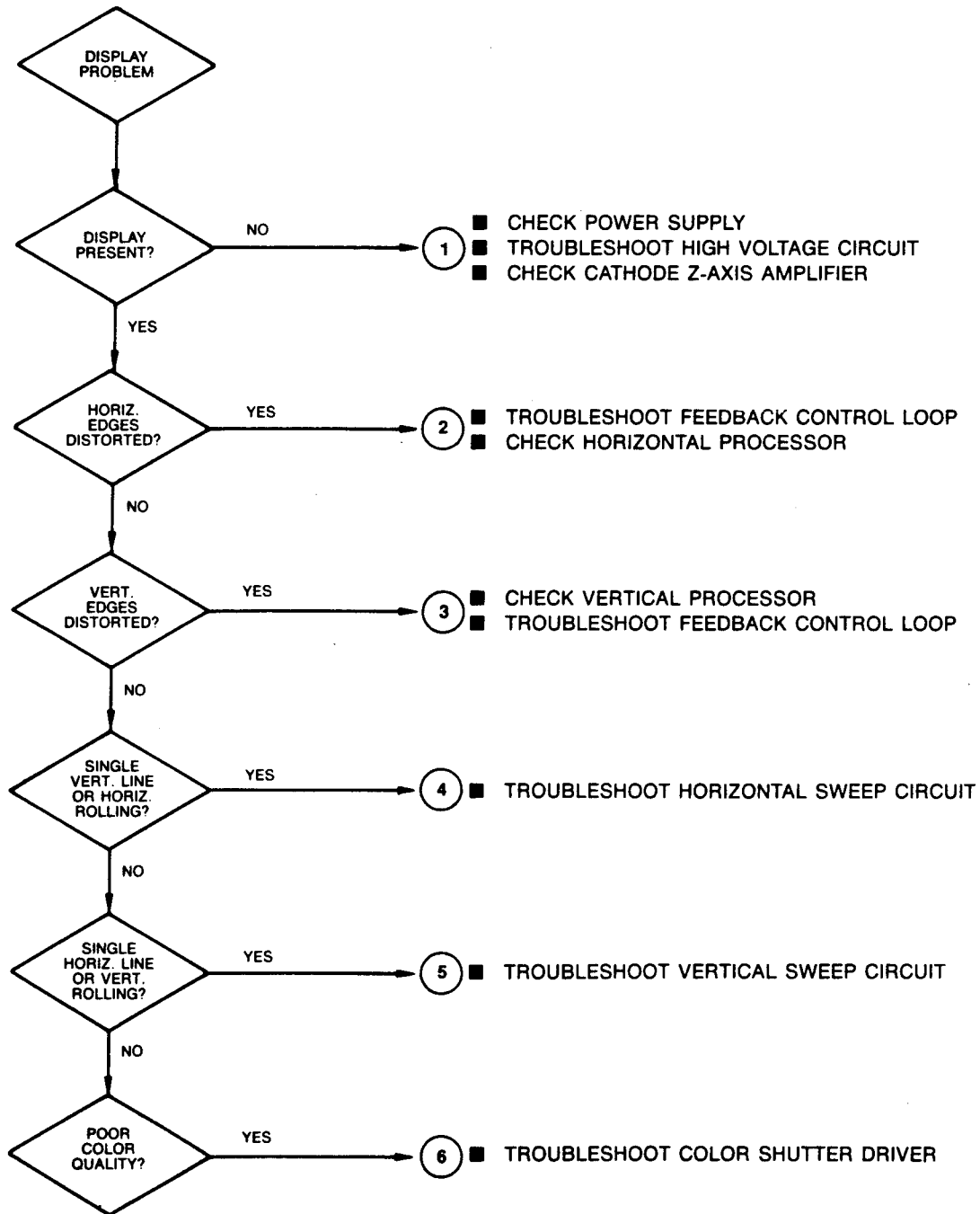
Figure 8-2. 1241 CRT Drive Board troubleshooting tree.
