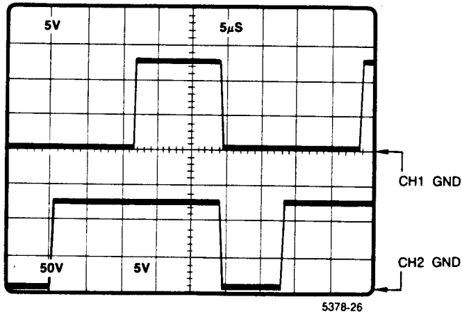
Figure 8-6. A13TP344 Q334 gate drive; A13TP340 Q534 gate drive.
