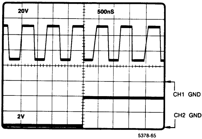
Figure 8-9. A13TP650 cathode Z-axis amplifier; A13TP225 HDRIVE(L).
