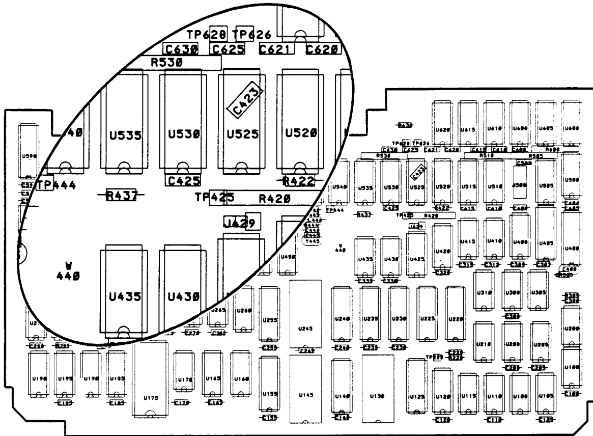
Figure 5-4. Expanded view of the Display Board shows components used in the Counter/Timer Adjust.
