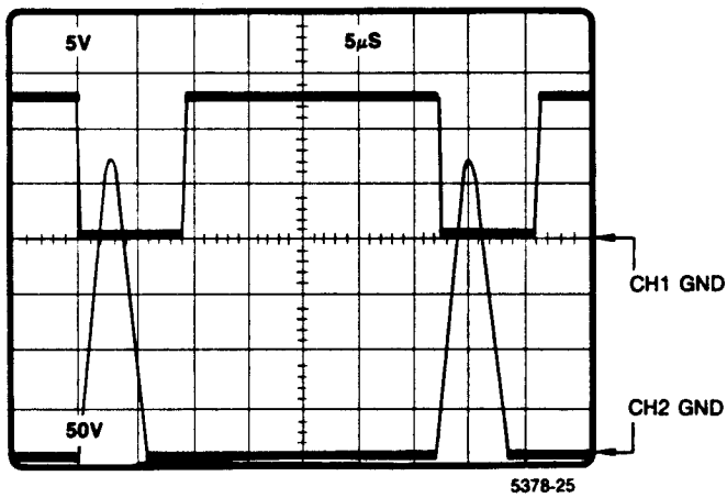
Figure 8-5. A13TP340 Q534 gate drive; A13TP534 transformer flyback.
