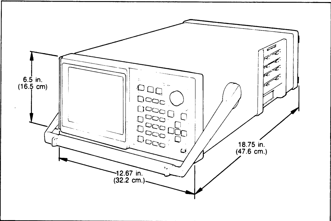
Figure 2-3. 1241 dimensions.
