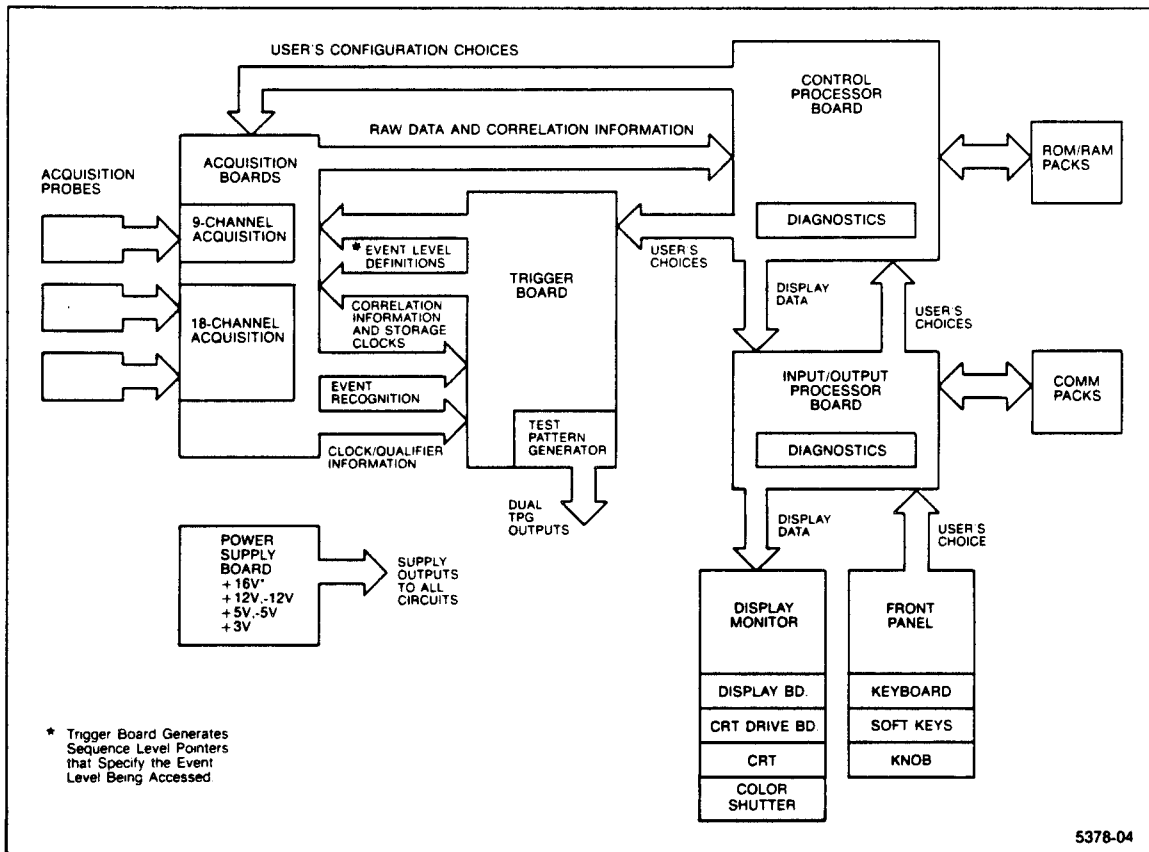
Figure 4-1. 1241 system block diagram.
