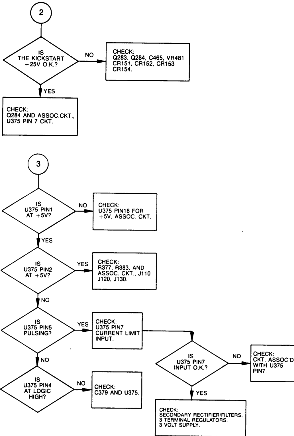
Figure 8-1. 1241 power supply troubleshooting tree (cont.).
