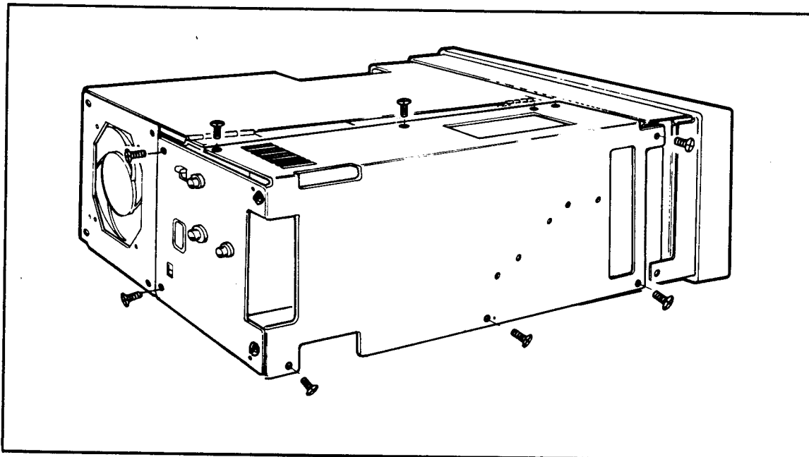
Figure 6-1. Location of screws for CRT Drive Board bracket removal.
