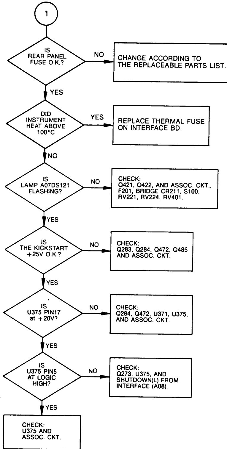
Figure 8-1. 1241 power supply troubleshooting tree (cont.).
