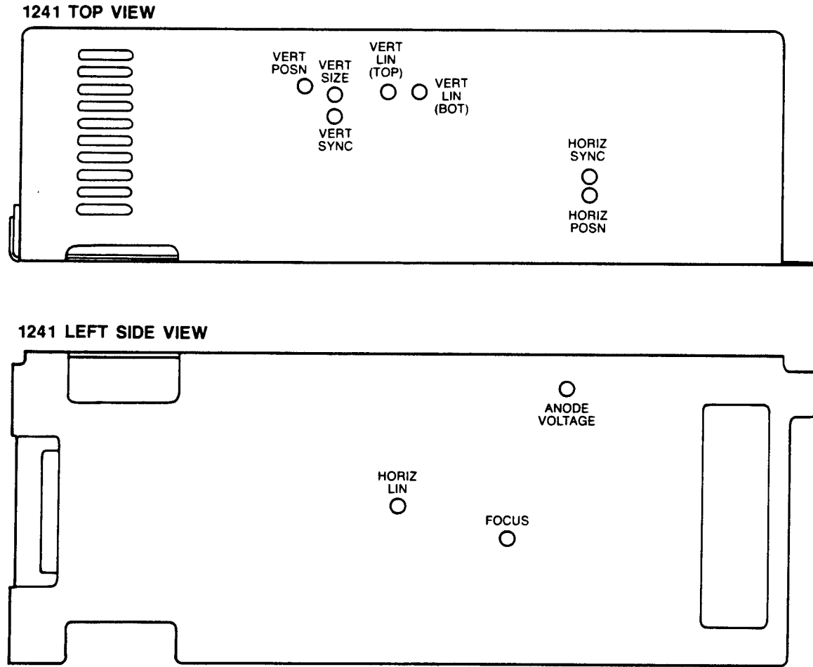
Figure 5-2. 1241 CRT Drive Board adjustment holes.
