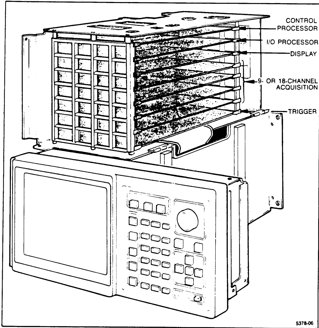
Figure 4-3. 1241 card-cage board locations.
