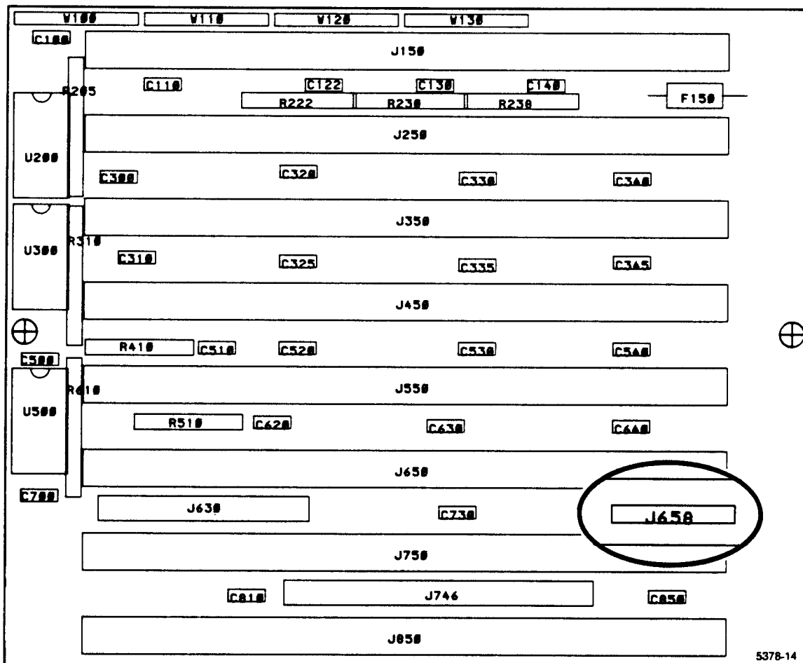
Figure 5-1. Expanded view of the Interface Board shows power supply measurement pins.
