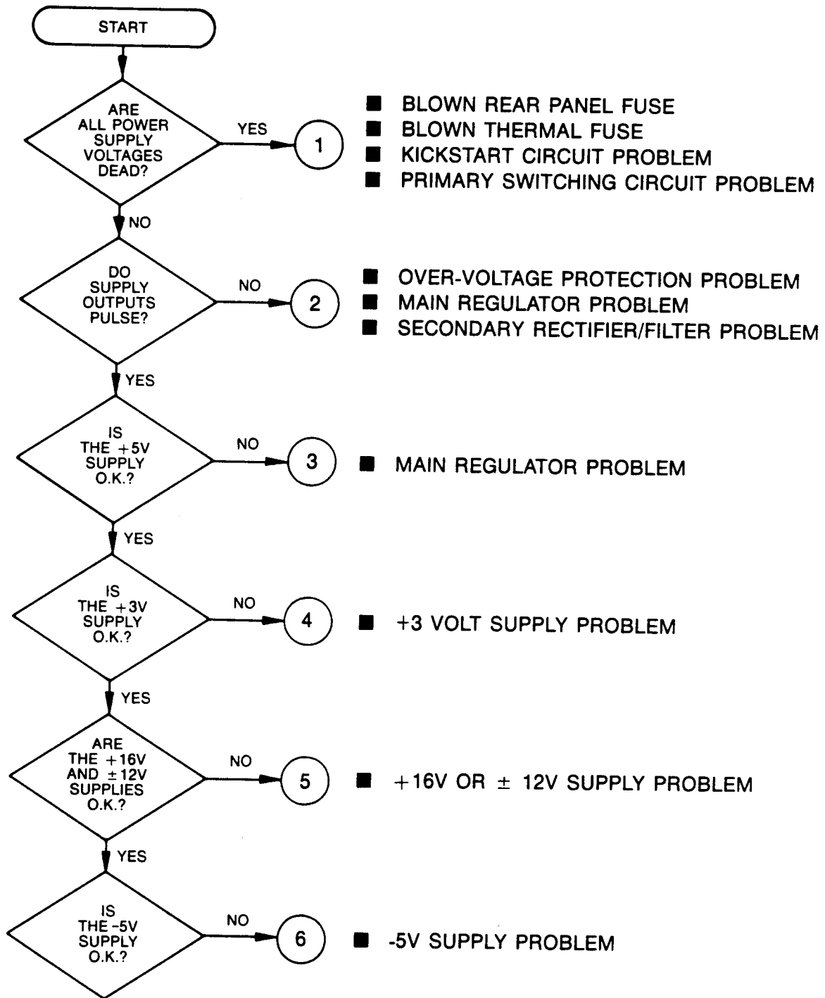
Figure 8-1. 1241 power supply troubleshooting tree.
