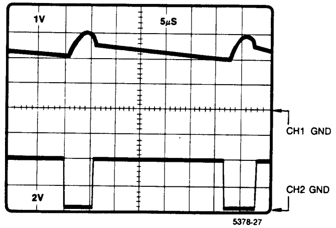
Figure 8-7. A13U218-4 sawtooth input; A13TP225 HDRIVE(L).
