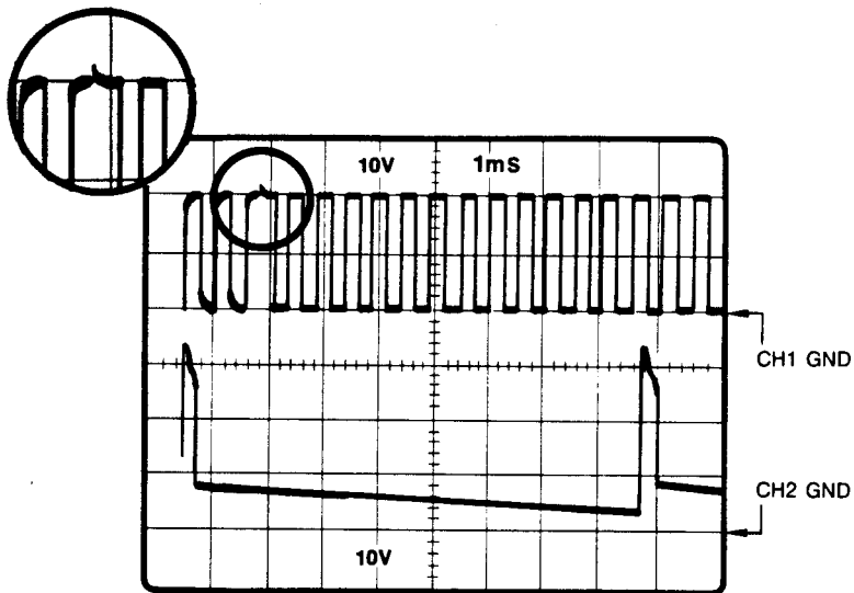
Figure 8-12. A13J200-4 color shutter drive; A13TP148 vertical flyback.
