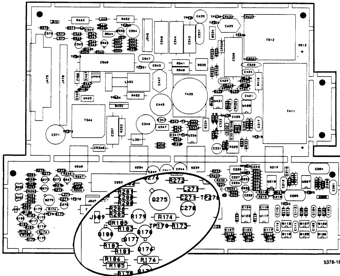
Figure 5-5. Expanded view of the CRT Drive Board shows components used in the External Trigger Adjust.
