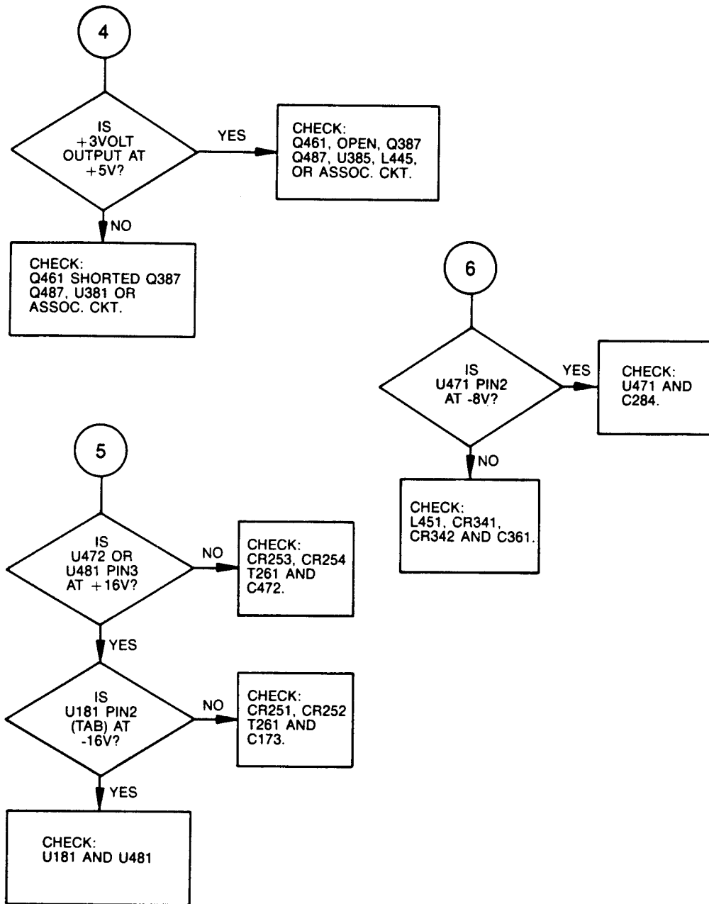
Figure 8-1. 1241 power supply troubleshooting tree (cont.).
