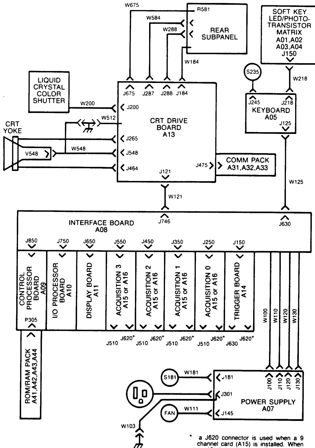
Figure 4-4. 1241 cables and connections.
