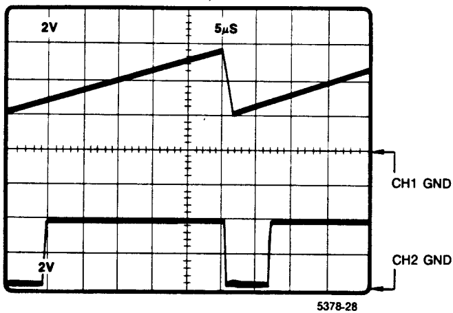
Figure 8-8. A13TP223 horizontal oscillator; A13TP225 HDRIVE(L).
