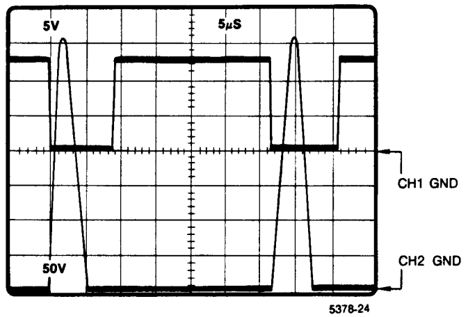
Figure 8-4 A13TP340 Q534 gate drive; A13TP456 horizontal flyback.
