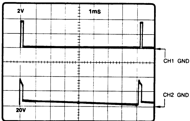
Figure 8-14. A13U138-12 VDRIVE(H); A13TP148 vertical flyback.
