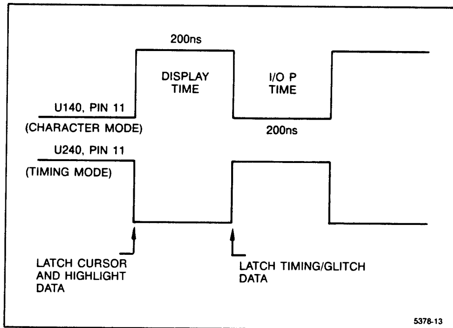
Figure 4-10. Display memory access times.
