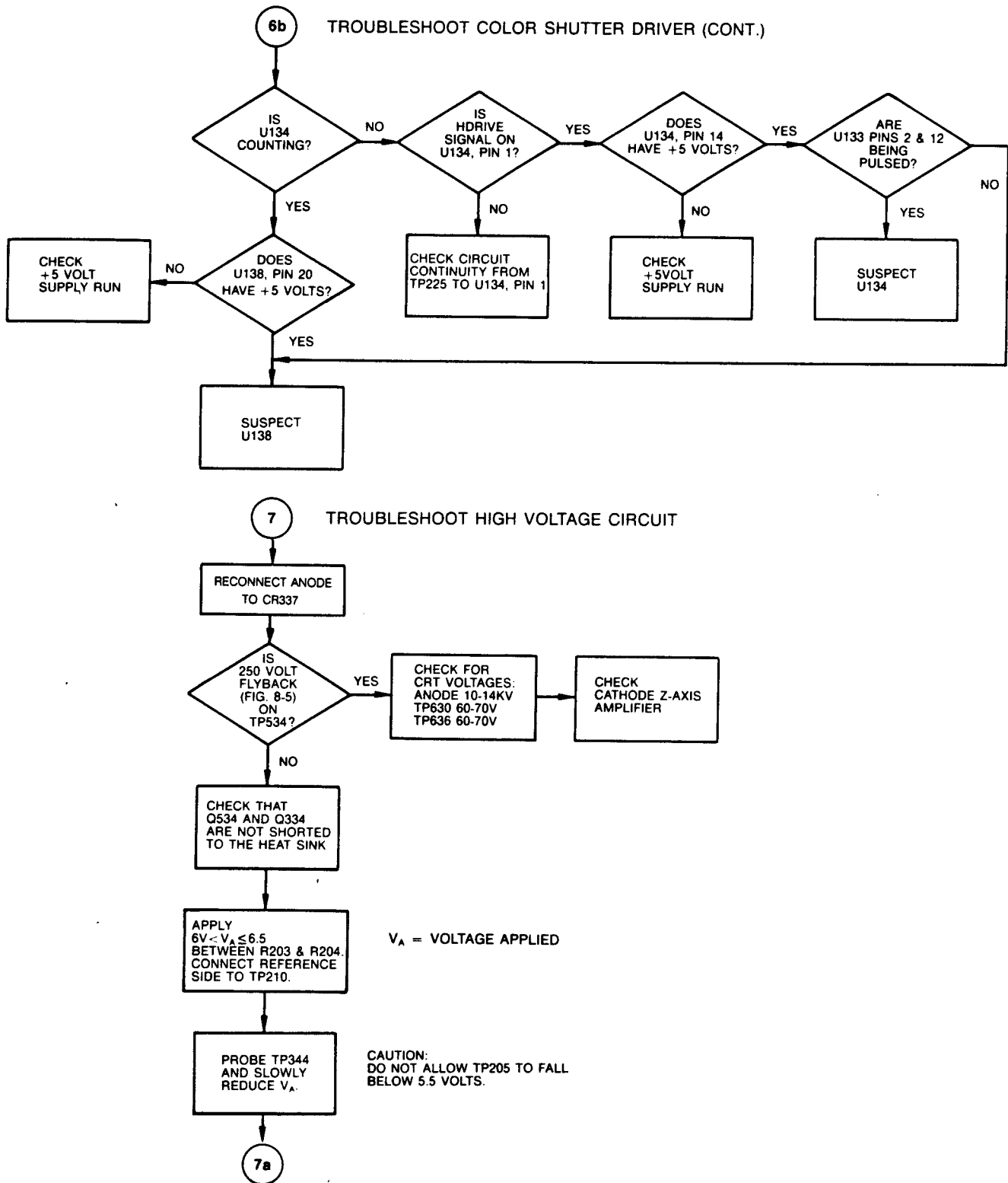
Figure 8-2. 1241 CRT Drive Board troubleshooting tree (cont.).
