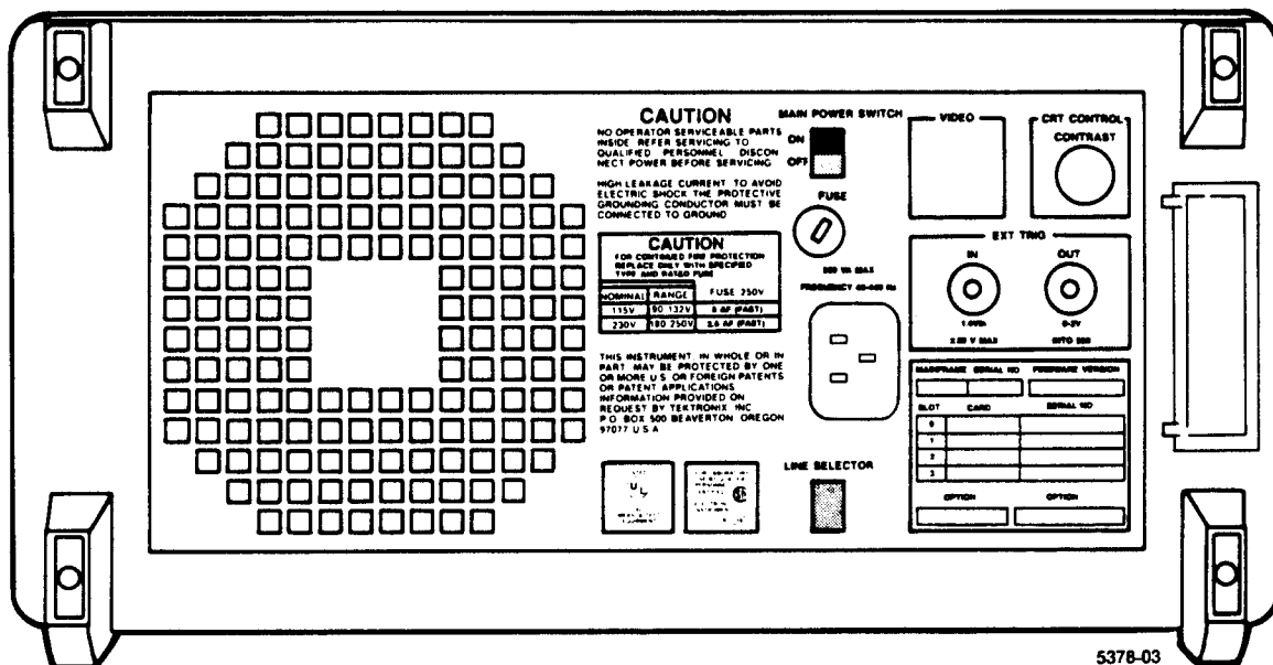
Figure 3-1. 1241 rear panel.
