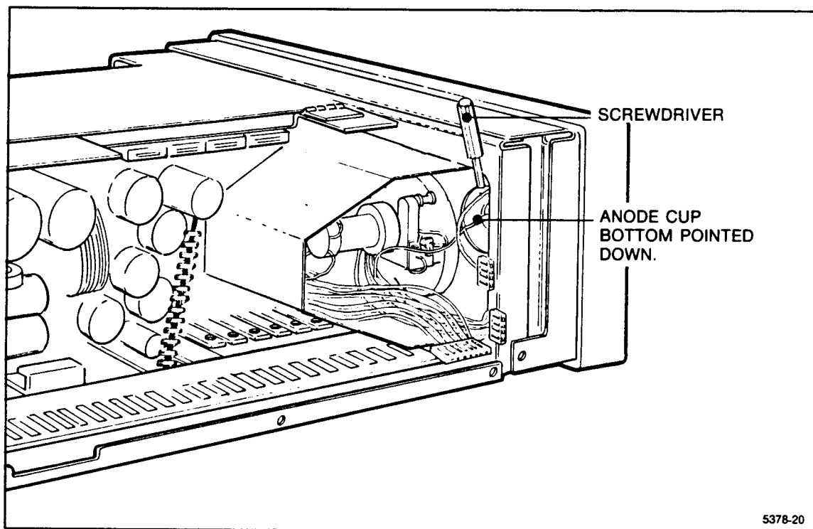
Figure 6-2. Discharging a CRT using a flat-blade screwdriver.
