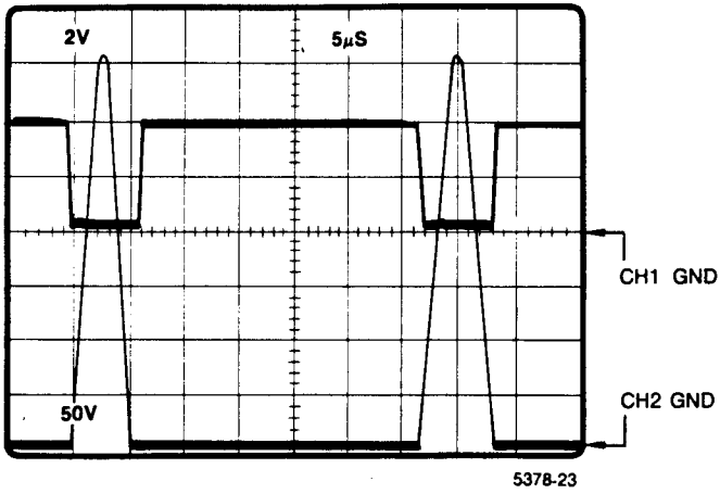
Figure 8-3. A13TP225 HDRIVE(L); A13TP456 horizontal flyback.
