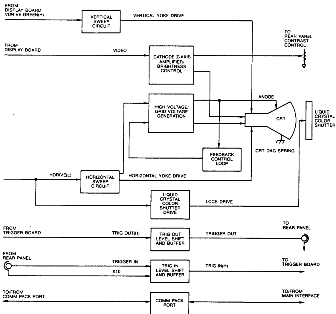
Figure 4-6. CRT Drive Board functional block diagram.
