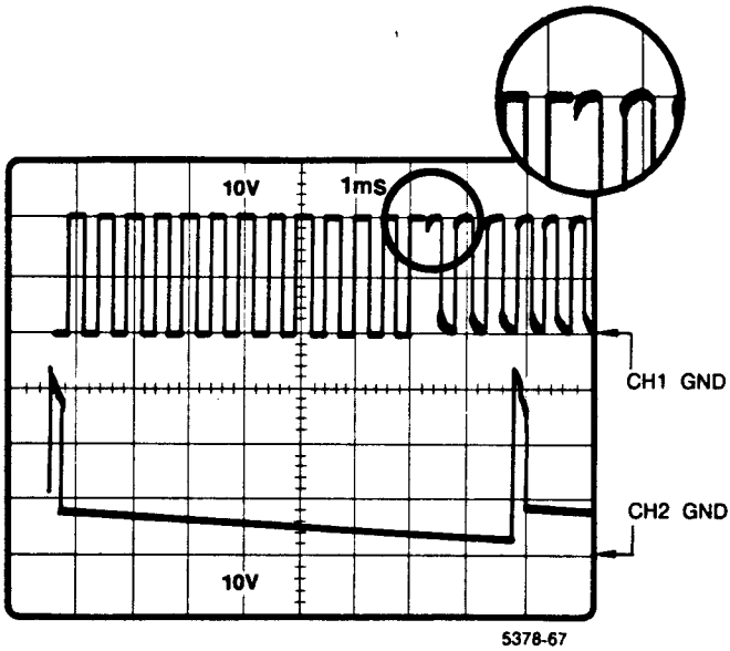
Figure 8-11. A13J200-3 color shutter drive; A13TP148 vertical flyback.
