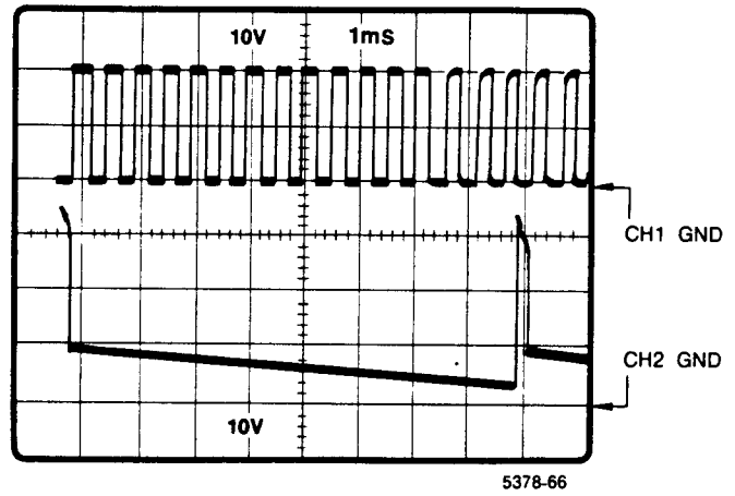
Figure 8-10. A13J200-1 and J200-2 color shutter drive; A13TP148 vertical flyback.
