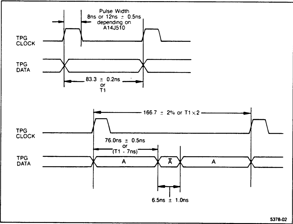
Figure 2-2. TPG clock and data outputs.
