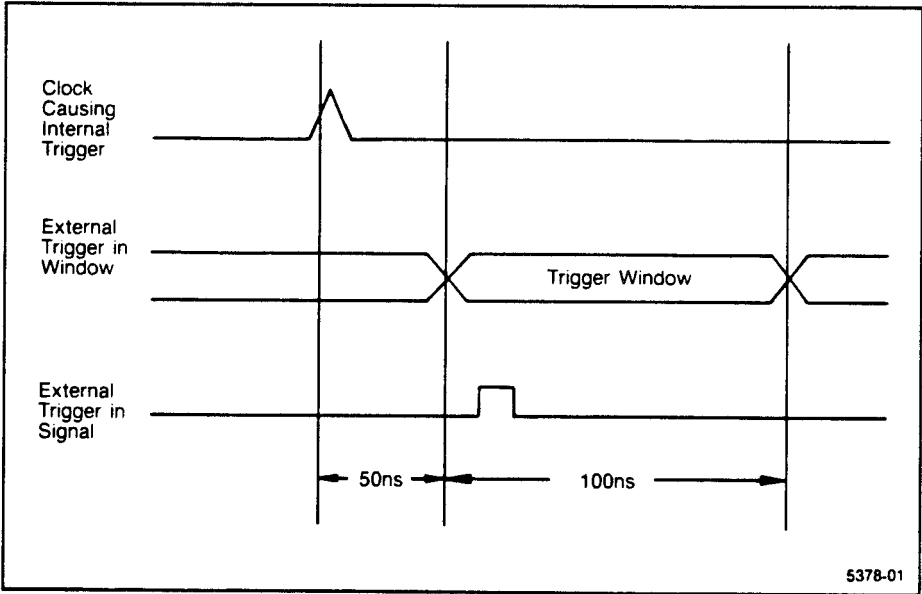
Figure 2-1. External Trigger In acceptance window.
