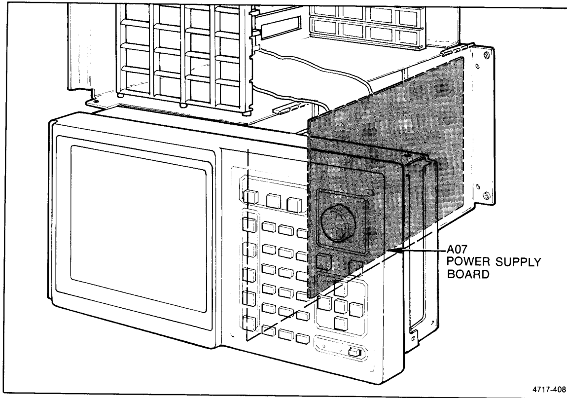
Figure 10-4. A07 1241 Power Supply Board Mainframe Location.
