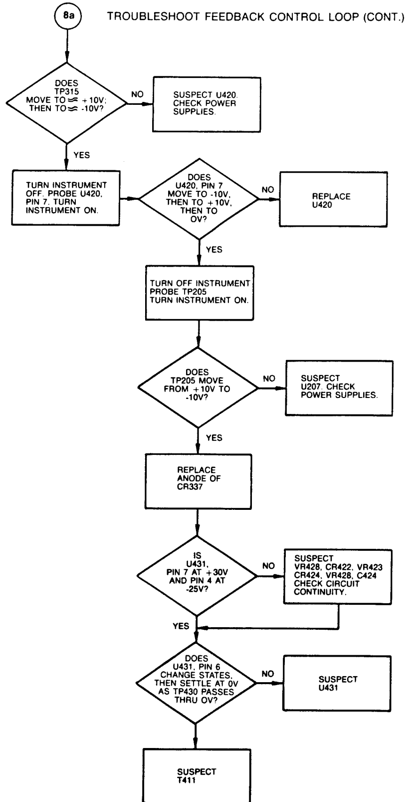
Figure 8-2. 1241 CRT Drive Board troubleshooting tree (cont.).
