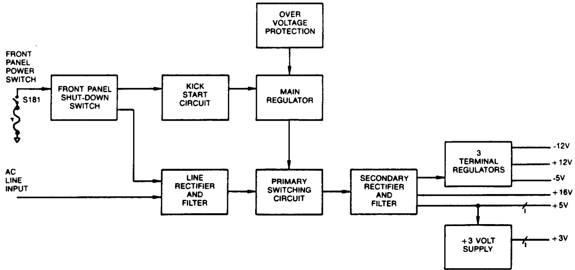
Figure 4-5. 1241 Power Supply Board functional block diagram.
