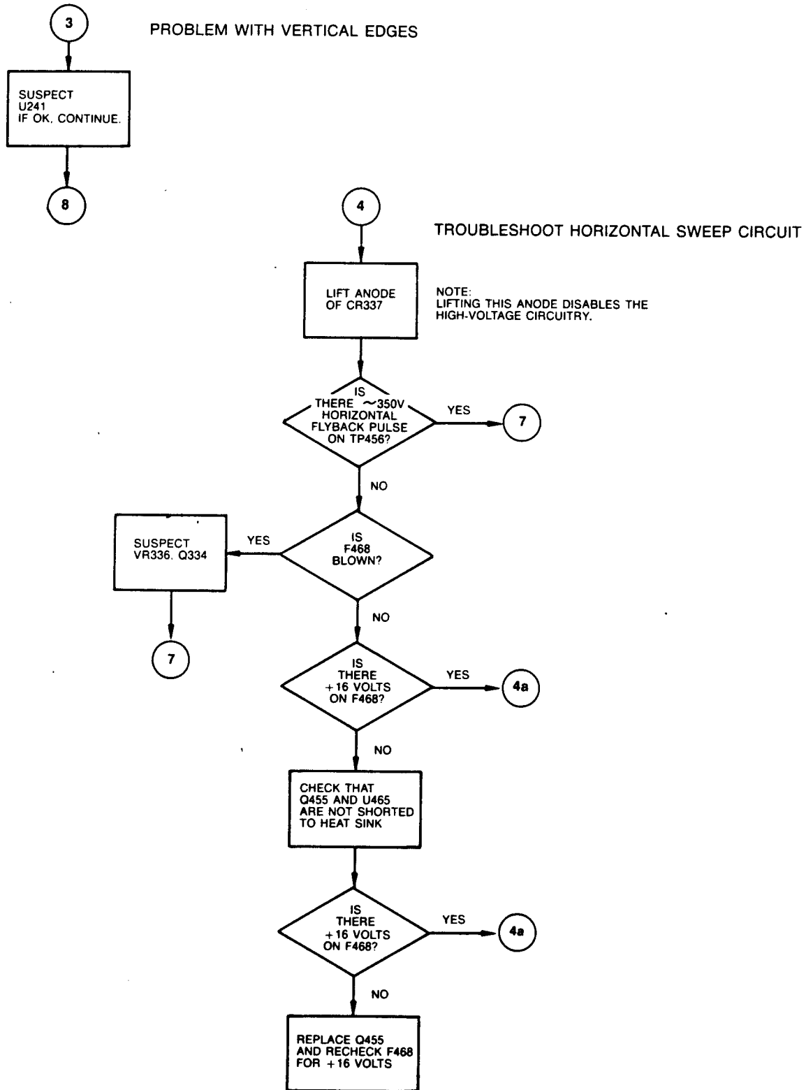
Figure 8-2. 1241 CRT Drive Board troubleshooting tree (cont.).
