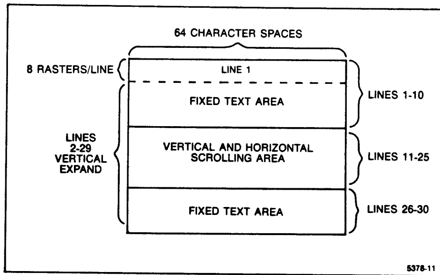
Figure 4-8. An example of 1241 display screen memory.
