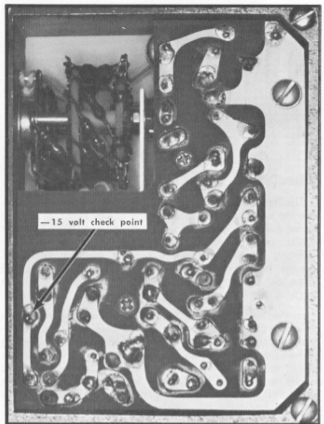
Fig. 6-2. Method used to modify the oscilloscope calibrator. This method provides a simple, accurate, 4-ma current probe source which is readily available for checking the probe.
