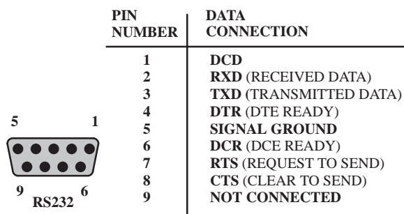
Figure 2–11: Rear panel RS232 connector
