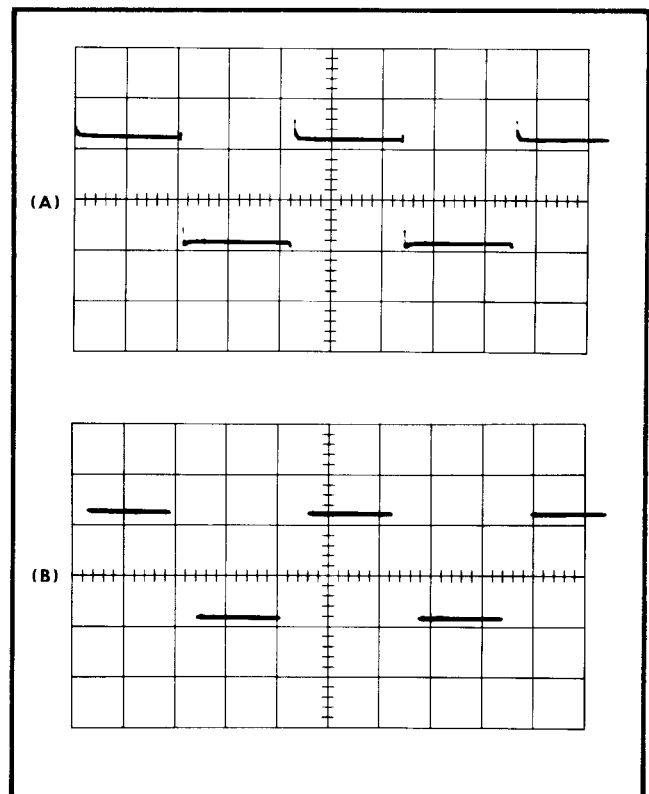
Fig. 7-7. (A) Unblanking chopped-mode waveform, and (B) blanked waveform. Sweep rate is 1 \mu\text{sec}/\text{div} .
