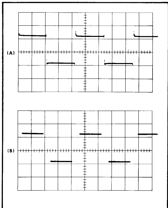
Fig. 6-1. (A) Unblanked chopped-mode waveform, and (B) blanked waveform. Sweep rate is 1 \mu sec/div.
