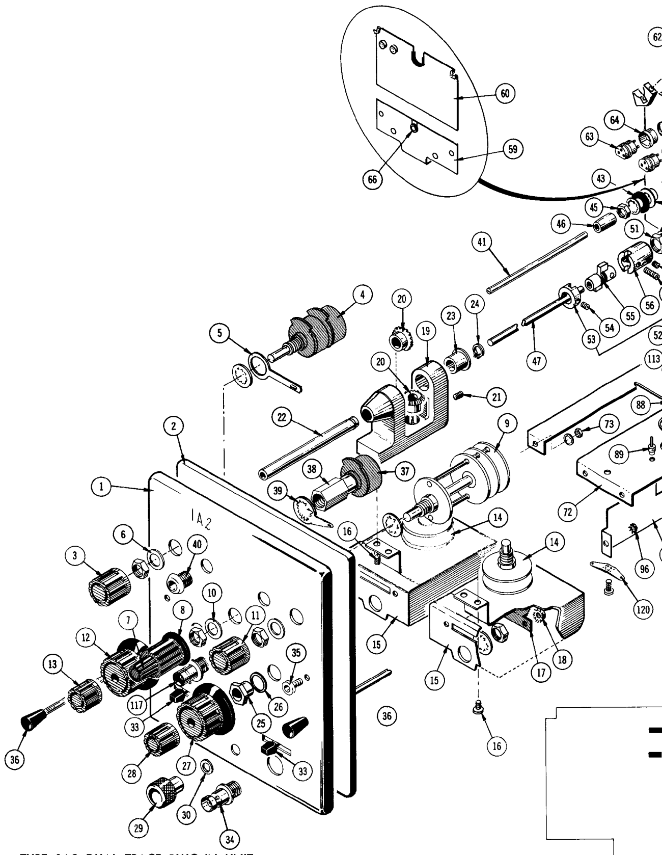
TYPE 1A2 DUAL TRACE PLUG-IN UNIT
