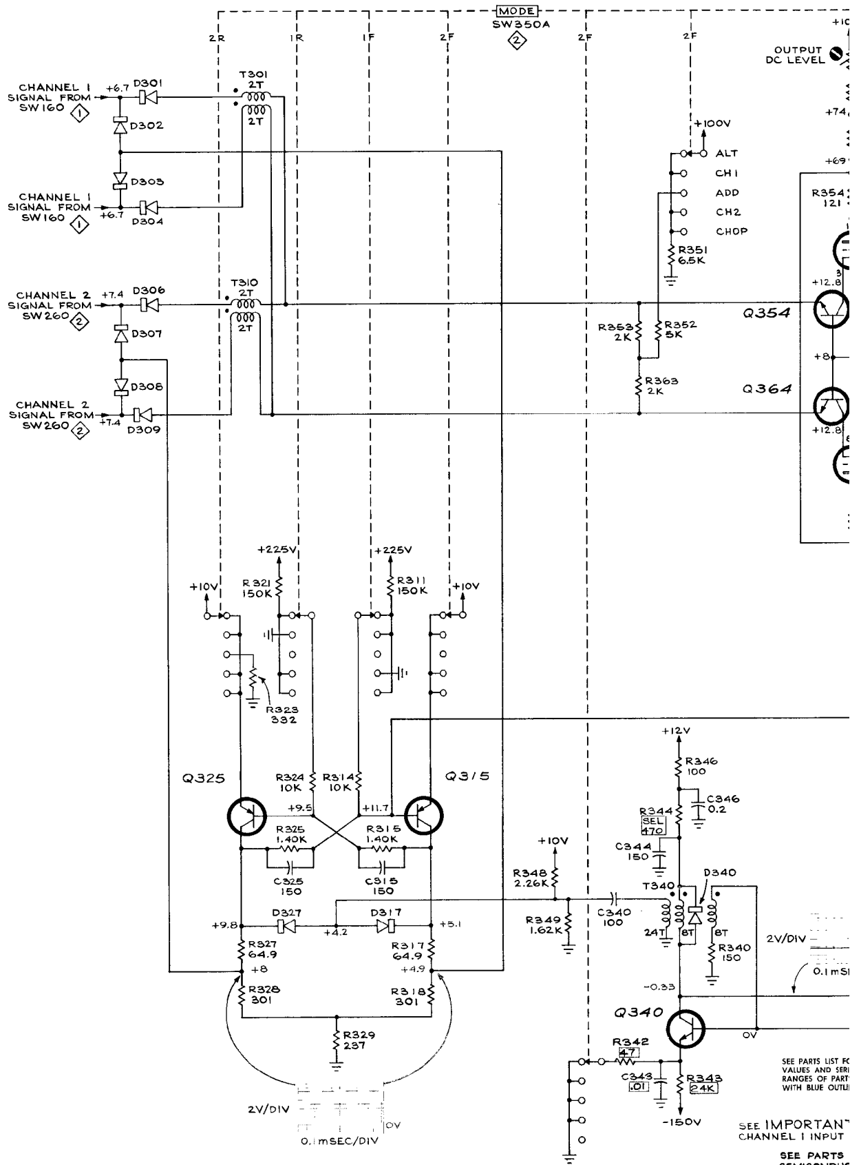
TYPE 1A2 PLUG-IN
