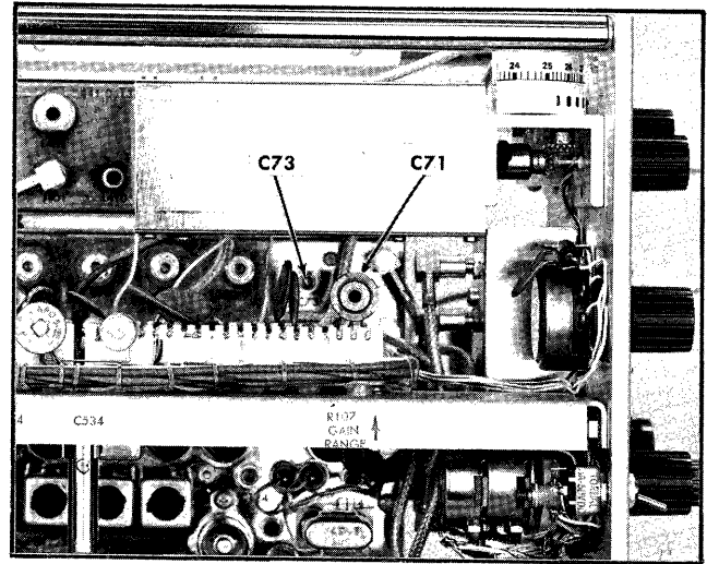
Fig. 4-16. Location of Balanced Mixer adjustments.
