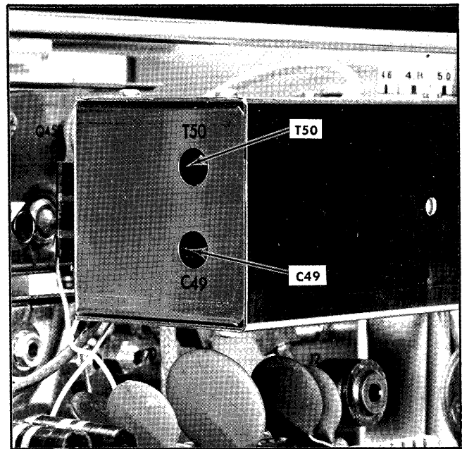
Fig. 4-20. Location of oscillator adjustments.
