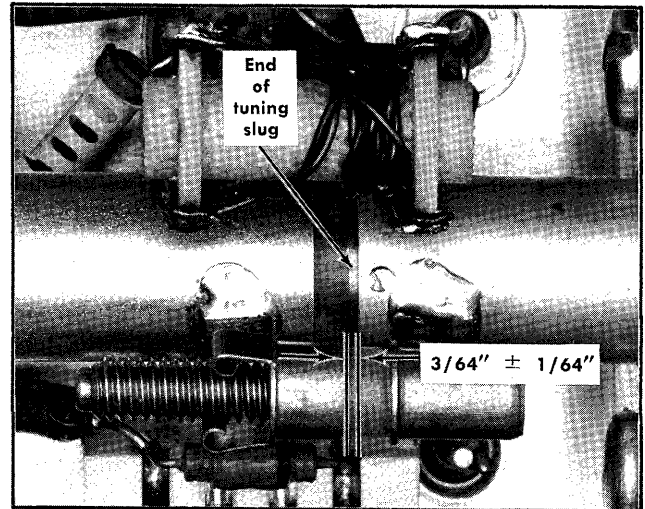
Fig. 4-21. Proper position of oscillator tuning slug when the dial reading is 36 mc.
