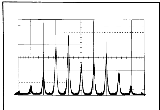
Fig. 4-5. A 5-mc signal modulated with a 2-kc audio signal. DISPERSION-KC/CM switch set at 2.
