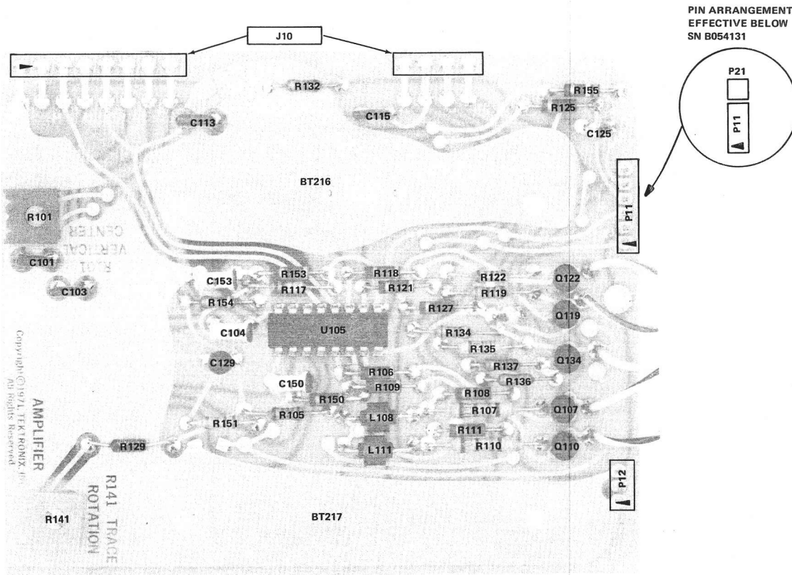
Fig. 9-2. A2 Amplifier Board
