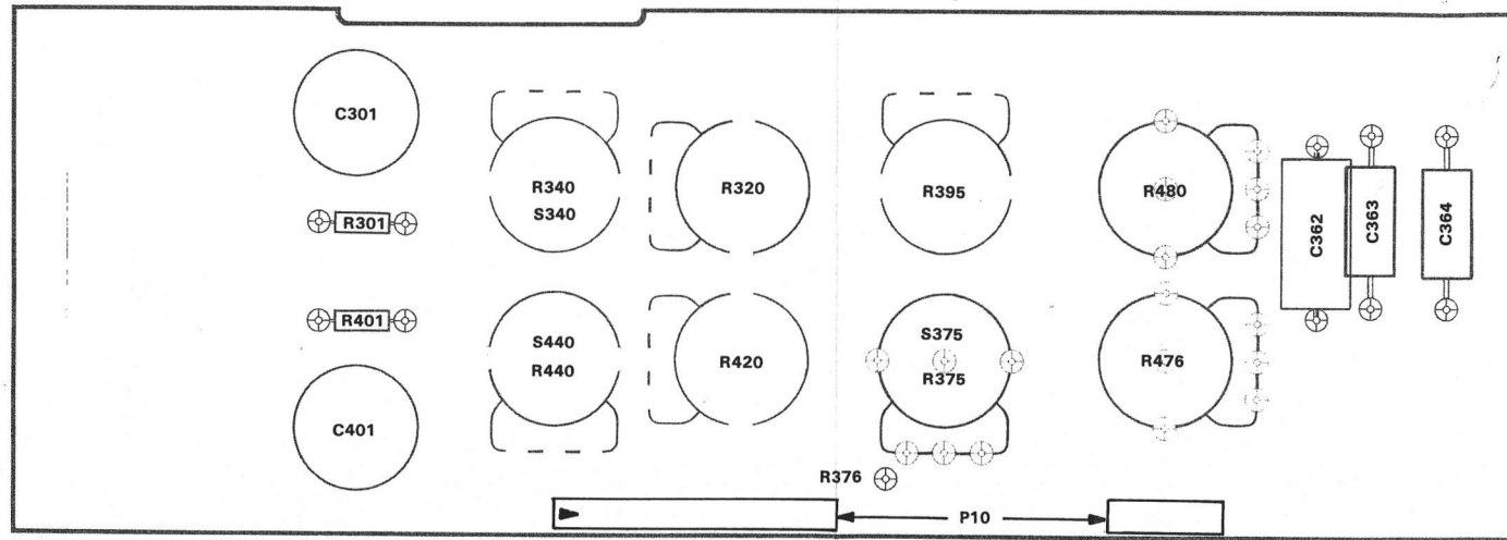
Bottom View
