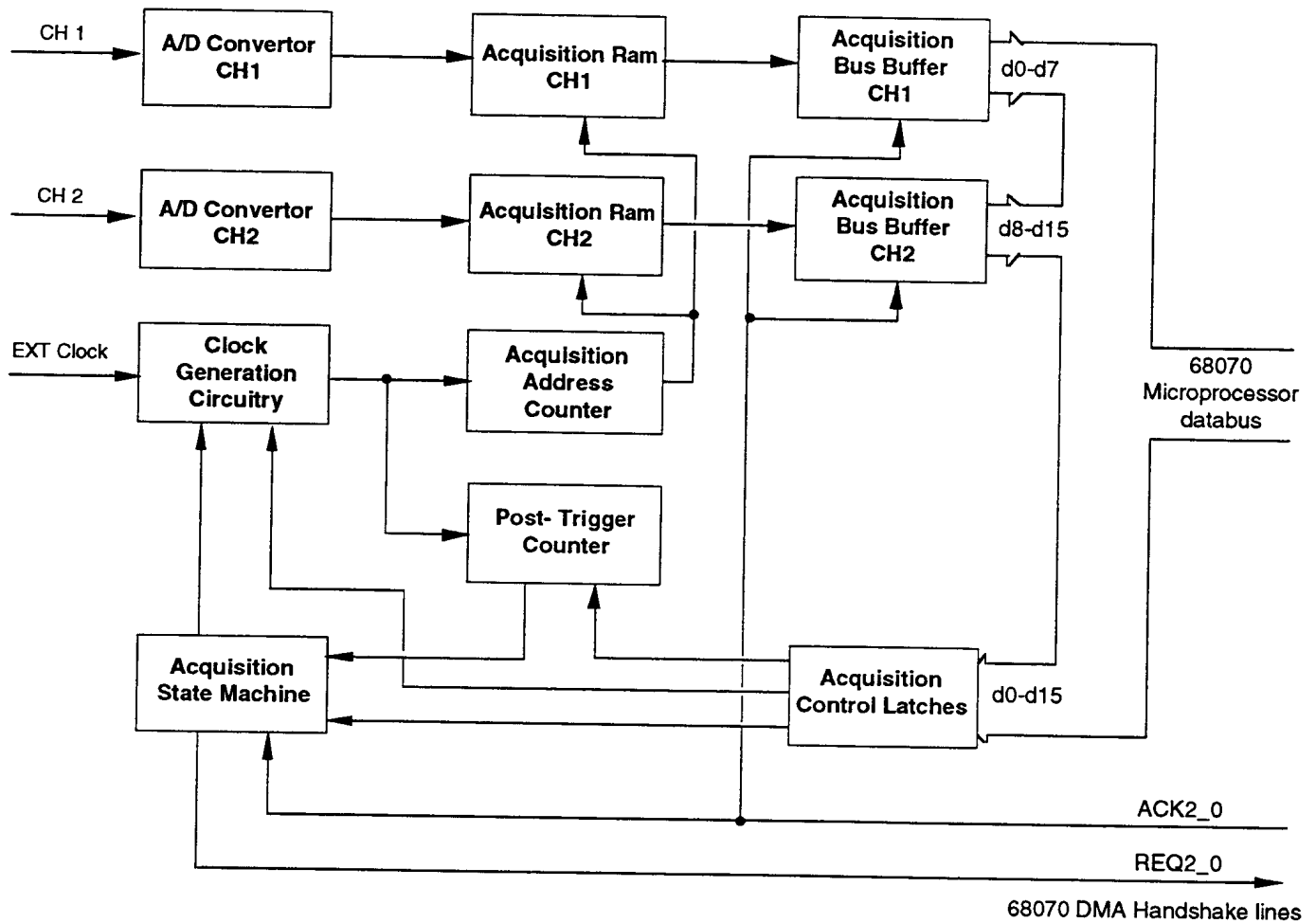
Figure 3-7: 2212 Acquisition Block Diagram
