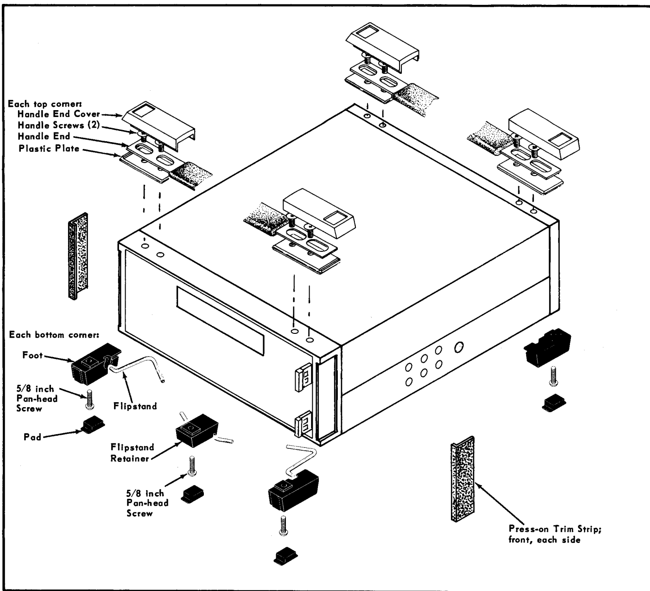
Fig. 9-1. Parts peculiar to the Type 241.
