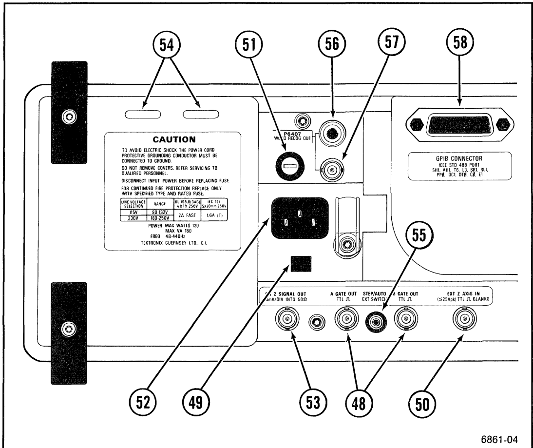
Figure 5-7. Rear panel controls and connectors.
