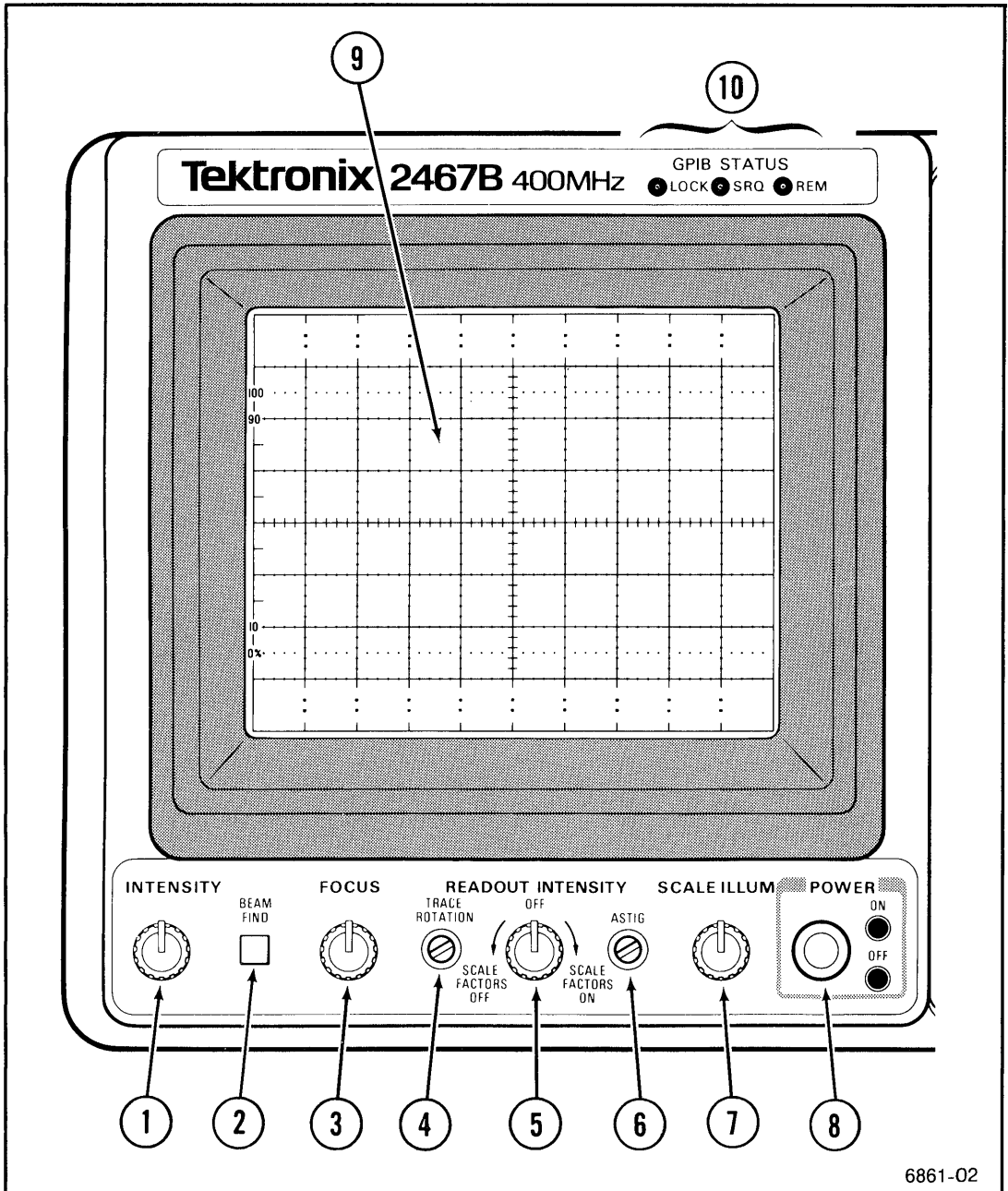
Figure 5-1. Power and display controls.
