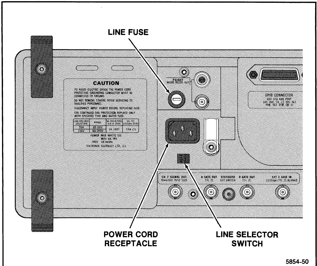
Figure 1-1. Line selector switch, line fuse, and detachable power cord.
