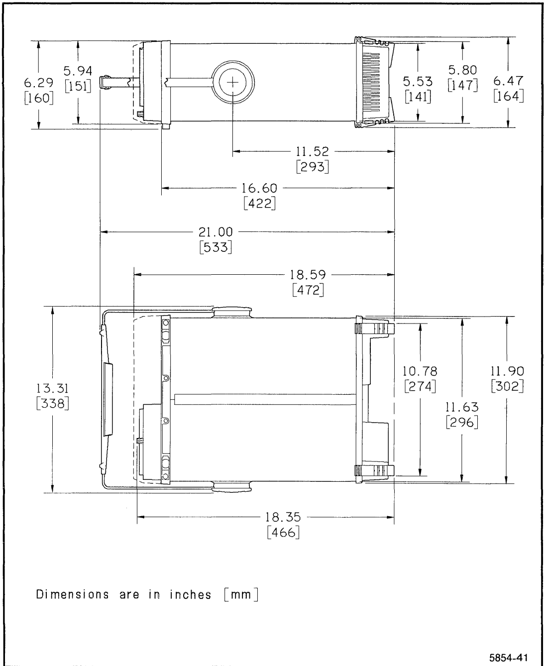
Figure 6-1. Dimensional drawing.
