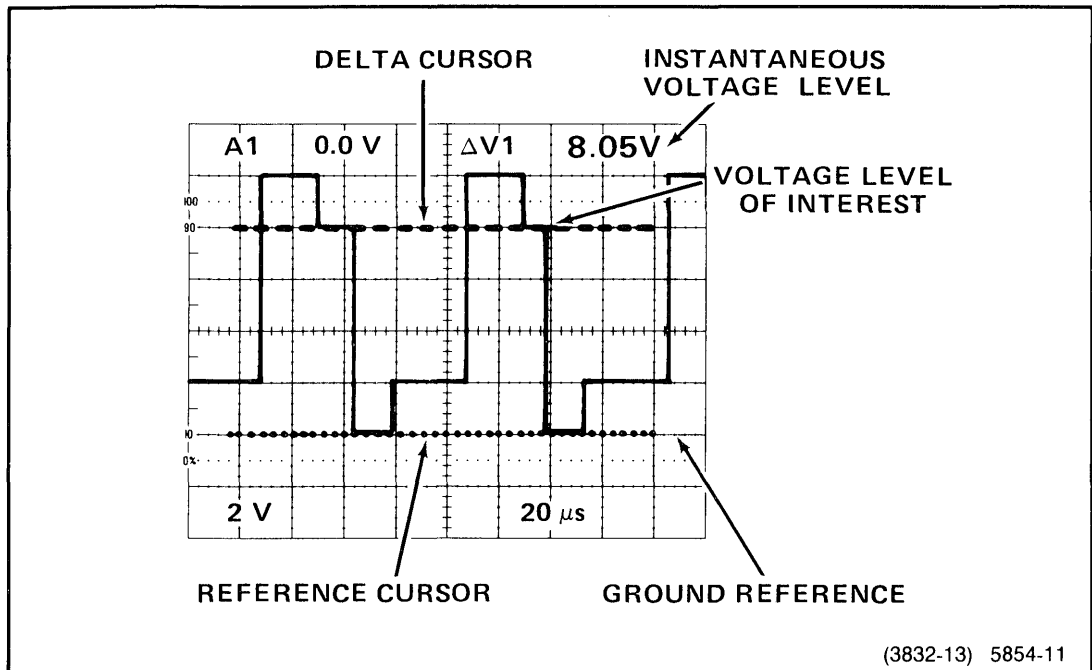
Figure 3-1. Instantaneous voltages.
