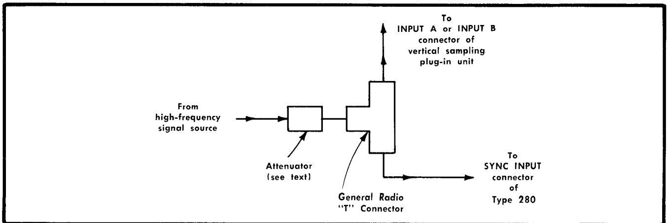
Fig. 2-7. Method of obtaining a sync signal when none is available at source. See text for limitations of this network.
