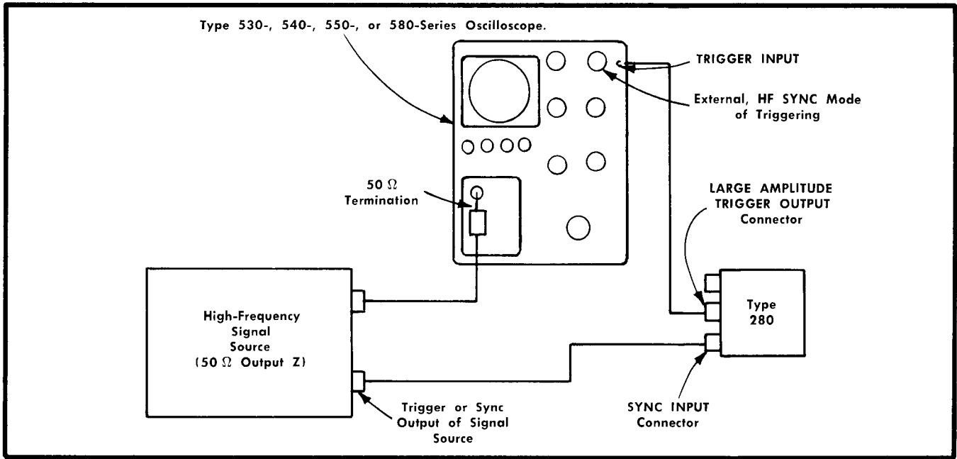
Fig. 2-6. The Type 280 Trigger Countdown Unit connected for use with Tektronix 530-, 540-, 550-, or 580-Series Oscilloscope.
