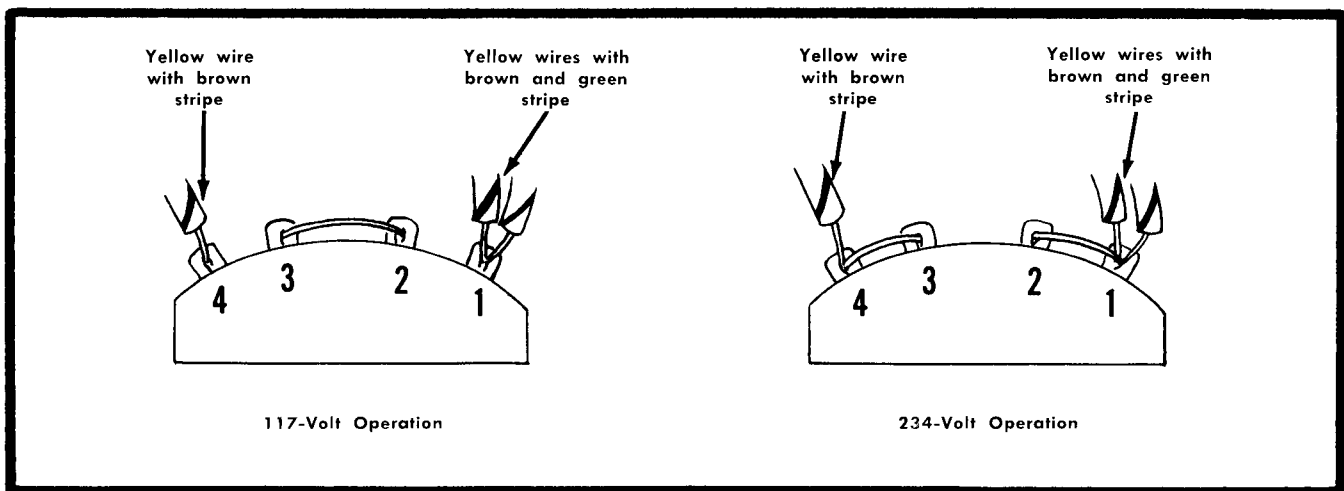
Fig. 2-1. Line transformer connections for 117- and 234-volt operation.
