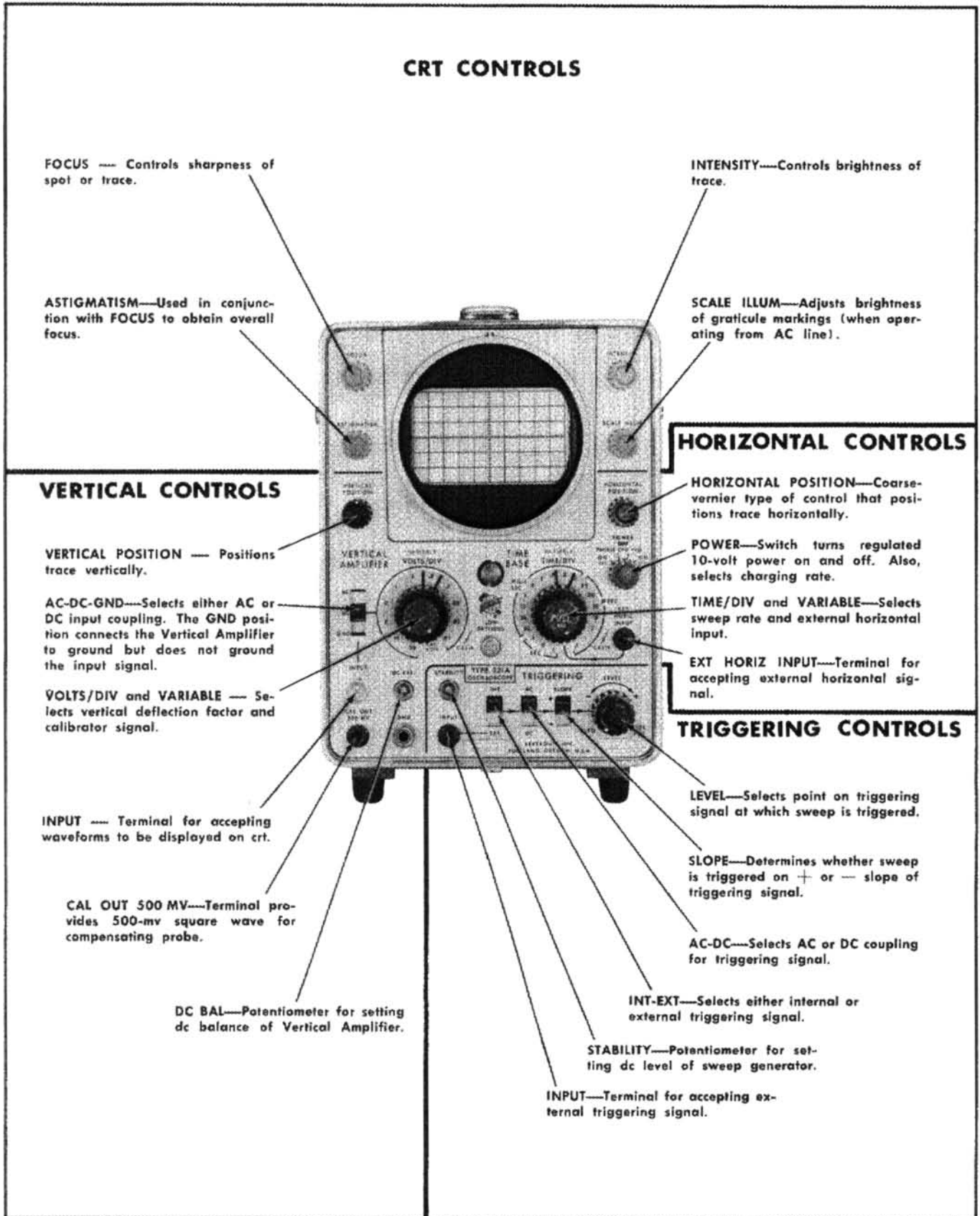
Fig. 3-1. Functions of the Type 321A Oscilloscope front-panel controls.
