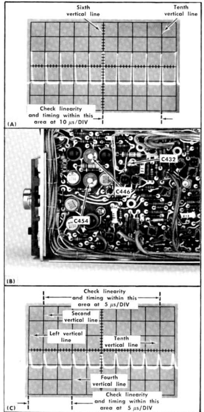
Fig. 6-17. (A) Typical CRT display showing correct high-speed linearity and timing at 10\ \mu\text{s}/\text{DIV} , (B) location of high-speed timing adjustments (Main board), (C) typical CRT display showing correct high-speed linearity and timing at 5\ \mu\text{s}/\text{DIV} .
