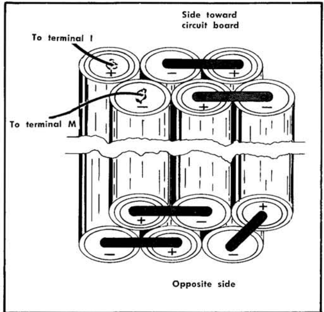
Fig. 4-11. Battery wiring.
