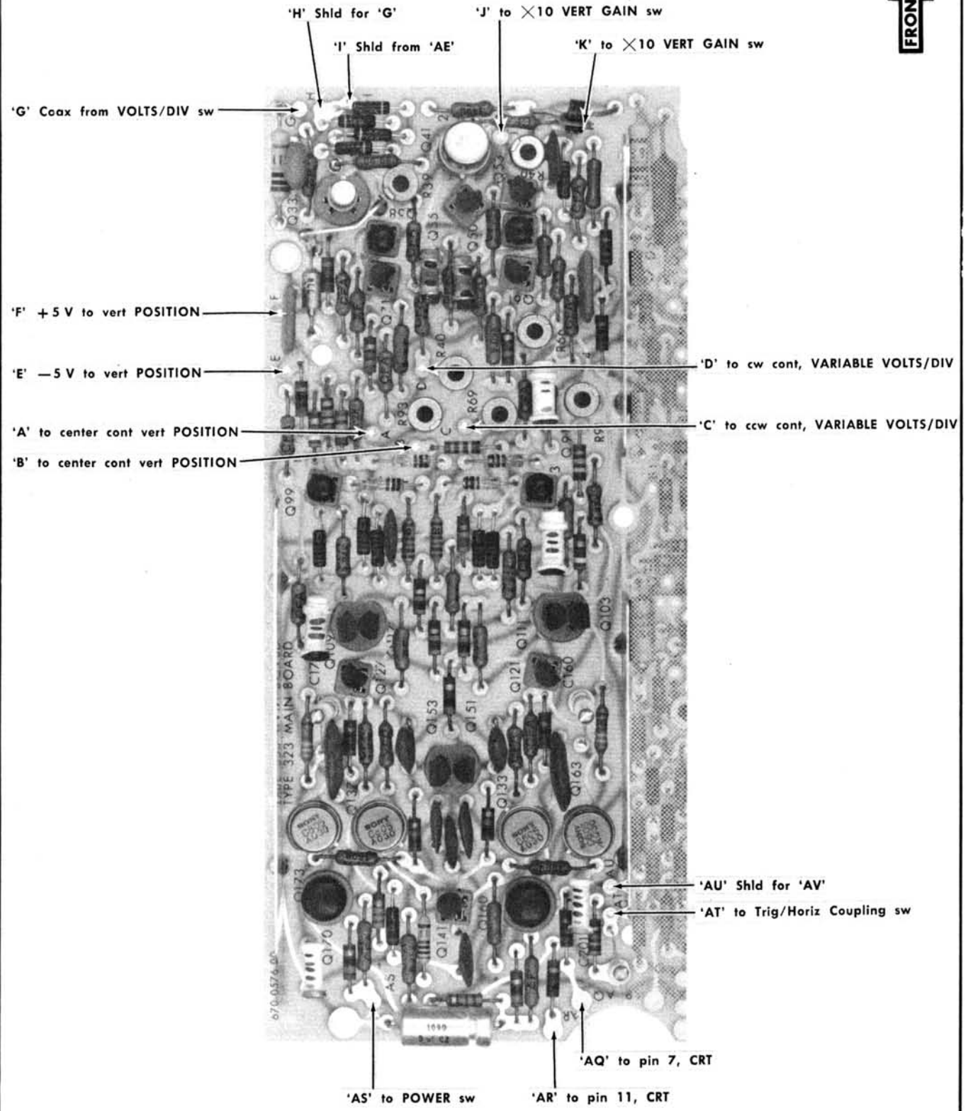
Fig. 4-16. Main circuit board (partial); left side—wire connections.
