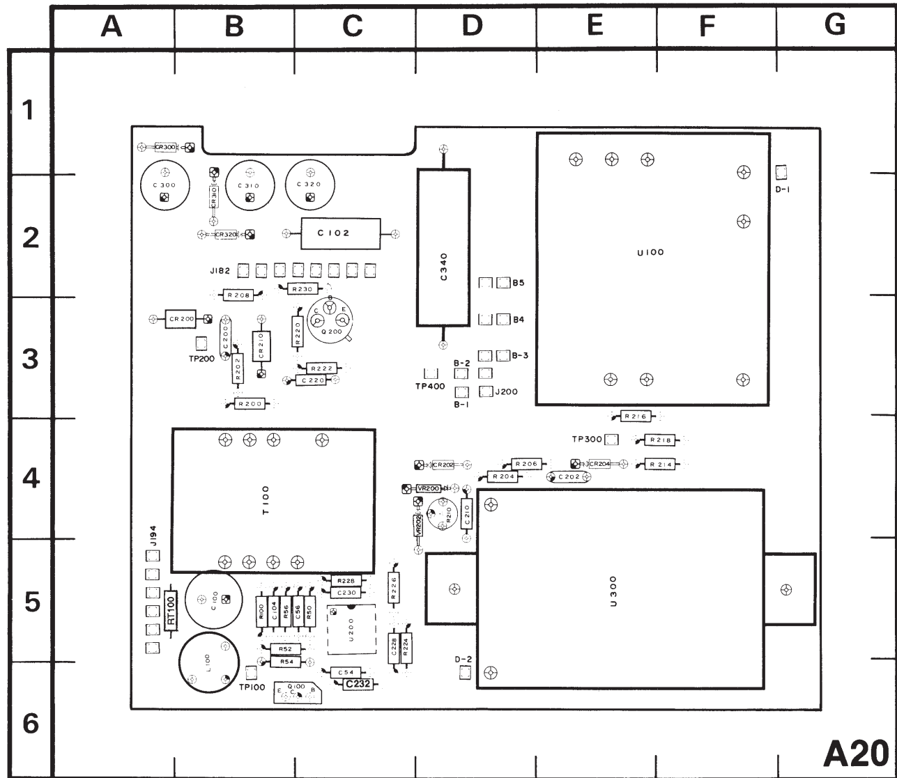
Figure 7-24. A20 — High Voltage Regulator circuit board assembly.
