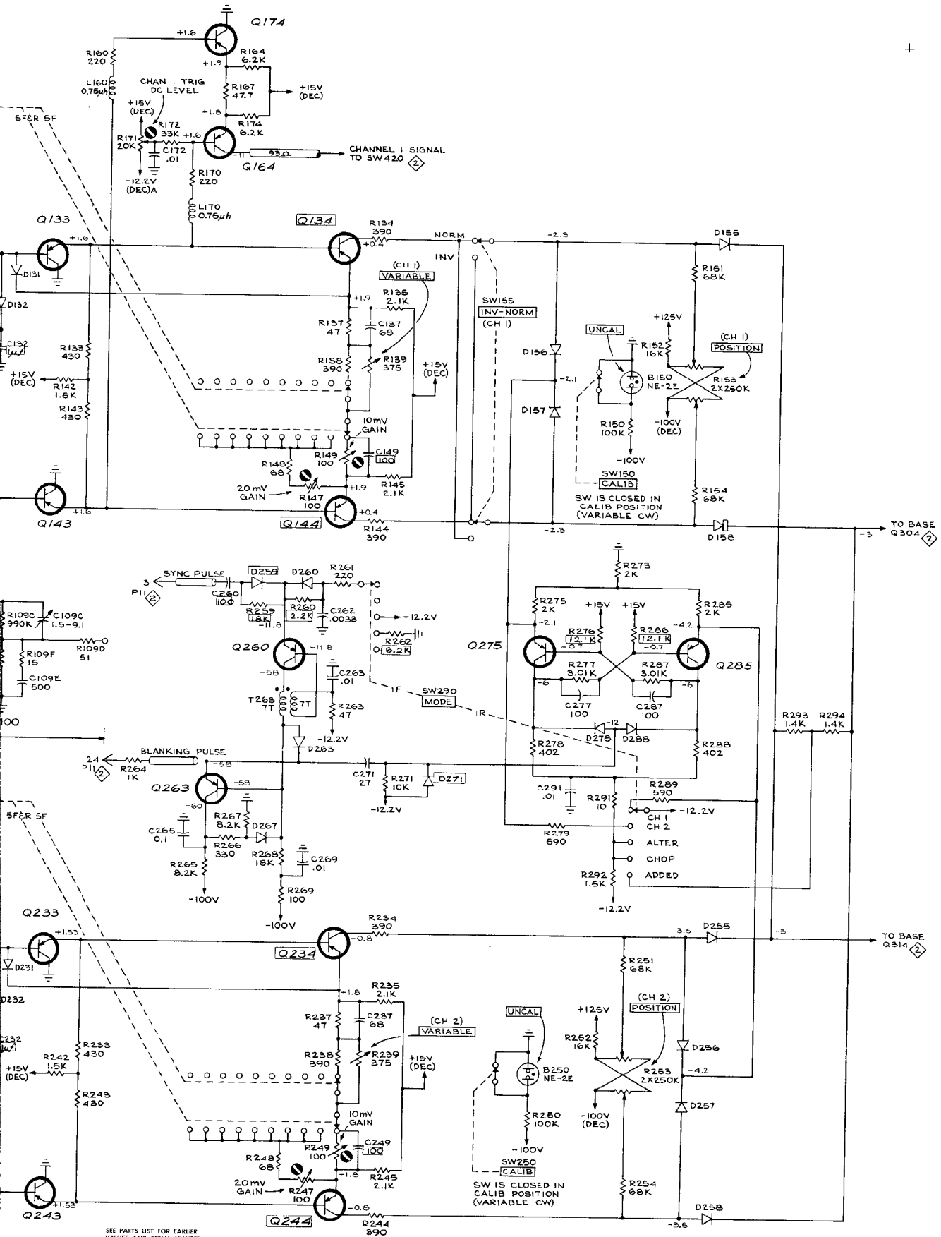
INPUT AMPLIFIER & SWITCHING CIRCUIT
