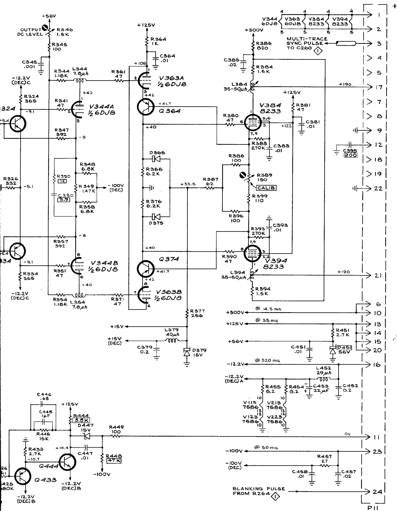
269 OUTPUT AMPLIFIER
