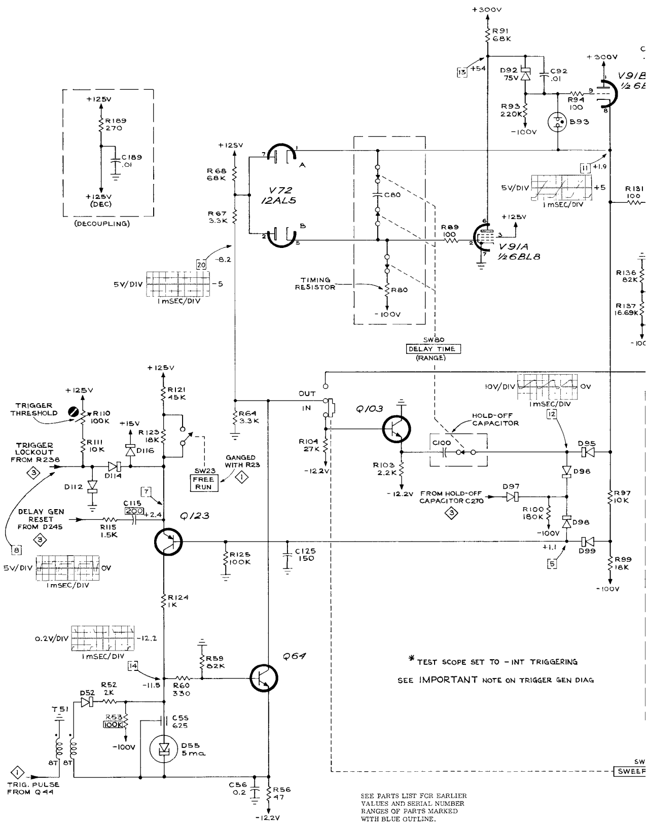
TYPE 3B2 PLUG-IN
