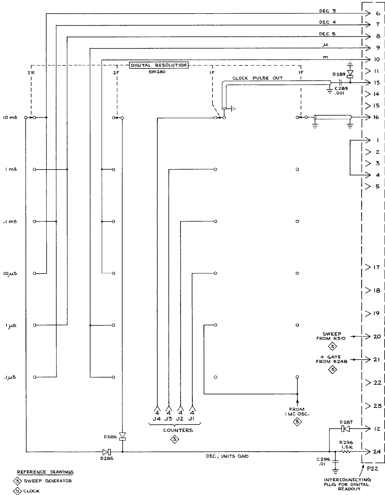
TIMING & RESOLUTION SWITCHES
