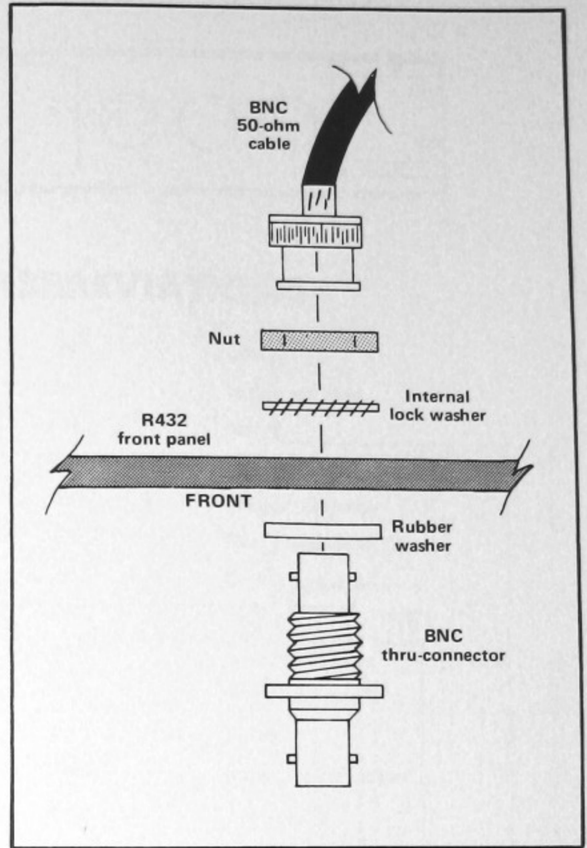
Fig. 6-5. Mounting a chassis-mount BNC thru-connector.
