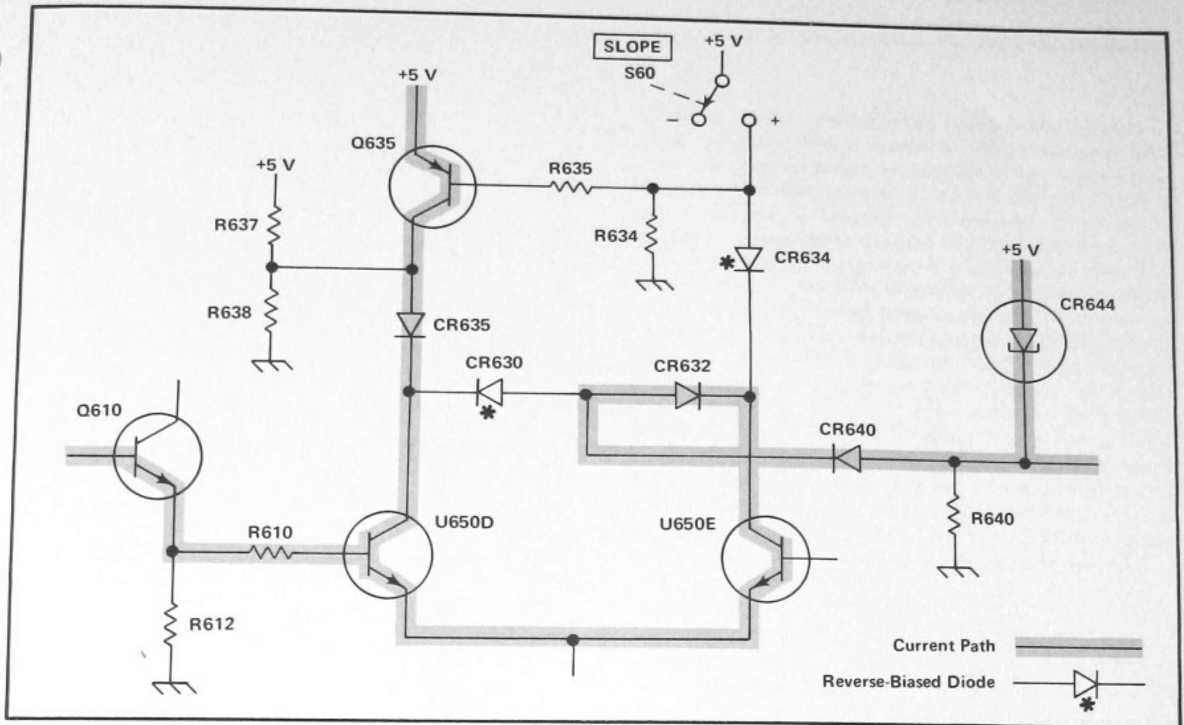
Fig. 3-10. Trigger signal path for negative-slope triggering (simplified Trigger Generator diagram).
