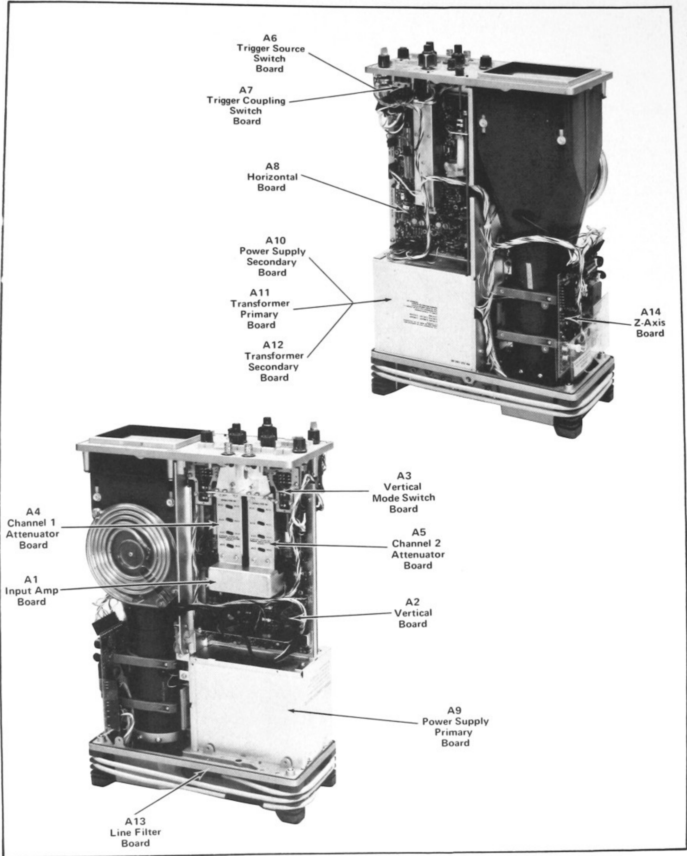
Fig. 4-5. Location of circuit boards in the 432.
