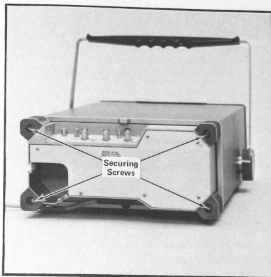
Fig. 4-1. Removing wrap-around cabinet.
