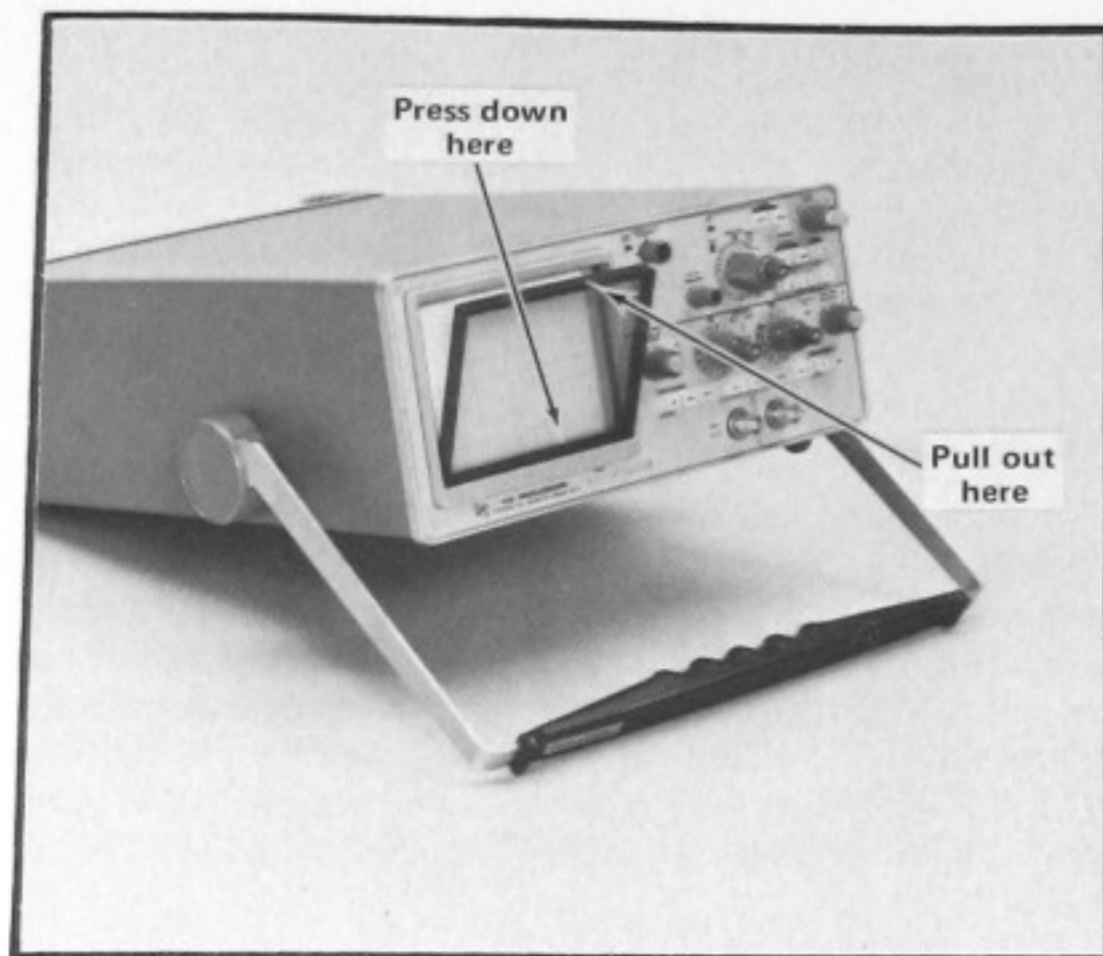
Fig. 2-4. Removing the filter.
