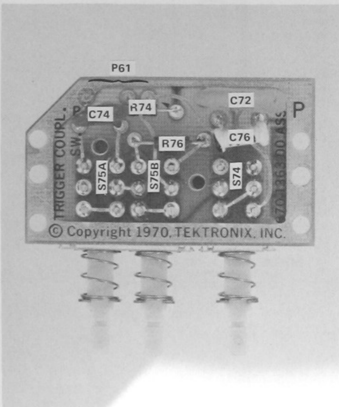
Fig. 8-11. A7. Trigger Coupling Switch Circuit board. ©
