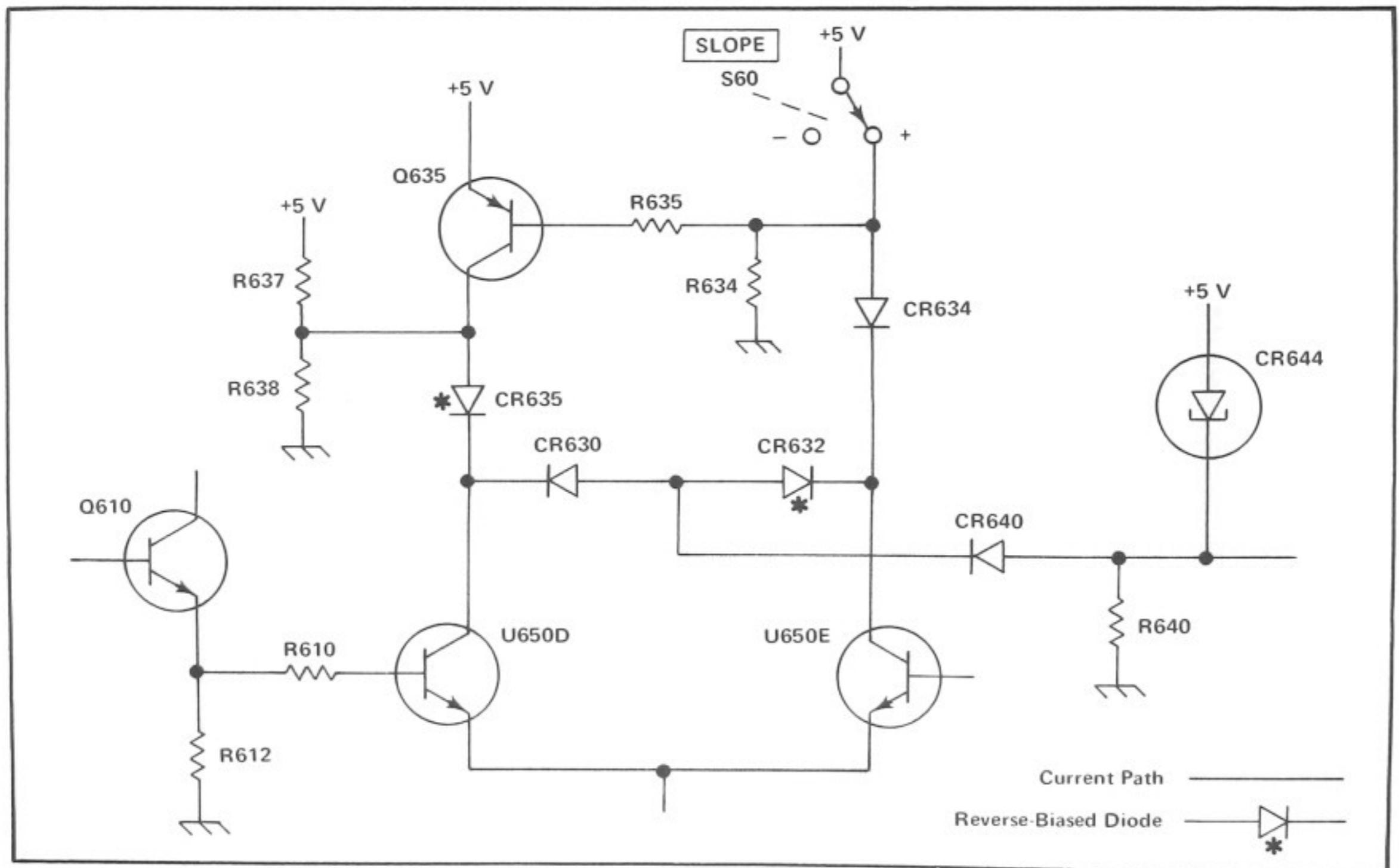
Fig. 3-9. Trigger signal path for positive-slope triggering (simplified Trigger Generator diagram).
