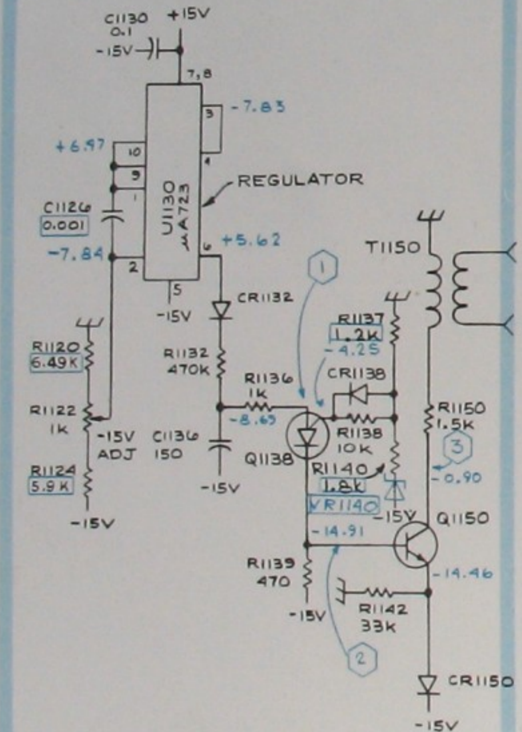
P/O A10 POWER SUPPLY SECONDARY CIRCUIT BOARD
