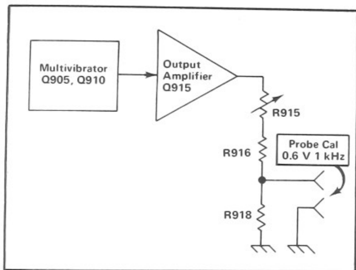
Fig. 3-15. Calibrator detailed block diagram.
