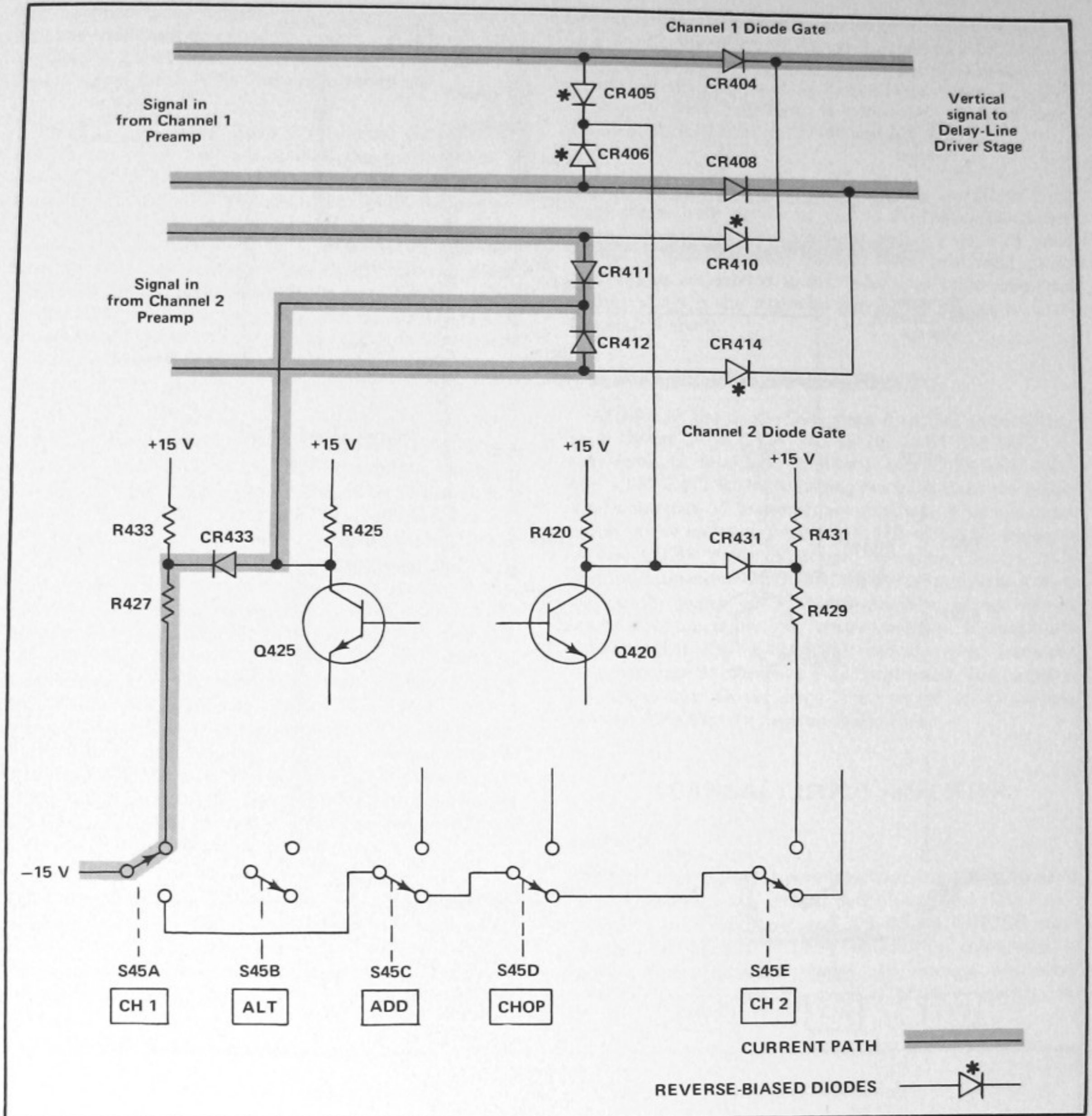
Fig. 3-5. Effect of Diode Gates on signal path (simplified path). Conditions shown for CH 1 mode of operation.
