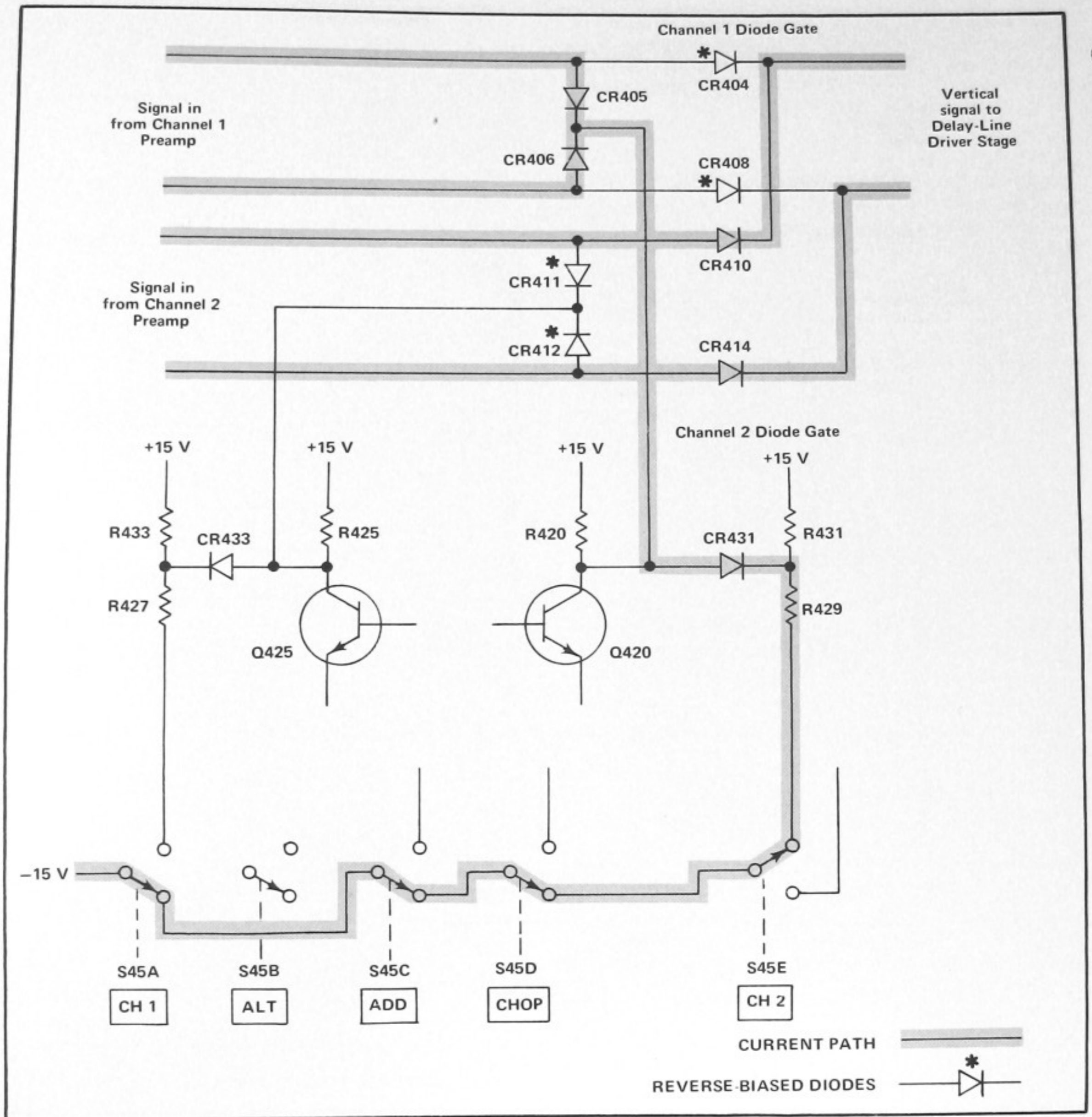
Fig. 3-6. Effect of Diode Gates on signal path (simplified path). Conditions shown for CH 2 mode of operation.
