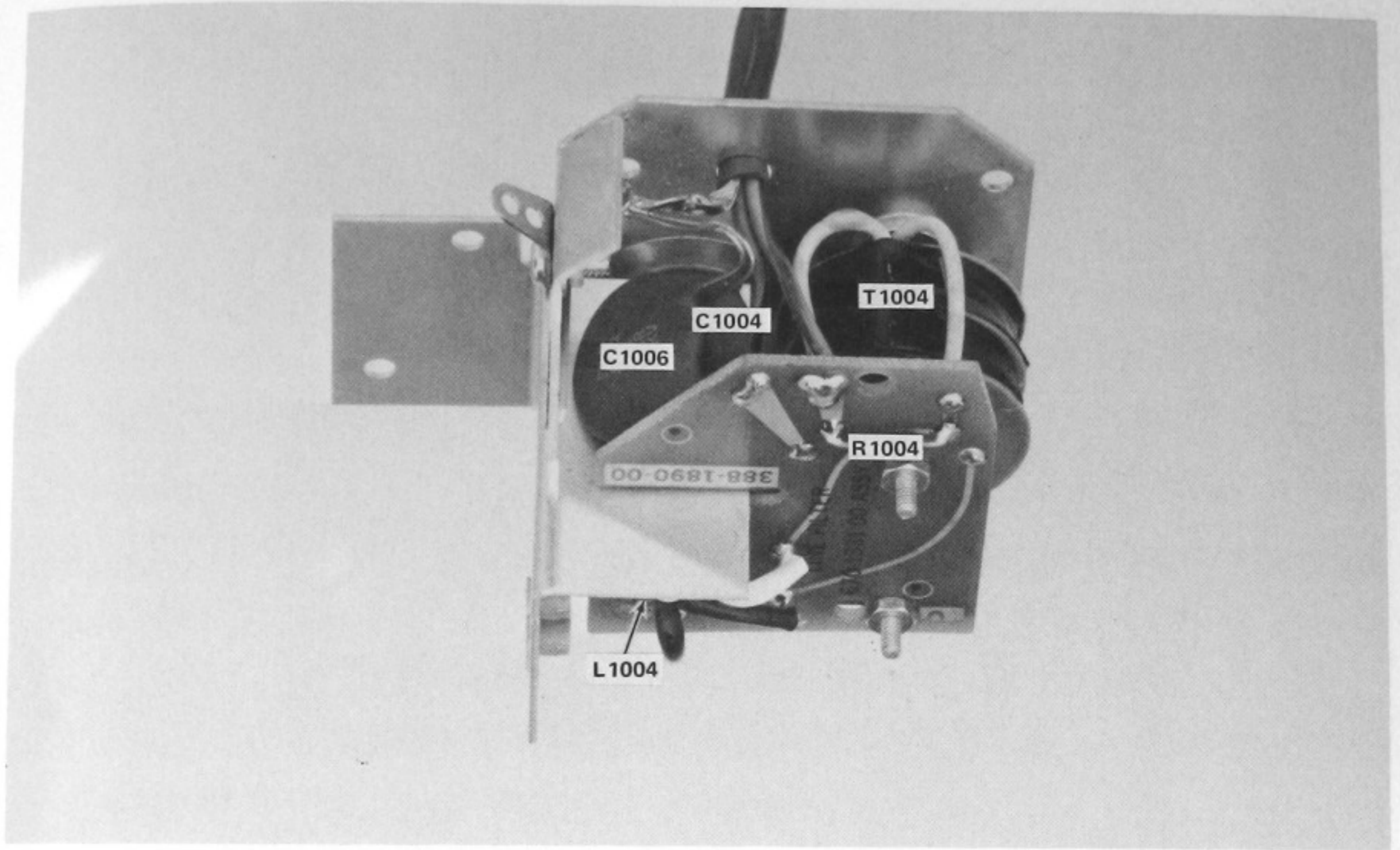
Fig. 8-19. A13. Line filter circuit board.
