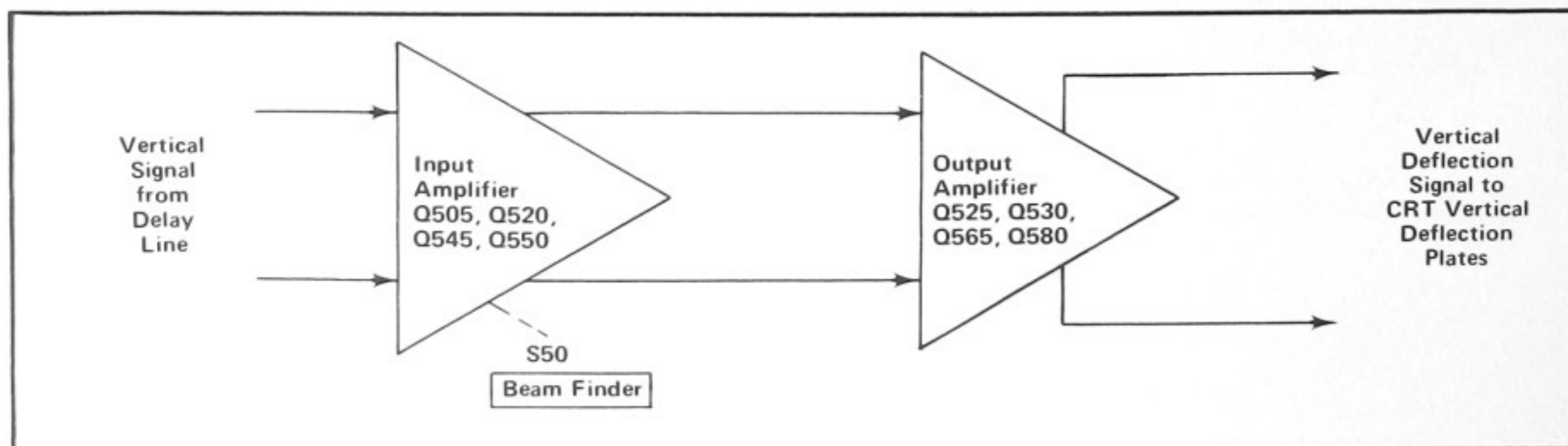
Fig. 3-7. Vertical Output Amplifier detailed block diagram.
