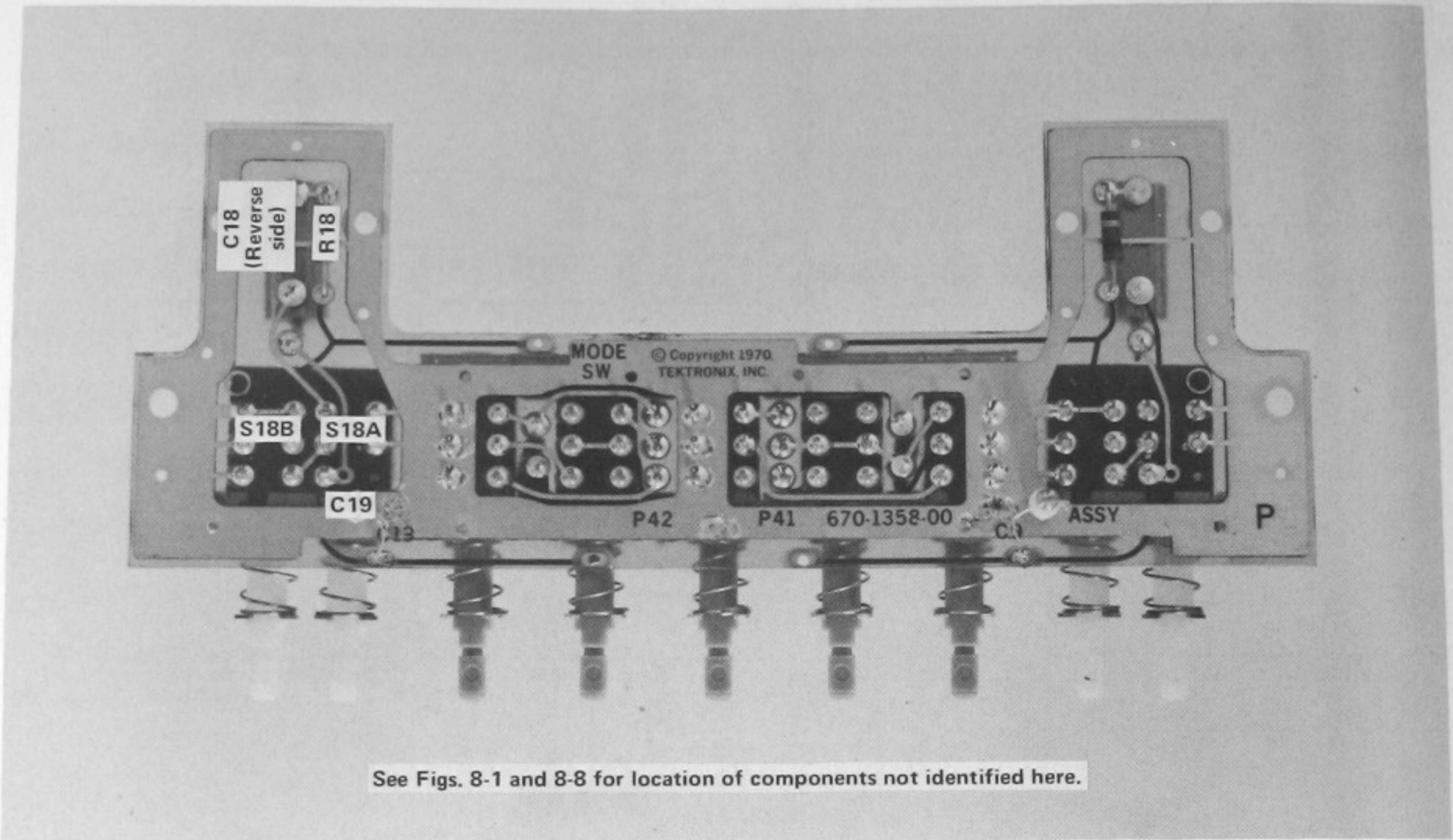
Fig. 8-4. P/O A3. Partial Vertical Mode Switch circuit board.
