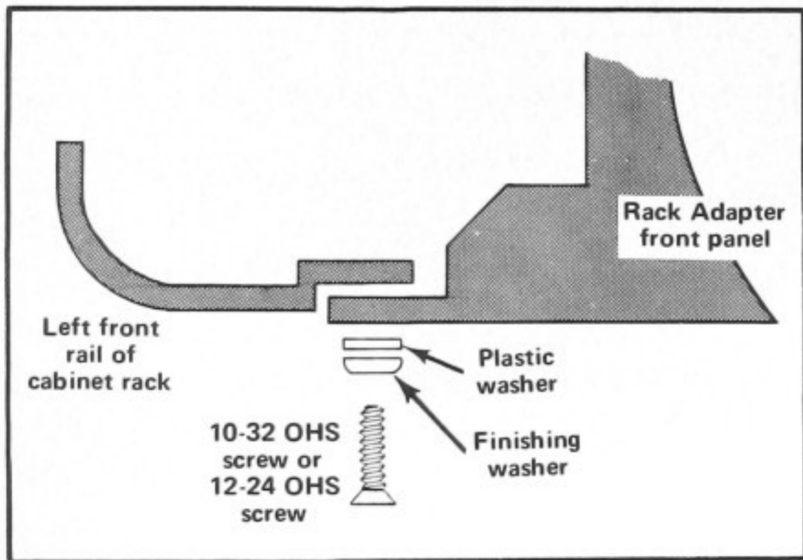
Fig. 6-3. Mounting the instrument to the front rails.
