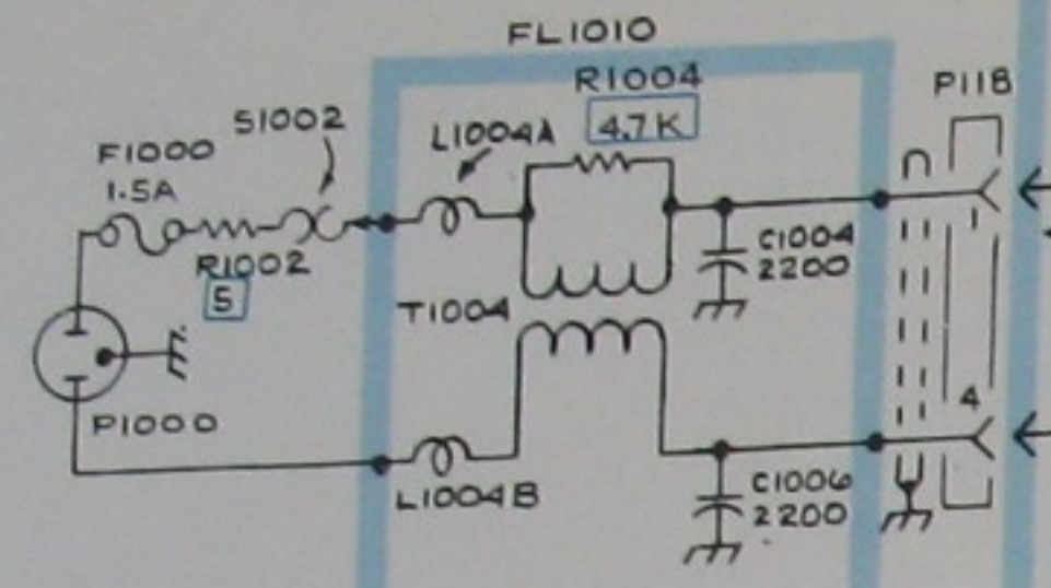
A13 LINE FILTER CKT BOARD
