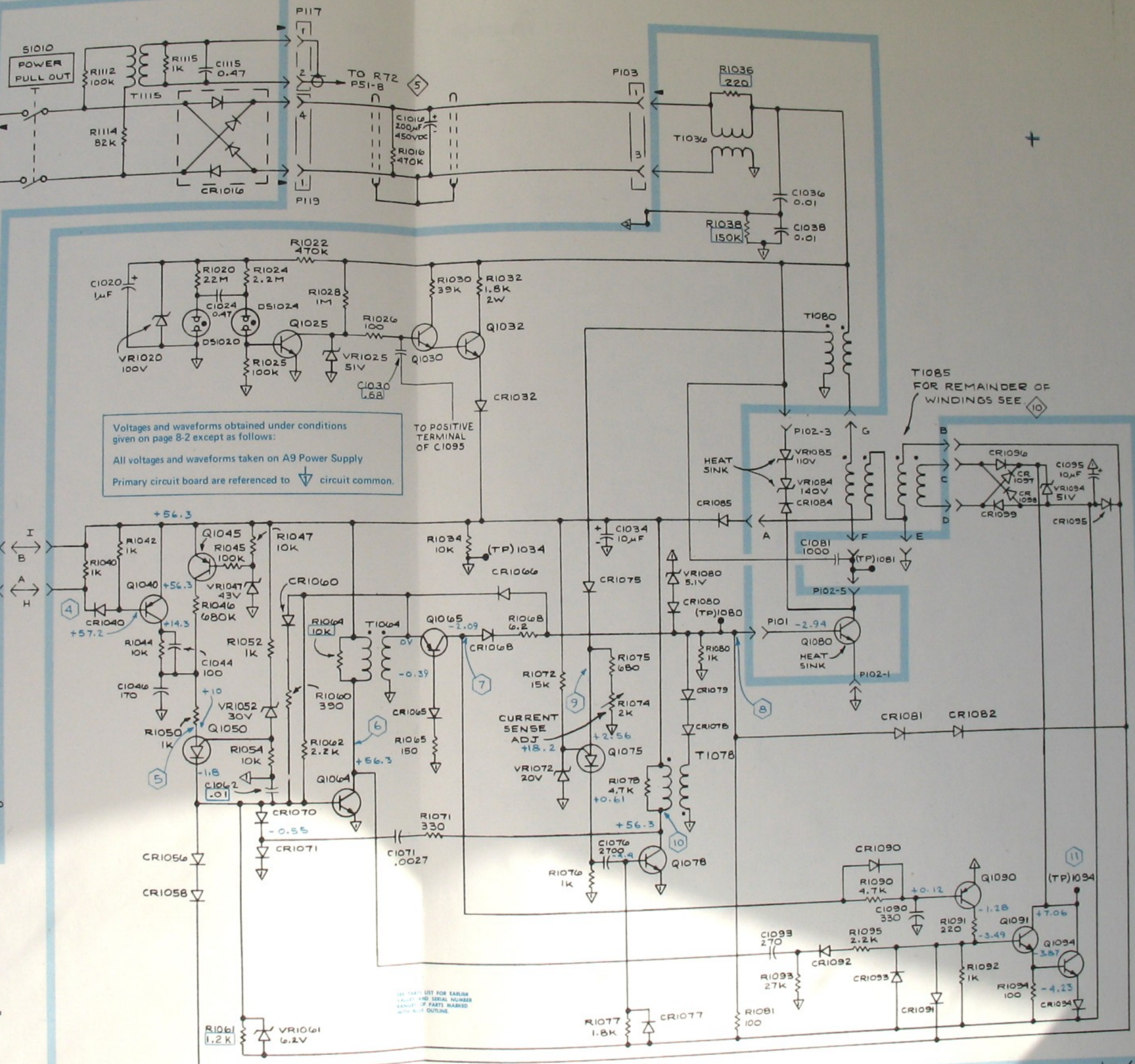
A9 POWER SUPPLY PRIMARY CIRCUIT BOARD
