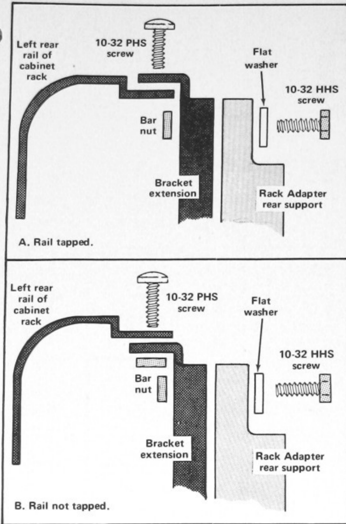
Fig. 6-4. Installing the rear bracket extensions.
