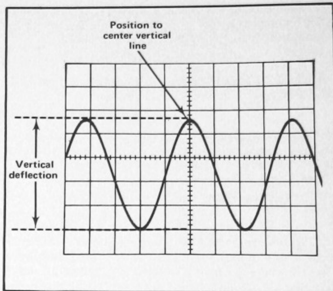
Fig. 2-7. Measuring peak-to-peak voltage of a waveform.
