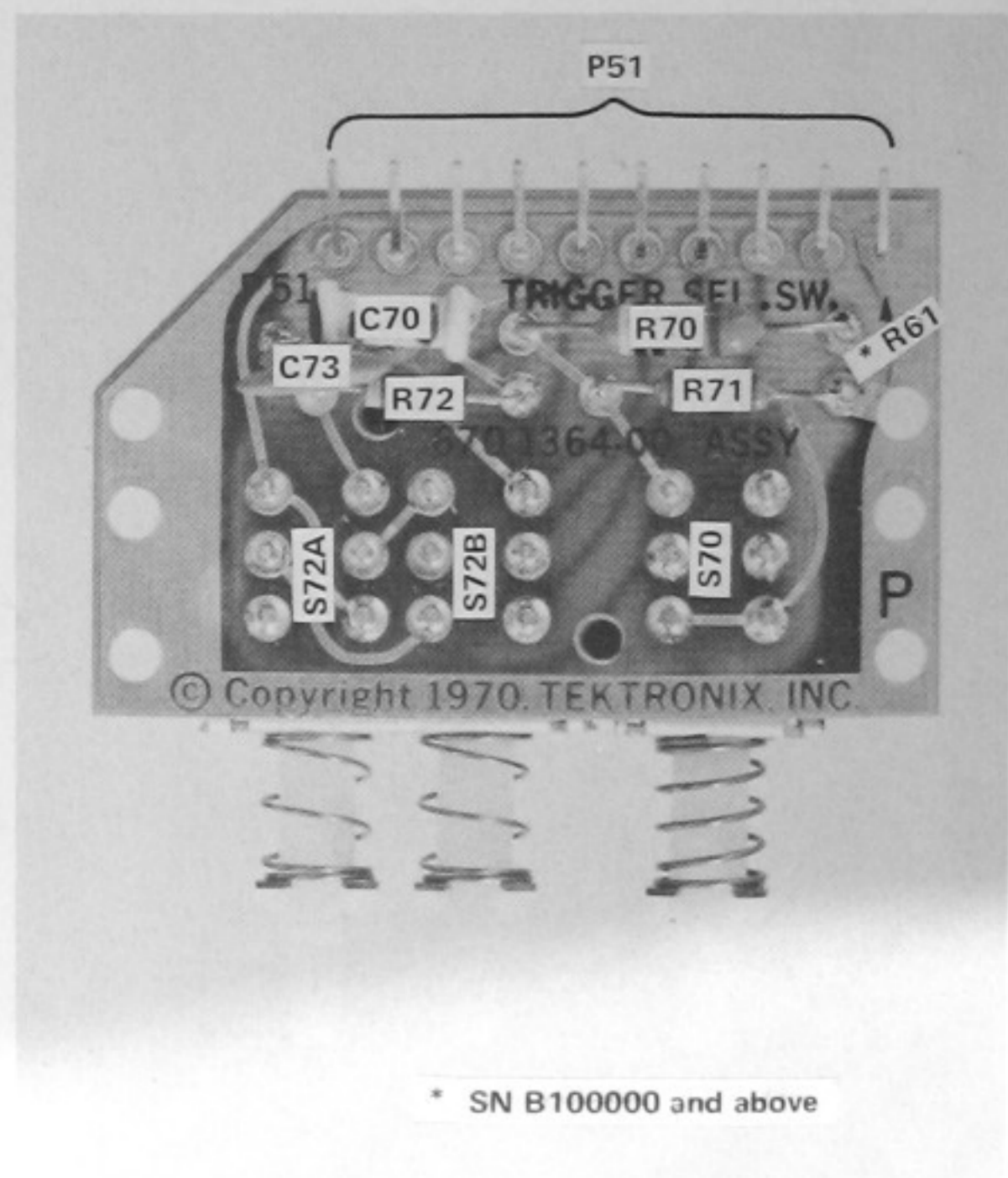
Fig. 8-12. A6. Trigger Source Switch circuit board. ©
