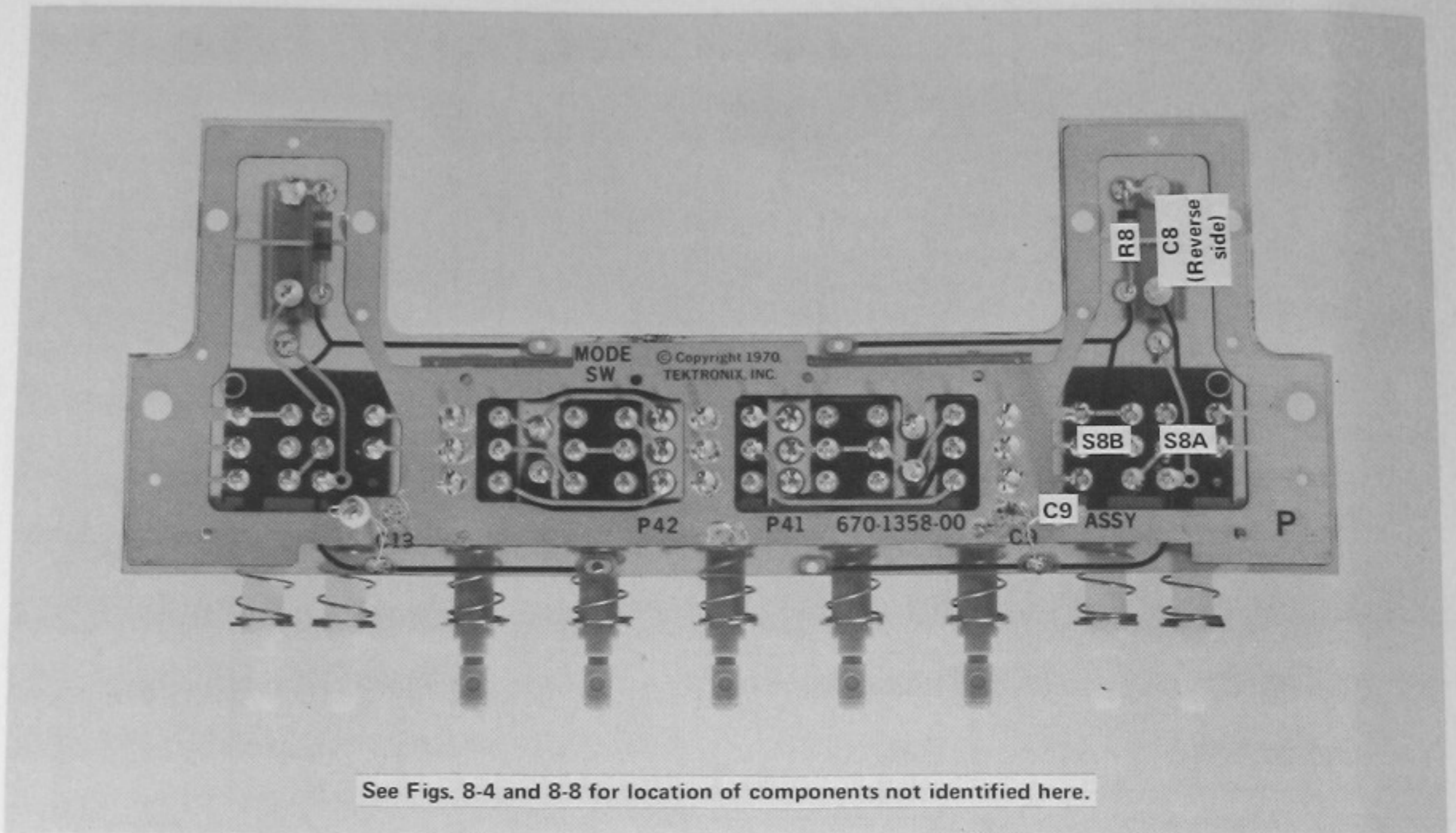
Fig. 8-1. P/O A3. Partial Vertical Mode Switch circuit board.
