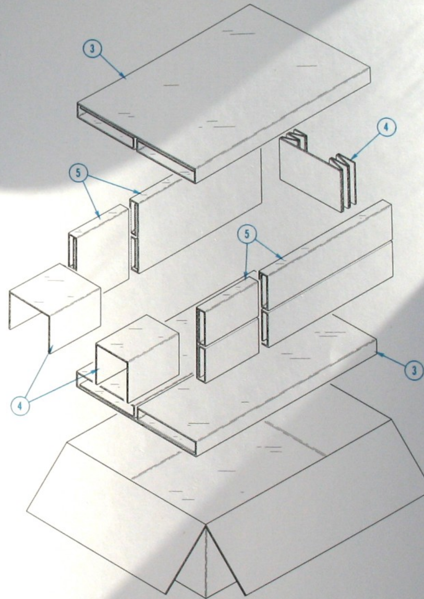
CARTON ASSEMBLY (Part No. 065-0157-00)
