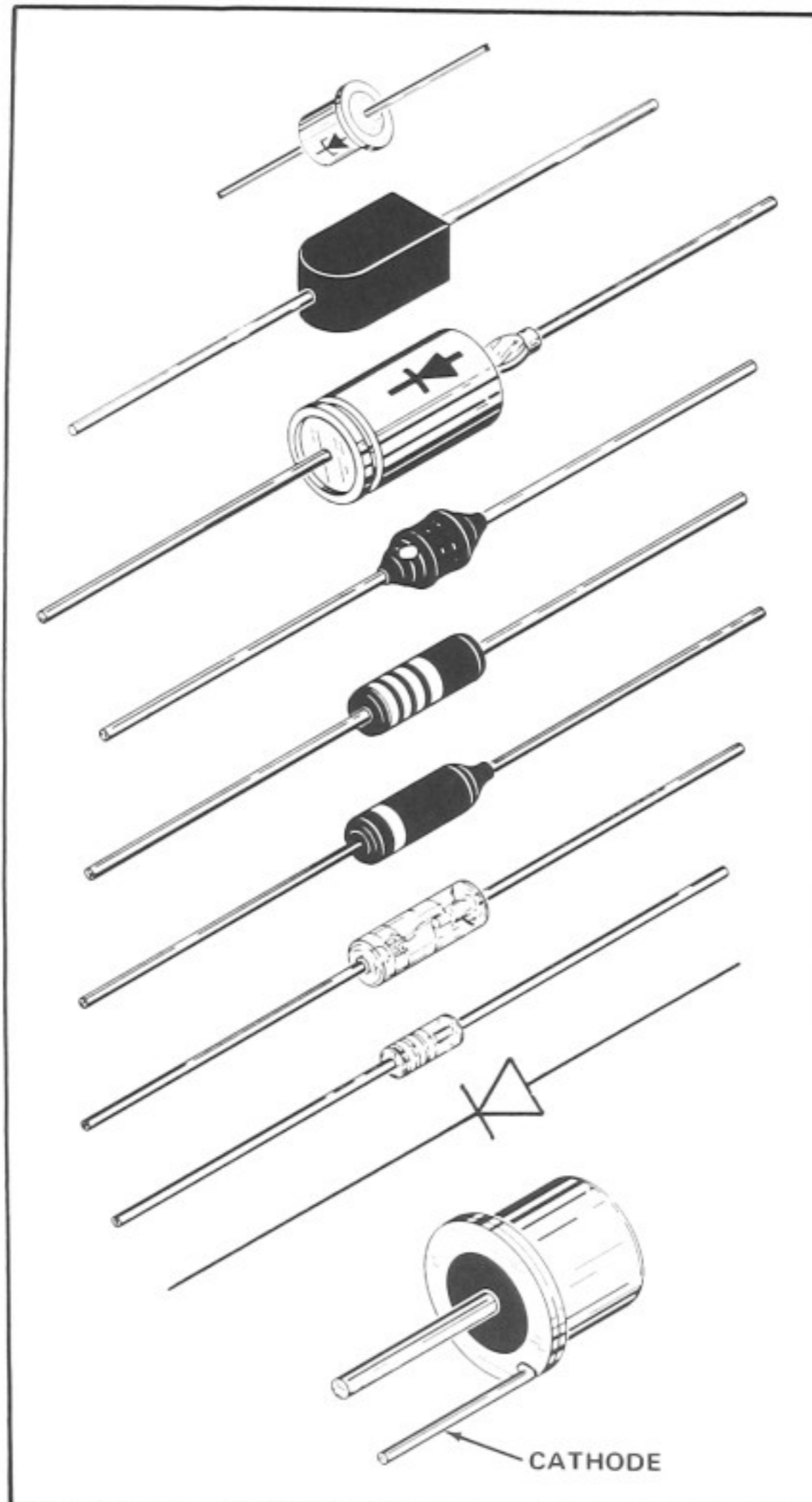
Fig. 4-3. Diode polarity markings.
