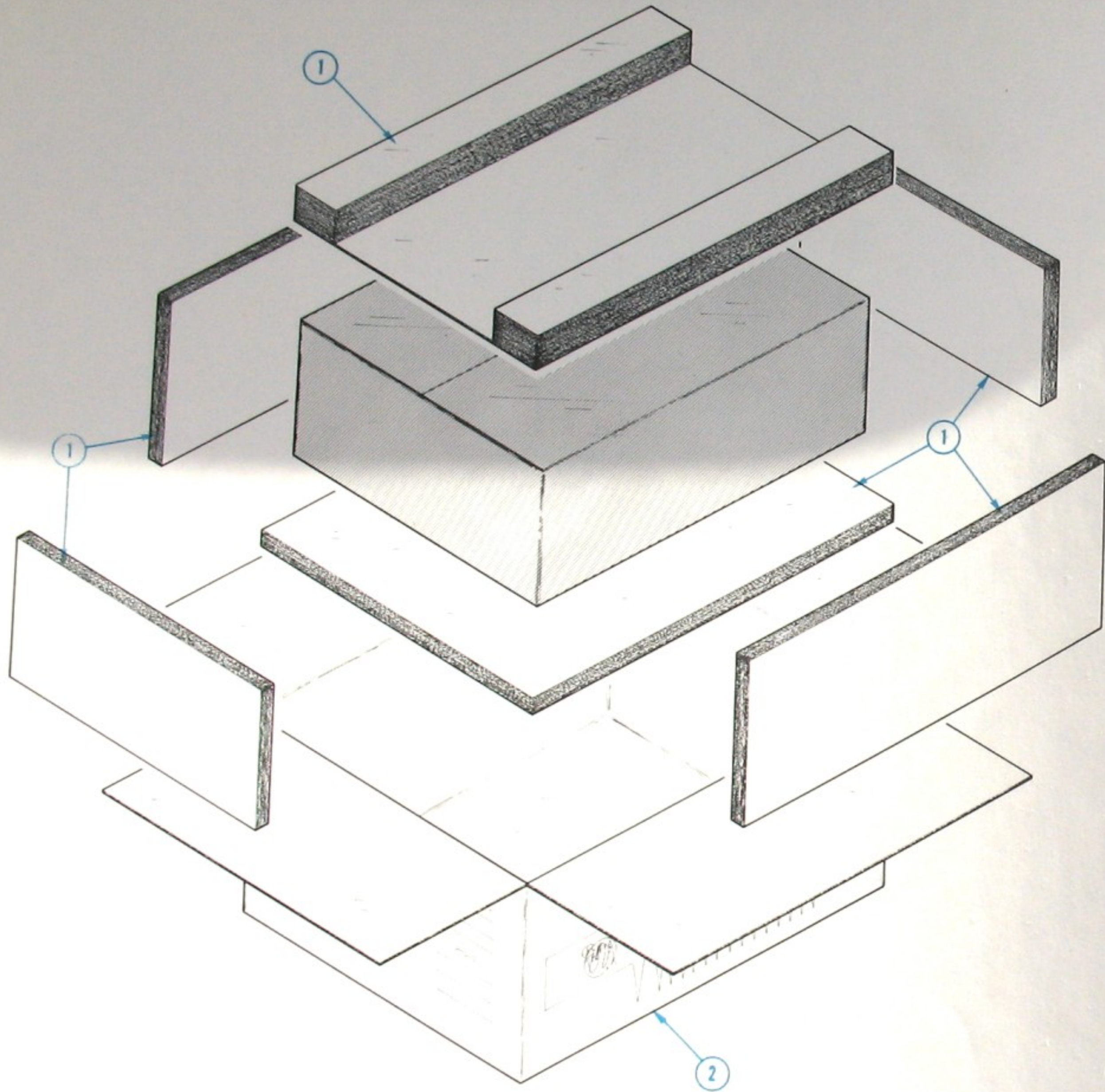
CARTON ASSEMBLY (Part No. 065-0157-00)
