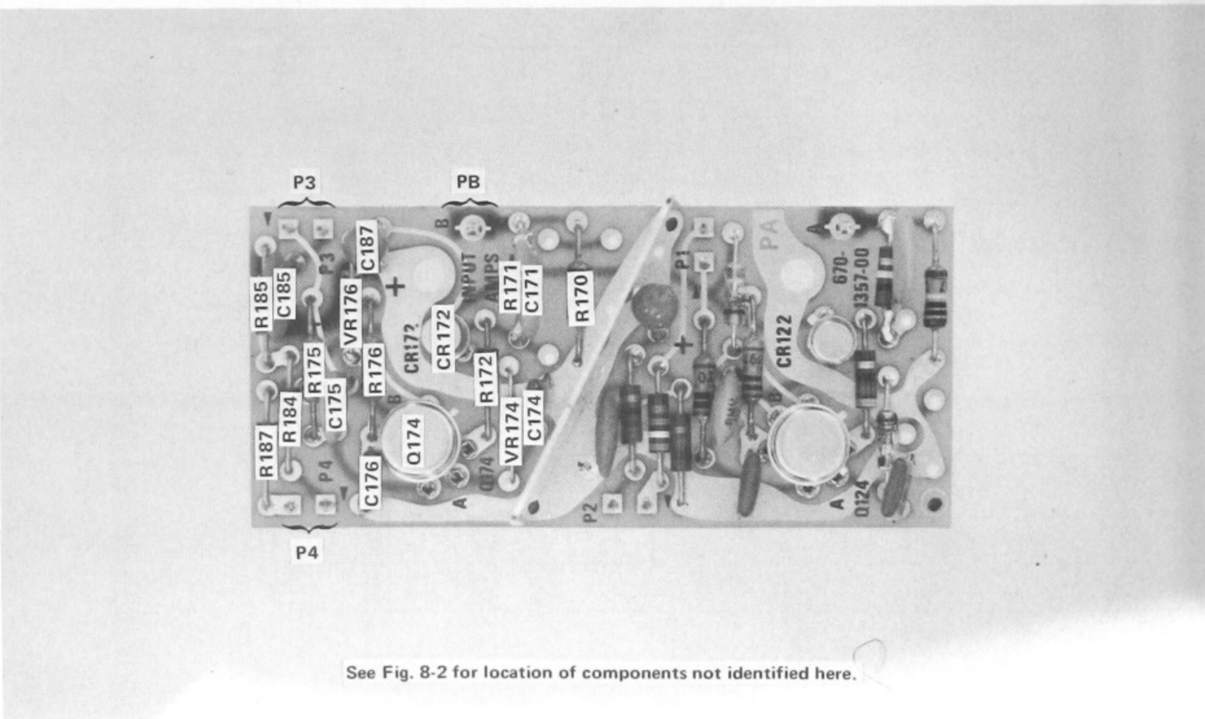
Fig. 8-5. P/O A1. Partial Input Amplifier circuit board.
