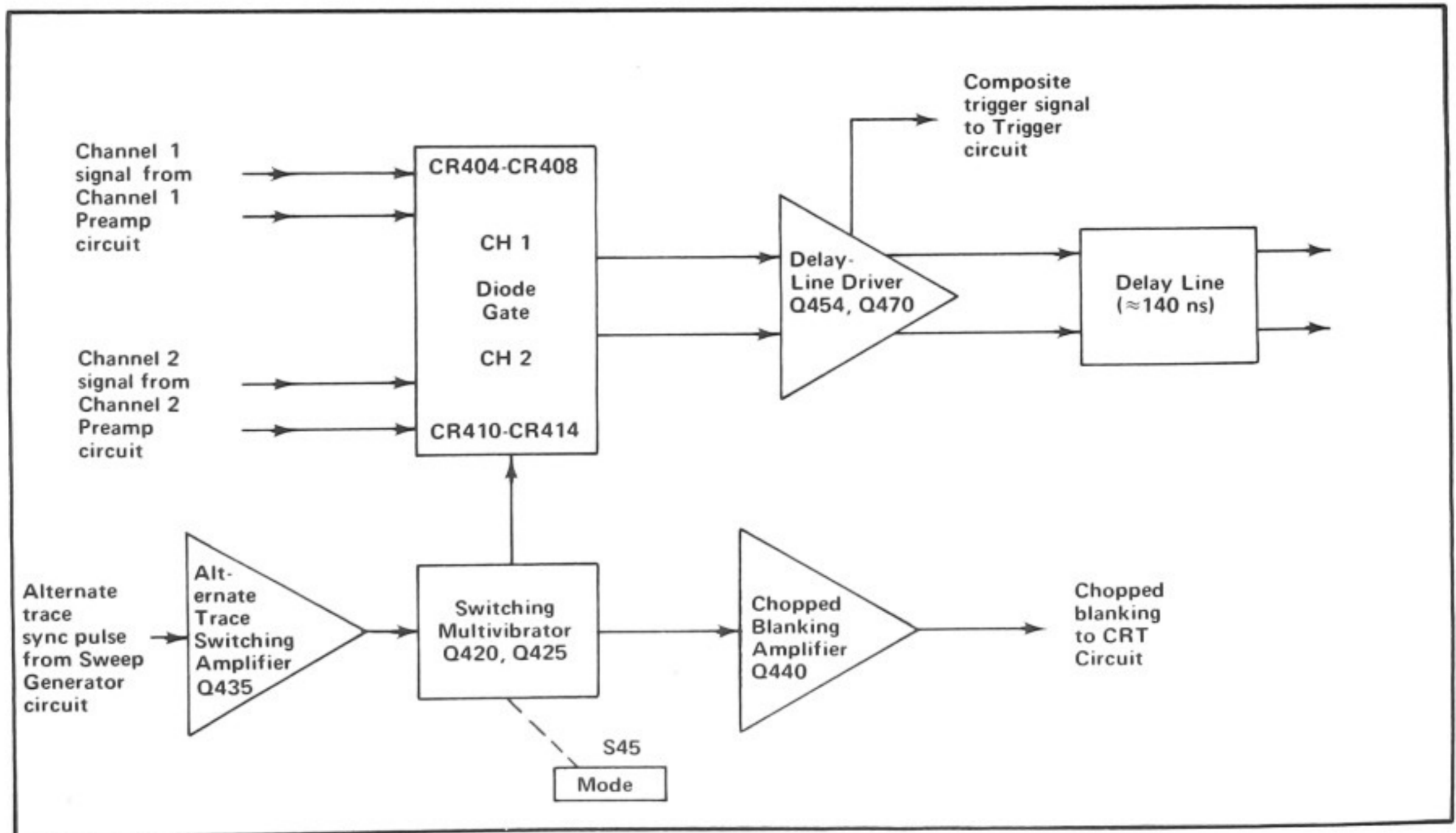
Fig. 3-4. Channel Switch detailed block diagram.
