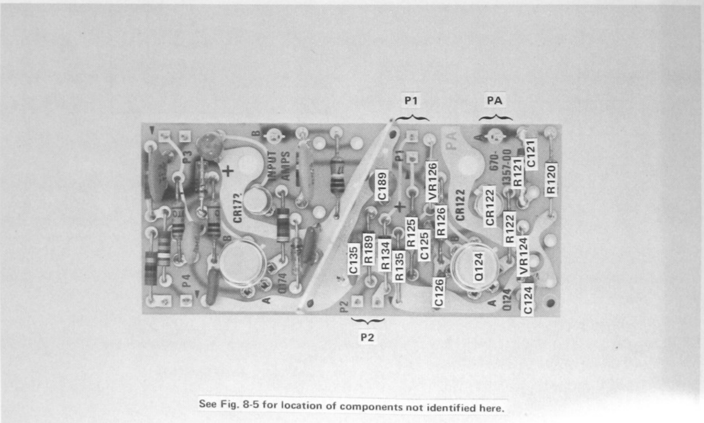
Fig. 8-2. P/O A1. Partial Input Amplifier circuit board.
