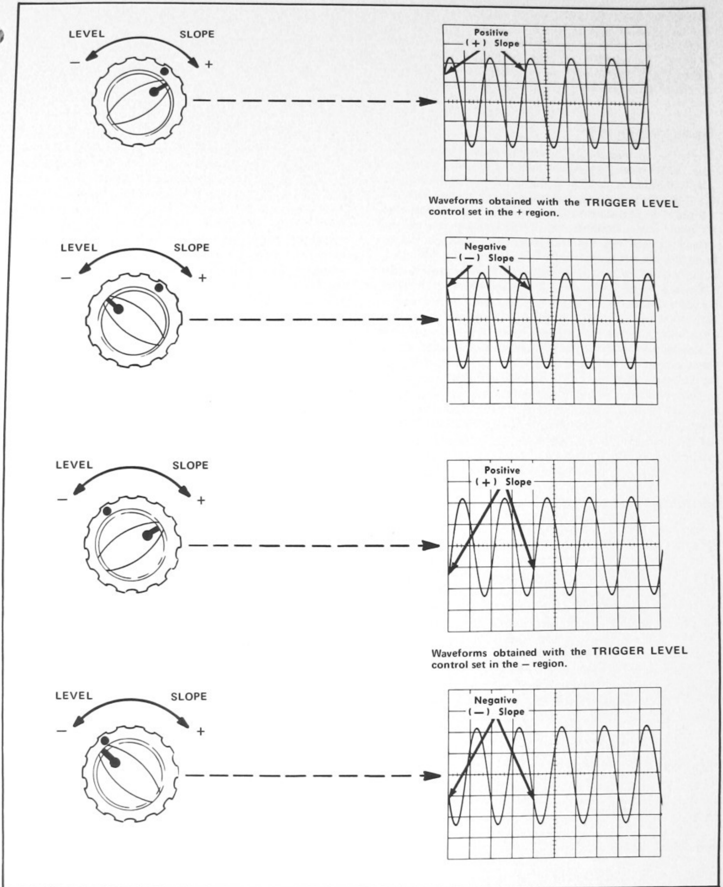
Fig. 2-6. Effect of the TRIGGER LEVEL control and SLOPE switch on the CRT display.
