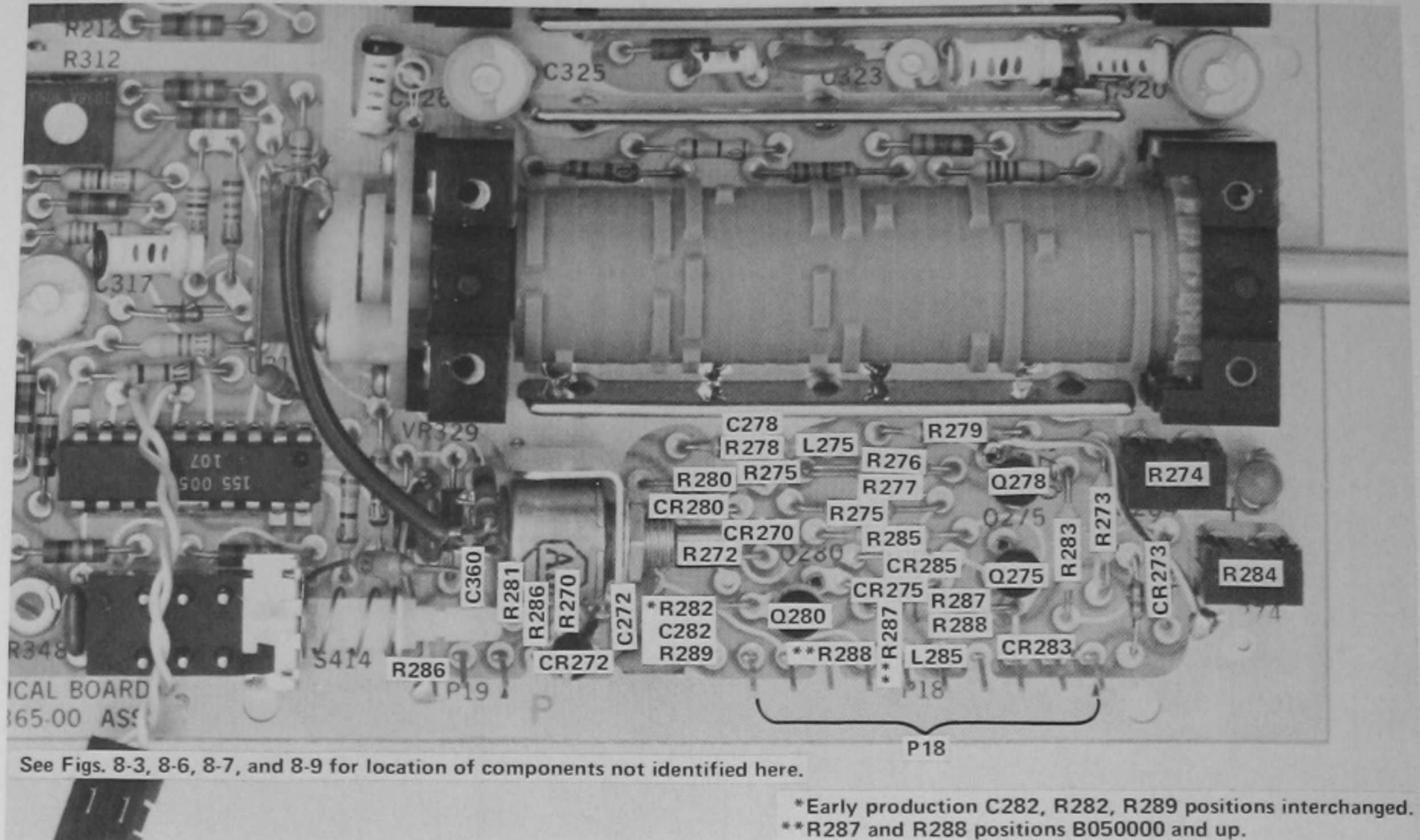
Fig. 8-10. P/O A2. Partial Vertical circuit board. ©
