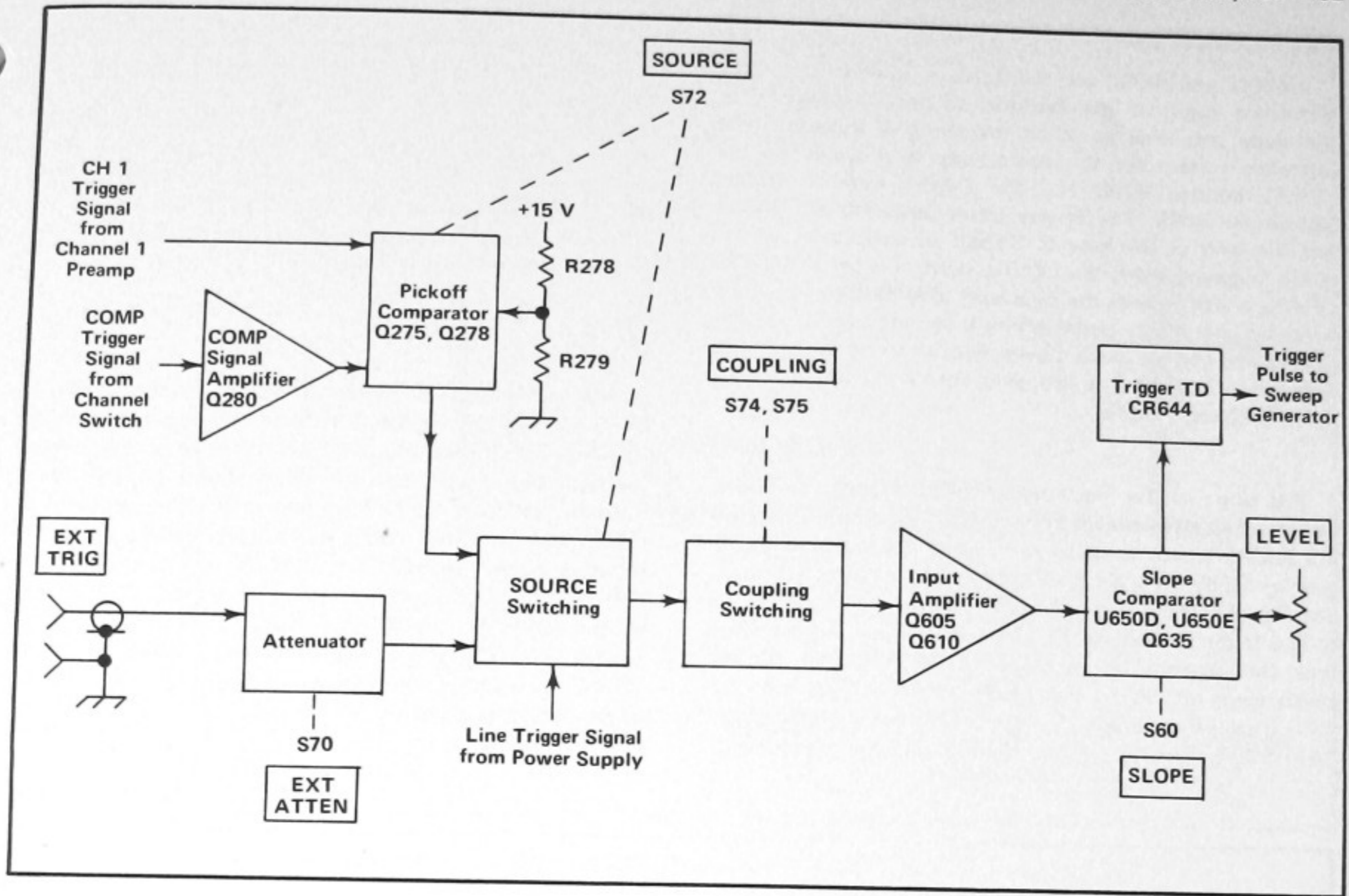
Fig. 3-8. Trigger Pickoff and Generator detailed block diagram.
