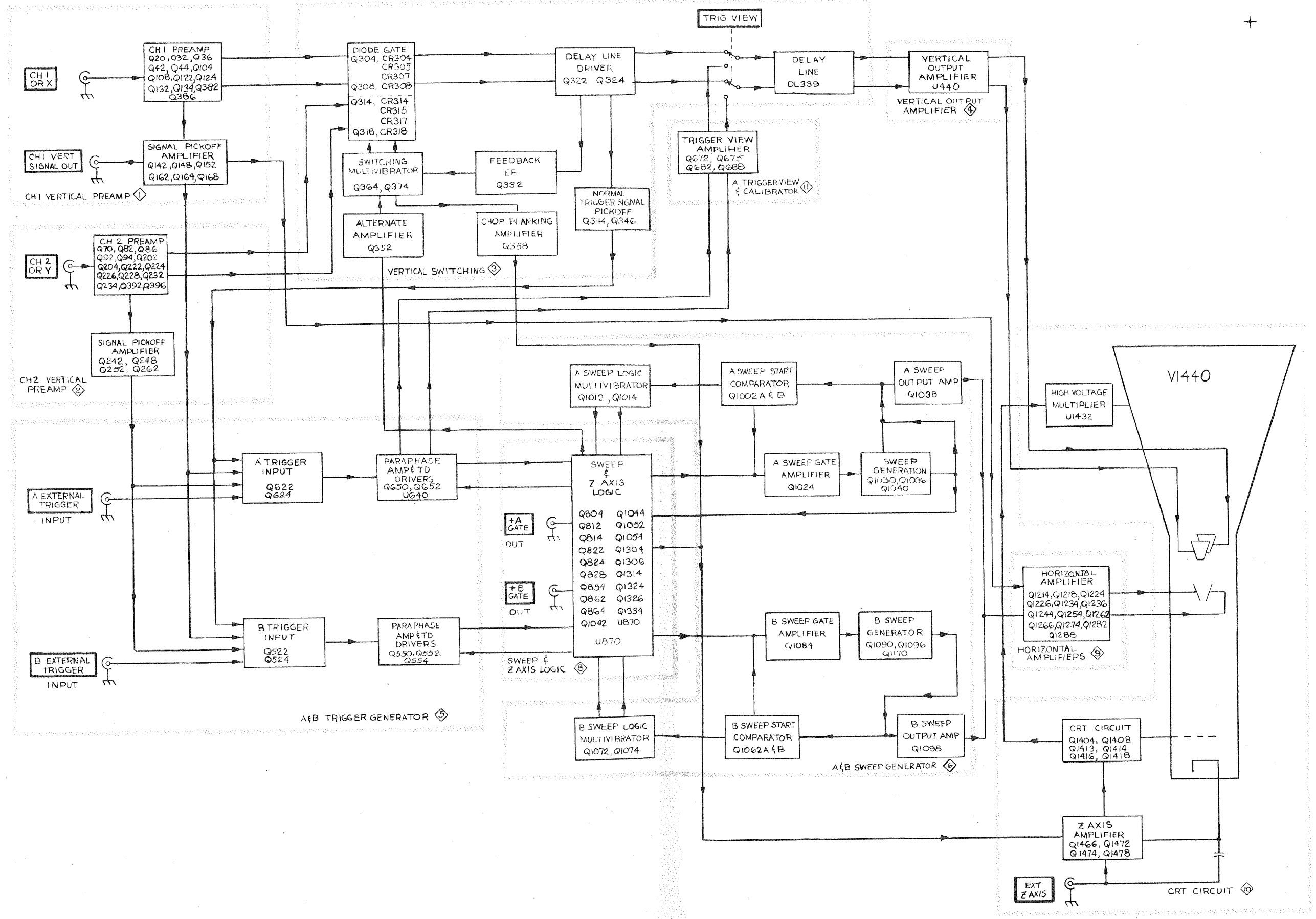
BLOCK DIAGRAM
