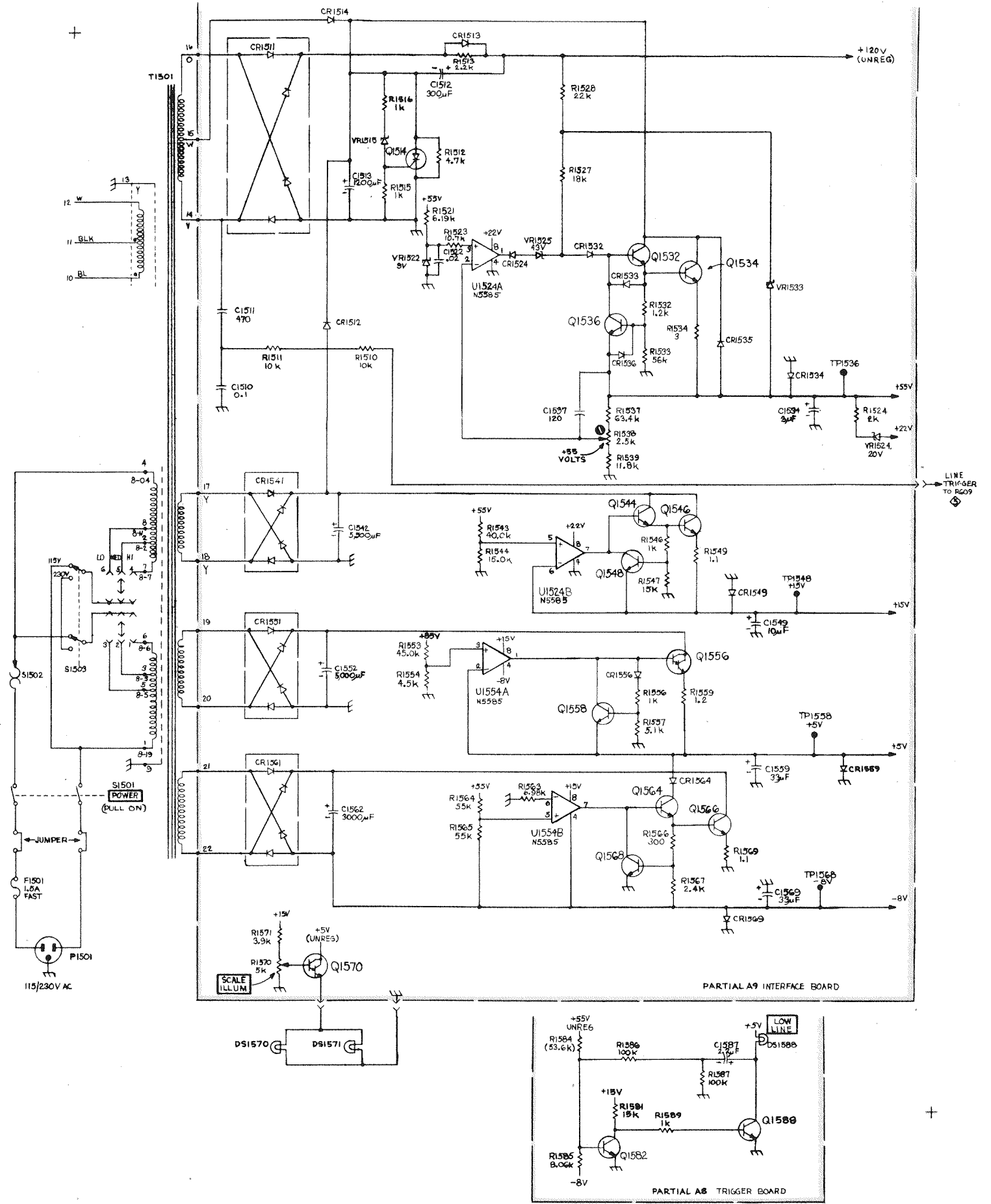
463 OSCILLOSCOPE
