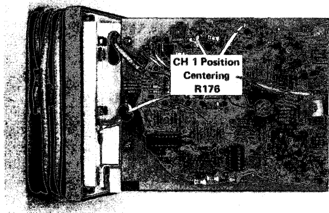
Fig. 5-9. Location of CH 1 Position Centering adjustment.
